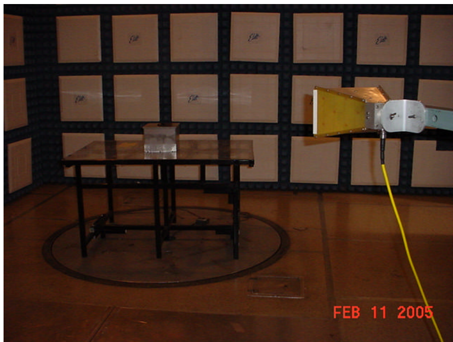
TEST SETUP FOR MEASUREMENT OF RADIATED EMISSIONS, HORIZONTAL POLARIZATION
