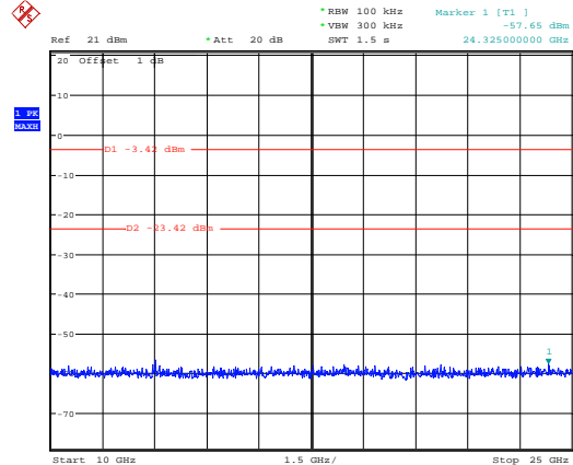
10GHz~25GHz
