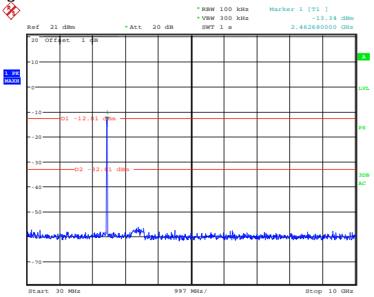
30MHz~10GHz
