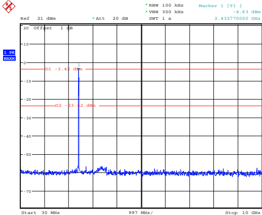
30MHz~10GHz
