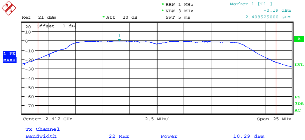
Lowest channel
