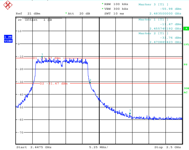
Highest channel
