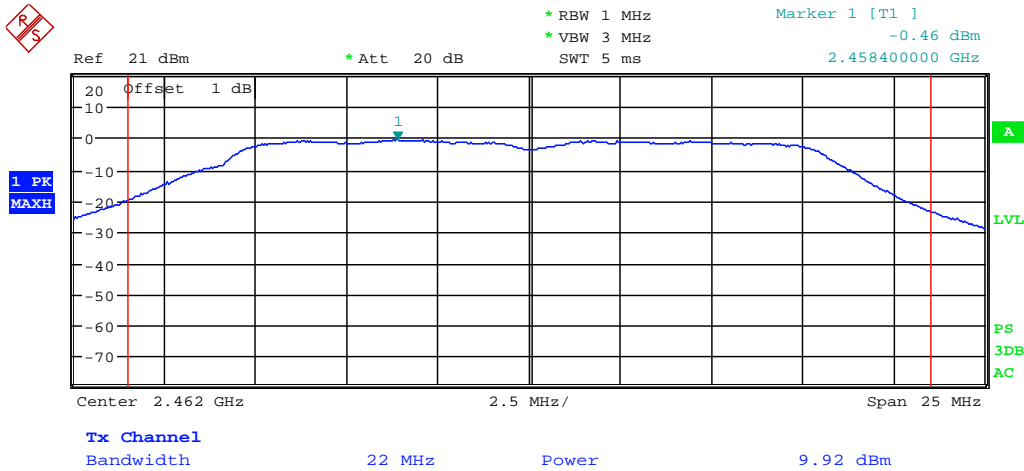
Highest channel
