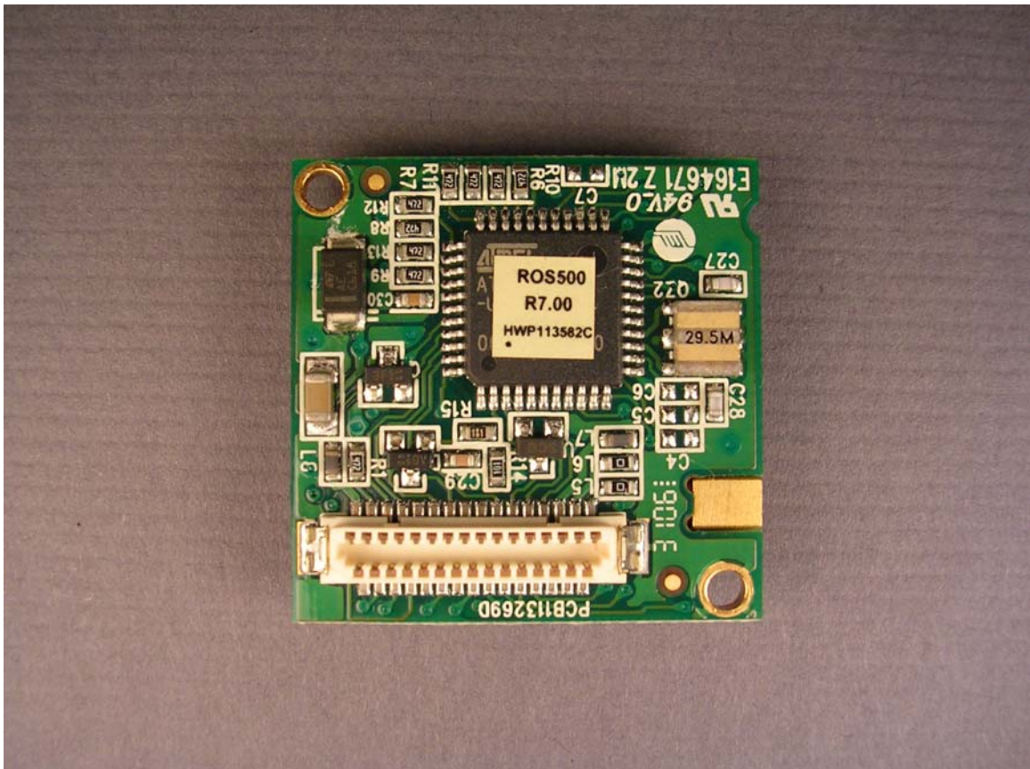
DataCard SCRDTX Internal Photo
