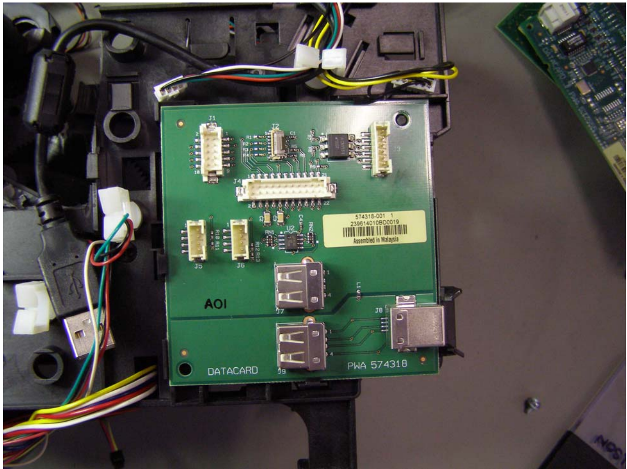
PWA USB Front
