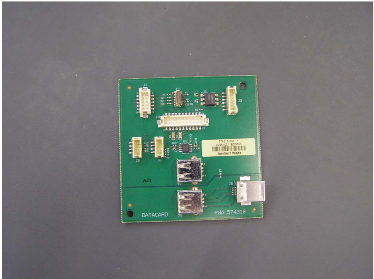
PWA USB Front – alternate view of board removed from unit
