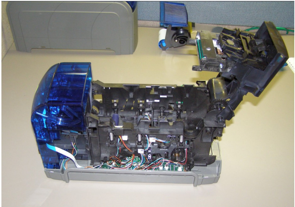
RIGHT SIDE INTERNAL VIEW
