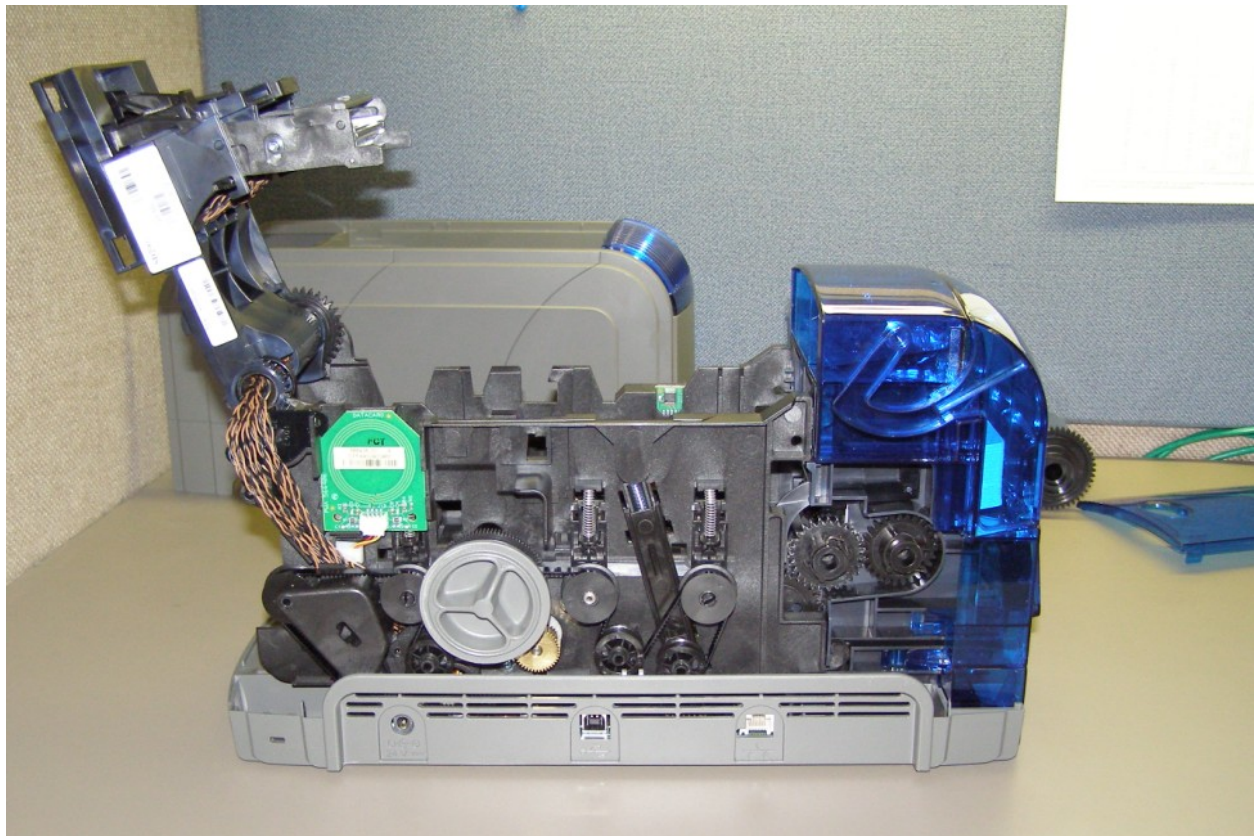
RIGHT SIDE INTERNAL VIEW
