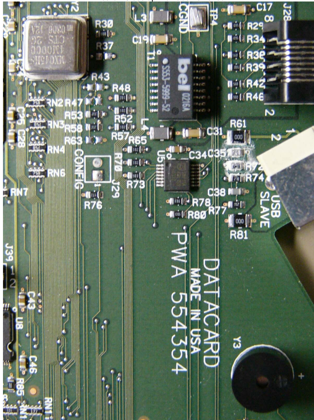
Board - Close up with label removed
