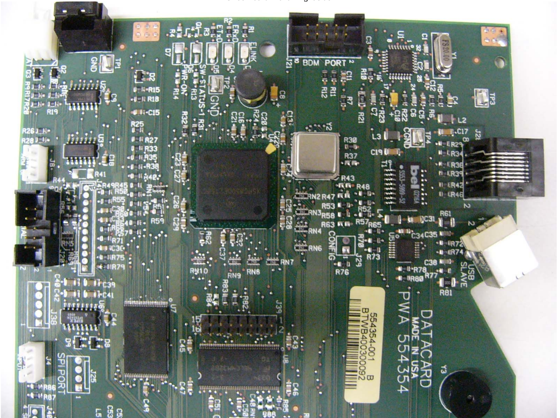
SP55 Board Front - Right side
