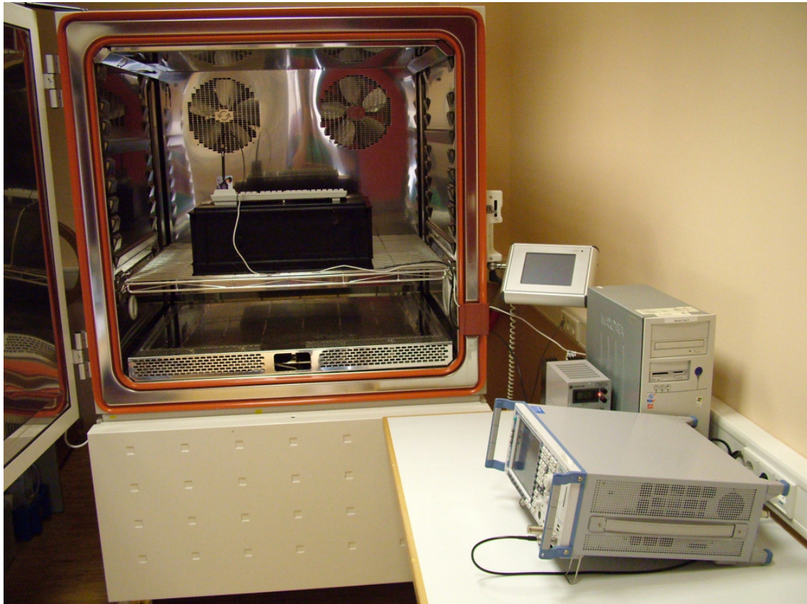
Picture 15-6: Carrier frequency stability test setup
