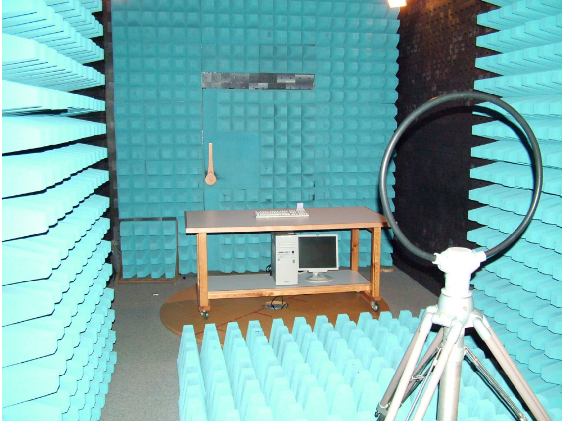
Picture 15-5: Occupied bandwidth setup
