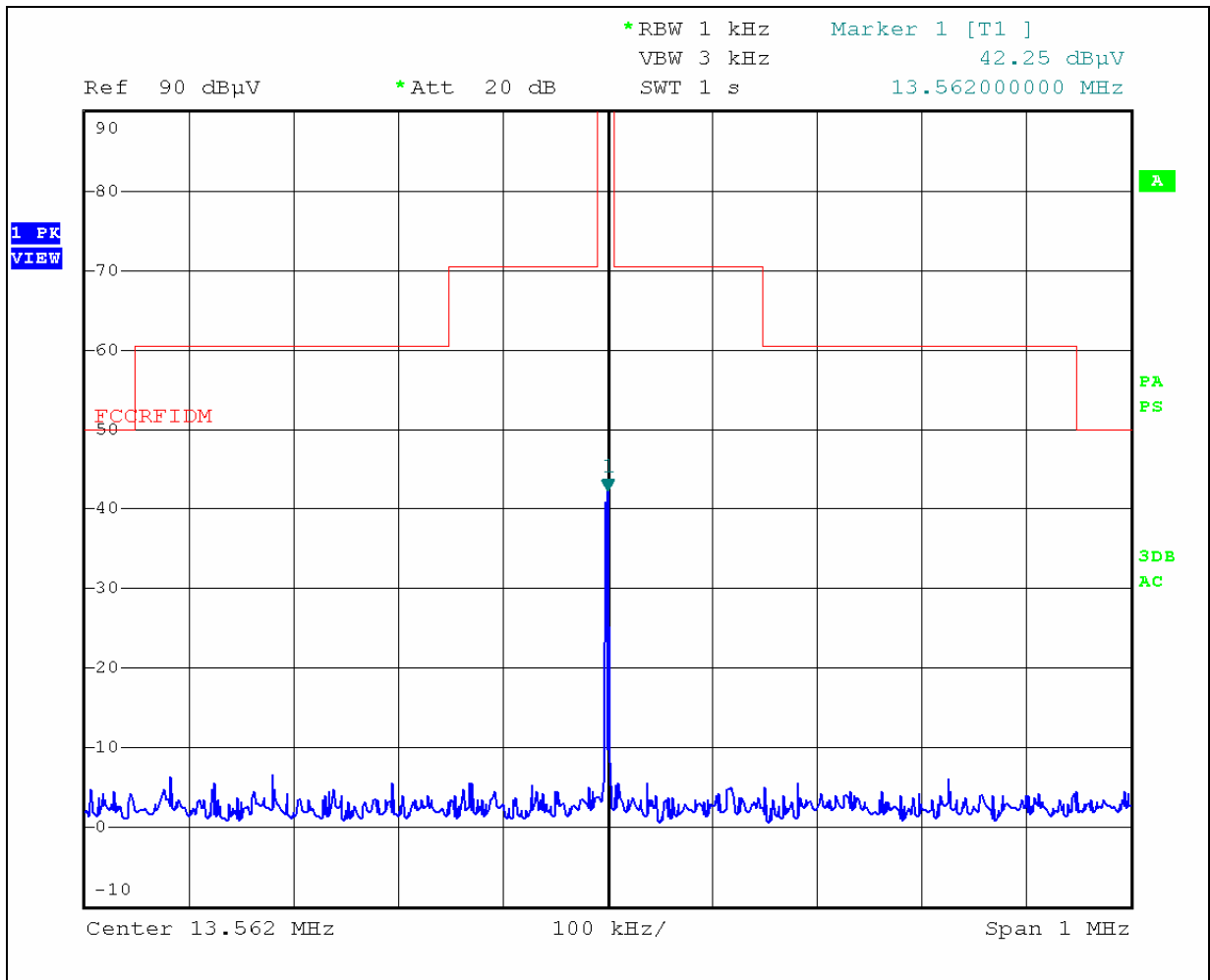
Picture 4-1:Result of spectrum mask measurement
