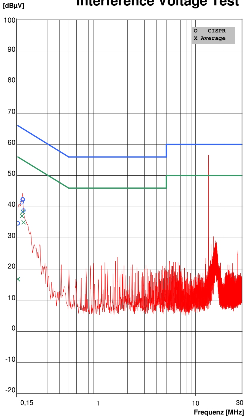
Diagram 5-1: Conducted emission on phase
