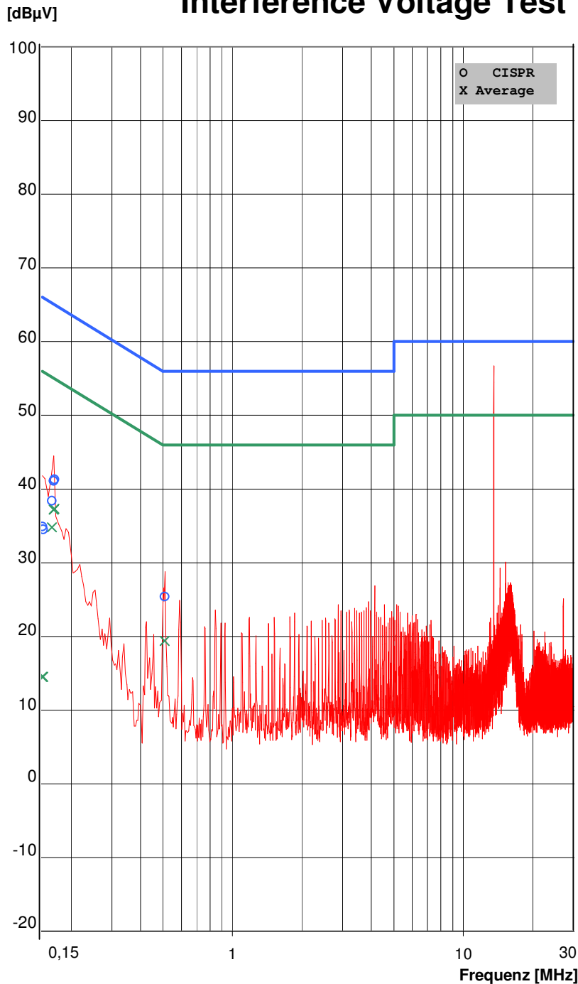
Diagram 5-3: conducted emission on neutral
