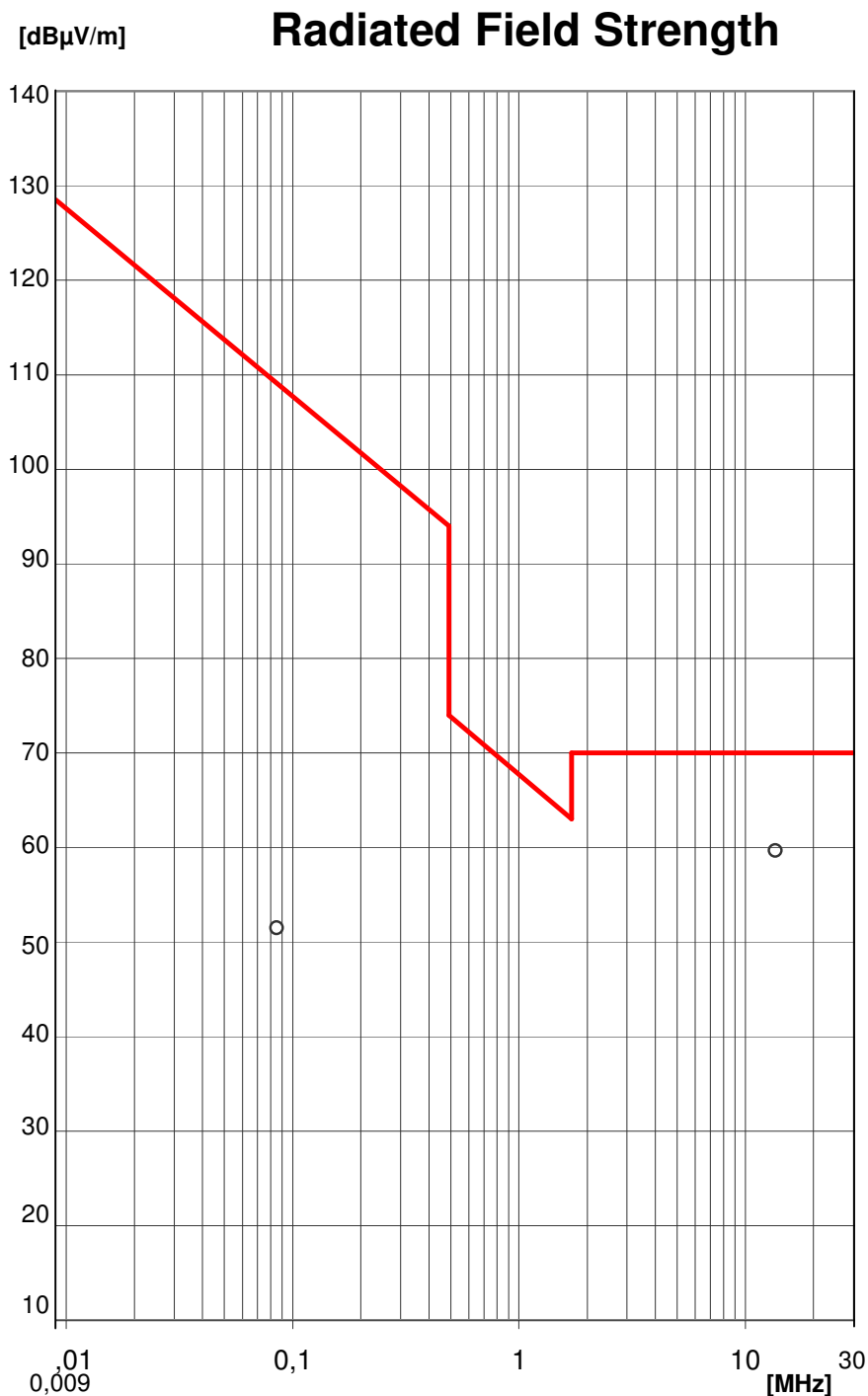
Picture: 6-2 Radiated field strength 0,009 MHz – 30 MHz (final)
