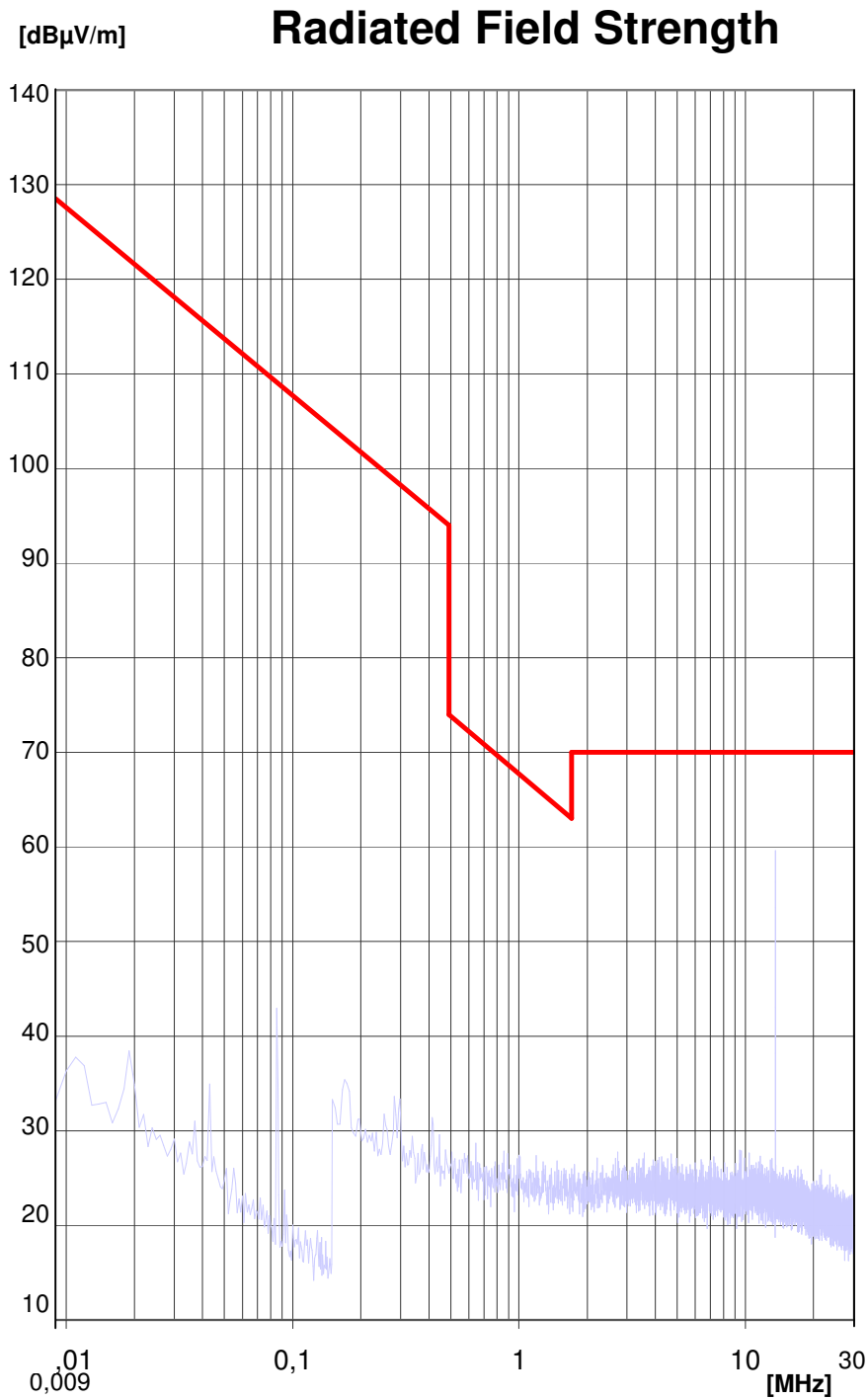
Picture: 6-1 Radiated field strength 0,009 MHz – 30 MHz (pre scan)
