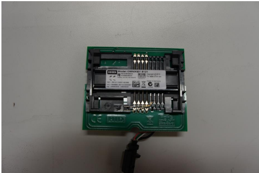
Picture 3: PCB top side
