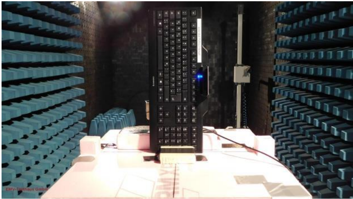
Picture 9: EUT-position 3
