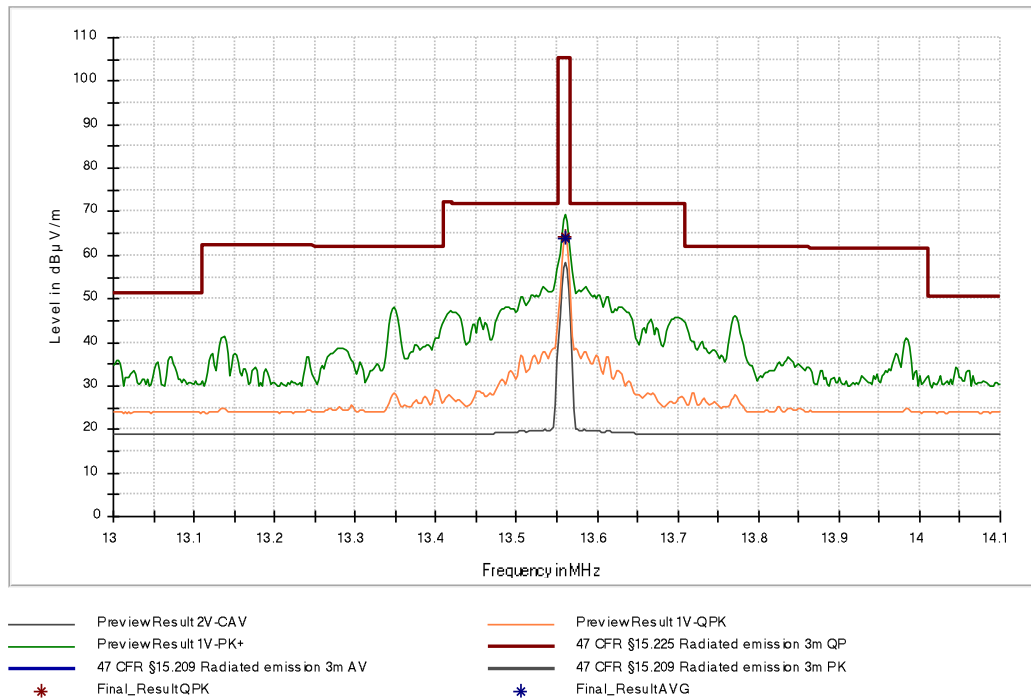
Figure 11: Chart of emission within the band 13.110 MHz to 14.010 MHz, without tag, position 3, antenna in line at 3m distance
