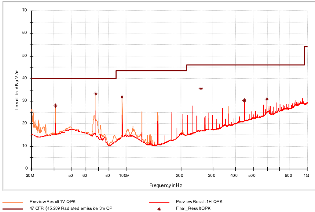
Figure 13: Chart of emissions test from 30 MHz to 1 GHz with tag in position 1 at 3 m
