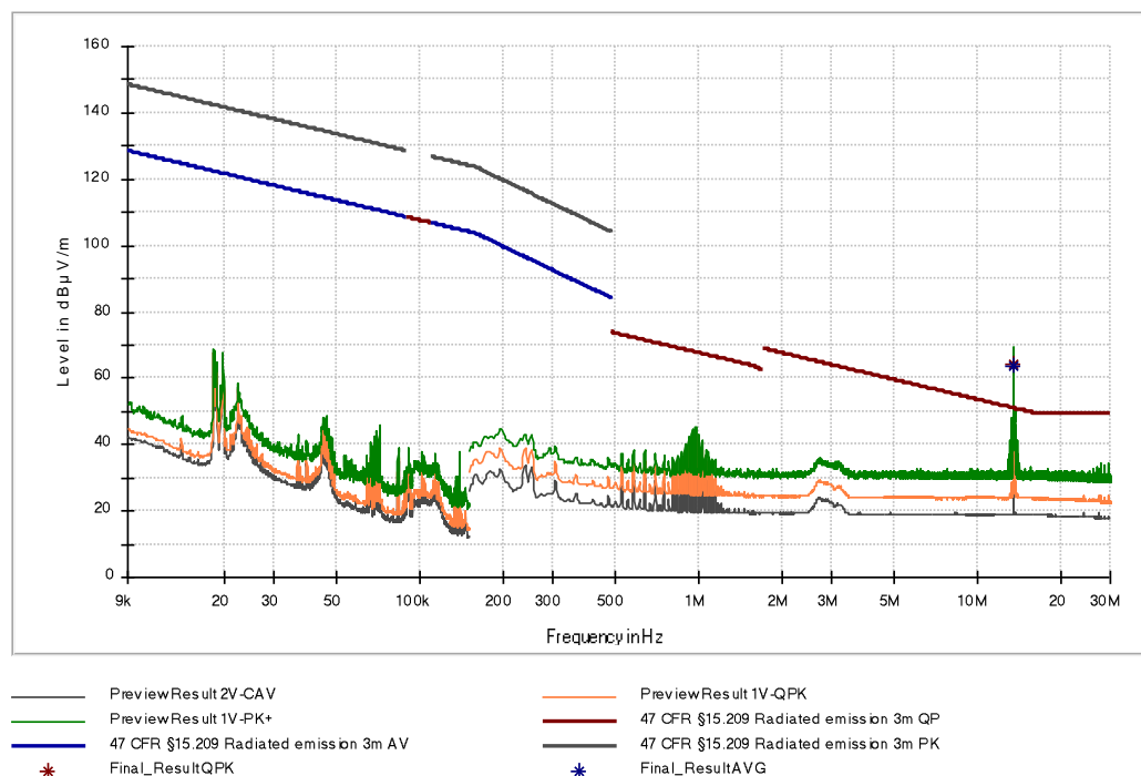
Figure 12: Chart of emissions test below 30 MHz without tag in position 3, antenna in line at 3 m
