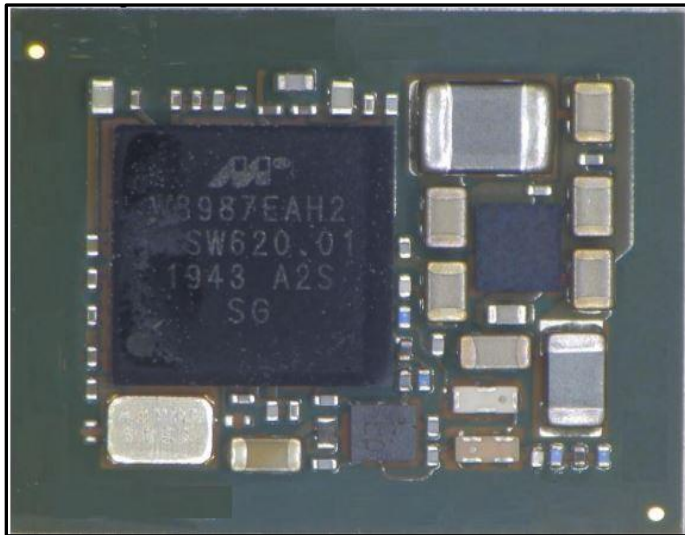
Module interior photo with top removed
