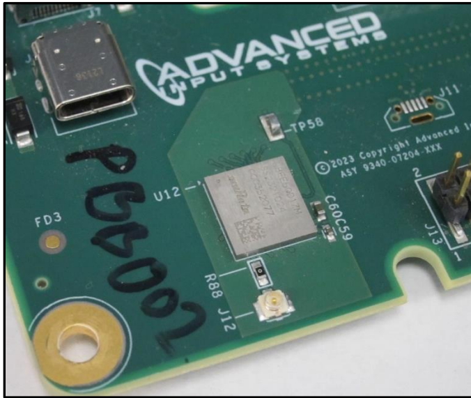
Radio module (U12) on PCB and antenna connection port (J12)
