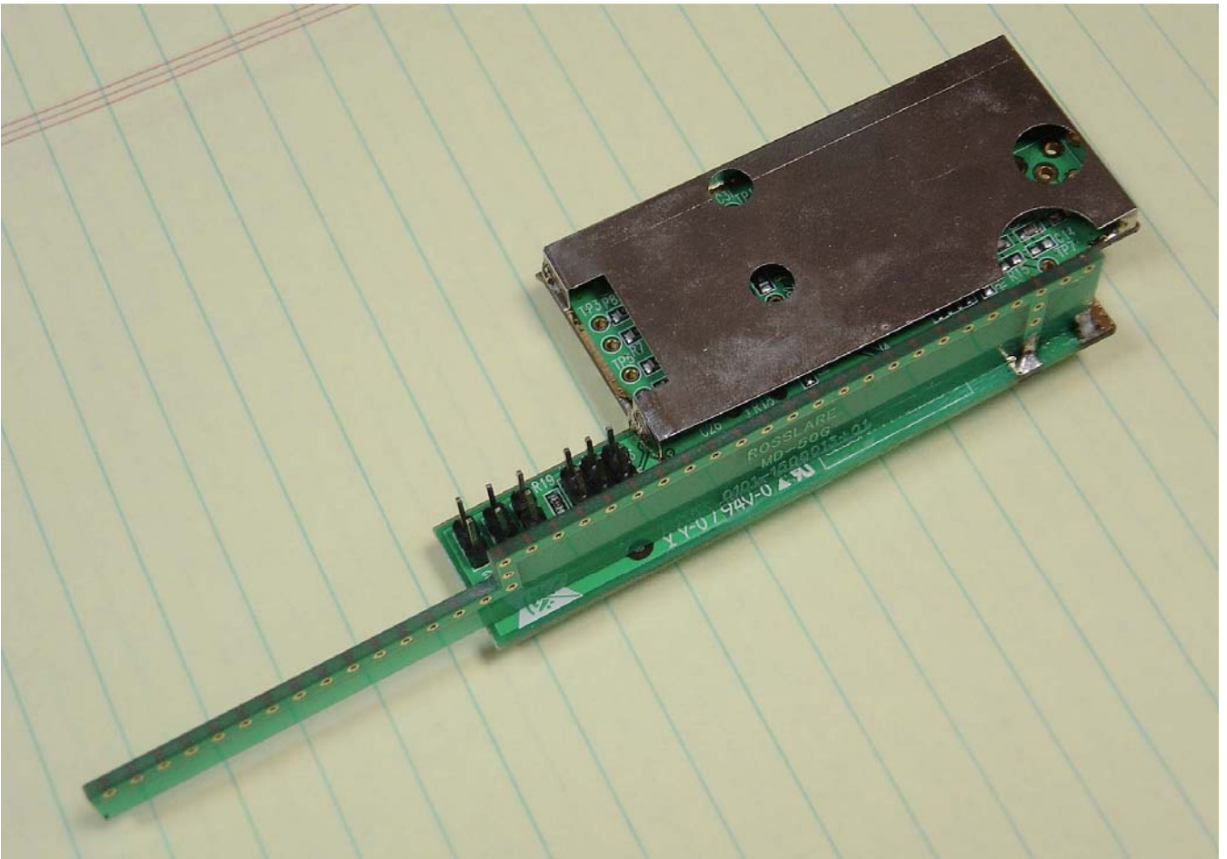
SP-N6G RF Module Board Top with Shield
