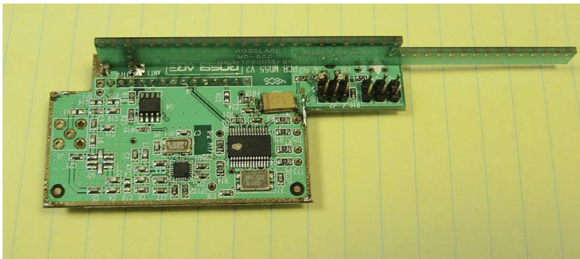
SP-N6G RF Module Board Top without Shield
