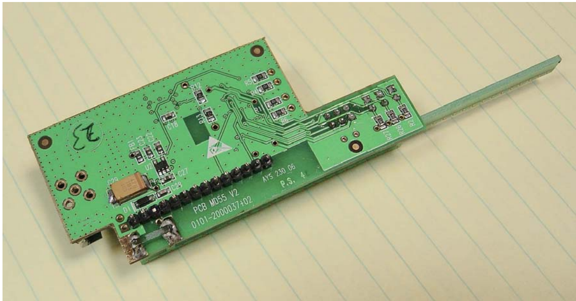
SP-N6G RF Module Board Bottom
