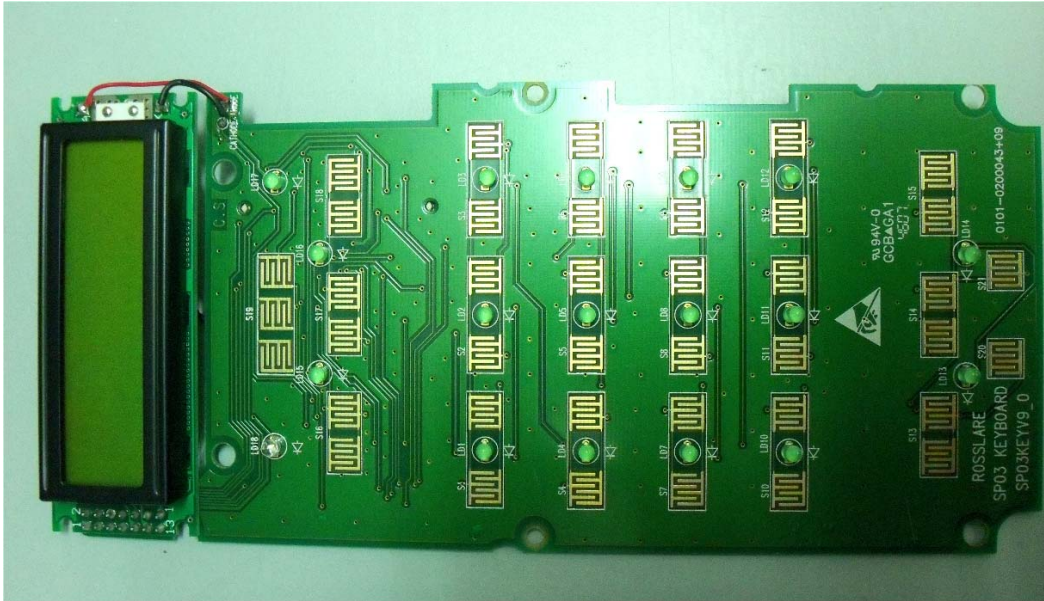
Photograph No.12 SP-03V2G keyboard PCB second side view
