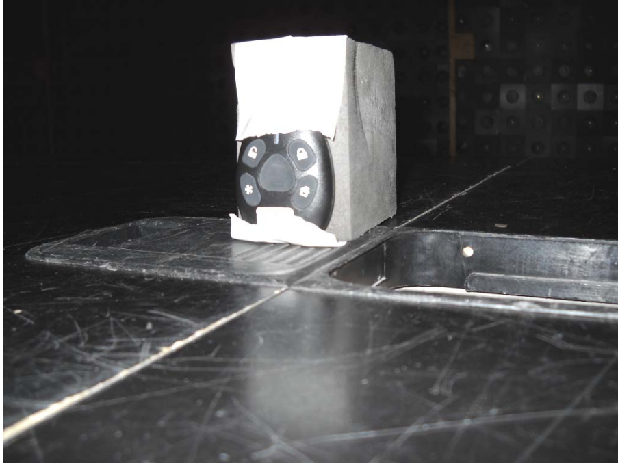
Photograph No.4 Setup for radiated emission measurements in the anechoic chamber, EUT close view
