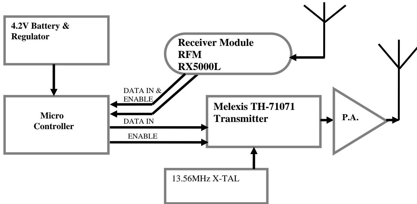
SA-29G WIRELESS REPEATER POWER DISTRIBUTION DIAGRAM
