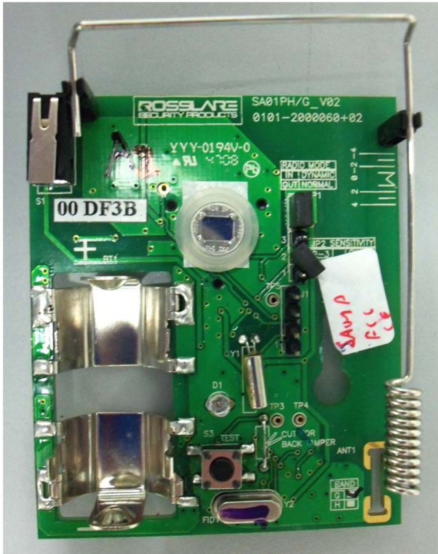
Photograph No.4 PCB top view
