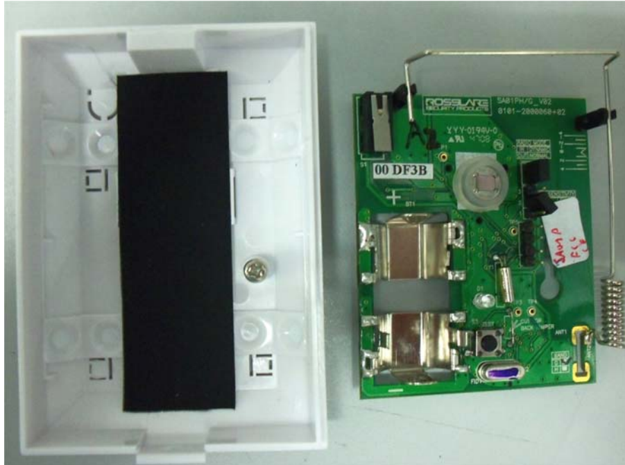
Photograph No.3 SA-01PG PIR detector internal view
