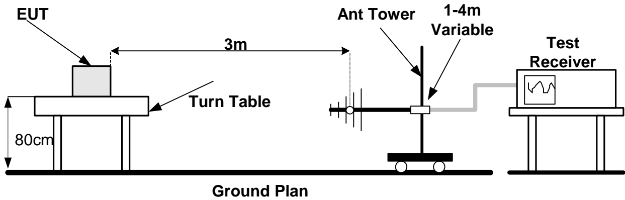
Figure 2: Radiated Emission Set up
