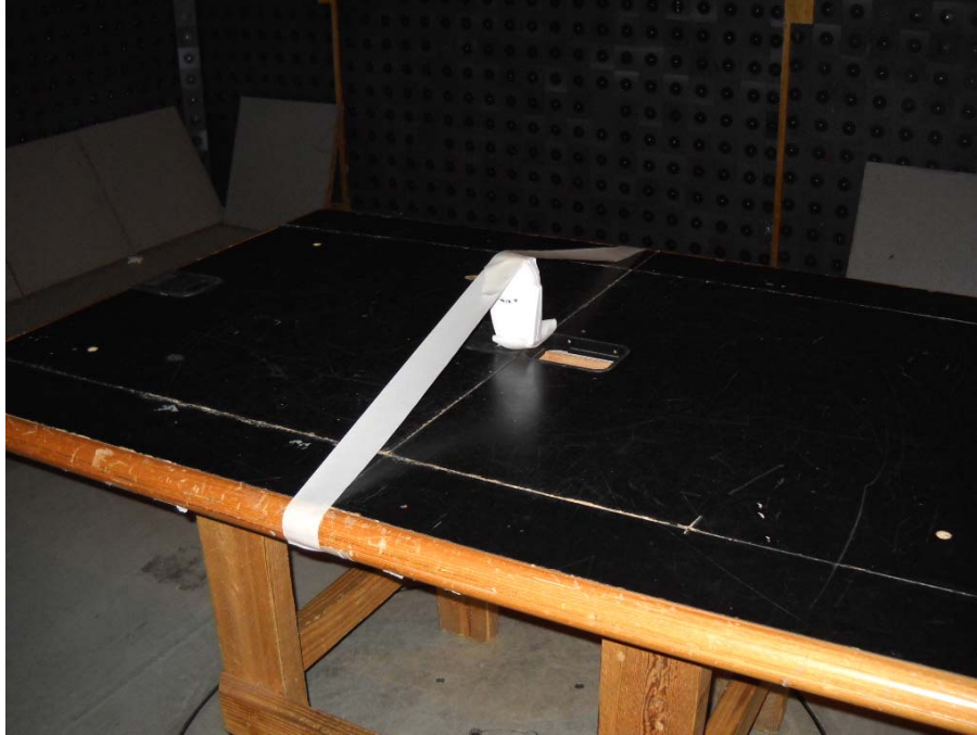
Photograph No.3 Setup for radiated emission measurements in the anechoic chamber, EUT close view
