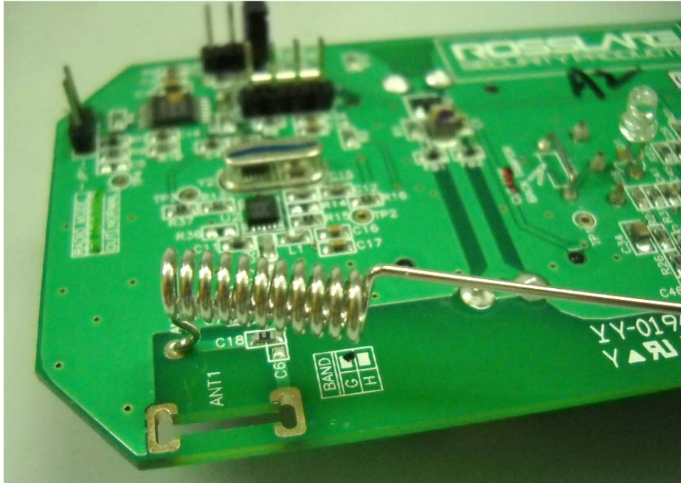
Photograph No.5 Antenna close view
