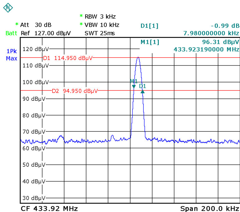
Test Plot
