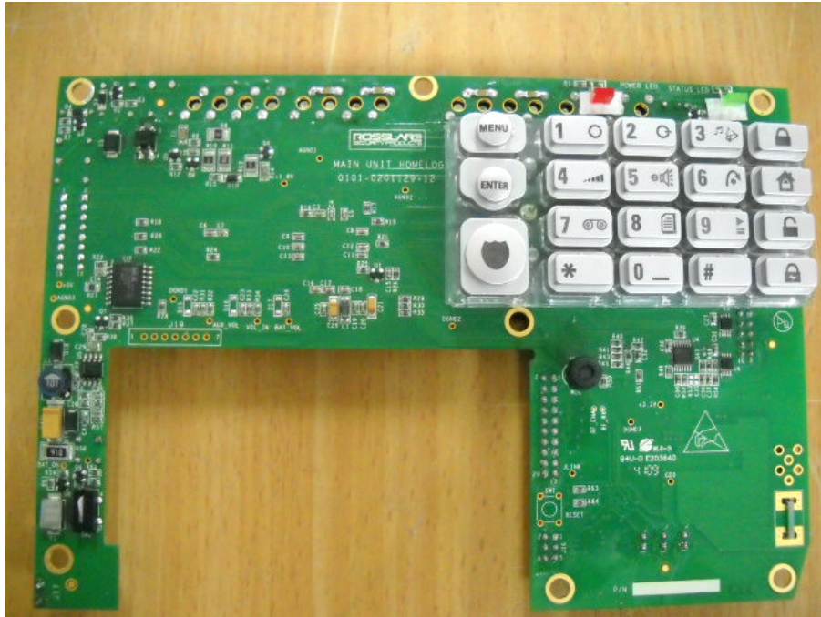
Photograph No.6 HLX-40BGE wireless security panel PCB second side view
