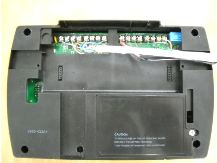
Photograph No.1 HLX-40BGE wireless security panel without cover view
