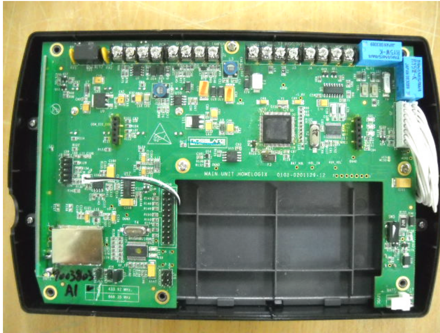
Photograph No.3 HLX-40BGE wireless security panel PCB top view
