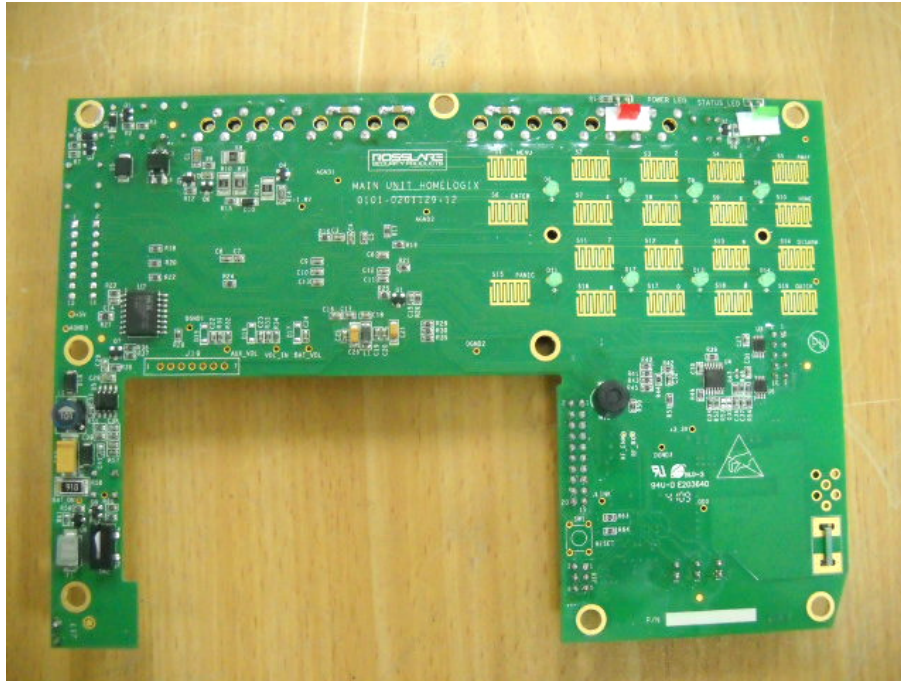
Photograph No.7 HLX-40BGE wireless security panel PCB second side view
