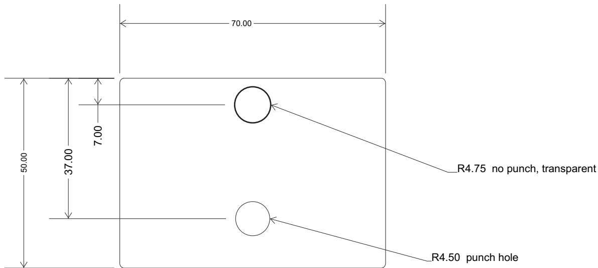
Dimension drawing
