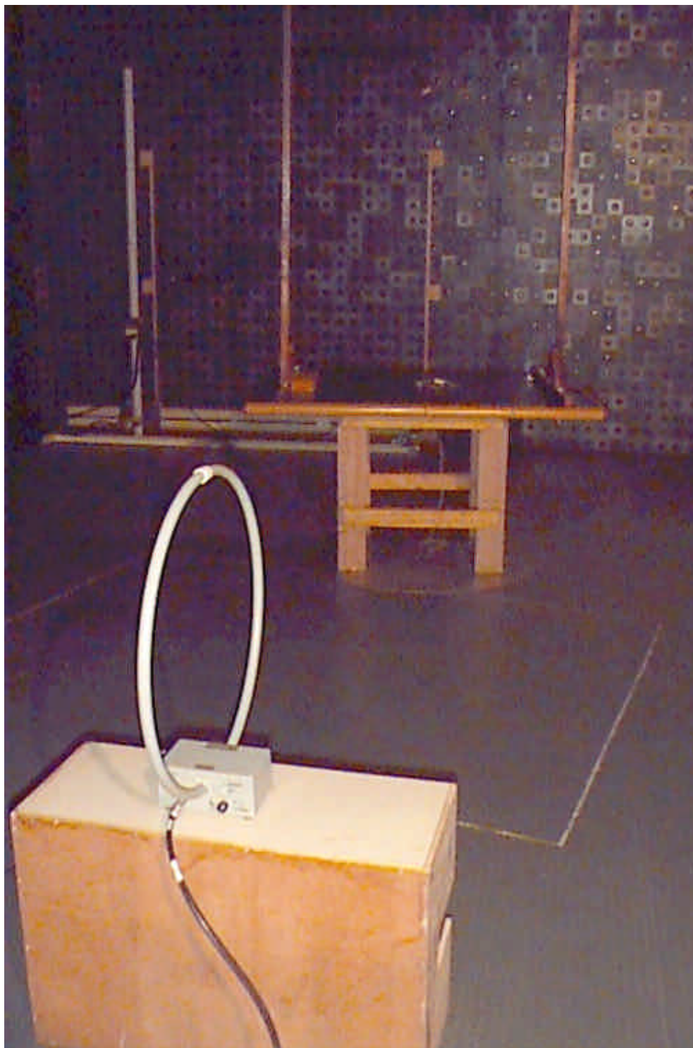
Photograph No.1 Radiated emissions measurement setup
