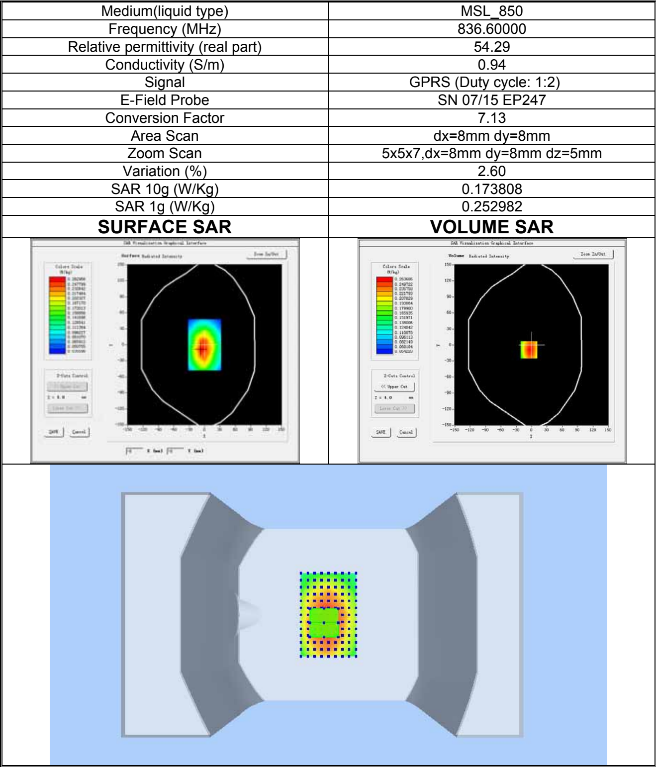
Plot 8: GPRS850MHz, Mid channel(Body-worn, Left edge) Product Description: MOBILE PHONE Test Date: 2018-09-25
