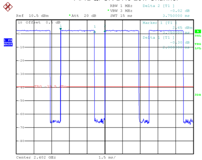
Pi/4DQPSK DH5 Low Channel
