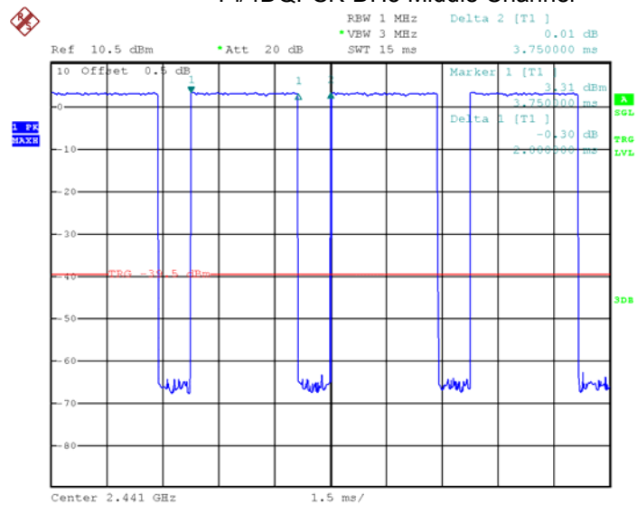
Pi/4DQPSK DH5 Middle Channel
