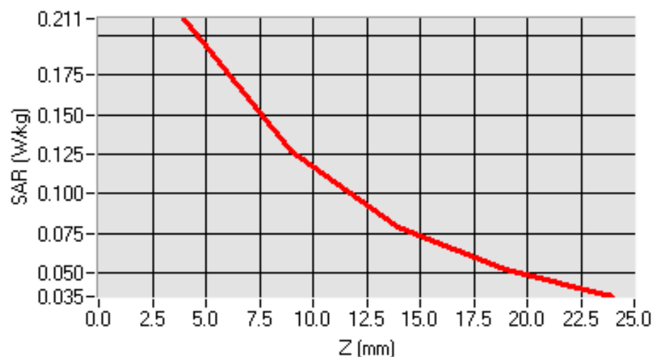
SAR, Z Axis Scan (X = 7, Y = -24)
