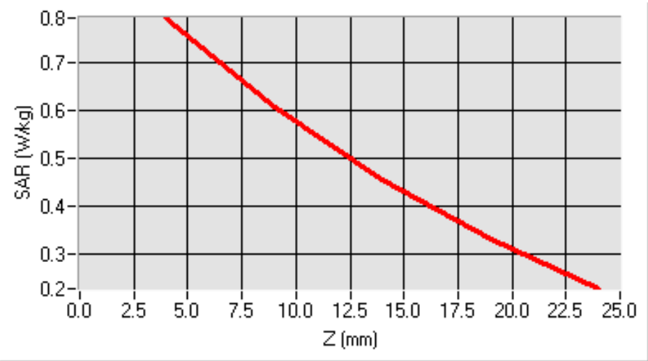
SAR, Z Axis Scan (X = -22, Y = -11)
