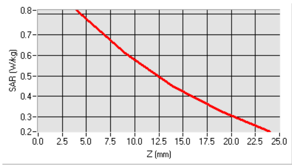
SAR, Z Axis Scan (X = -23, Y = -10)
