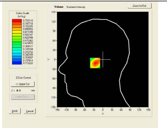
SAR, Z Axis Scan (X = -22, Y = -11)
