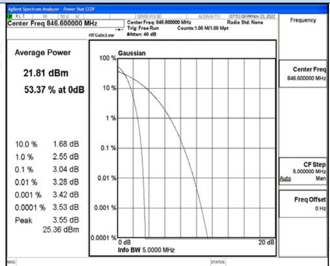
Channel 4233/ 846.6 MHz
