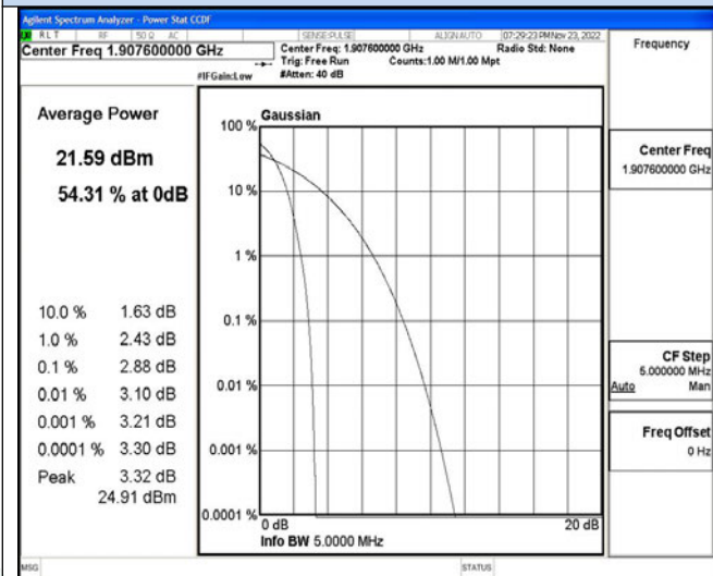
Channel 9538 / 1907.6 MHz
