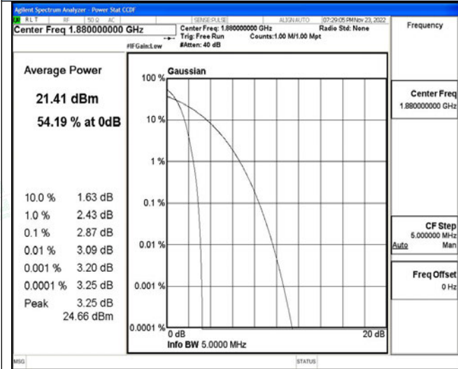
Channel 9400 / 1880.0 MHz
