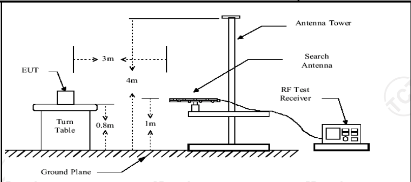
Above 1GHz
