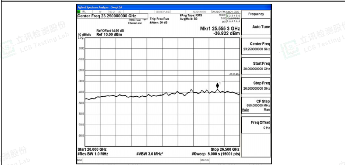
Band38-20MHz-16QAM-38150-1RB#0-Range6:20000~26500MHz
