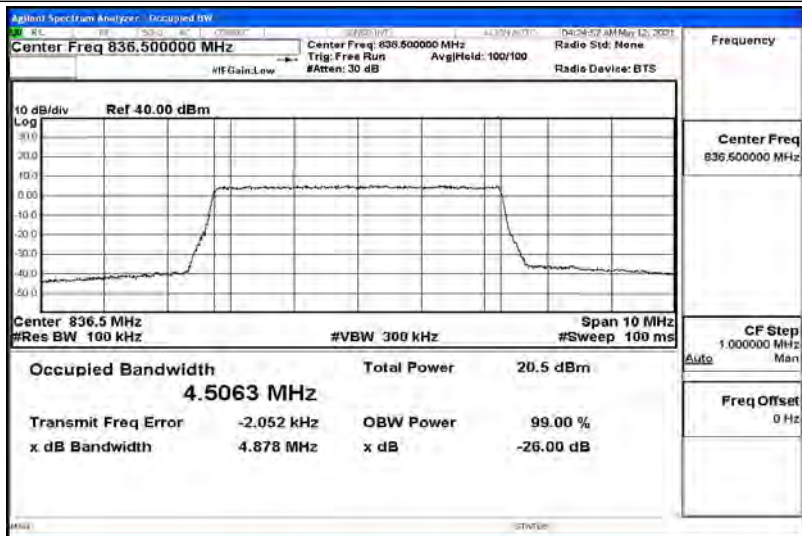
Band5-5MHz-16QAM-20625-25RB#0-4.5063
