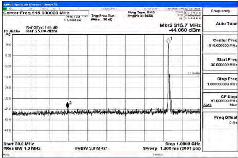
Band5-10MHz-16QAM-20525-1RB#0-Range2:1000~10000MHz
