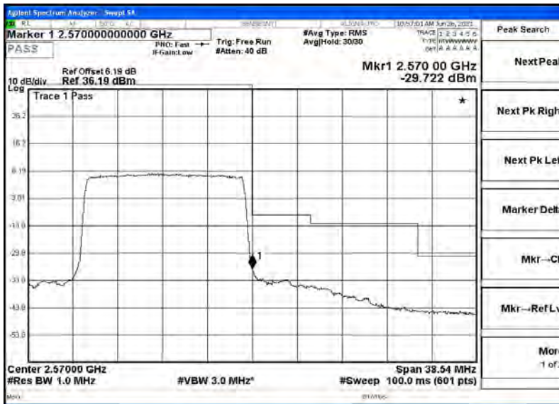
Band7-15MHz-QPSK-21375-75RB#0
