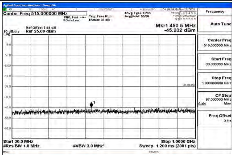
Band7-5MHz-QPSK-21425-1RB#0-Range2:1000~10000MHz
