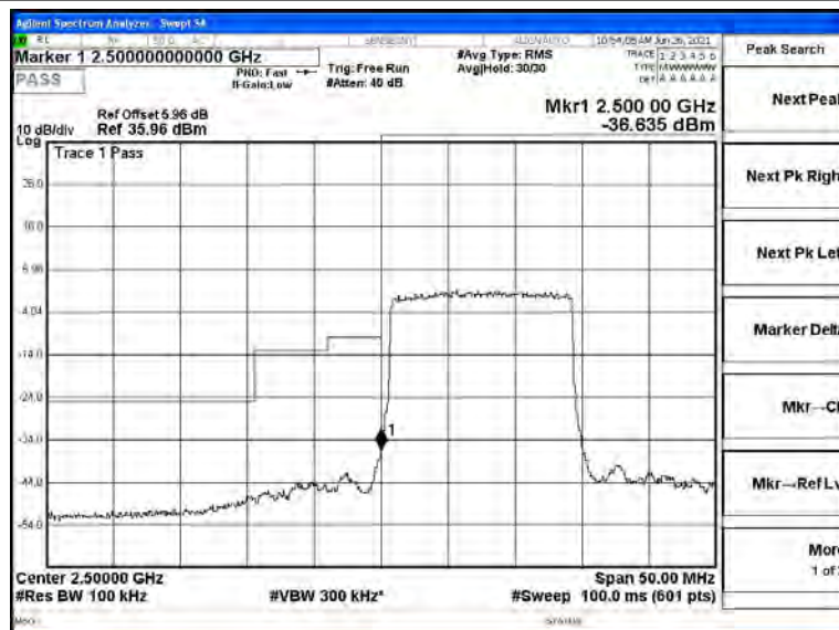
Band7-15MHz-16QAM-20825-75RB#0
