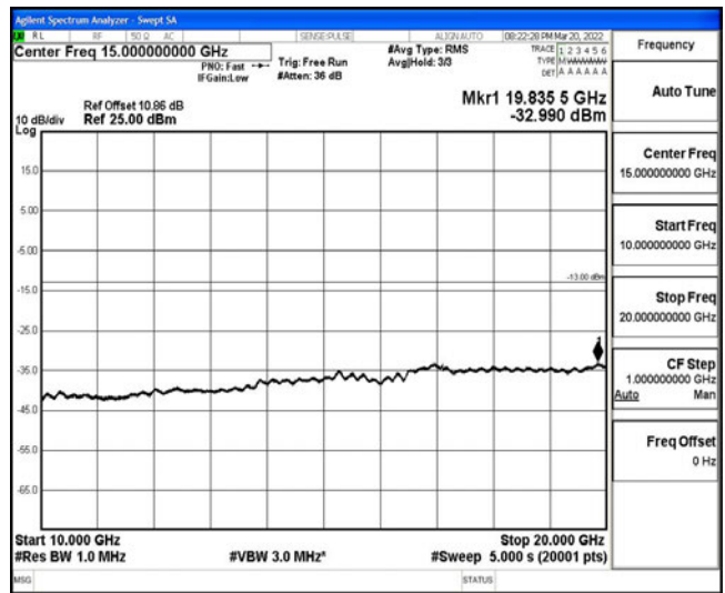
Band4-20MHz-16QAM-20300-1RB#0-Range5:10000~20000MHz
