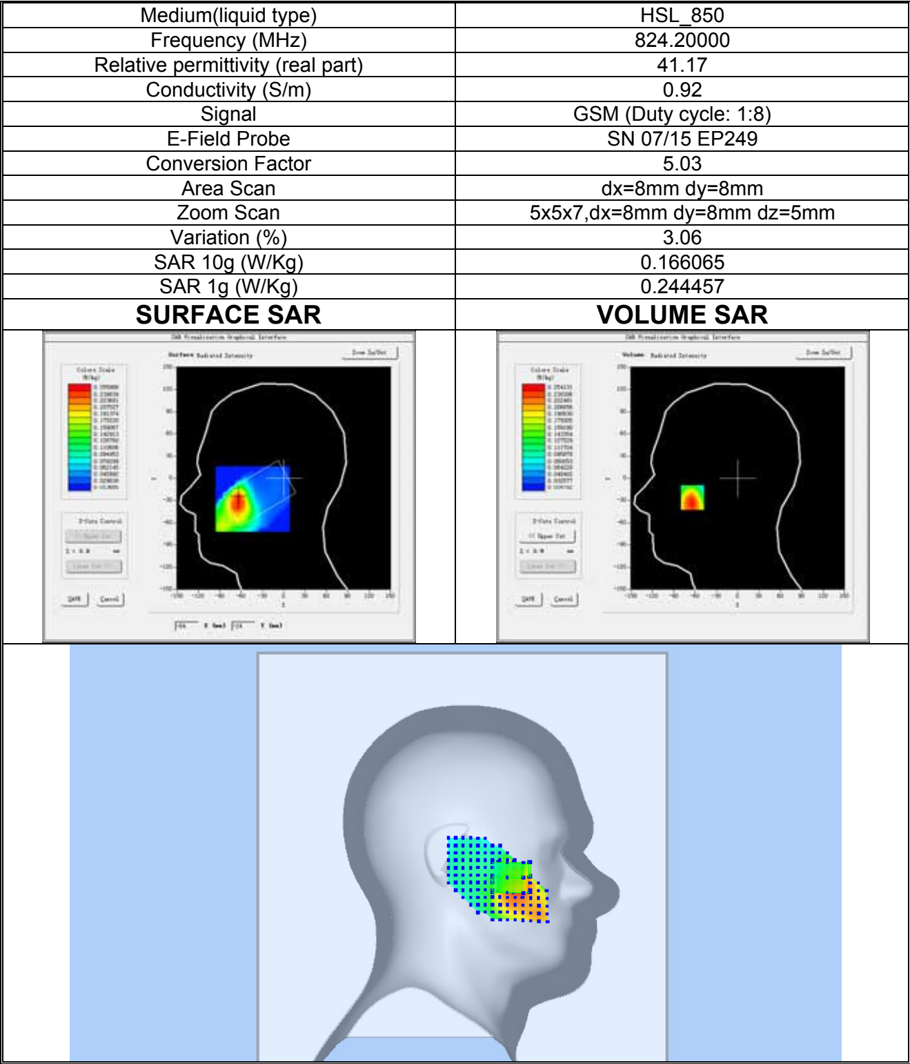
Plot 3: GSM850MHz, Low channel (Left Head , Cheek) Product Description: MOBILE PHONE Test Date:2018-03-05
