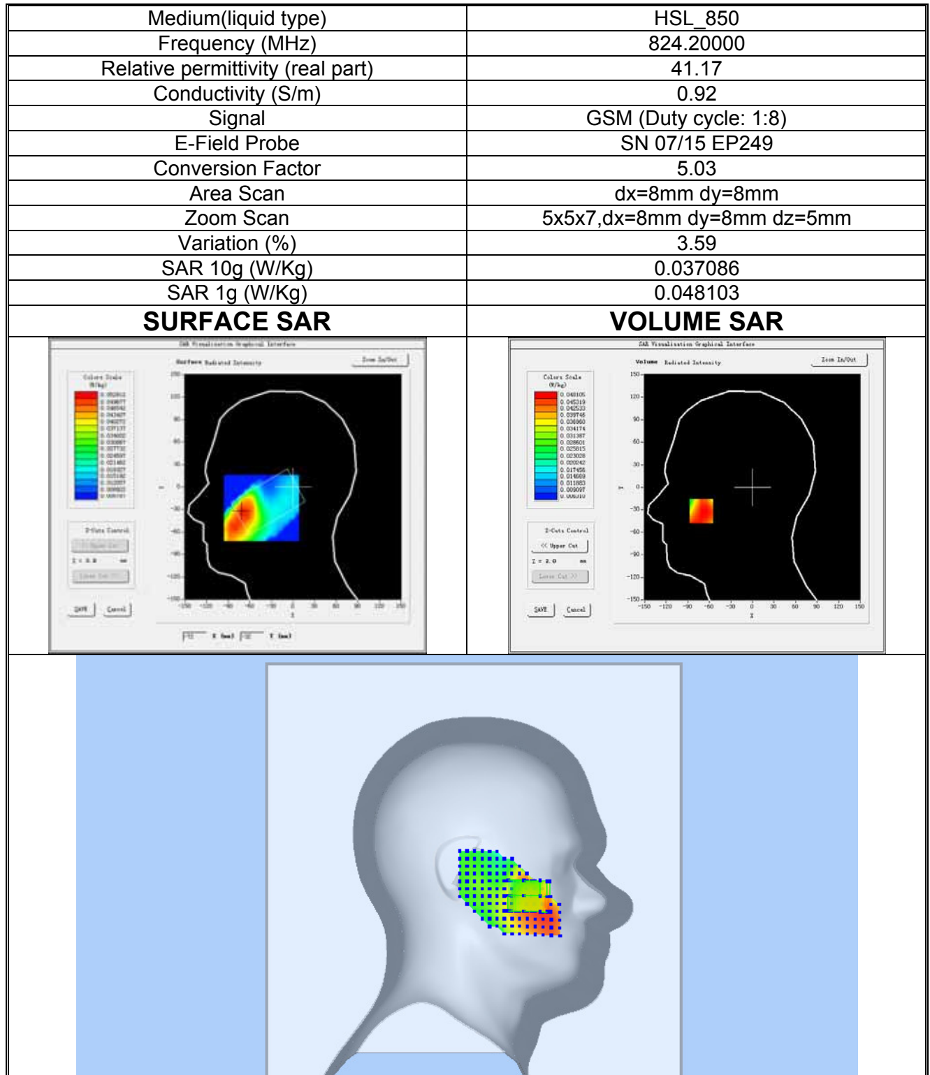
Plot 4: GSM850MHz, channel (Left Head , Tilt) Product Description: MOBILE PHONE Test Date:2018-03-05
