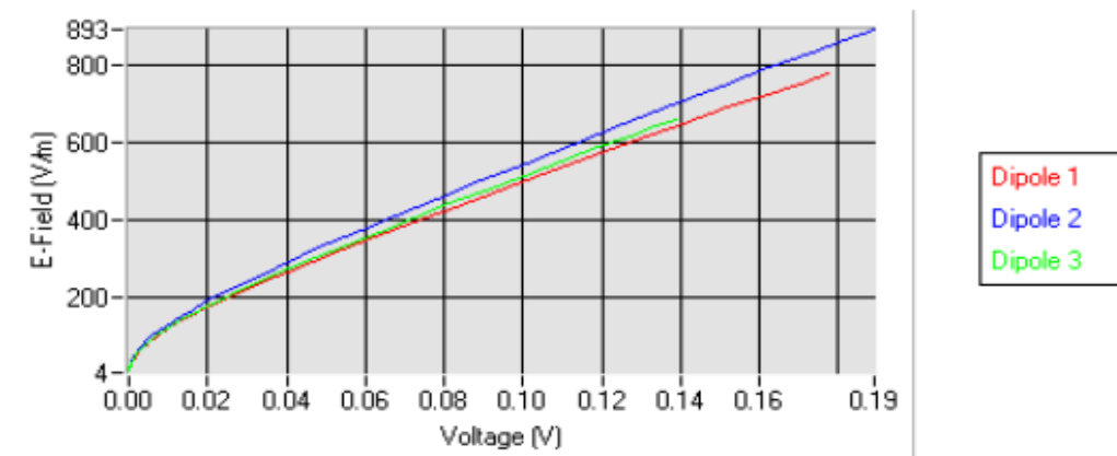
Calibration curves
