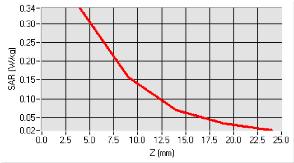
SAR, Z Axis Scan (X = -9, Y = -10)
