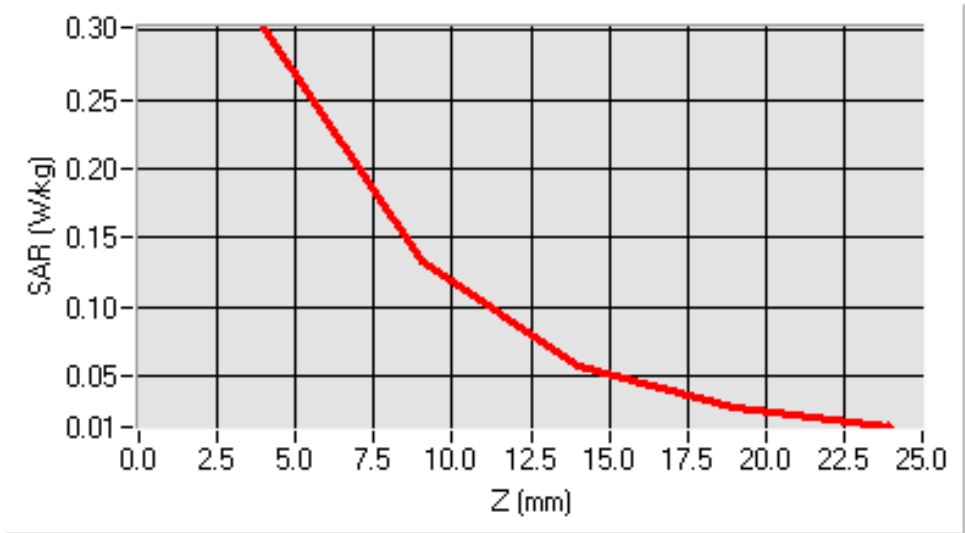
SAR, Z Axis Scan (X = 0, Y = -5)
