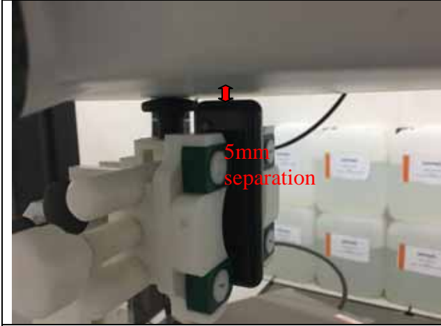
Body-Worn(Top edge)
