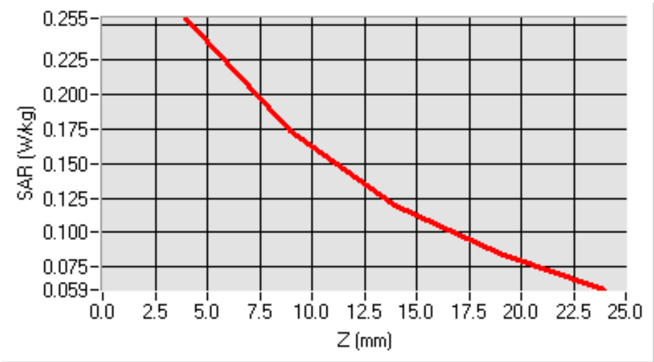
SAR, Z Axis Scan (X = -55, Y = -16)
