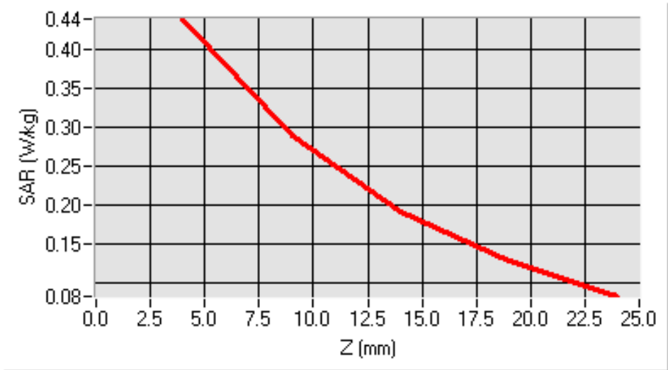
SAR, Z Axis Scan (X = 8, Y = -54)
