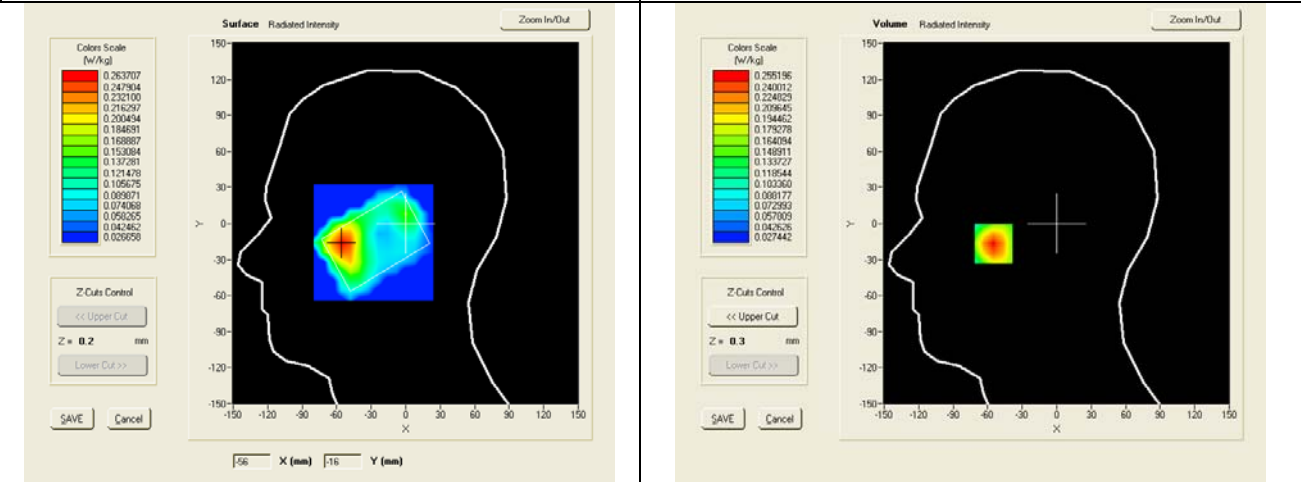
SAR, Z Axis Scan (X = -55, Y = -16)
