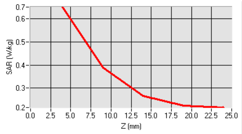
SAR, Z Axis Scan (X = -15, Y = -56)
