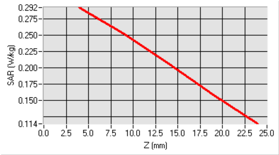
SAR, Z Axis Scan (X = -40, Y = -30)
