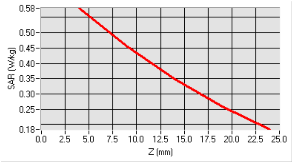
SAR, Z Axis Scan (X = 7, Y = -41)
