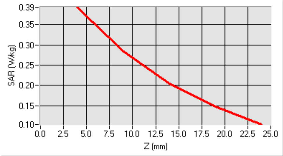
SAR, Z Axis Scan (X = -41, Y = -23)
