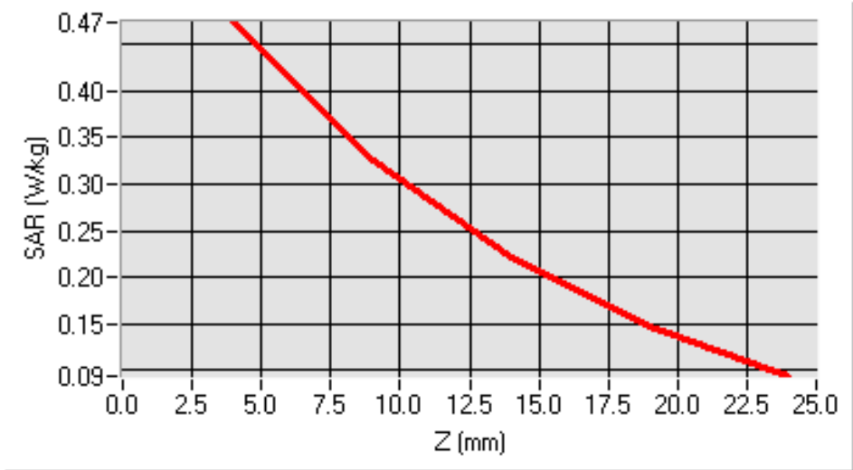
SAR, Z Axis Scan (X = -65, Y = -23)
