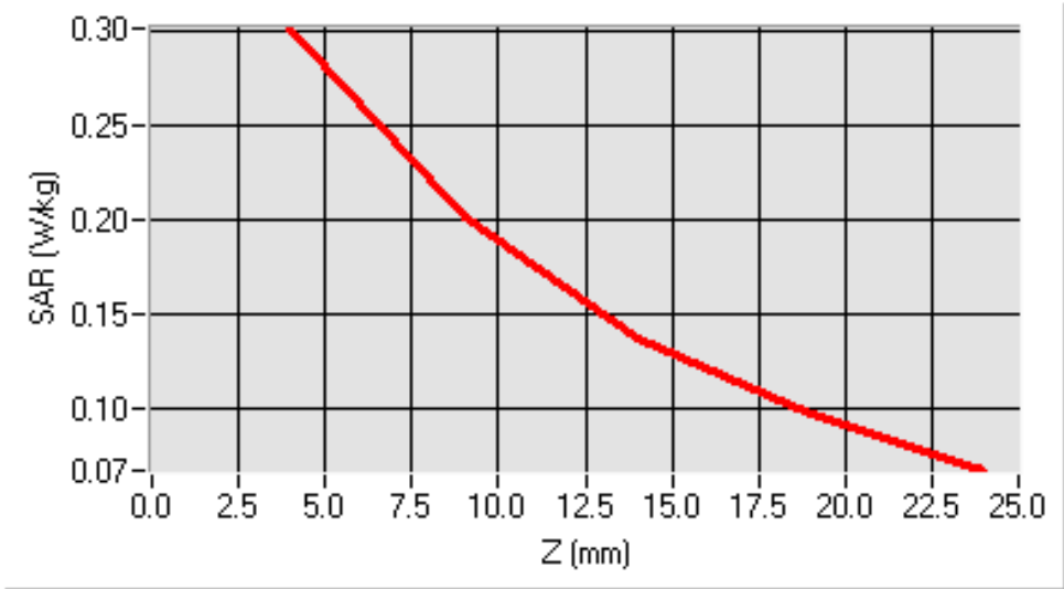
SAR, Z Axis Scan (X = -41, Y = -38)
