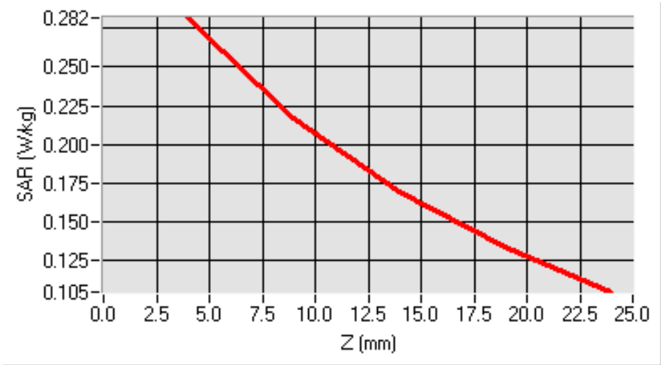
SAR, Z Axis Scan (X = -32, Y = -16)
