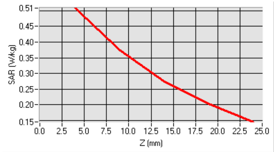
SAR, Z Axis Scan (X = -48, Y = -48)
