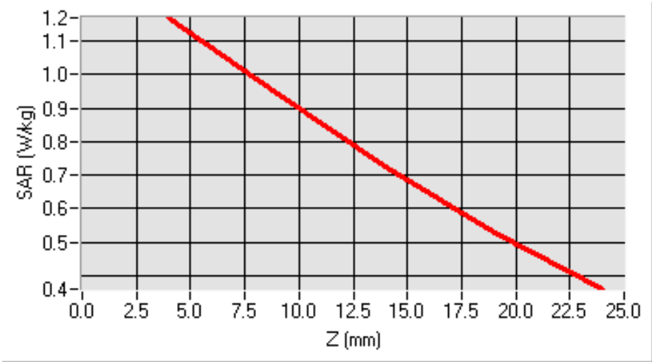
SAR, Z Axis Scan (X = -1, Y = -41)
