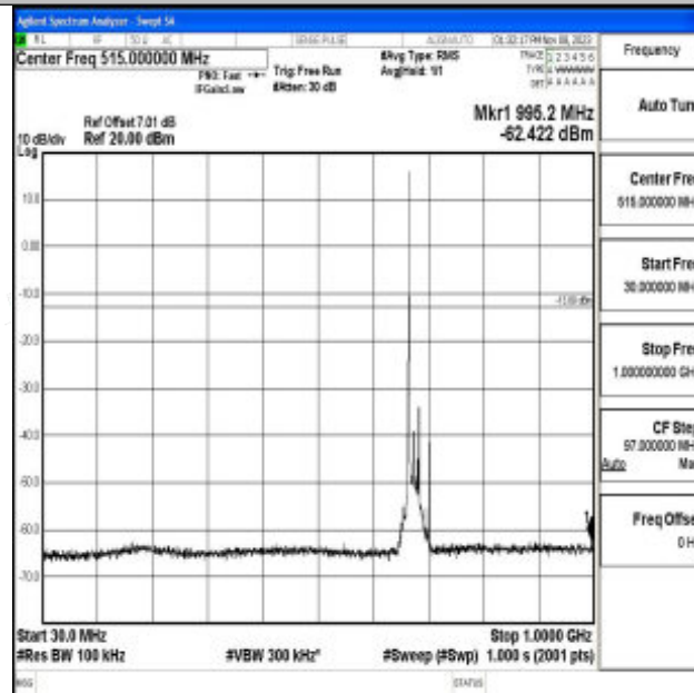
Band71_20MHz_QPSK_133322_1RB#0_30~1000_30~1000
