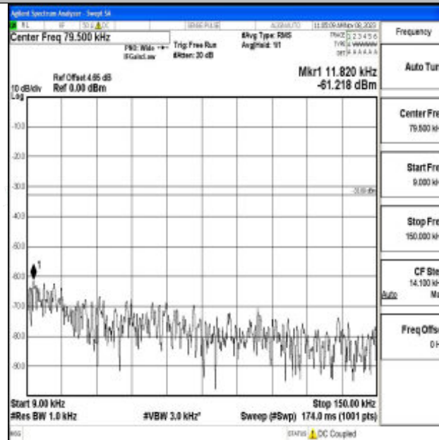
Band71_5MHz_16QAM_133147_1RB#0_0.009~0.15_0.009~0.15
