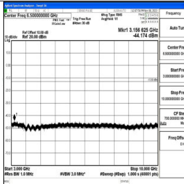
Band71_10MHz_QPSK_133422_1RB#0_3000~10000_3000~10000
