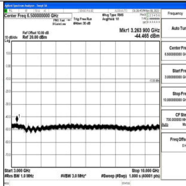
Band71_20MHz_QPSK_133222_1RB#0_3000~10000_3000~10000
