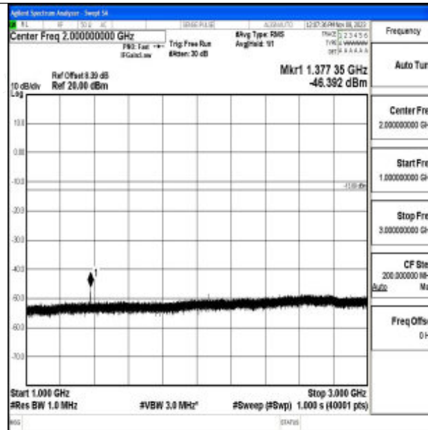
Band71_10MHz_QPSK_133422_1RB#0_1000~3000_1000~3000
