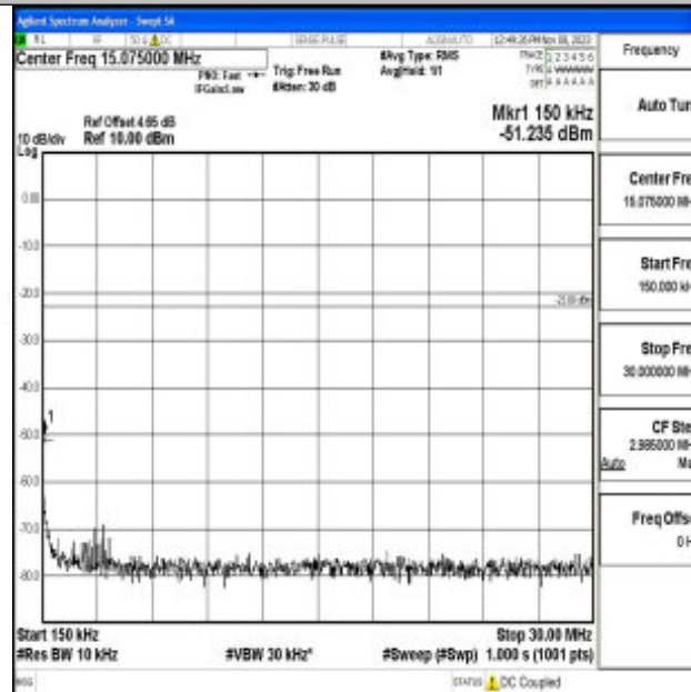
Band71_15MHz_16QAM_133297_1RB#0_0.15~30_0.15~30
