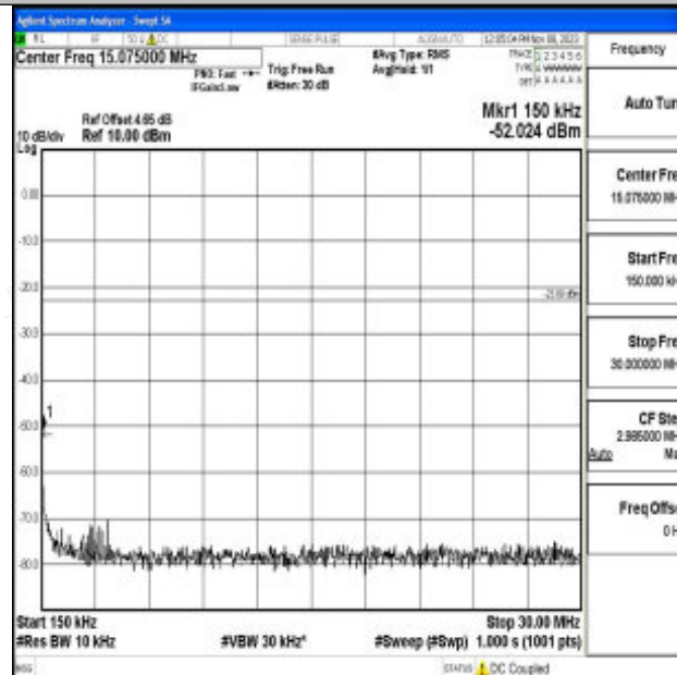
Band71_10MHz_64QAM_133297_1RB#0_0.15~30_0.15~30
