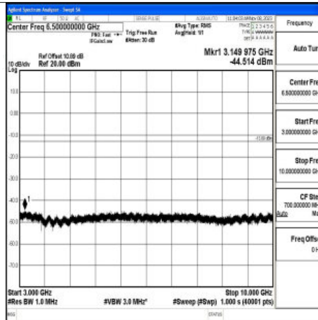
Band71_5MHz_QPSK_133147_1RB#0_3000~10000_3000~10000
