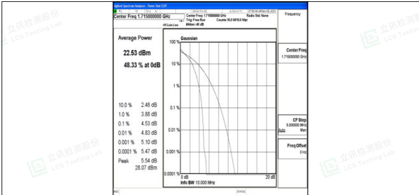
Band66-10MHz-64QAM-132022-1RB#0-PASS
