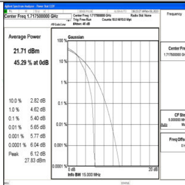
Band66-15MHz-16QAM-132047-1RB#0-PASS
