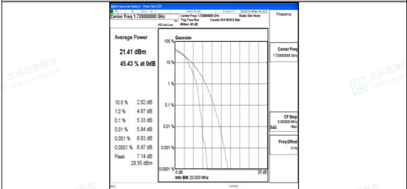
Band66-20MHz-16QAM-132072-1RB#0-PASS
