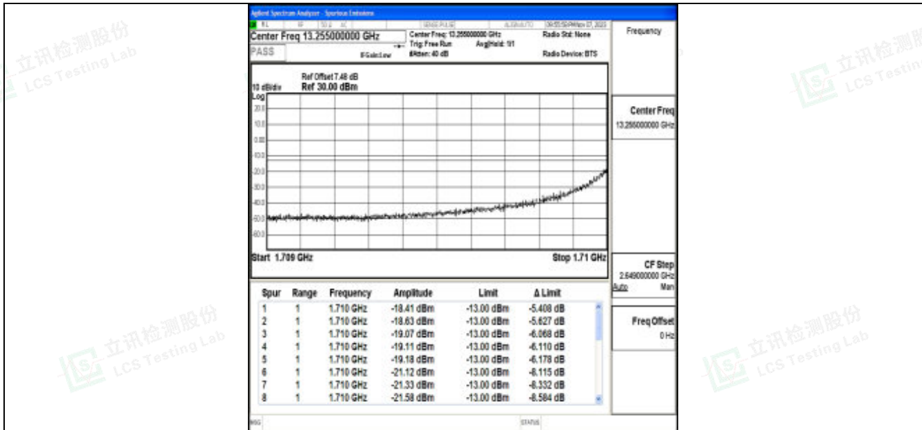
Band66_3MHz_64QAM_131987_1RB#0
