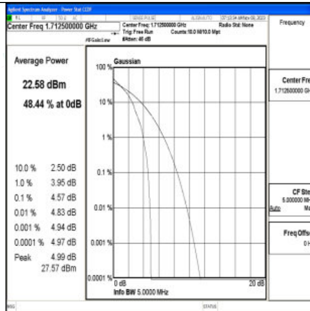
Band66-5MHz-64QAM-131997-1RB#0-PASS
