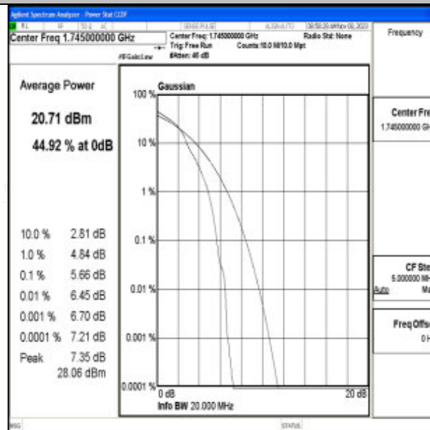
Band66-20MHz-16QAM-132322-1RB#0-PASS
