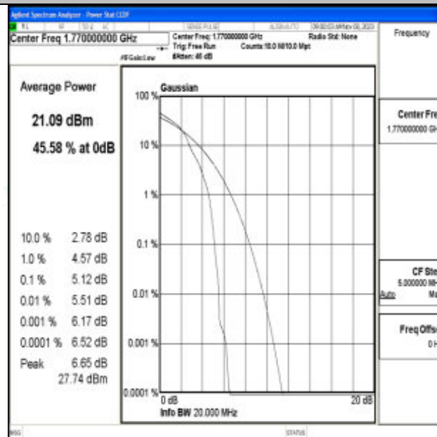
Band66-20MHz-16QAM-132572-1RB#0-PASS
