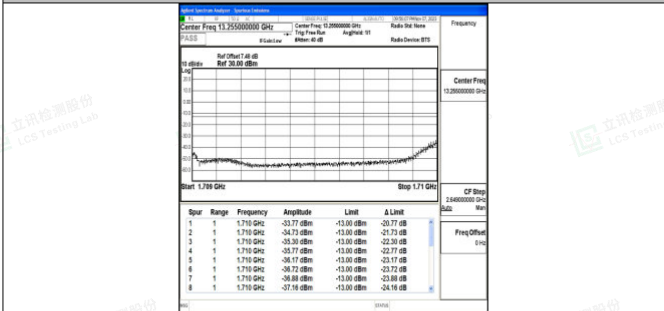
Band66_3MHz_QPSK_131987_1RB#14
