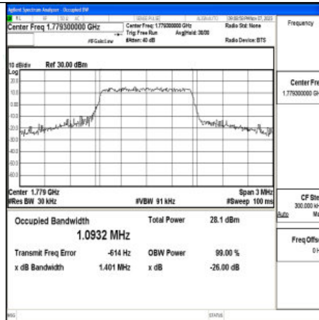
Band66-1.4MHz-QPSK-132665-6RB#0-PASS
