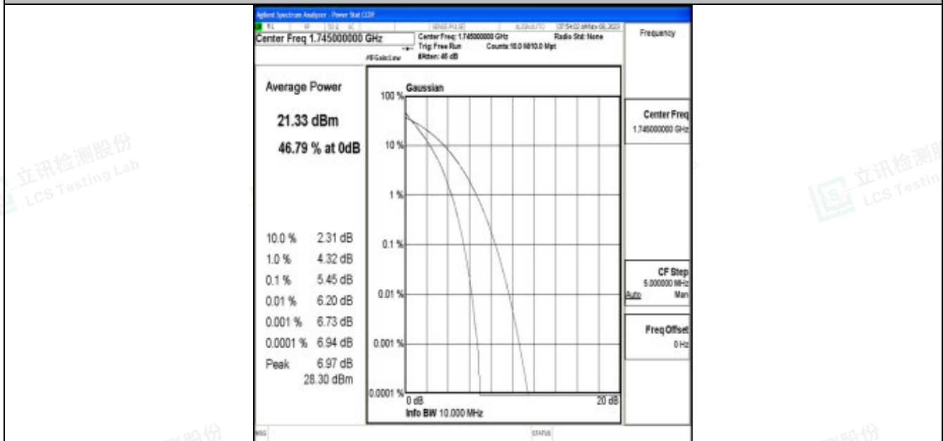
Band66-10MHz-64QAM-132322-50RB#0-PASS
