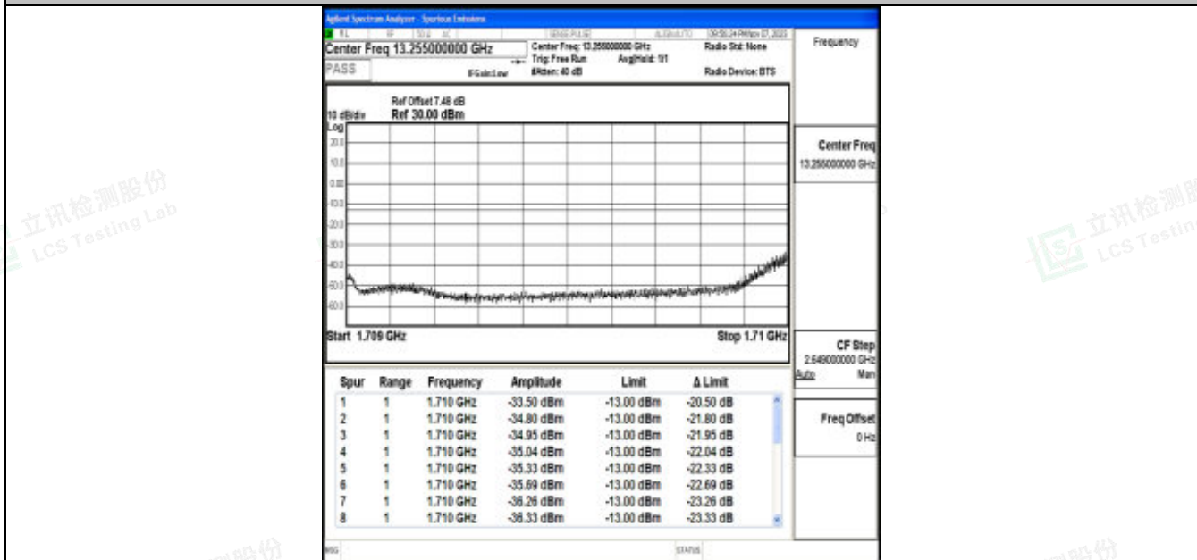
Band66_3MHz_64QAM_131987_1RB#14
