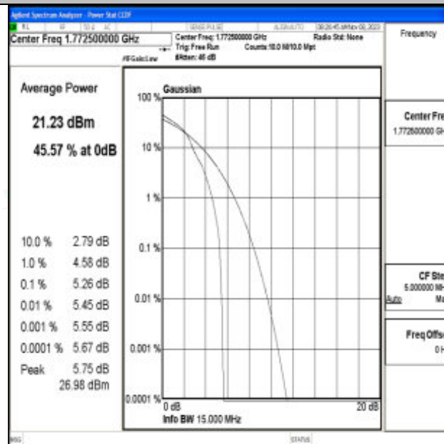
Band66-15MHz-16QAM-132597-1RB#0-PASS
