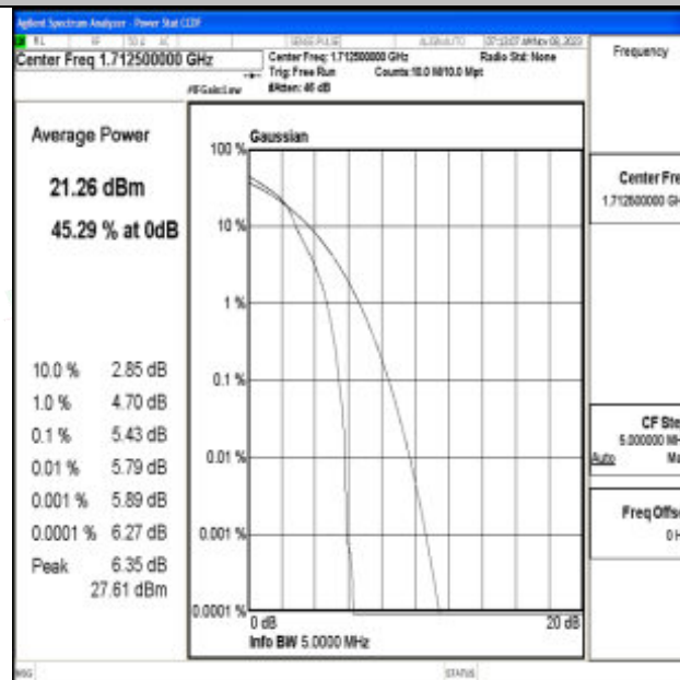
Band66-5MHz-16QAM-131997-1RB#0-PASS
