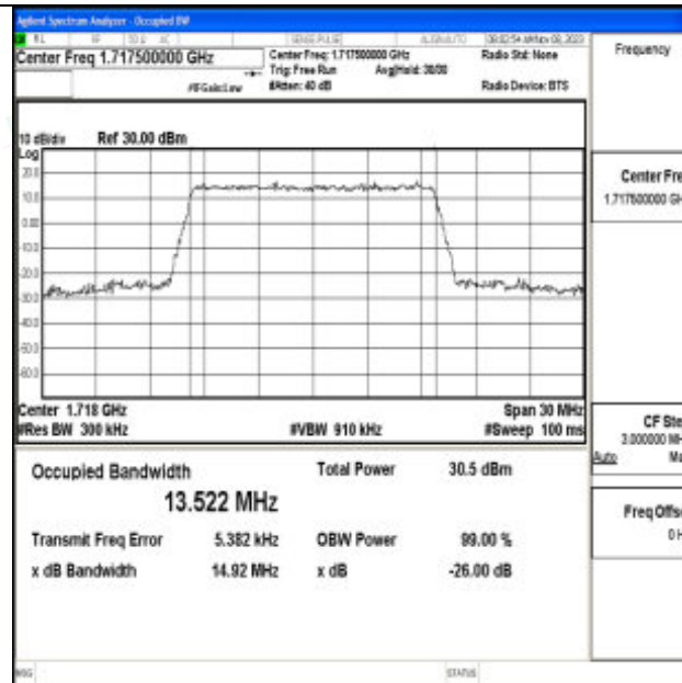
Band66-15MHz-QPSK-132047-75RB#0-PASS
