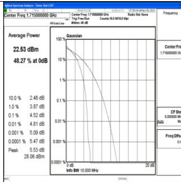
Band66-10MHz-QPSK-132022-1RB#0-PASS
