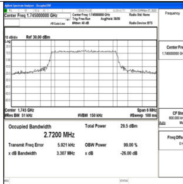
Band66-3MHz-64QAM-132322-15RB#0-PASS
