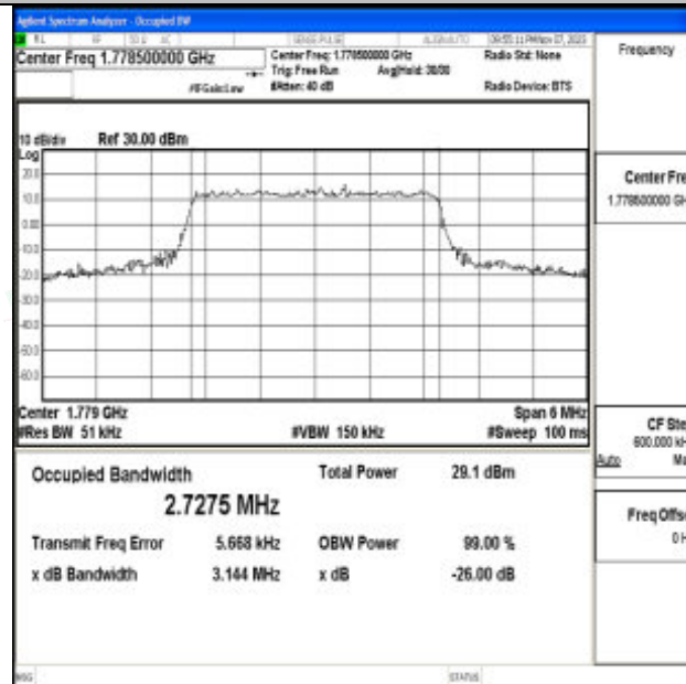
Band66-3MHz-64QAM-132657-15RB#0-PASS
