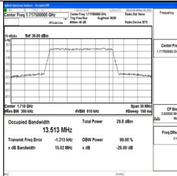
Band66-15MHz-16QAM-132047-75RB#0-PASS
