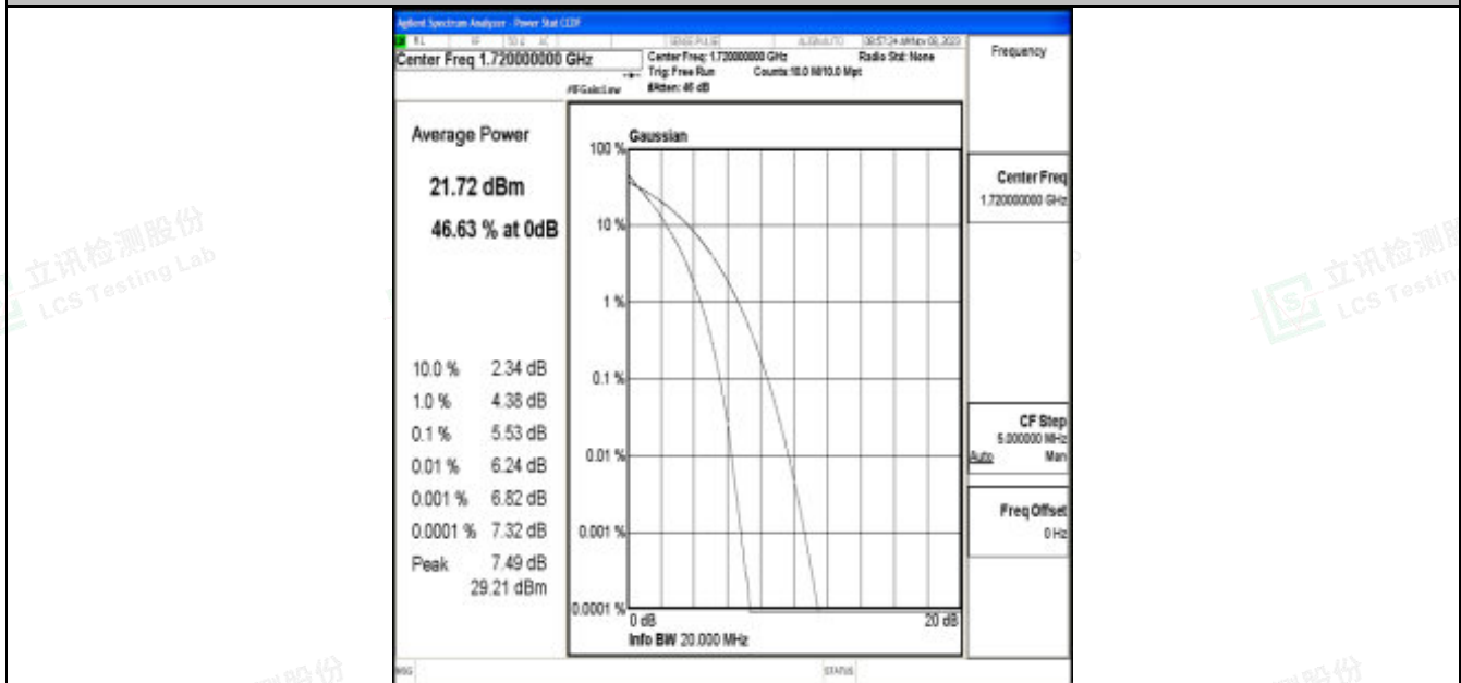
Band66-20MHz-QPSK-132072-100RB#0-PASS
