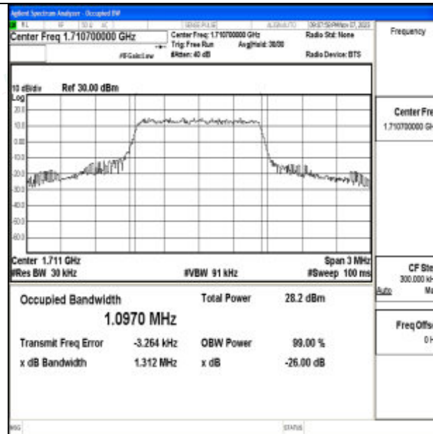
Band66-1.4MHz-64QAM-131979-6RB#0-PASS
