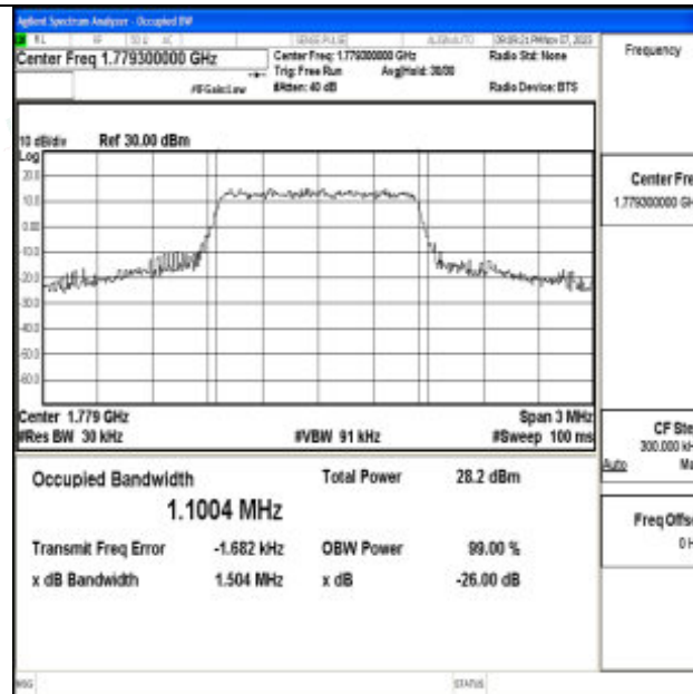
Band66-1.4MHz-64QAM-132665-6RB#0-PASS
