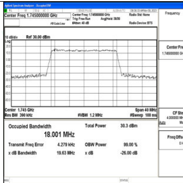
Band66-20MHz-64QAM-132322-100RB#0-PASS
