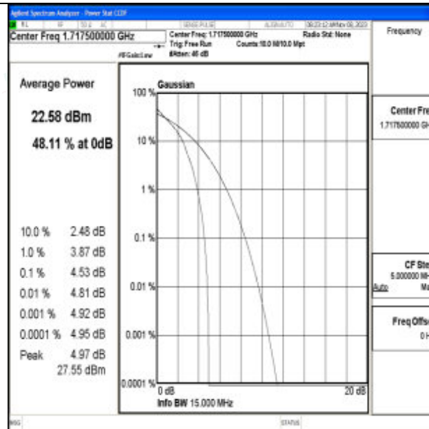
Band66-15MHz-QPSK-132047-1RB#0-PASS
