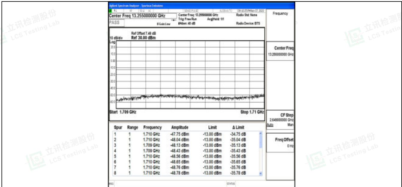
Band66_1.4MHz_16QAM_131979_1RB#5
