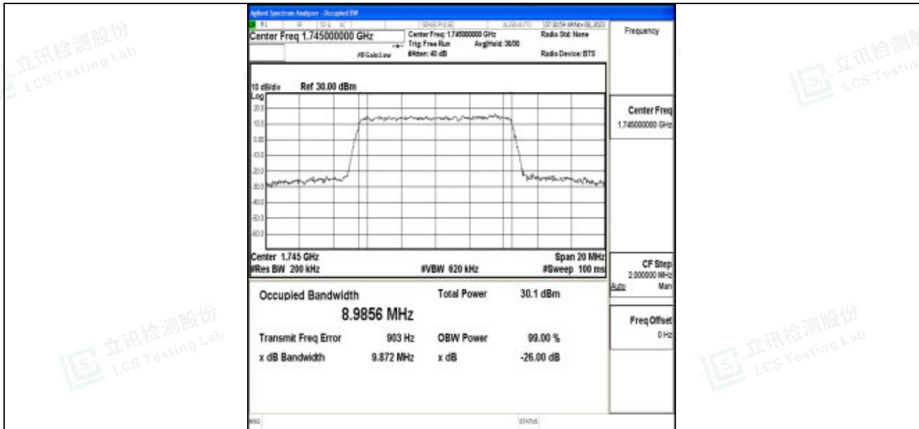
Band66-10MHz-64QAM-132322-50RB#0-PASS
