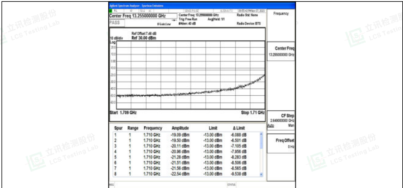
Band66_3MHz_QPSK_131987_1RB#0
