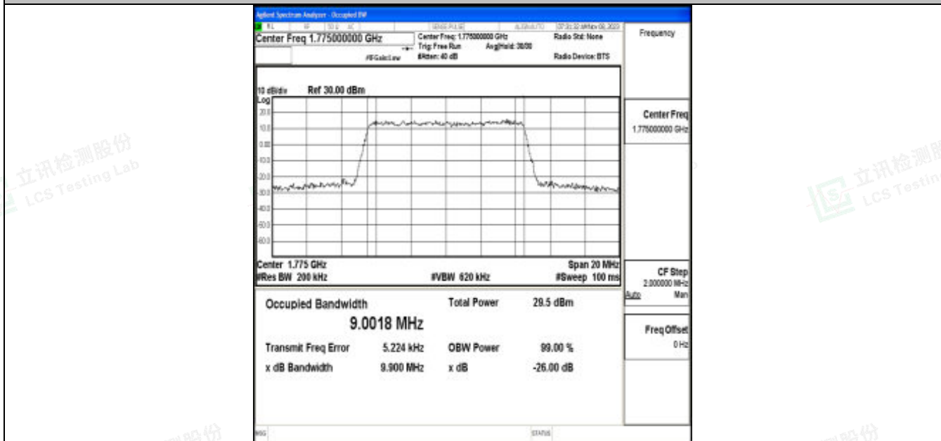
Band66-10MHz-64QAM-132622-50RB#0-PASS
