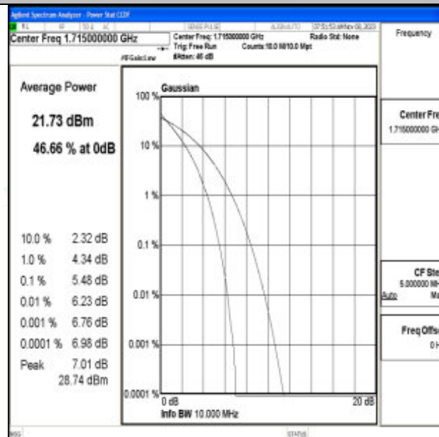
Band66-10MHz-64QAM-132022-50RB#0-PASS
