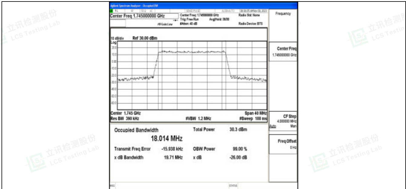
Band66-20MHz-QPSK-132322-100RB#0-PASS
