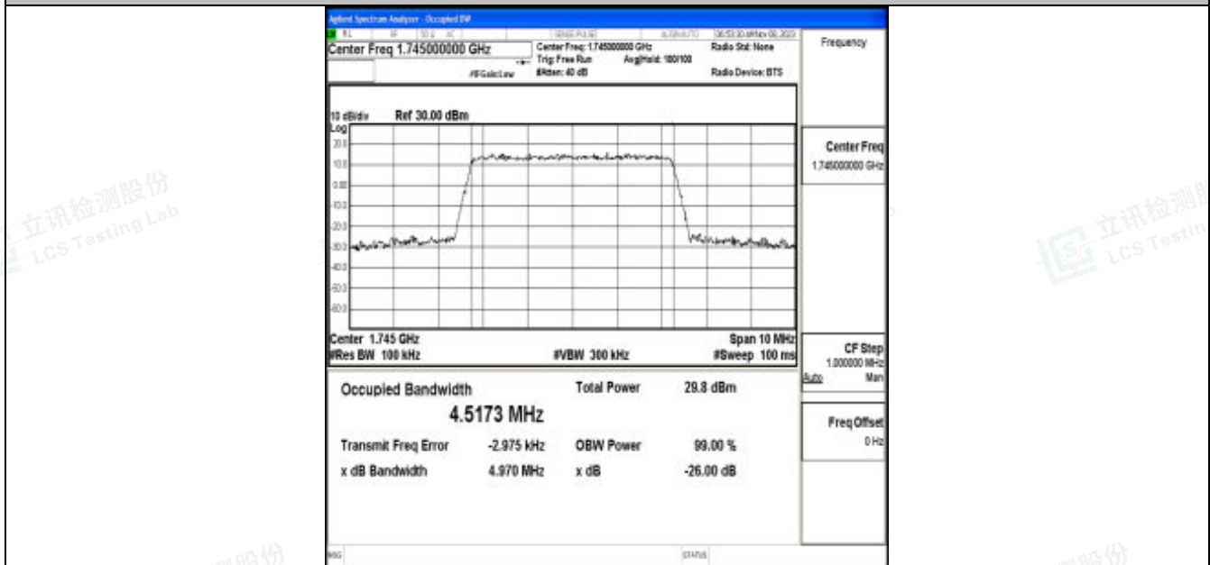
Band66-5MHz-QPSK-132322-25RB#0-PASS
