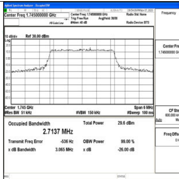
Band66-3MHz-QPSK-132322-15RB#0-PASS
