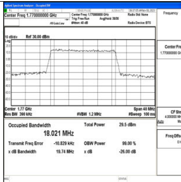
Band66-20MHz-16QAM-132572-100RB#0-PASS
