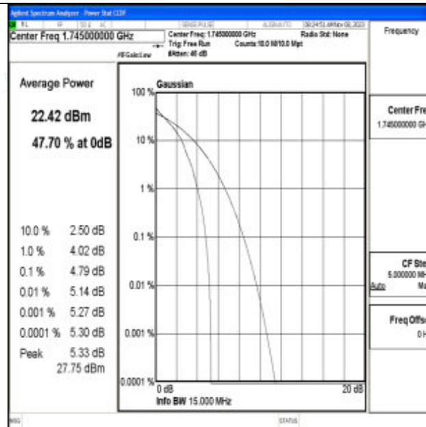
Band66-15MHz-QPSK-132322-1RB#0-PASS
