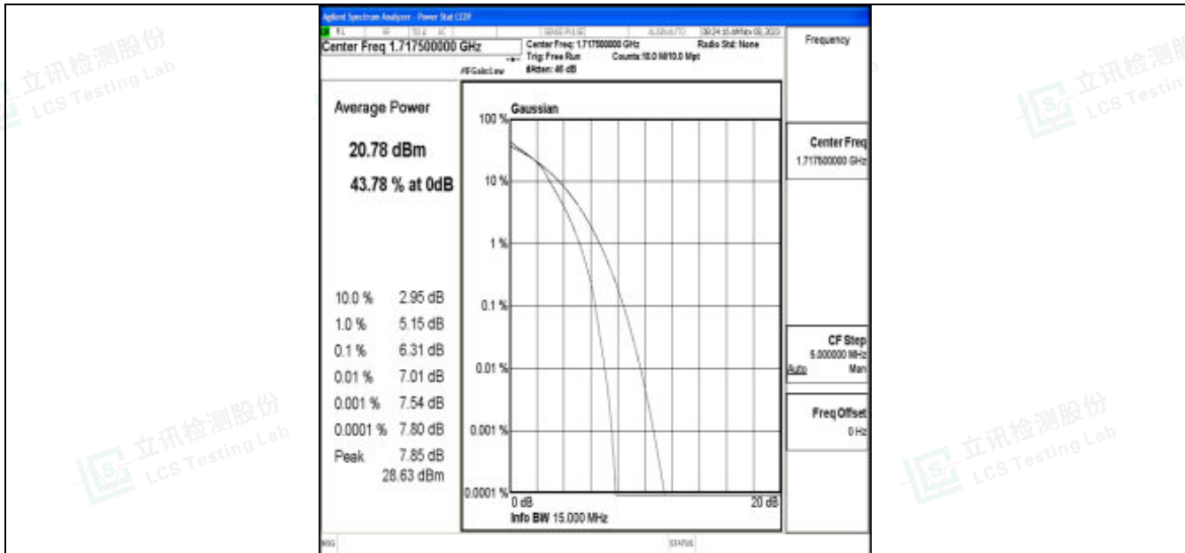
Band66-15MHz-16QAM-132047-75RB#0-PASS
