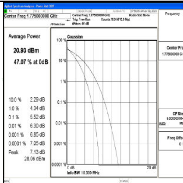
Band66-10MHz-64QAM-132622-50RB#0-PASS
