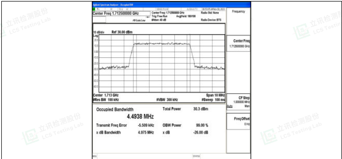
Band66-5MHz-64QAM-131997-25RB#0-PASS
