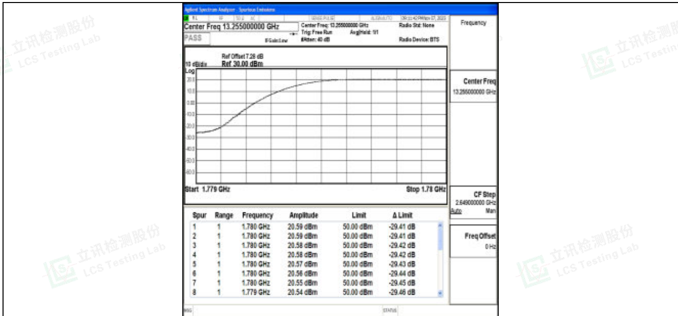
Band66_1.4MHz_QPSK_132665_1RB#5
