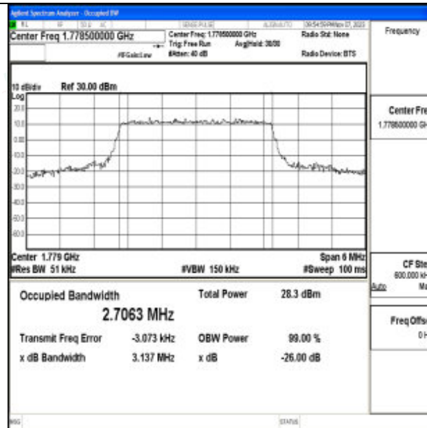
Band66-3MHz-16QAM-132657-15RB#0-PASS
