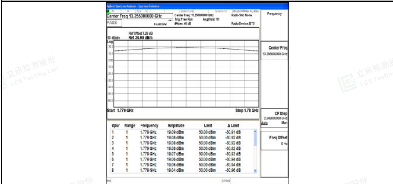
Band66_1.4MHz_64QAM_132665_6RB#0
