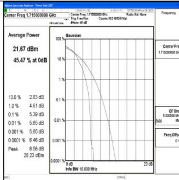
Band66-10MHz-16QAM-132022-1RB#0-PASS
