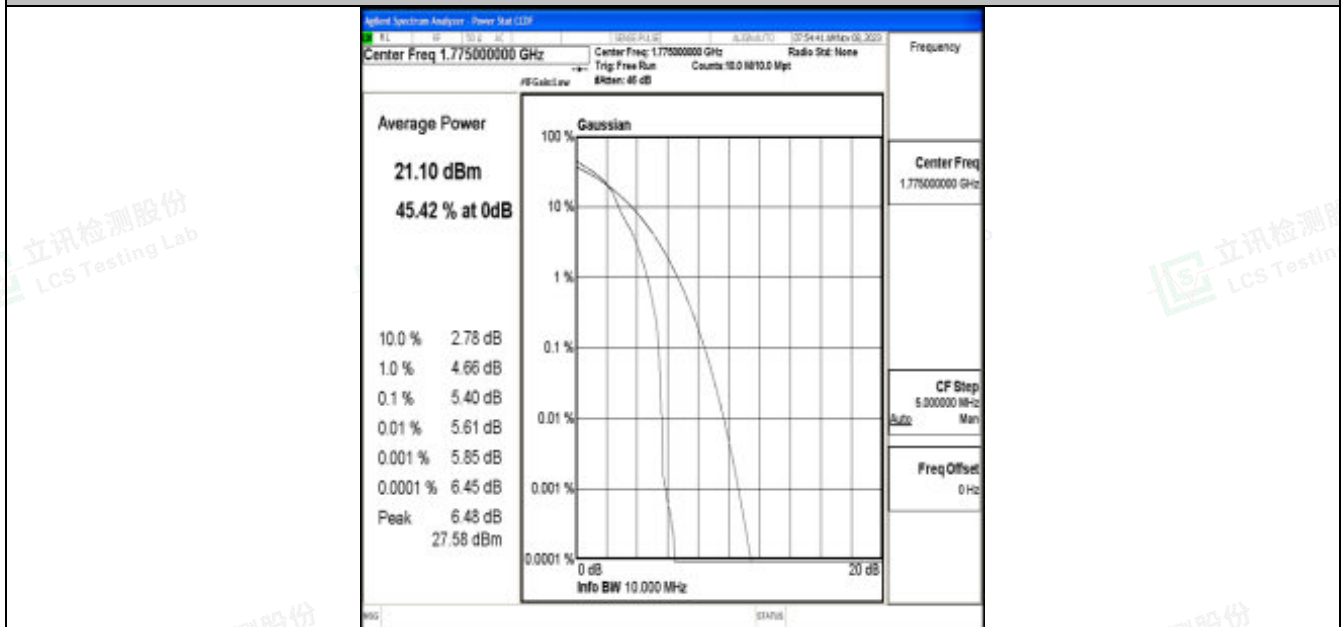
Band66-10MHz-16QAM-132622-1RB#0-PASS
