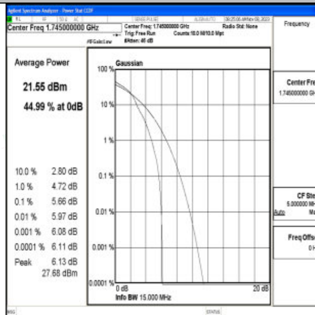
Band66-15MHz-16QAM-132322-1RB#0-PASS
