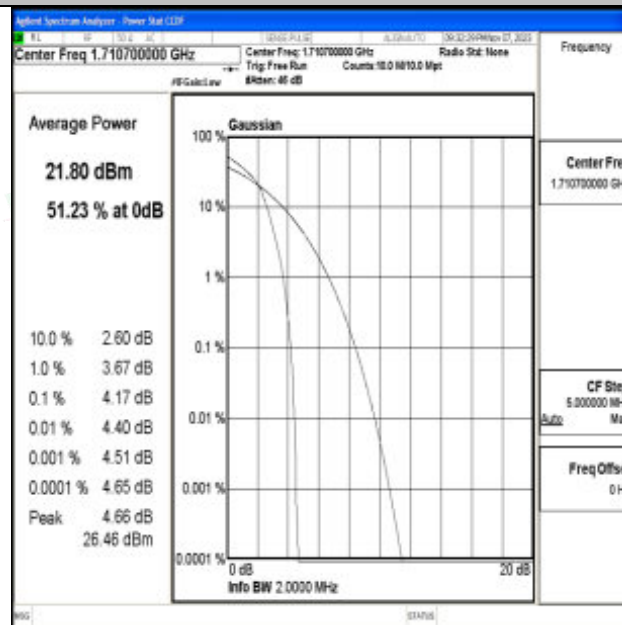
Band66-1.4MHz-16QAM-131979-1RB#0-PASS
