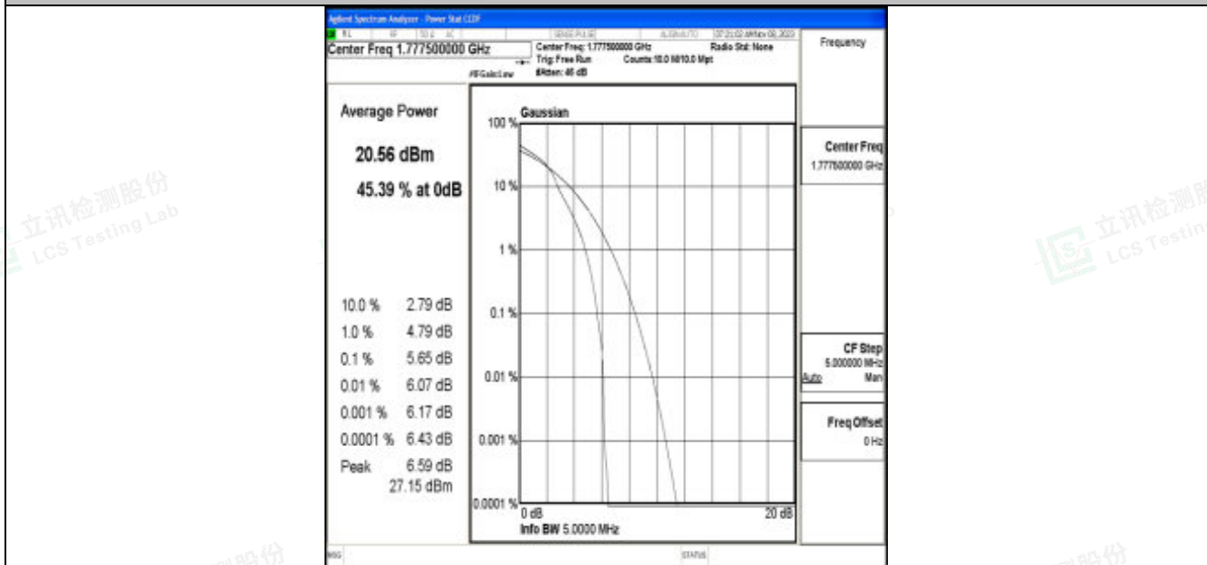
Band66-5MHz-16QAM-132647-1RB#0-PASS
