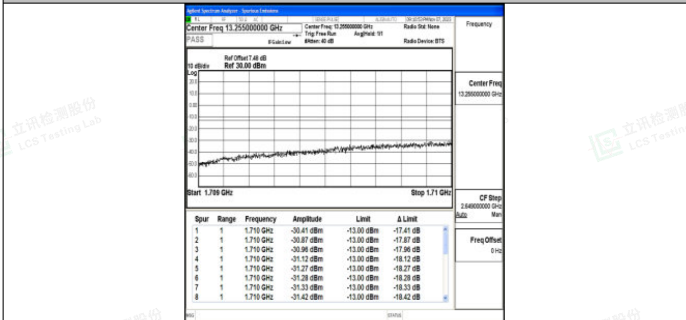
Band66_1.4MHz_16QAM_131979_6RB#0
