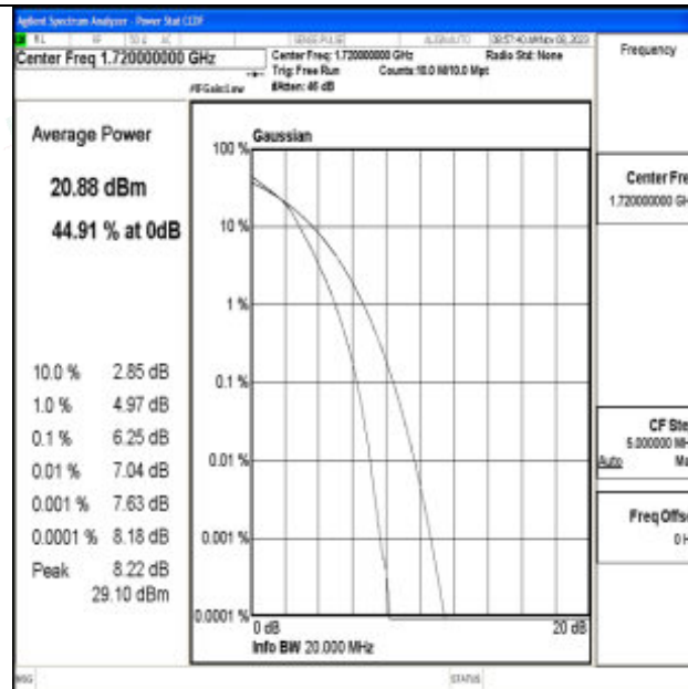
Band66-20MHz-16QAM-132072-100RB#0-PASS
