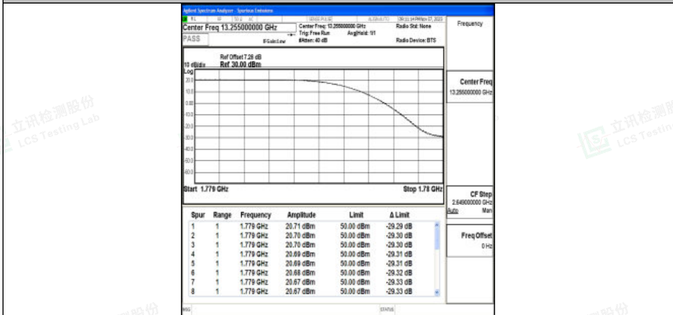
Band66_1.4MHz_QPSK_132665_1RB#0
