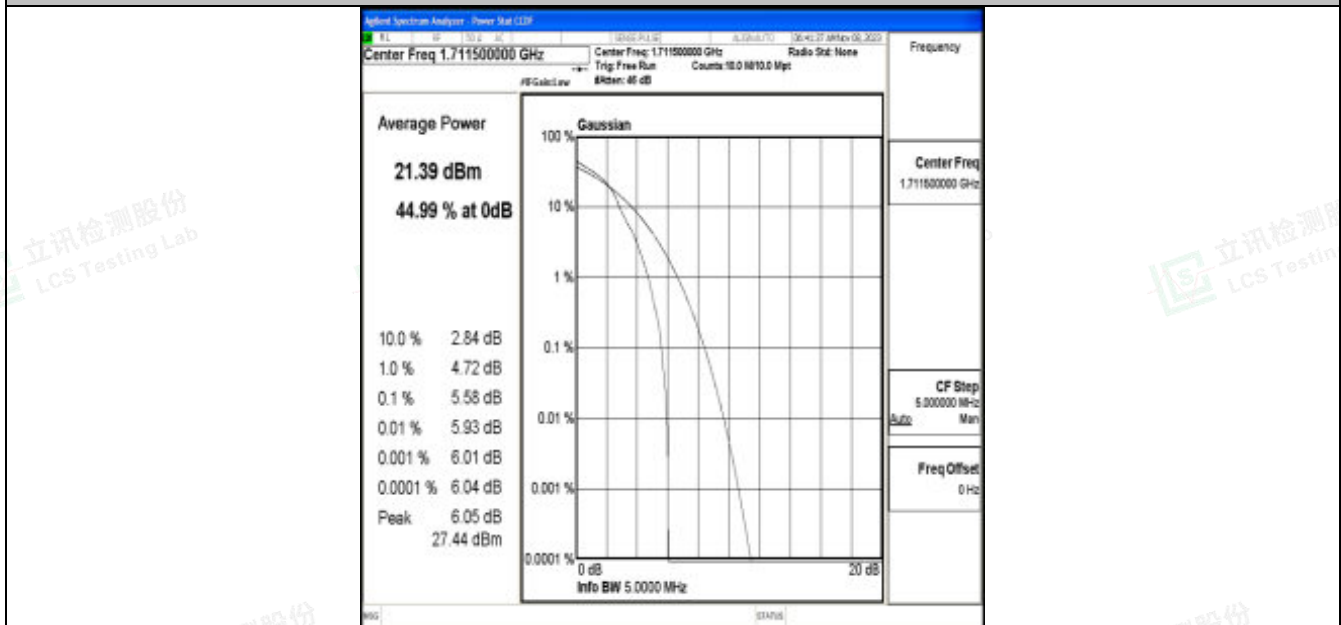
Band66-3MHz-16QAM-131987-1RB#0-PASS
