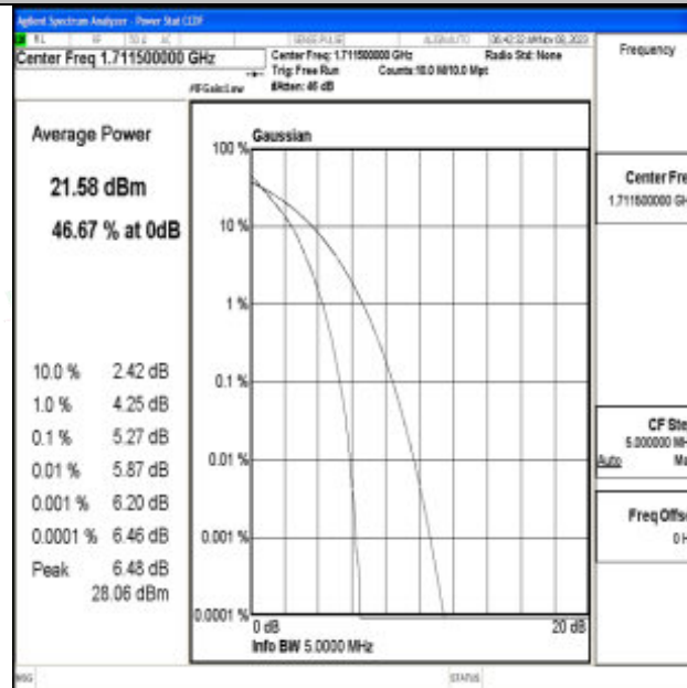
Band66-3MHz-QPSK-131987-15RB#0-PASS
