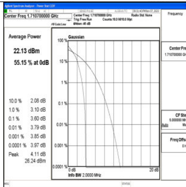
Band66-1.4MHz-QPSK-131979-1RB#0-PASS
