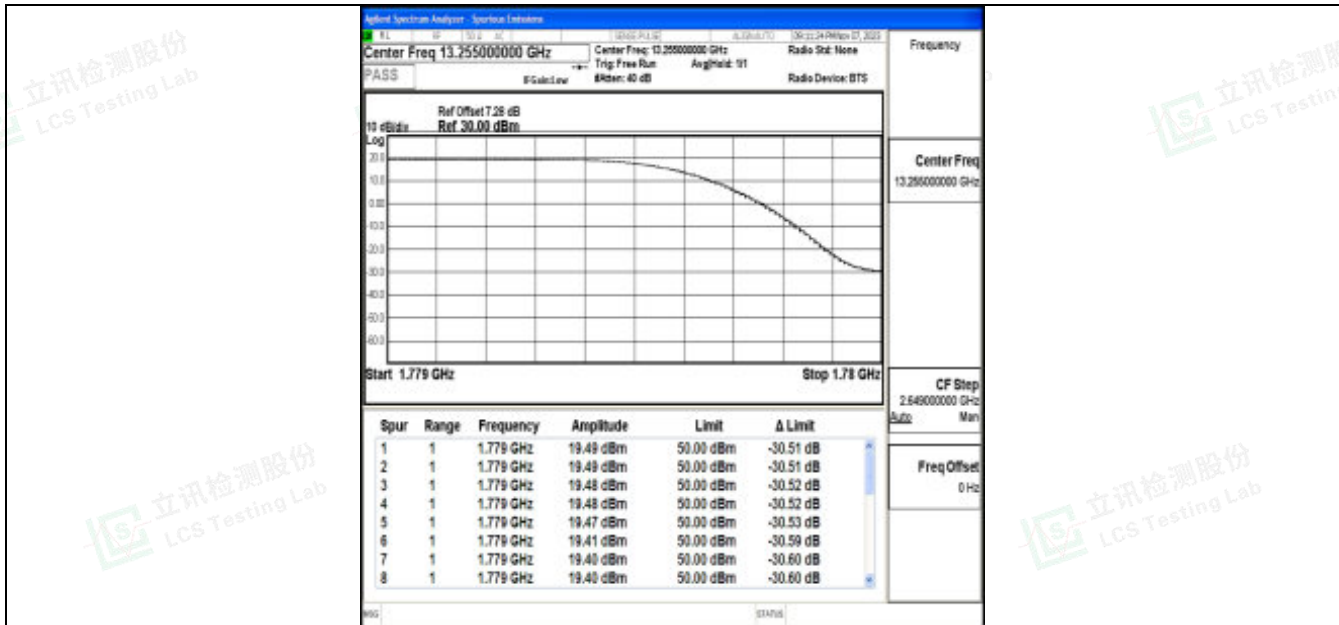
Band66_1.4MHz_16QAM_132665_1RB#0
