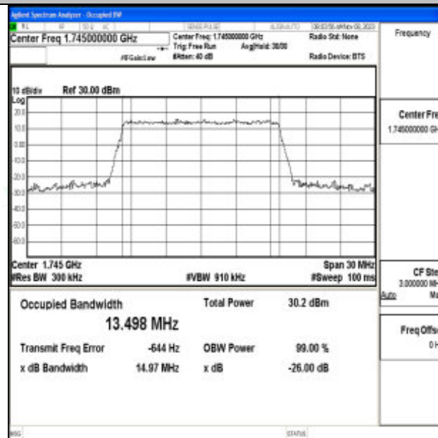
Band66-15MHz-64QAM-132322-75RB#0-PASS
