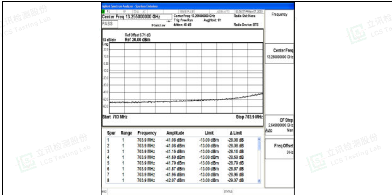
Band17_10MHz_QPSK_23780_1RB#0
