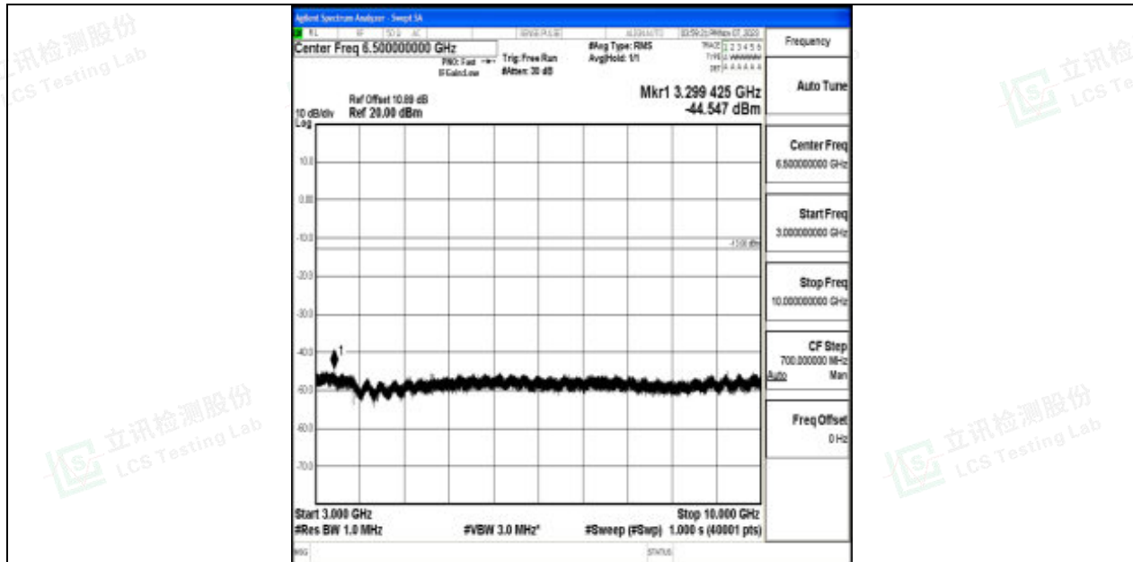
Band17_10MHz_QPSK_23800_1RB#0_3000~10000_3000~10000
