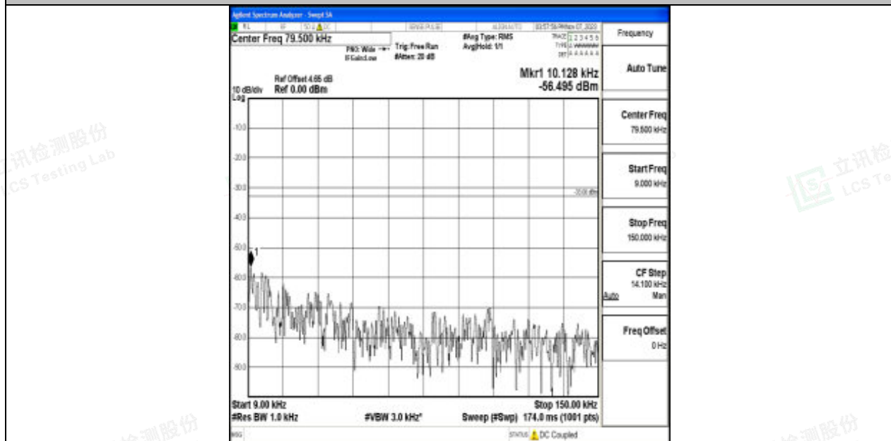
Band17_10MHz_64QAM_23790_1RB#0_0.009~0.15_0.009~0.15
