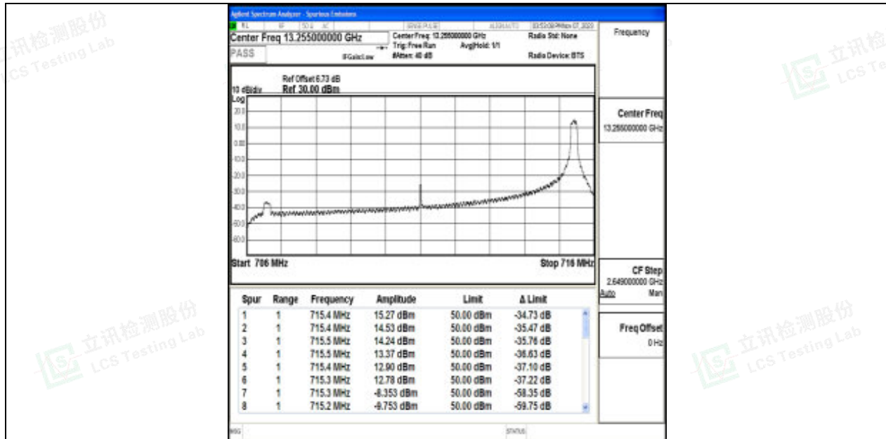
Band17_10MHz_64QAM_23800_1RB#49
