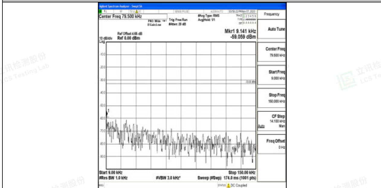
Band17_10MHz_QPSK_23790_1RB#0_0.009~0.15_0.009~0.15
