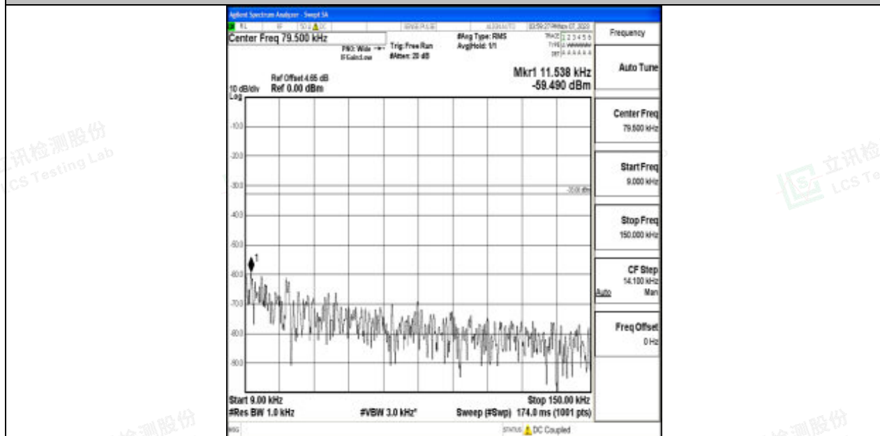
Band17_10MHz_16QAM_23800_1RB#0_0.009~0.15_0.009~0.15
