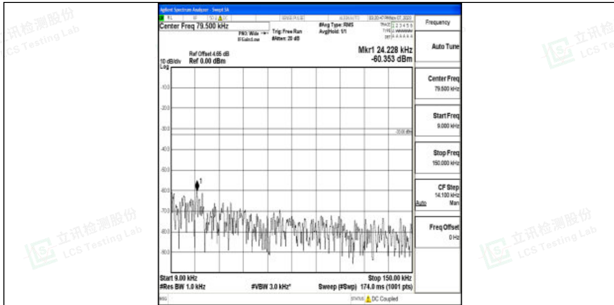
Band17_5MHz_16QAM_23755_1RB#0_0.009~0.15_0.009~0.15
