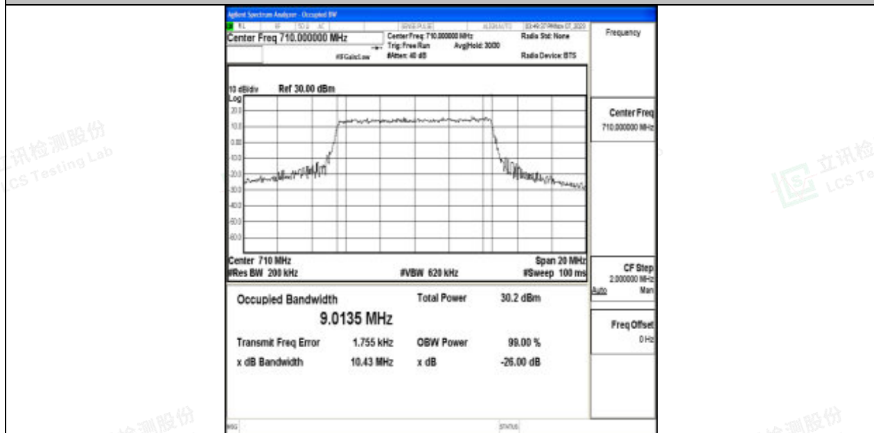
Band17-10MHz-16QAM-23790-50RB#0-PASS
