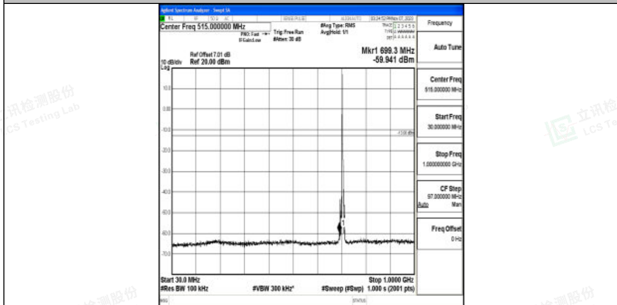
Band17_5MHz_QPSK_23825_1RB#0_30~1000_30~1000
