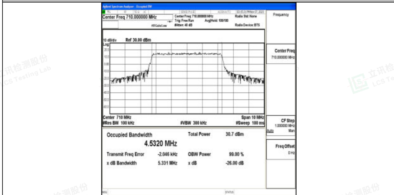
Band17-5MHz-64QAM-23790-25RB#0-PASS
