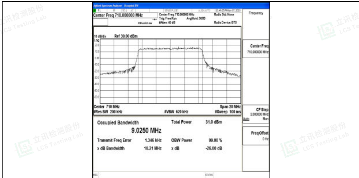
Band17-10MHz-QPSK-23790-50RB#0-PASS
