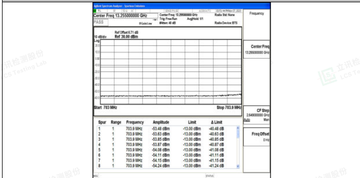
Band17_10MHz_64QAM_23780_1RB#49
