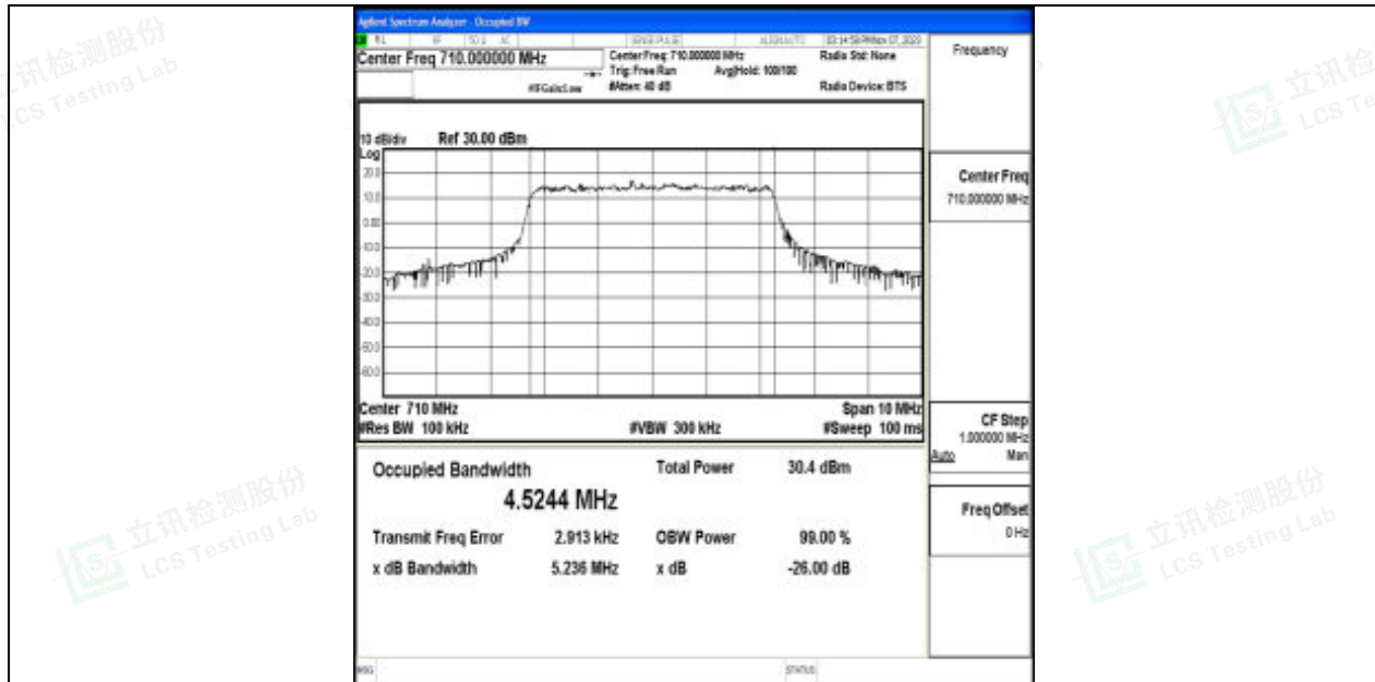
Band17-5MHz-16QAM-23790-25RB#0-PASS
