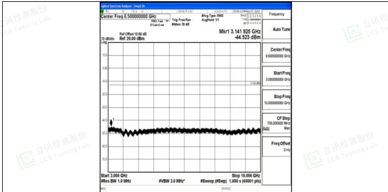
Band17_10MHz_64QAM_23780_1RB#0_3000~10000_3000~10000
