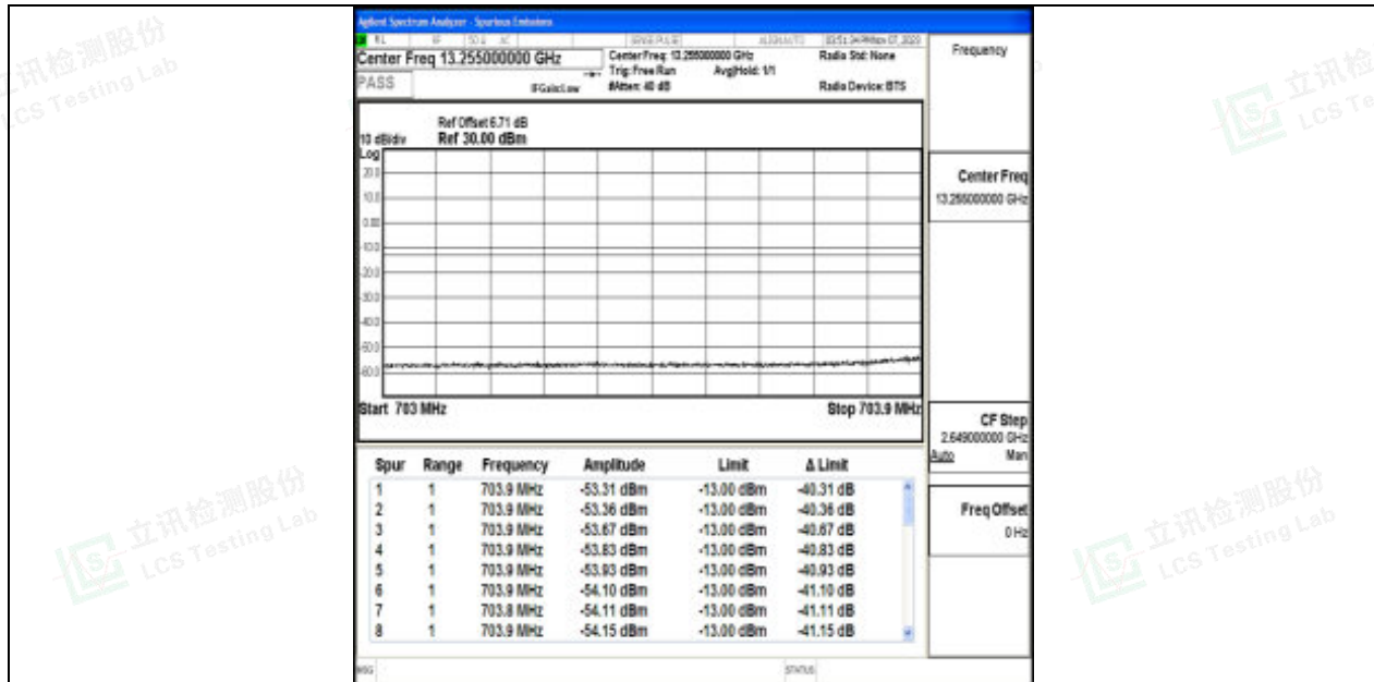
Band17_10MHz_16QAM_23780_1RB#49
