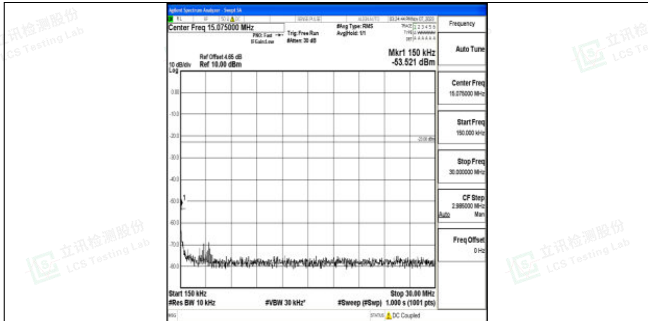
Band17_5MHz_QPSK_23825_1RB#0_0.15~30_0.15~30
