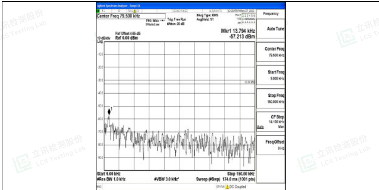
Band12_1.4MHz_16QAM_23017_1RB#0_0.009~0.15_0.009~0.15
