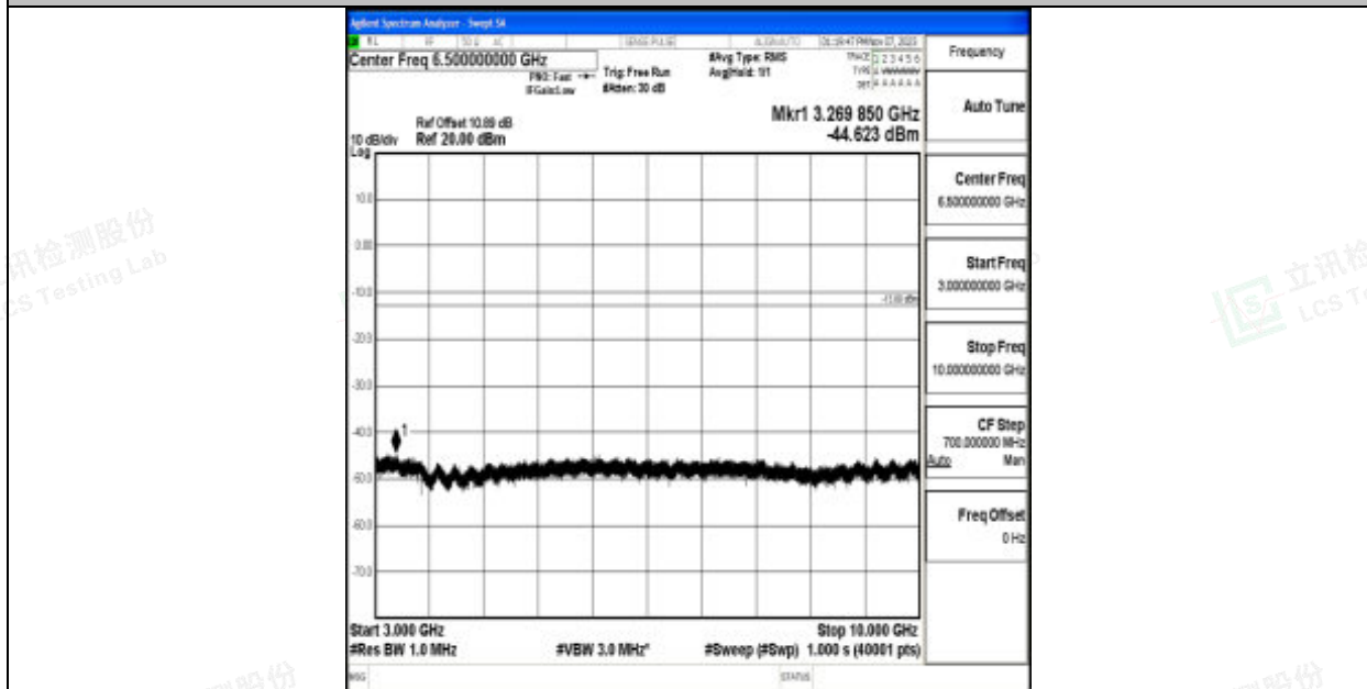
Band12_3MHz_16QAM_23025_1RB#0_3000~10000_3000~10000
