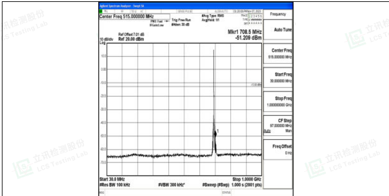
Band12_3MHz_64QAM_23025_1RB#0_30~1000_30~1000
