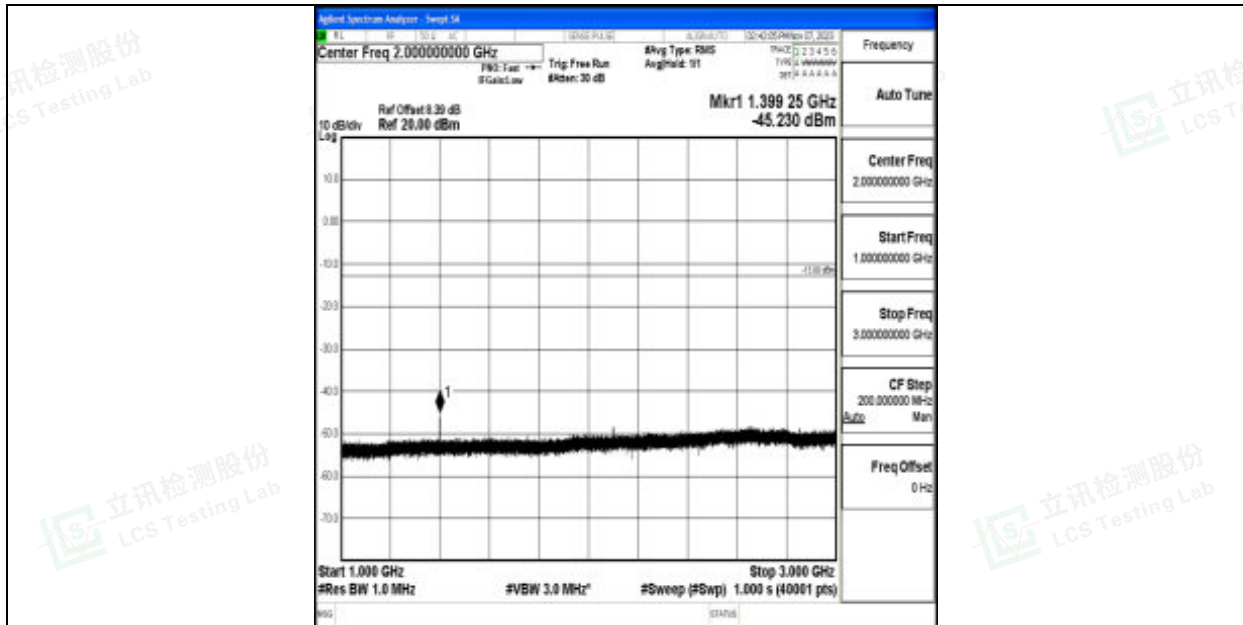
Band12_10MHz_16QAM_23060_1RB#0_1000~3000_1000~3000
