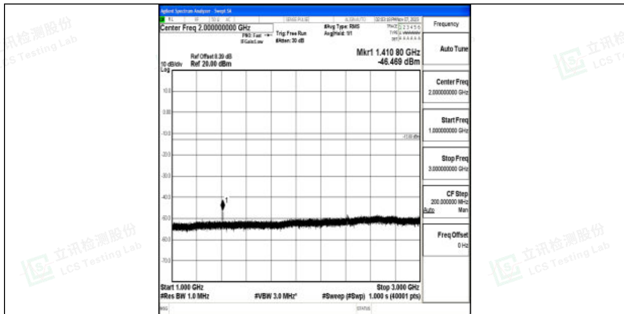
Band12_5MHz_16QAM_23095_1RB#0_1000~3000_1000~3000
