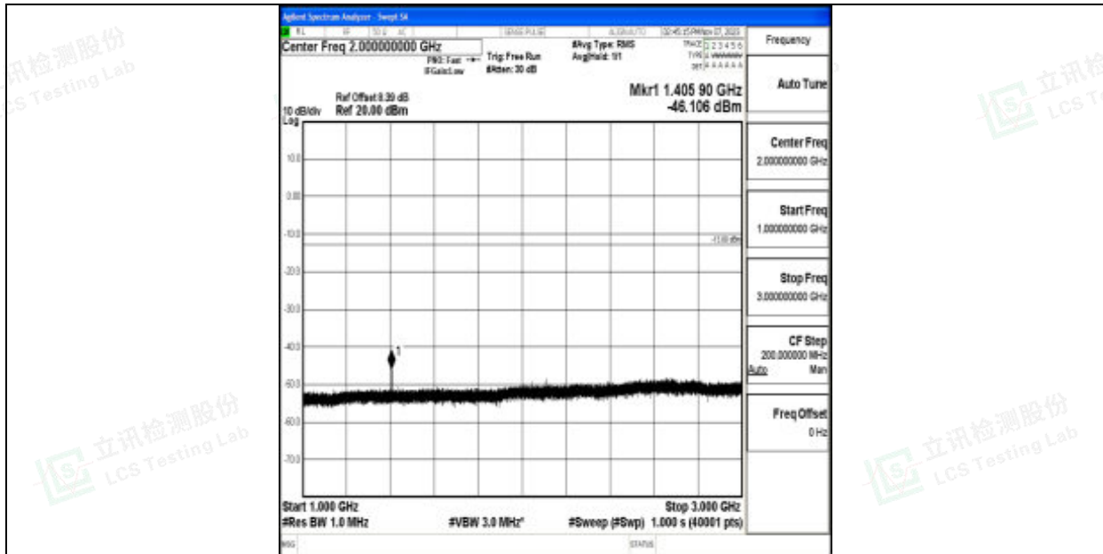
Band12_10MHz_64QAM_23095_1RB#0_1000~3000_1000~3000
