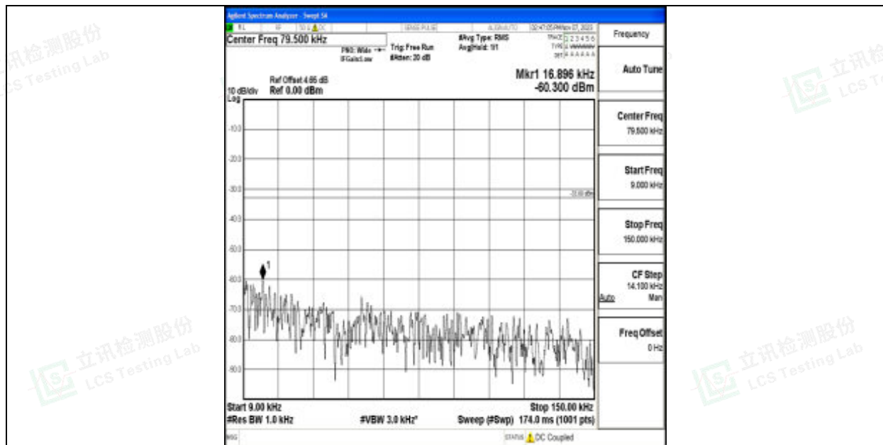
Band12_10MHz_64QAM_23130_1RB#0_0.009~0.15_0.009~0.15
