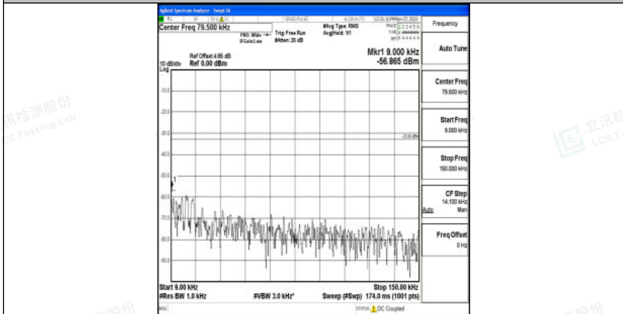
Band12_1.4MHz_16QAM_23095_1RB#0_0.009~0.15_0.009~0.15
