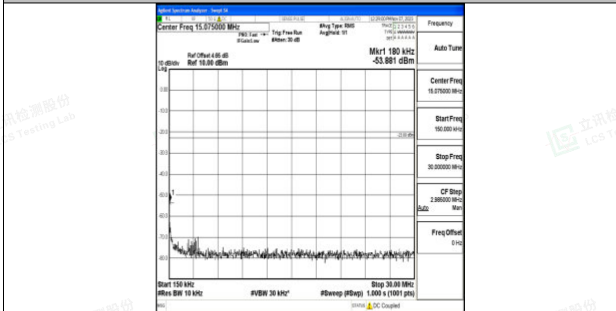
Band12_1.4MHz_16QAM_23017_1RB#0_0.15~30_0.15~30
