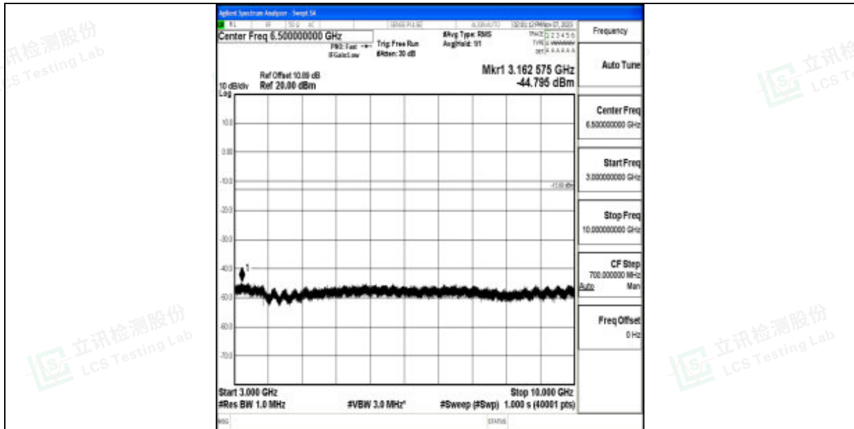
Band12_5MHz_16QAM_23035_1RB#0_3000~10000_3000~10000
