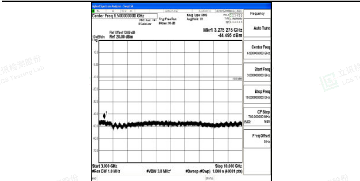
Band12_5MHz_64QAM_23035_1RB#0_3000~10000_3000~10000
