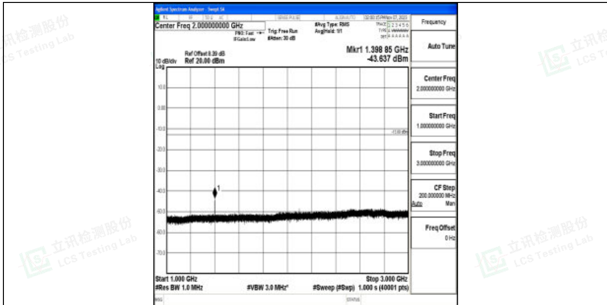
Band12_5MHz_QPSK_23035_1RB#0_1000~3000_1000~3000
