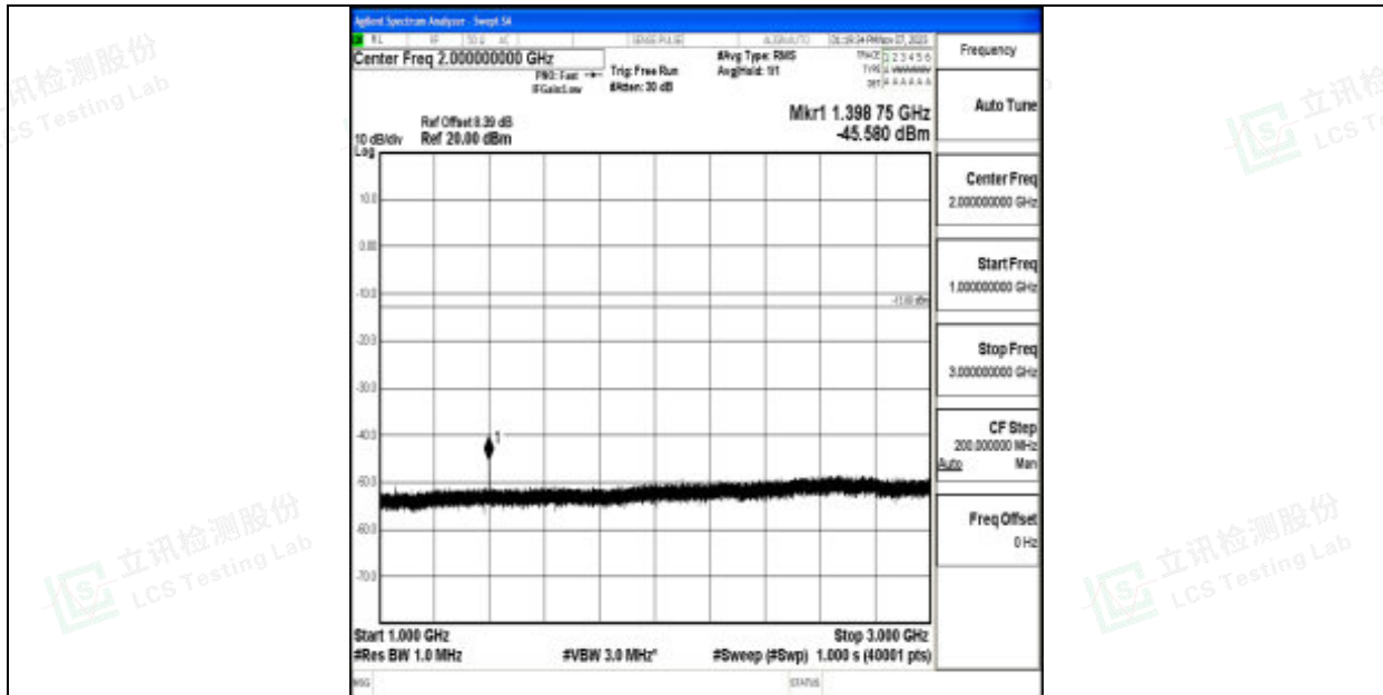
Band12_3MHz_16QAM_23025_1RB#0_1000~3000_1000~3000
