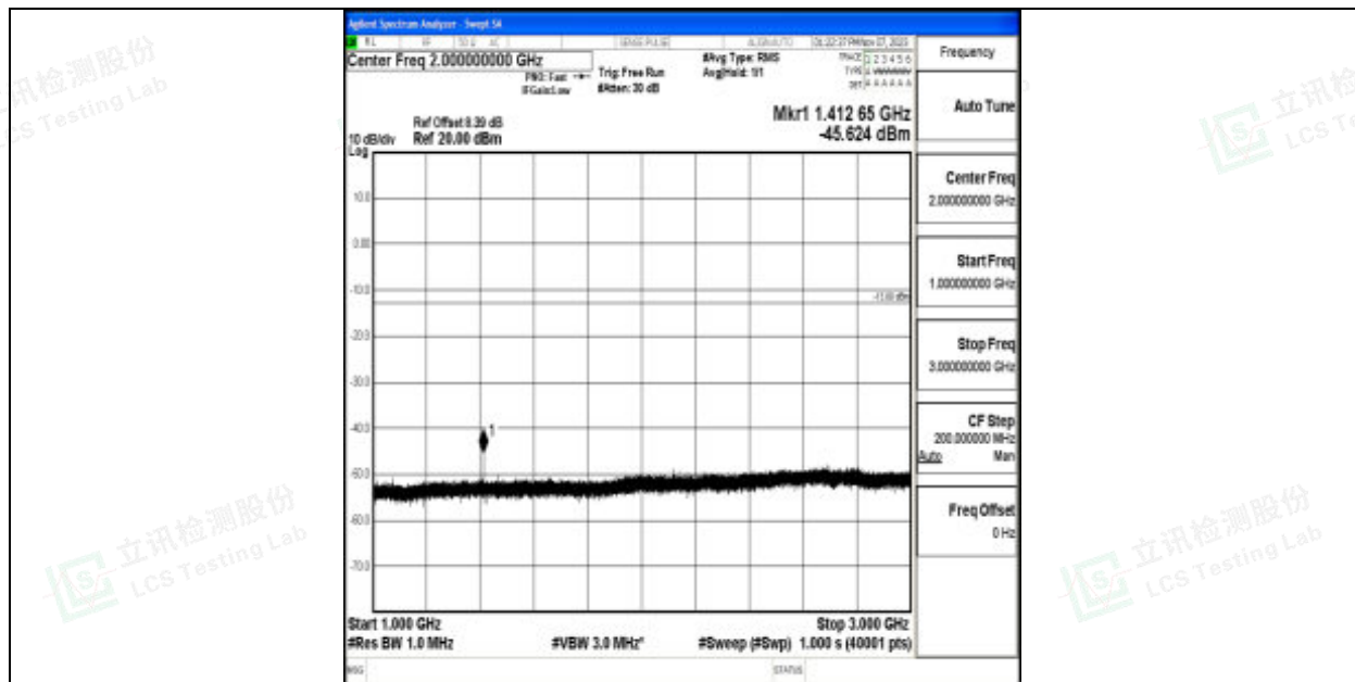
Band12_3MHz_64QAM_23095_1RB#0_1000~3000_1000~3000
