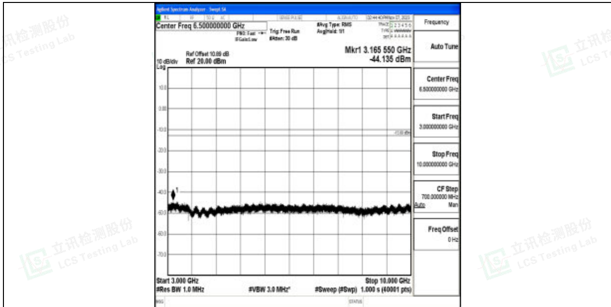
Band12_10MHz_16QAM_23095_1RB#0_3000~10000_3000~10000
