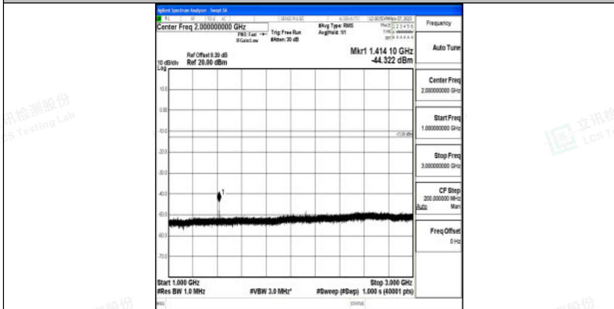
Band12_1.4MHz_QPSK_23095_1RB#0_1000~3000_1000~3000
