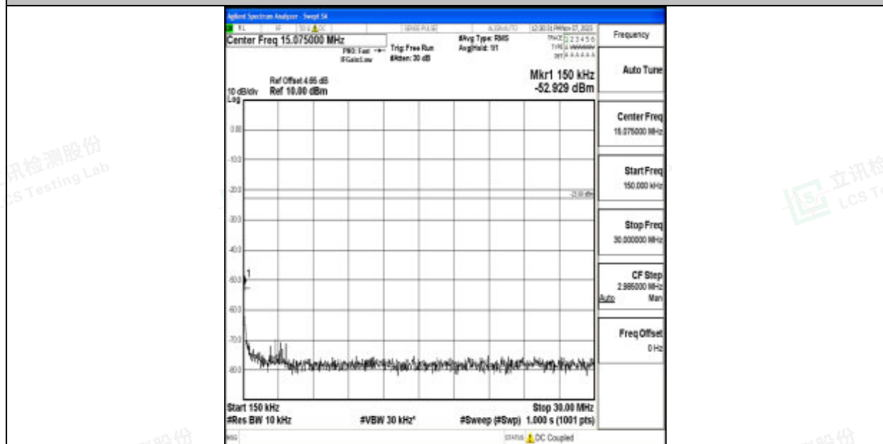
Band12_1.4MHz_QPSK_23095_1RB#0_0.15~30_0.15~30
