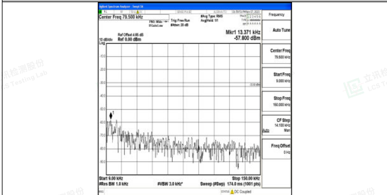
Band12_5MHz_QPSK_23035_1RB#0_0.009~0.15_0.009~0.15
