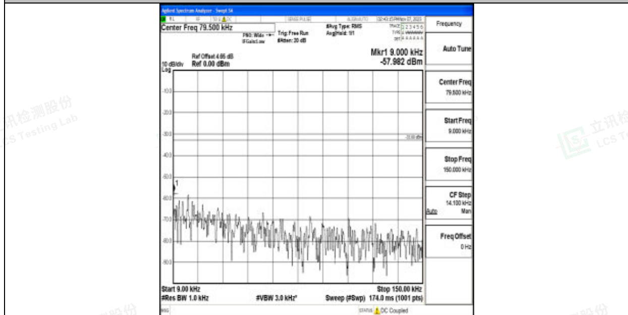
Band12_10MHz_QPSK_23095_1RB#0_0.009~0.15_0.009~0.15
