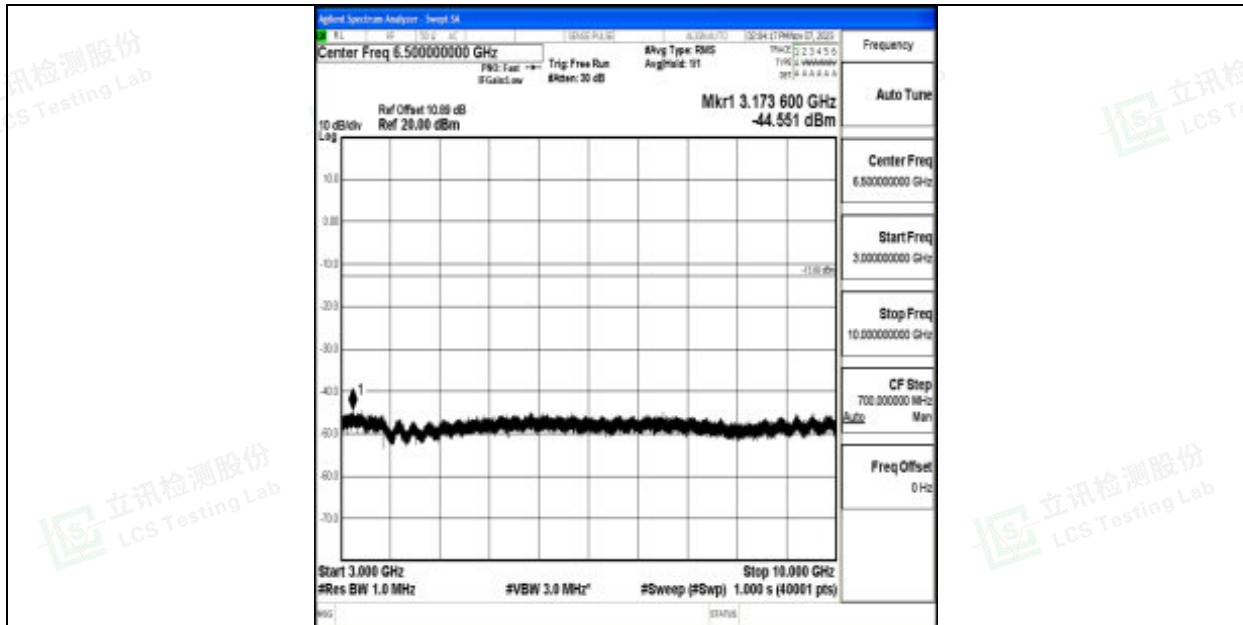
Band12_5MHz_64QAM_23095_1RB#0_3000~10000_3000~10000
