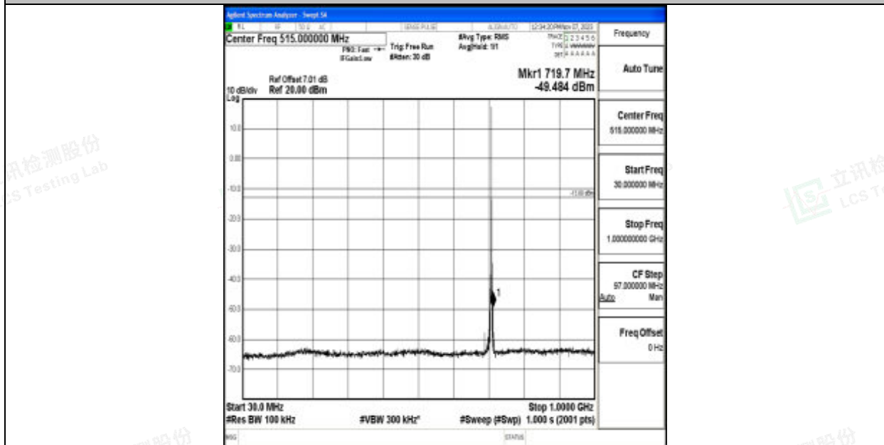
Band12_1.4MHz_64QAM_23173_1RB#0_30~1000_30~1000
