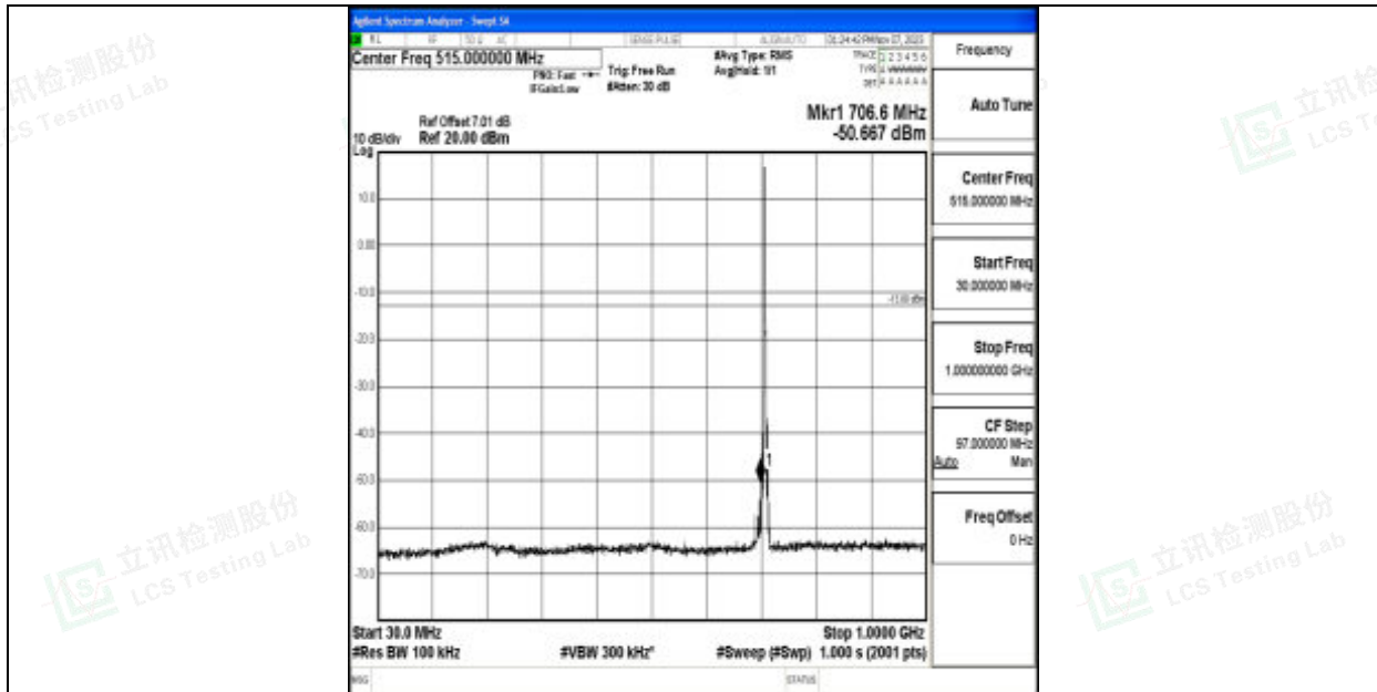
Band12_3MHz_64QAM_23165_1RB#0_30~1000_30~1000
