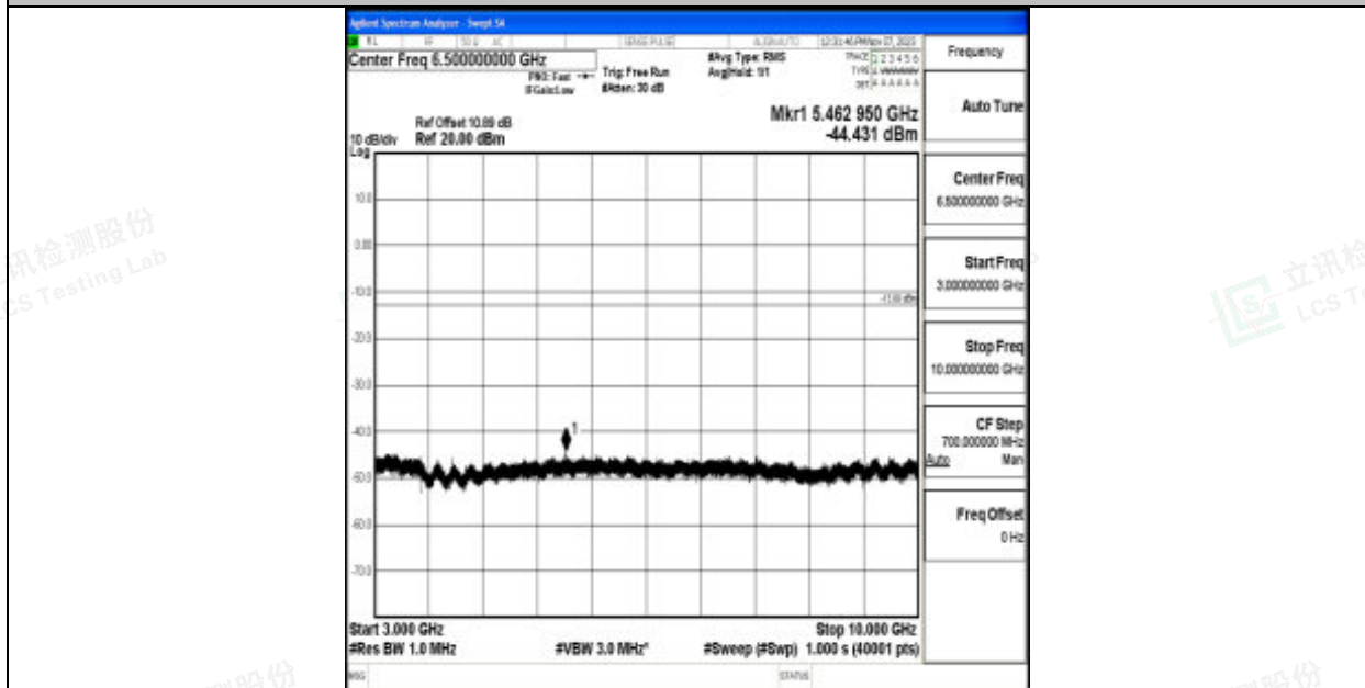
Band12_1.4MHz_16QAM_23095_1RB#0_3000~10000_3000~10000
