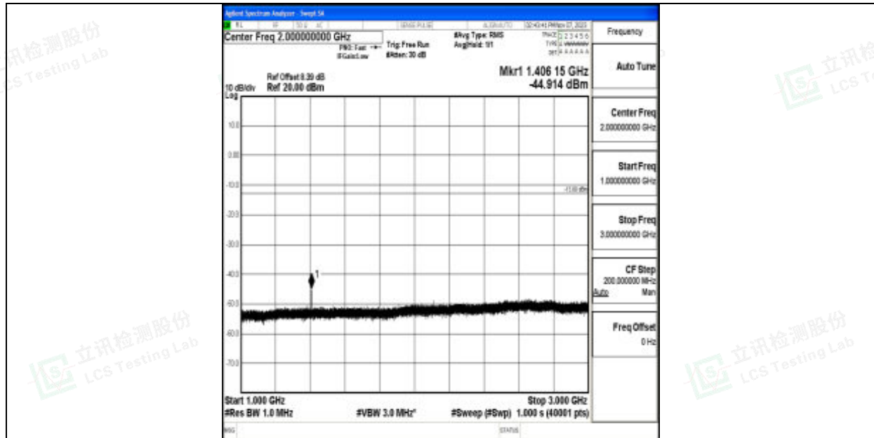
Band12_10MHz_QPSK_23095_1RB#0_1000~3000_1000~3000
