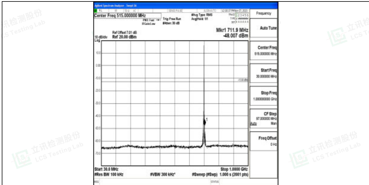
Band12_1.4MHz_QPSK_23095_1RB#0_30~1000_30~1000
