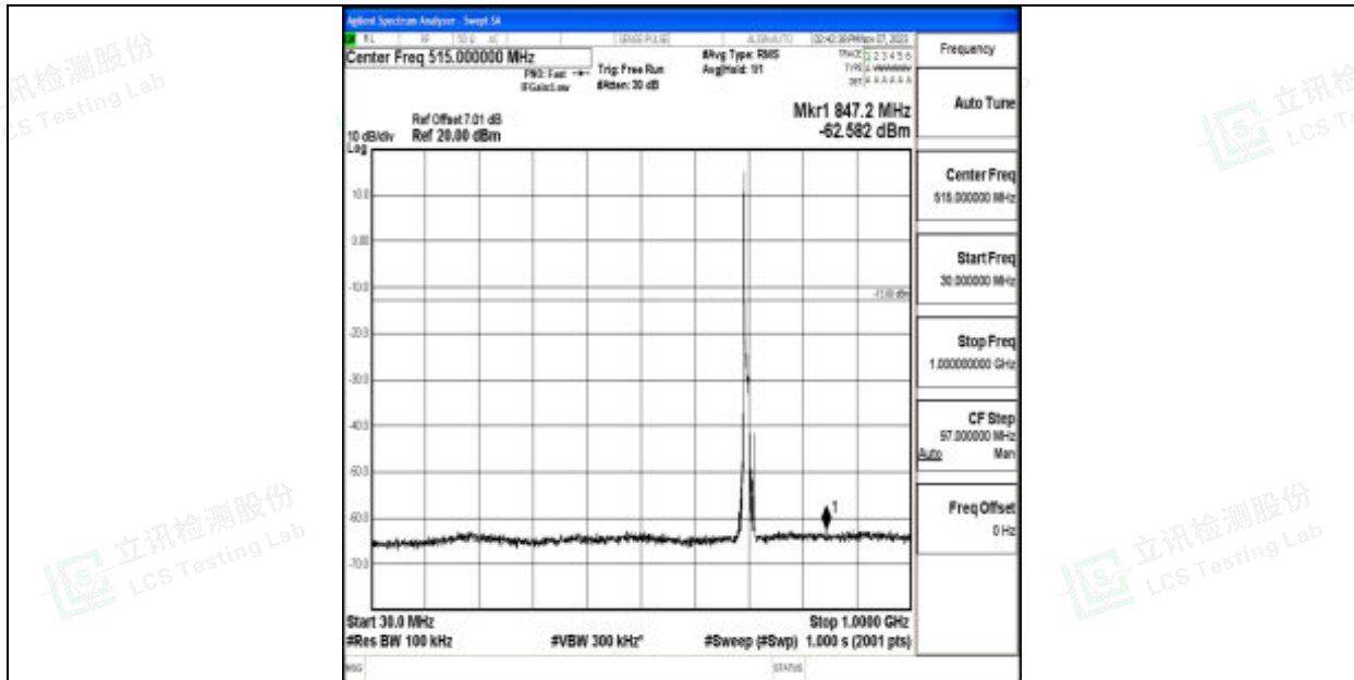
Band12_10MHz_64QAM_23060_1RB#0_30~1000_30~1000
