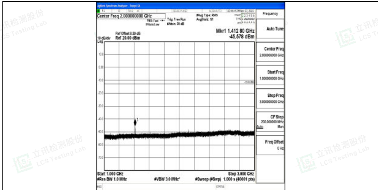
Band12_10MHz_16QAM_23130_1RB#0_1000~3000_1000~3000
