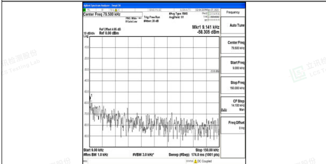
Band12_5MHz_QPSK_23155_1RB#0_0.009~0.15_0.009~0.15
