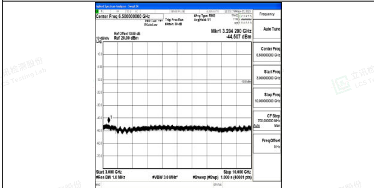
Band12_1.4MHz_QPSK_23173_1RB#0_3000~10000_3000~10000
