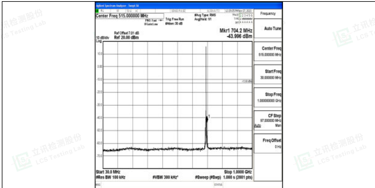
Band12_1.4MHz_16QAM_23017_1RB#0_30~1000_30~1000
