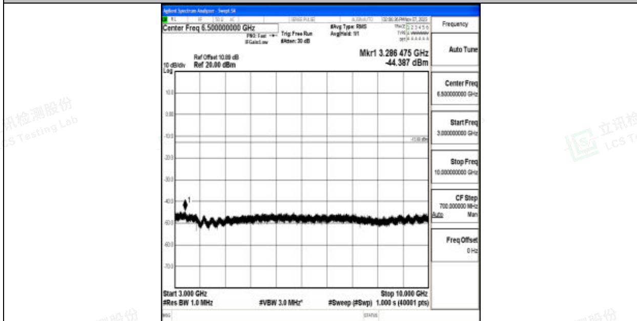
Band12_5MHz_64QAM_23155_1RB#0_3000~10000_3000~10000
