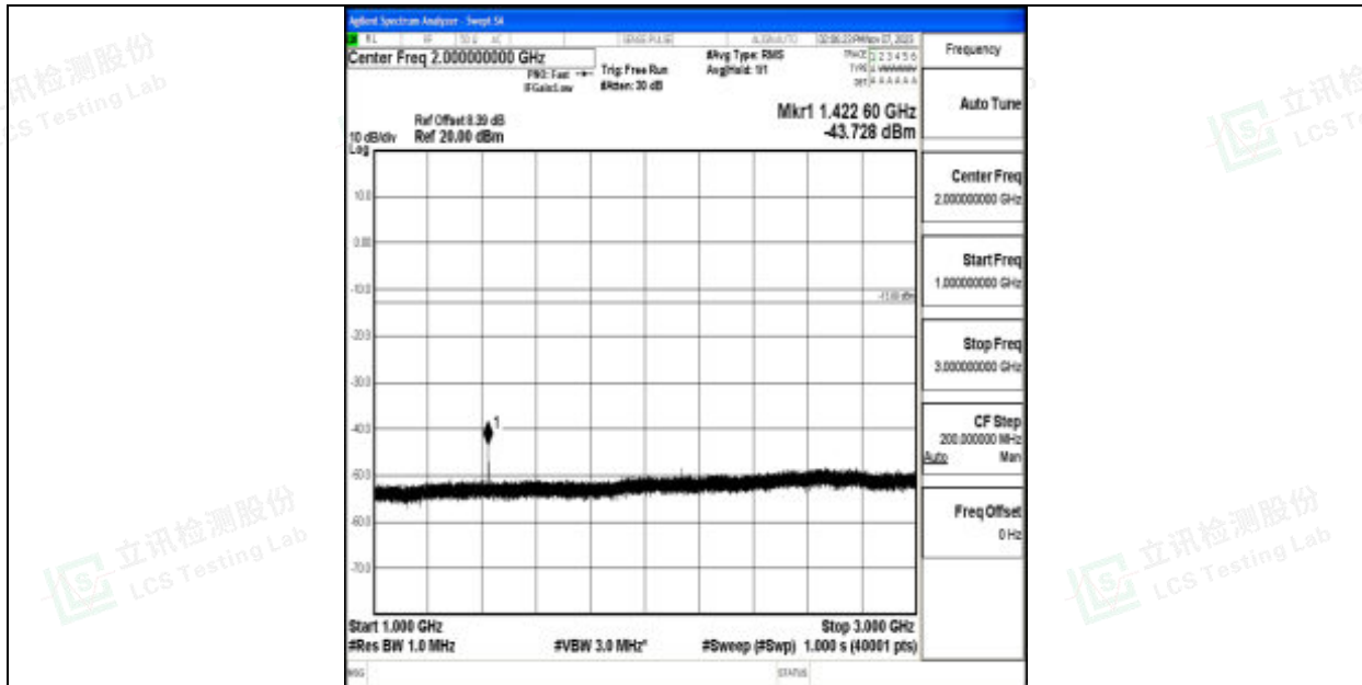
Band12_5MHz_64QAM_23155_1RB#0_1000~3000_1000~3000
