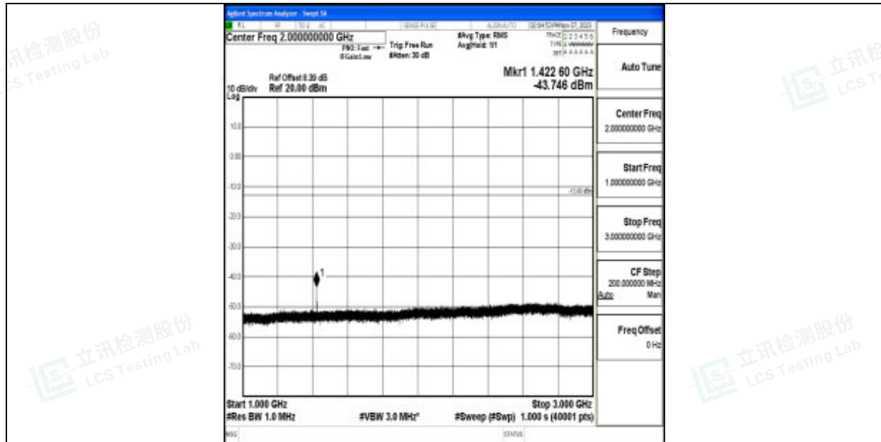
Band12_5MHz_QPSK_23155_1RB#0_1000~3000_1000~3000
