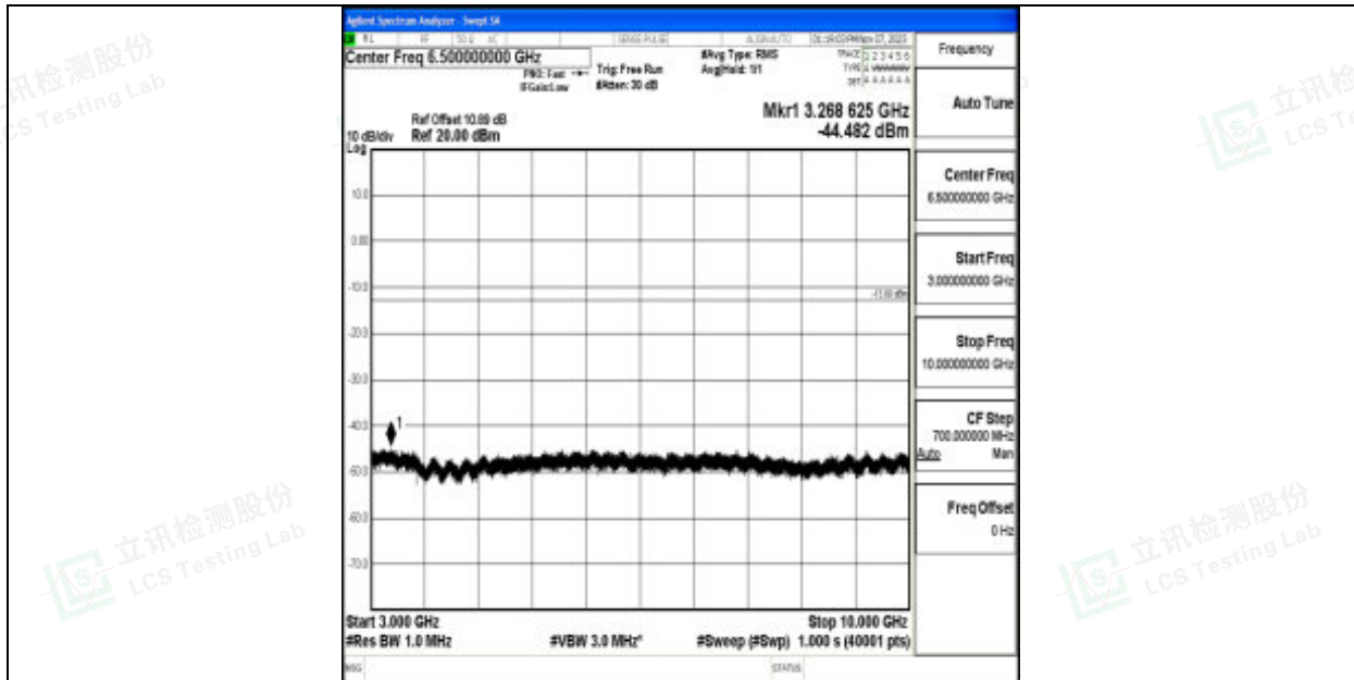
Band12_3MHz_QPSK_23025_1RB#0_3000~10000_3000~10000
