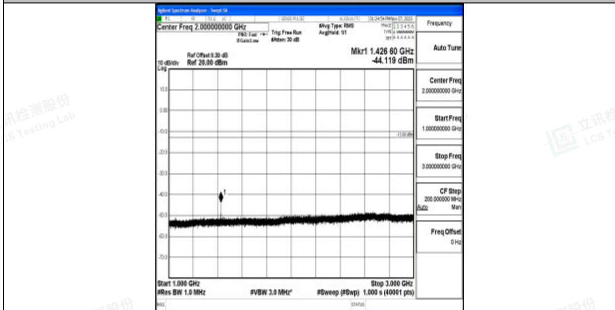
Band12_3MHz_64QAM_23165_1RB#0_1000~3000_1000~3000
