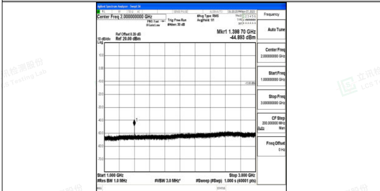
Band12_3MHz_64QAM_23025_1RB#0_1000~3000_1000~3000
