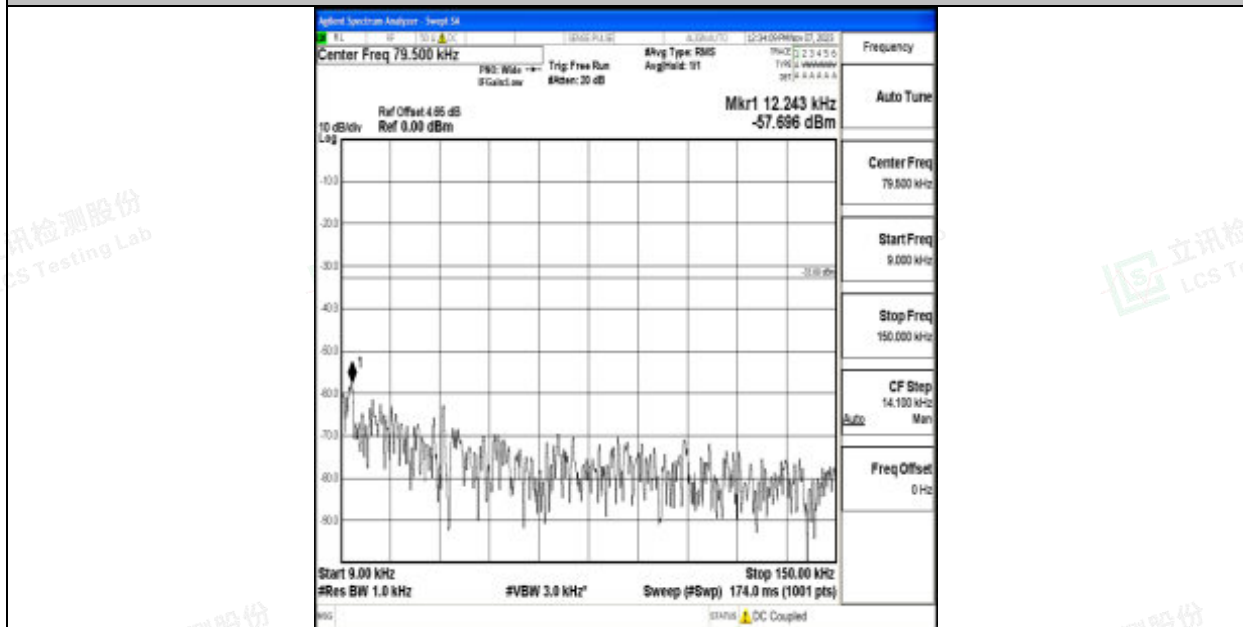
Band12_1.4MHz_64QAM_23173_1RB#0_0.009~0.15_0.009~0.15
