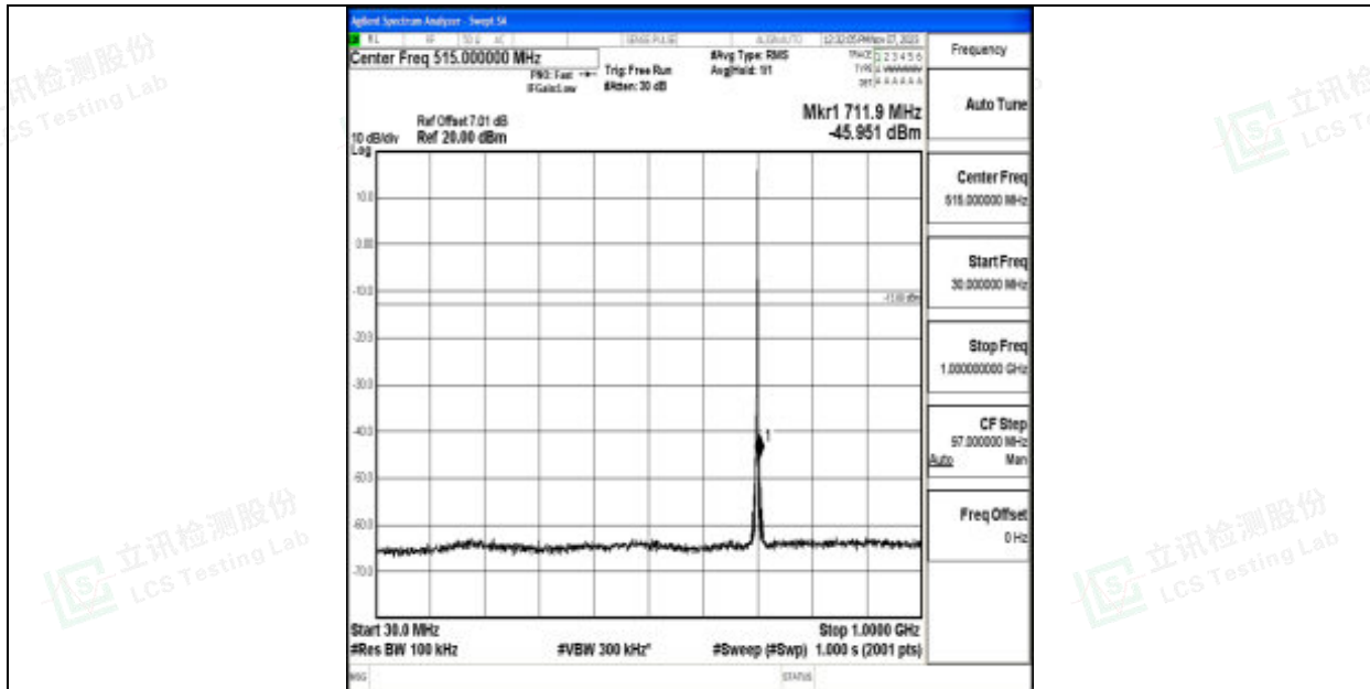
Band12_1.4MHz_64QAM_23095_1RB#0_30~1000_30~1000
