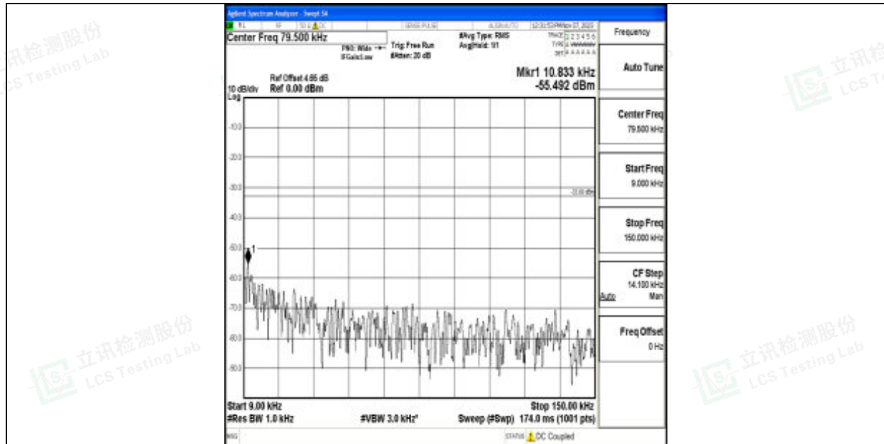
Band12_1.4MHz_64QAM_23095_1RB#0_0.009~0.15_0.009~0.15
