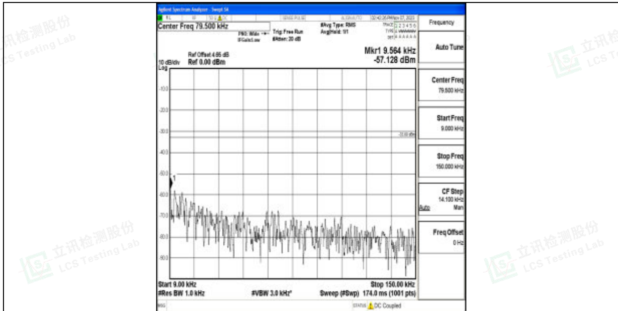
Band12_10MHz_64QAM_23060_1RB#0_0.009~0.15_0.009~0.15
