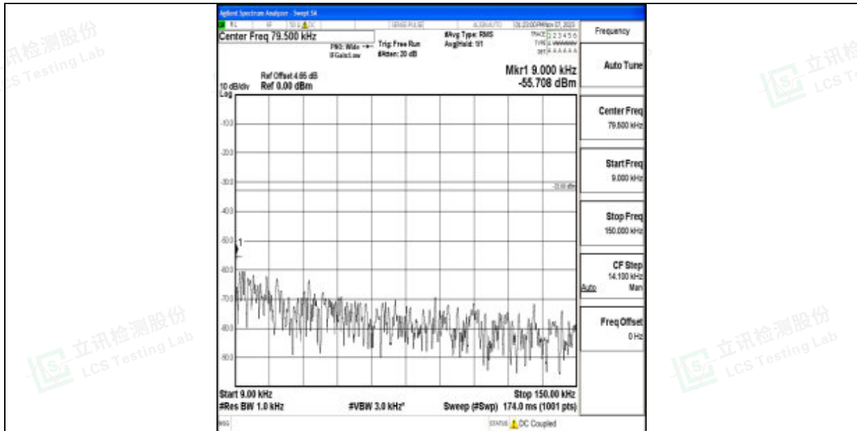
Band12_3MHz_QPSK_23165_1RB#0_0.009~0.15_0.009~0.15
