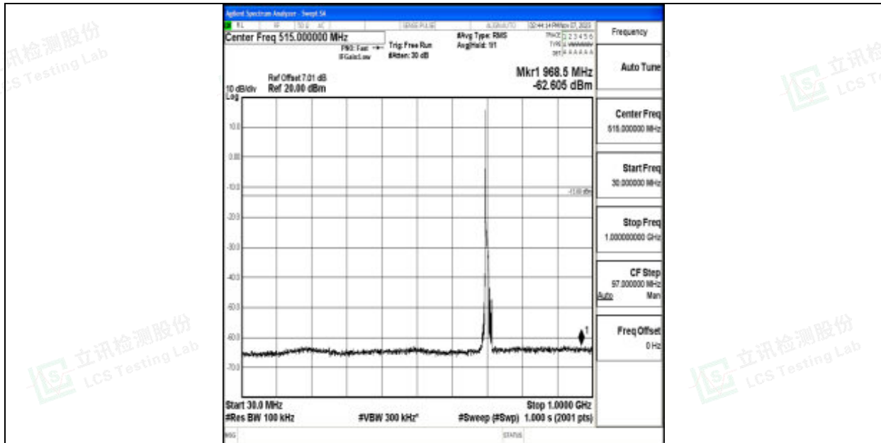
Band12_10MHz_16QAM_23095_1RB#0_30~1000_30~1000
