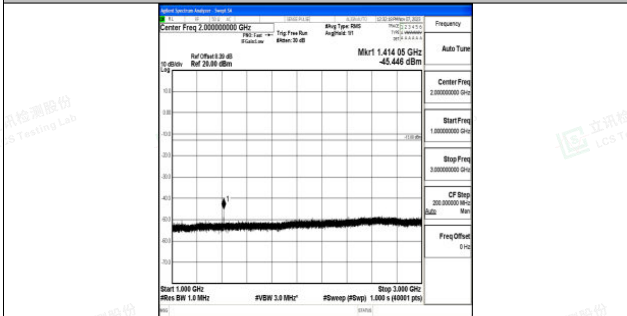
Band12_1.4MHz_64QAM_23095_1RB#0_1000~3000_1000~3000
