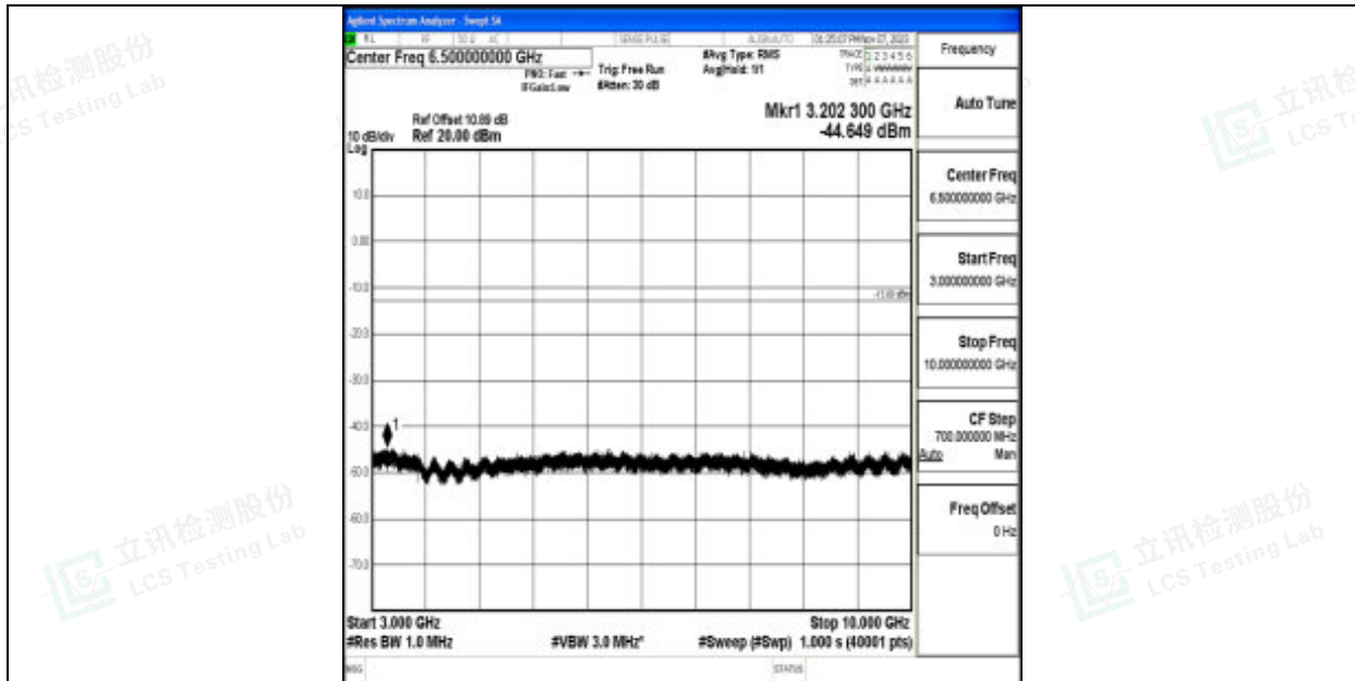
Band12_3MHz_64QAM_23165_1RB#0_3000~10000_3000~10000
