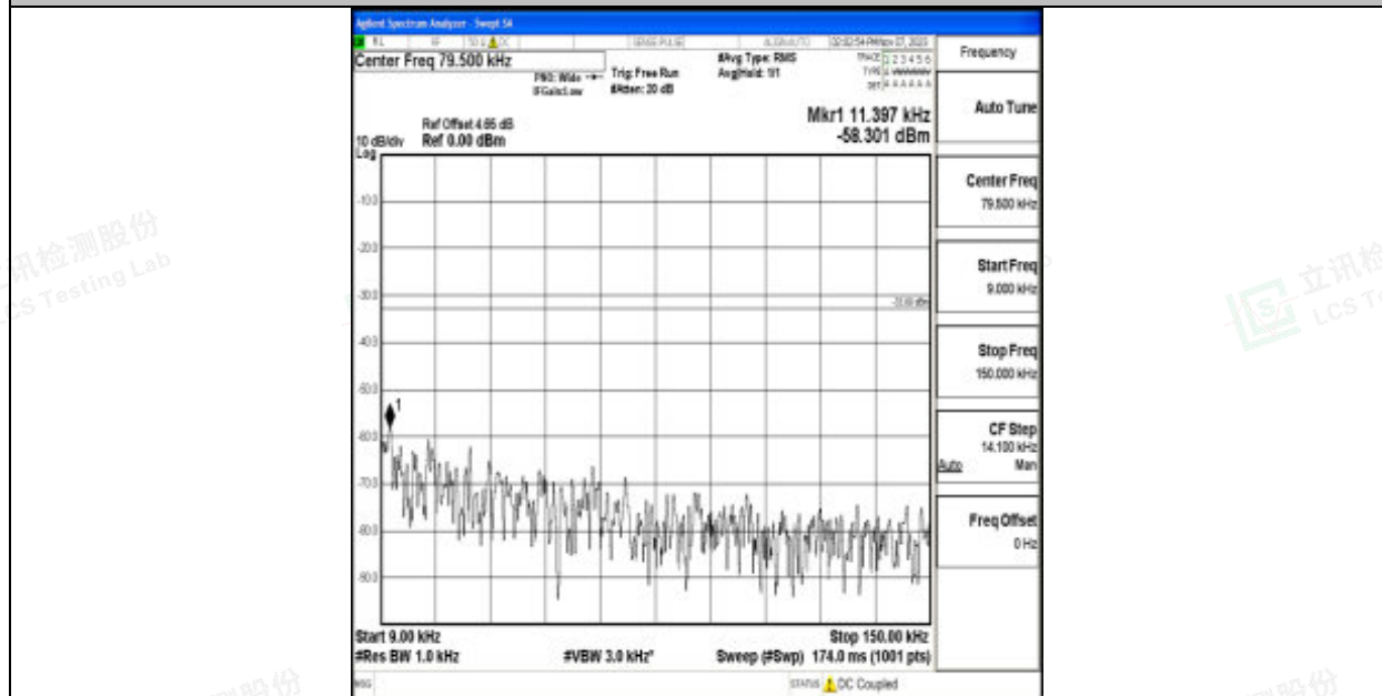
Band12_5MHz_16QAM_23095_1RB#0_0.009~0.15_0.009~0.15
