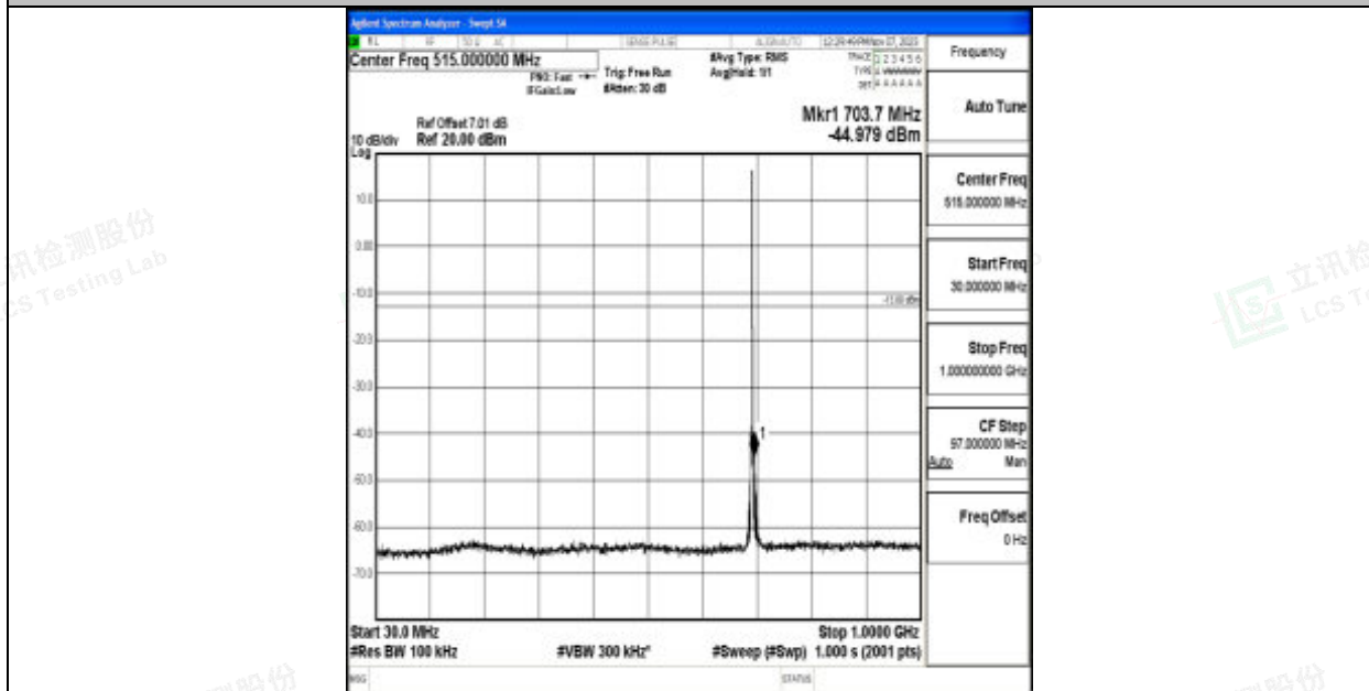
Band12_1.4MHz_64QAM_23017_1RB#0_30~1000_30~1000
