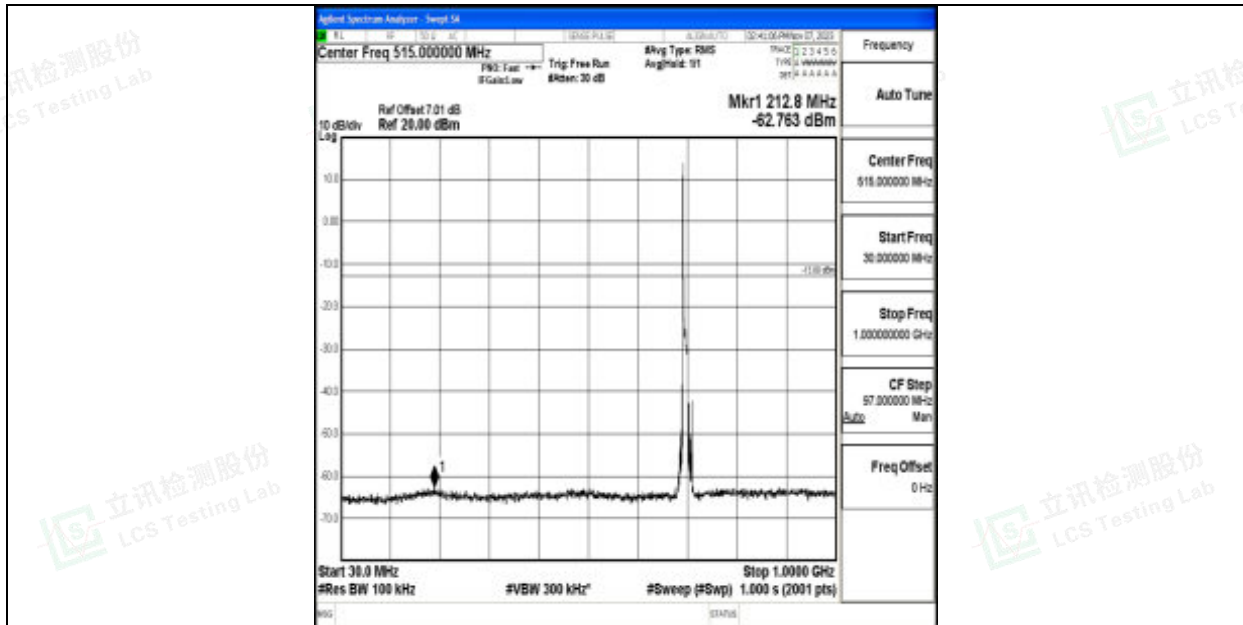
Band12_10MHz_QPSK_23060_1RB#0_30~1000_30~1000
