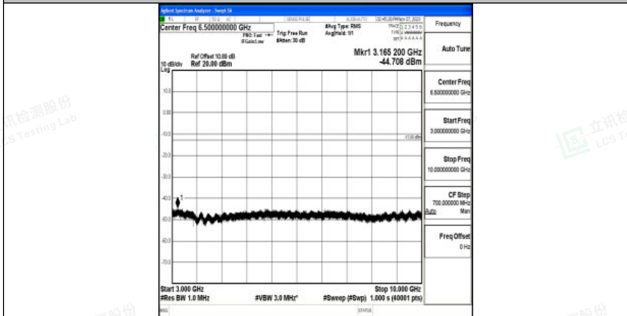
Band12_10MHz_64QAM_23095_1RB#0_3000~10000_3000~10000
