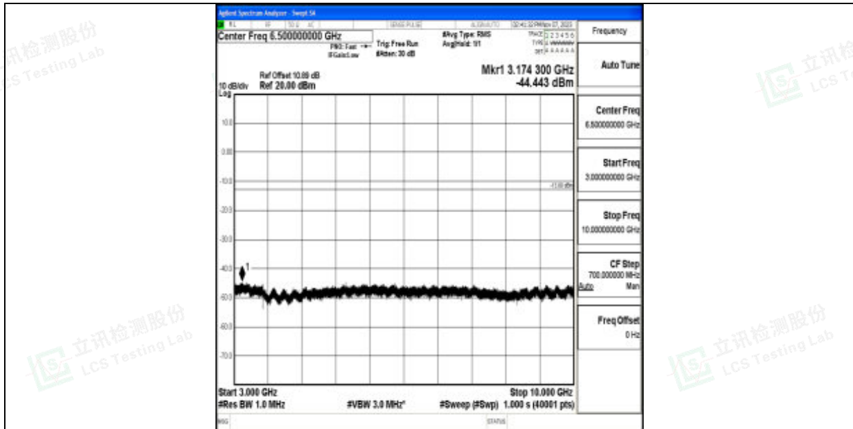
Band12_10MHz_QPSK_23060_1RB#0_3000~10000_3000~10000
