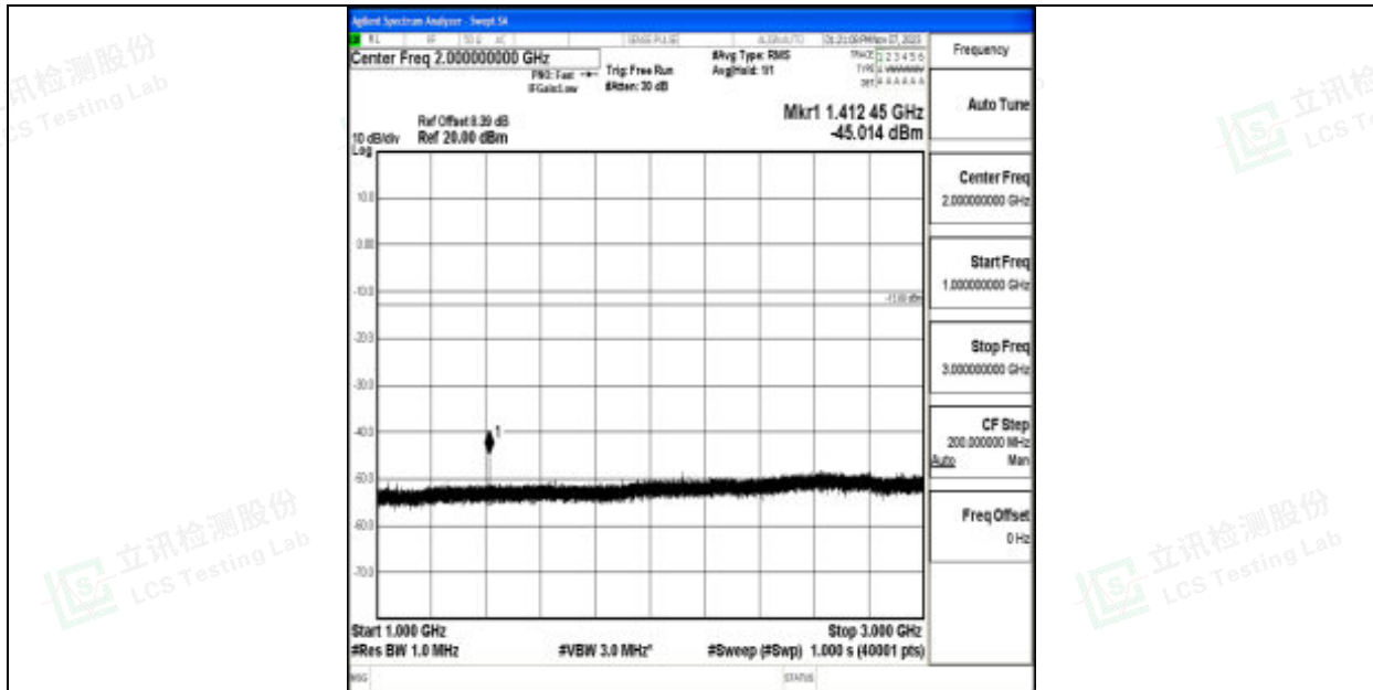
Band12_3MHz_QPSK_23095_1RB#0_1000~3000_1000~3000
