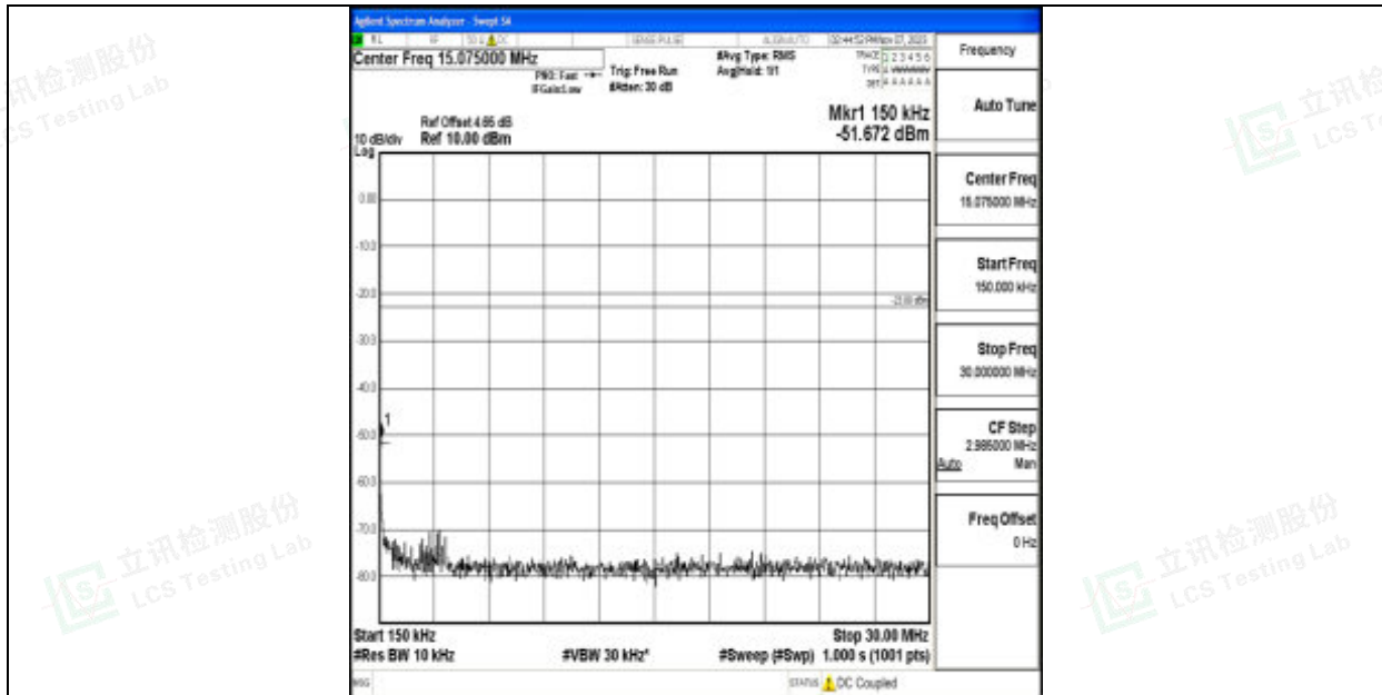
Band12_10MHz_64QAM_23095_1RB#0_0.15~30_0.15~30
