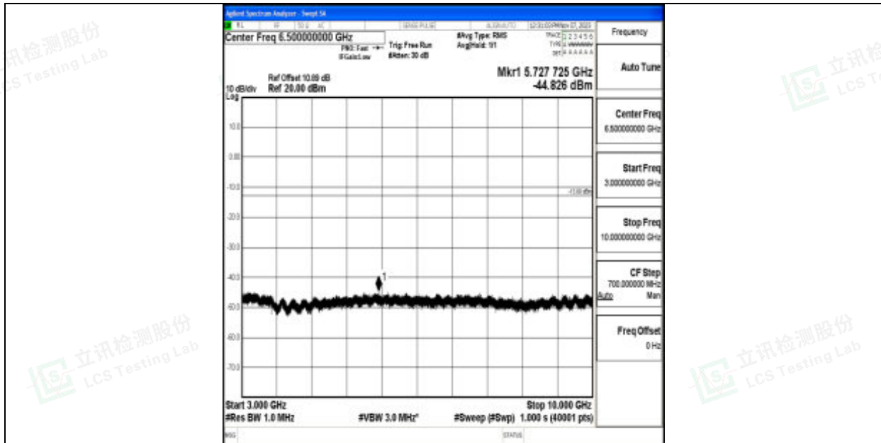
Band12_1.4MHz_QPSK_23095_1RB#0_3000~10000_3000~10000
