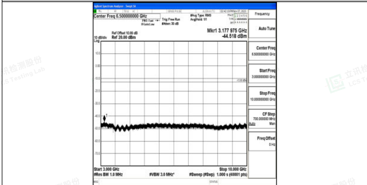
Band12_10MHz_16QAM_23060_1RB#0_3000~10000_3000~10000
