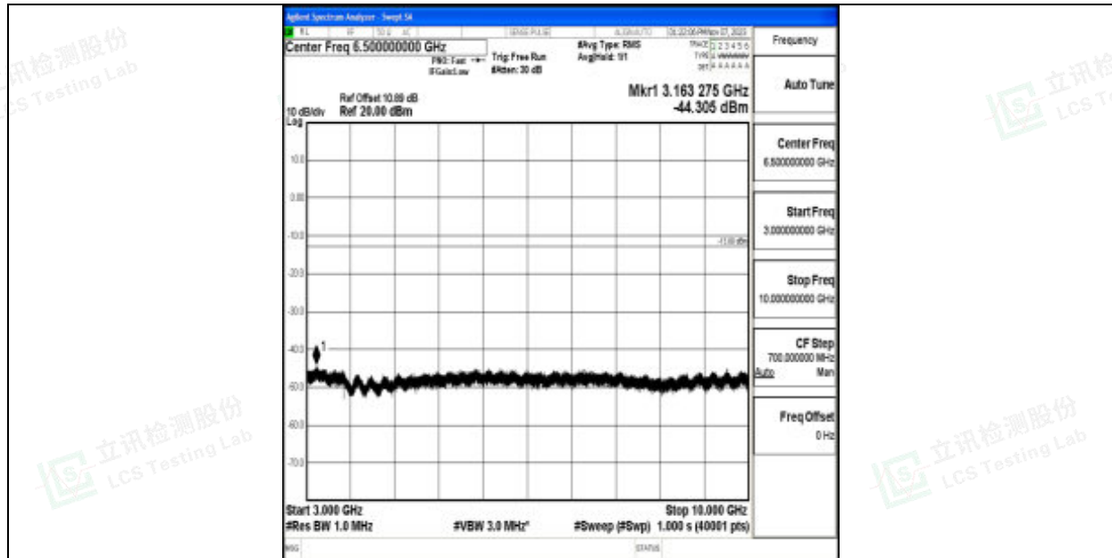
Band12_3MHz_16QAM_23095_1RB#0_3000~10000_3000~10000
