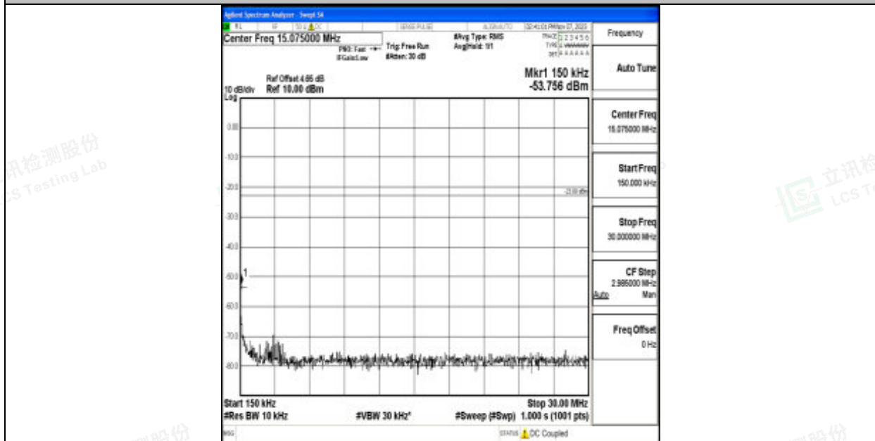
Band12_10MHz_QPSK_23060_1RB#0_0.15~30_0.15~30
