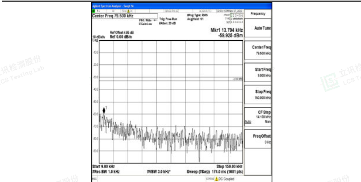
Band12_5MHz_64QAM_23035_1RB#0_0.009~0.15_0.009~0.15
