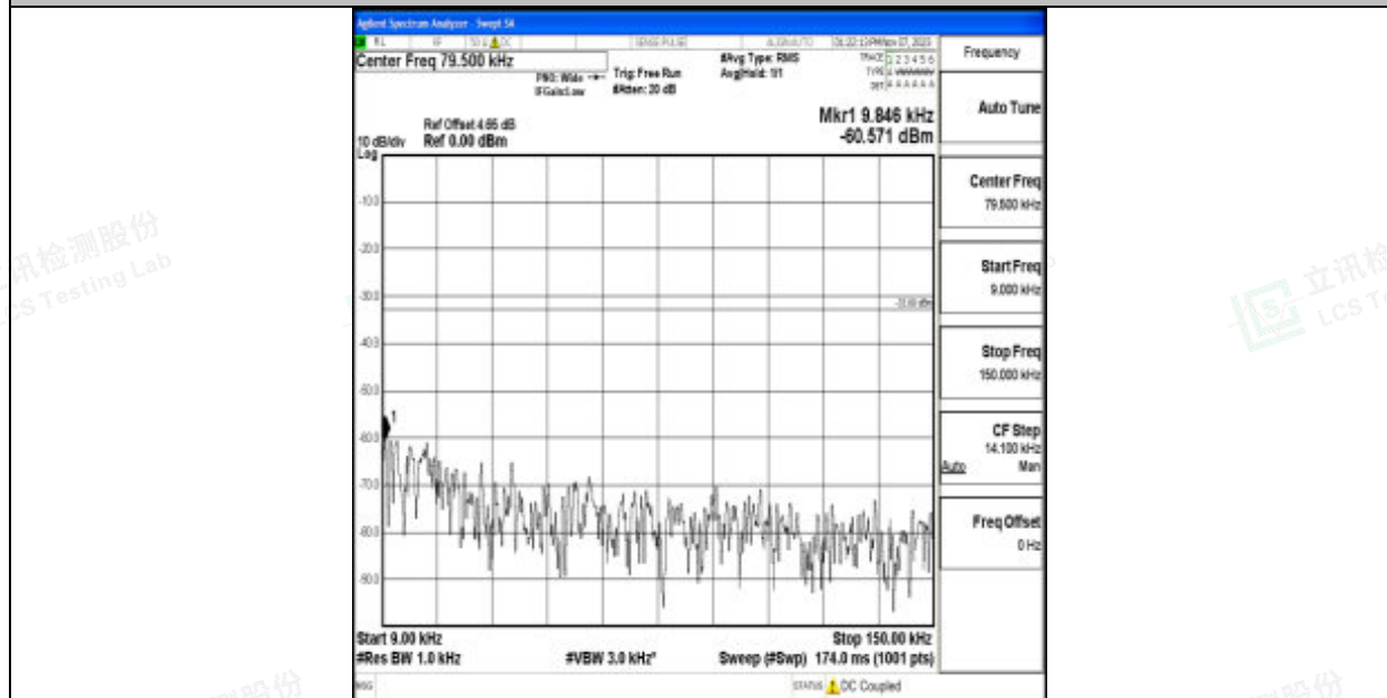
Band12_3MHz_64QAM_23095_1RB#0_0.009~0.15_0.009~0.15
