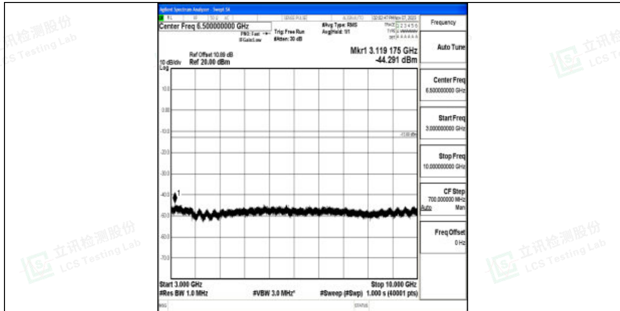
Band12_5MHz_QPSK_23095_1RB#0_3000~10000_3000~10000
