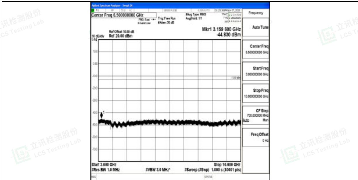
Band12_3MHz_QPSK_23165_1RB#0_3000~10000_3000~10000
