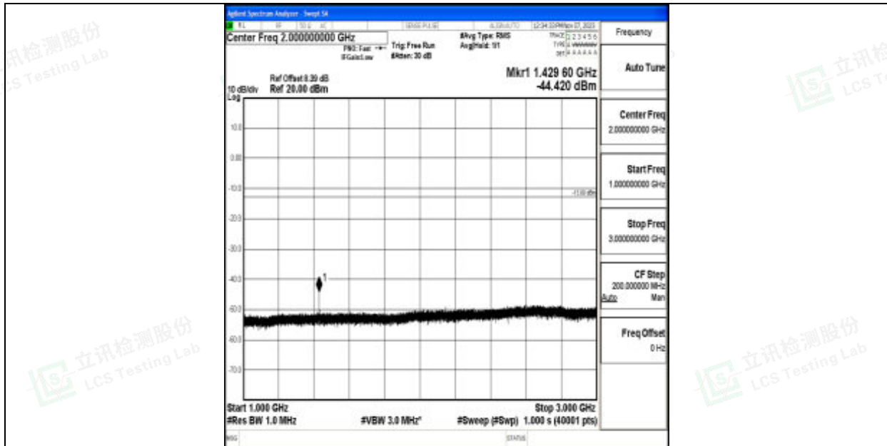
Band12_1.4MHz_64QAM_23173_1RB#0_1000~3000_1000~3000
