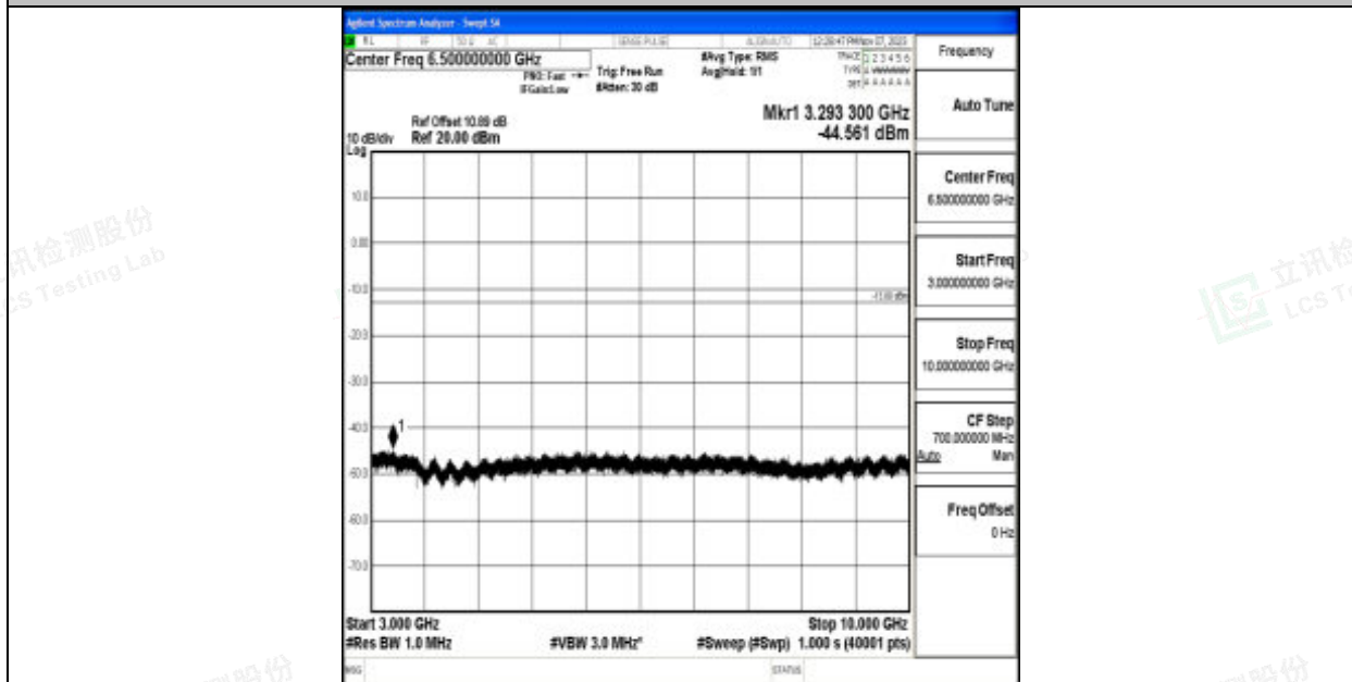
Band12_1.4MHz_QPSK_23017_1RB#0_3000~10000_3000~10000
