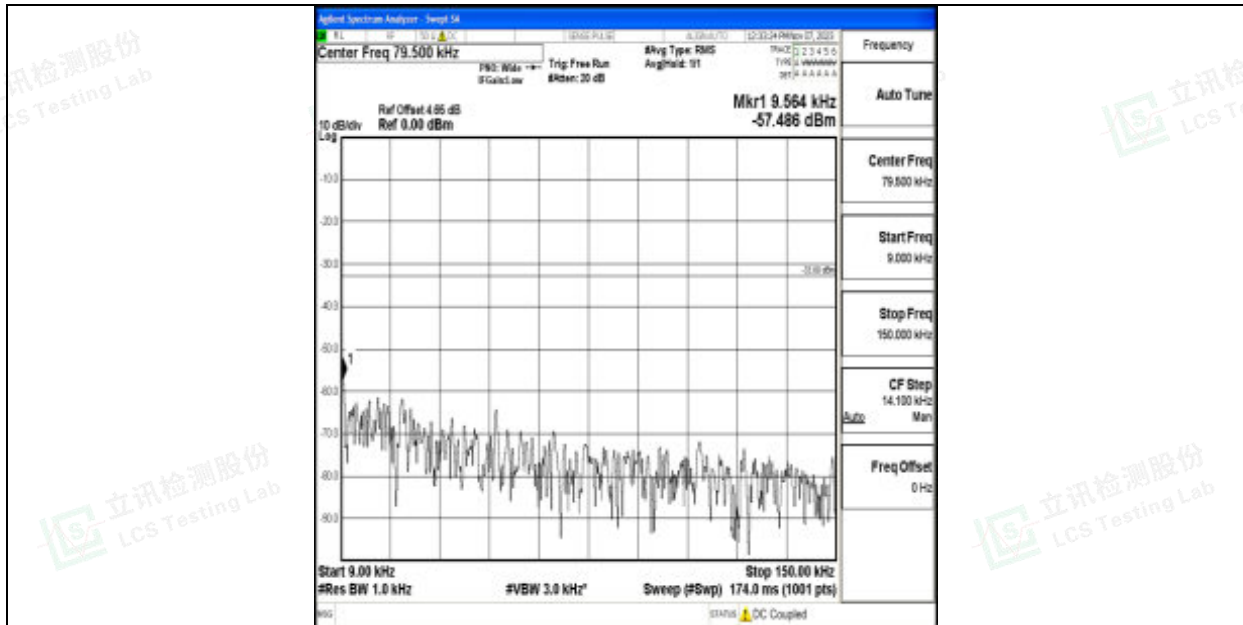
Band12_1.4MHz_16QAM_23173_1RB#0_0.009~0.15_0.009~0.15
