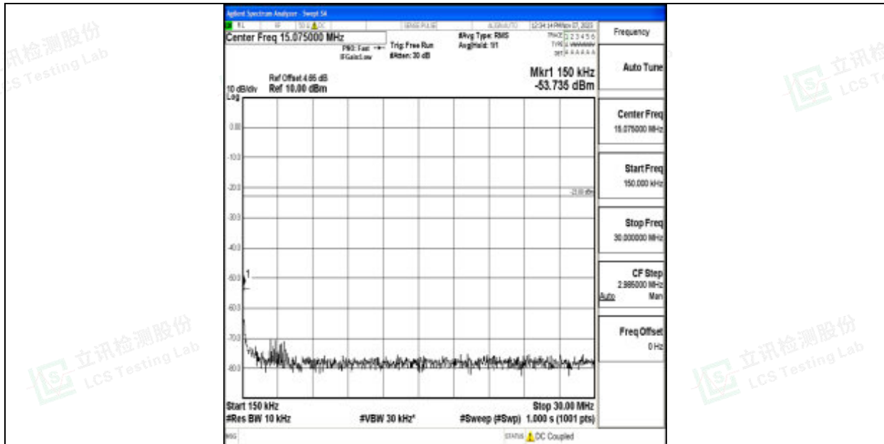
Band12_1.4MHz_64QAM_23173_1RB#0_0.15~30_0.15~30
