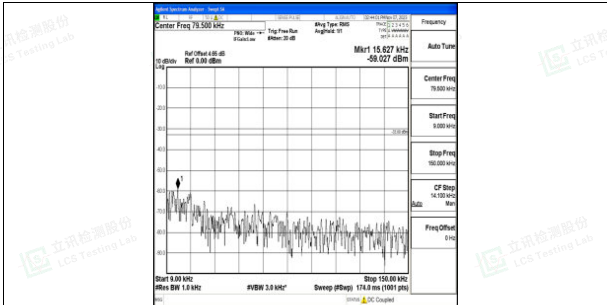
Band12_10MHz_16QAM_23095_1RB#0_0.009~0.15_0.009~0.15
