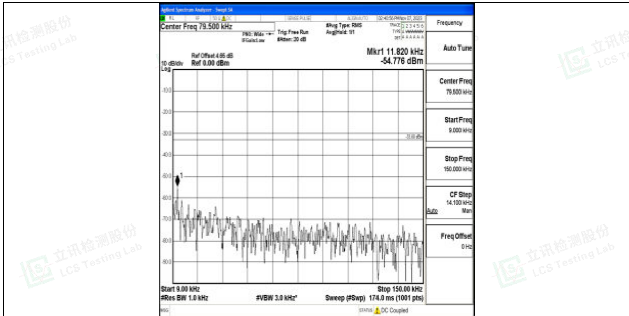
Band12_10MHz_QPSK_23060_1RB#0_0.009~0.15_0.009~0.15
