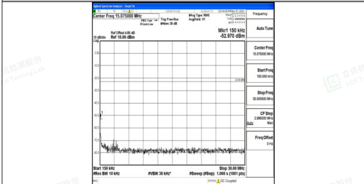
Band12_10MHz_16QAM_23095_1RB#0_0.15~30_0.15~30
