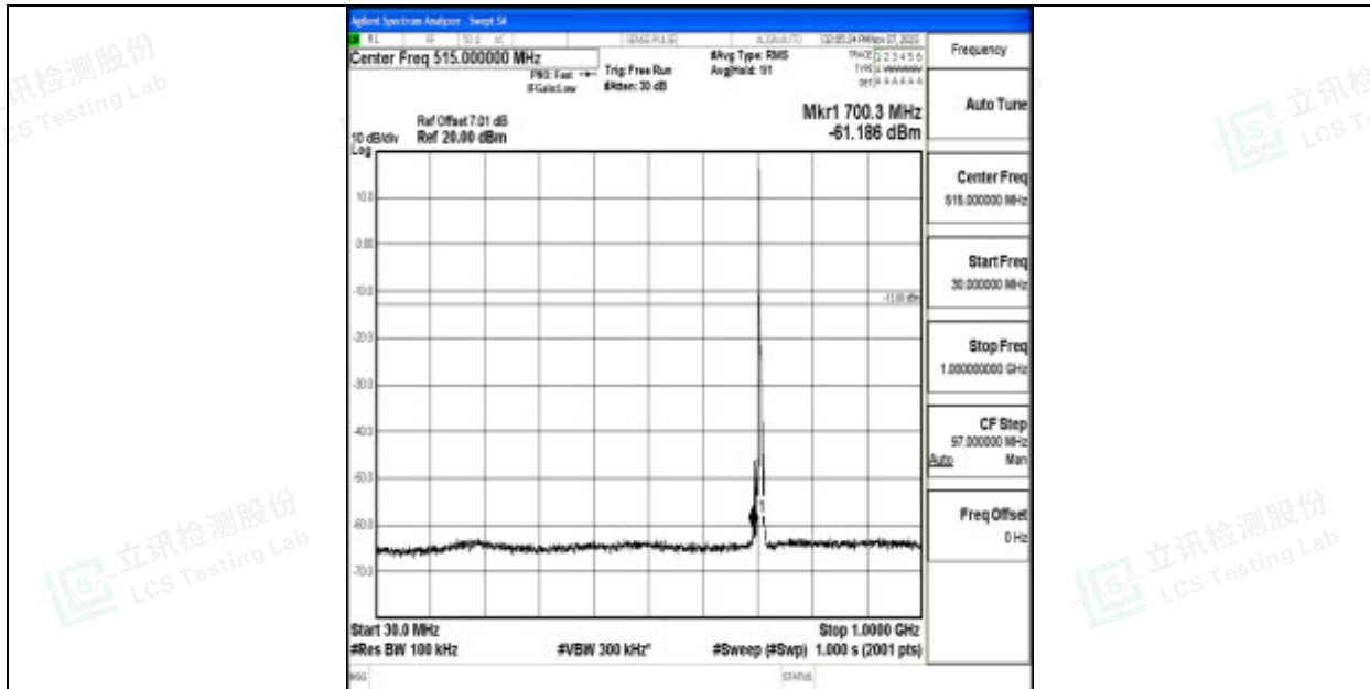
Band12_5MHz_16QAM_23155_1RB#0_30~1000_30~1000
