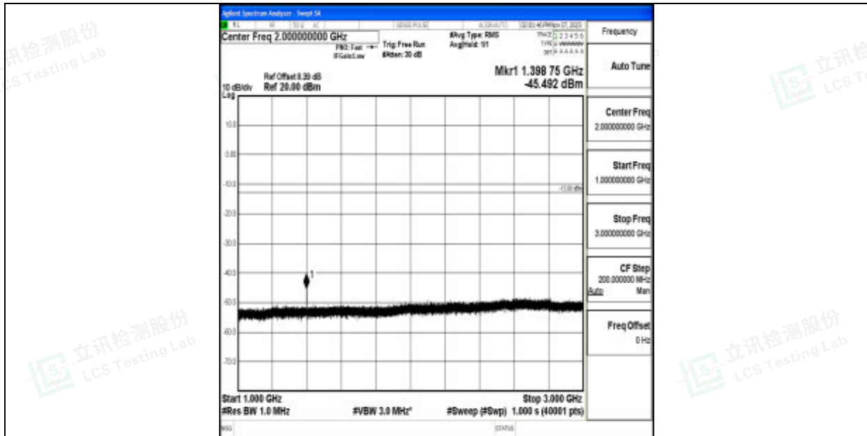
Band12_5MHz_64QAM_23035_1RB#0_1000~3000_1000~3000
