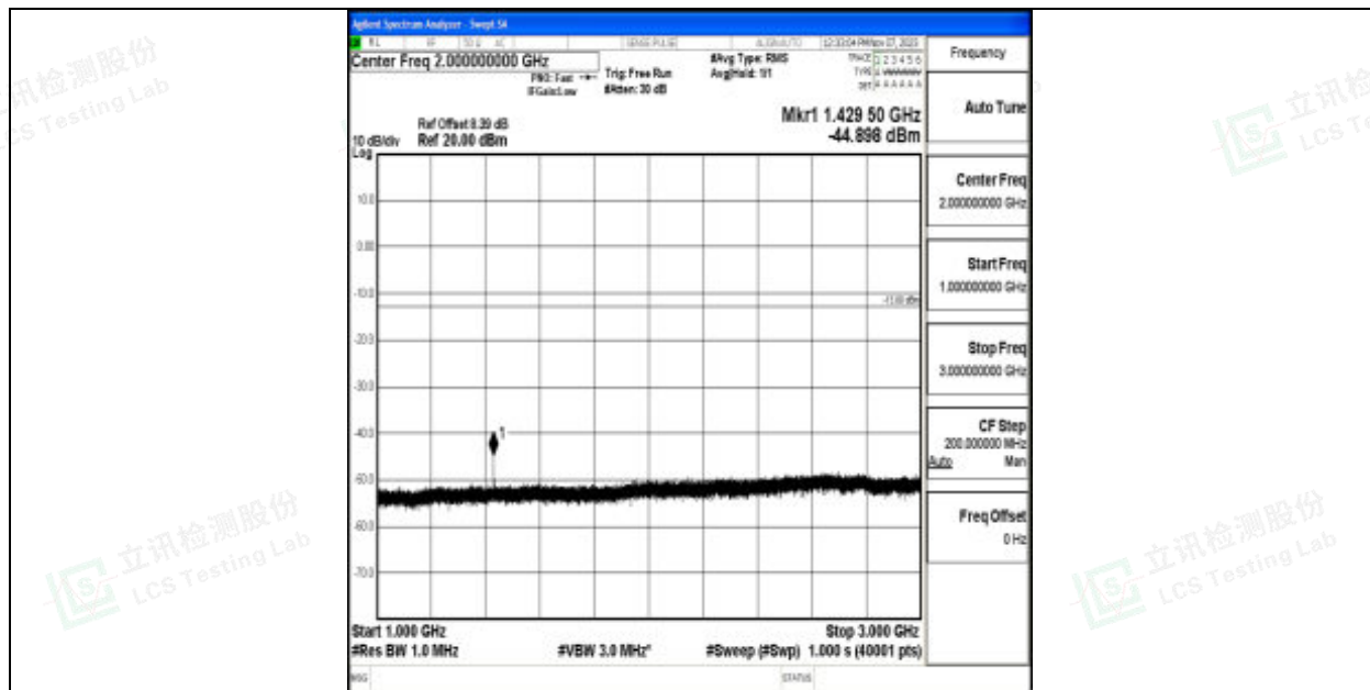
Band12_1.4MHz_QPSK_23173_1RB#0_1000~3000_1000~3000
