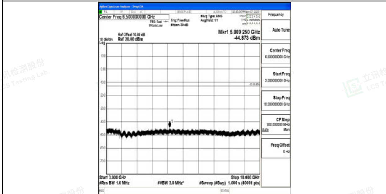
Band12_5MHz_QPSK_23155_1RB#0_3000~10000_3000~10000
