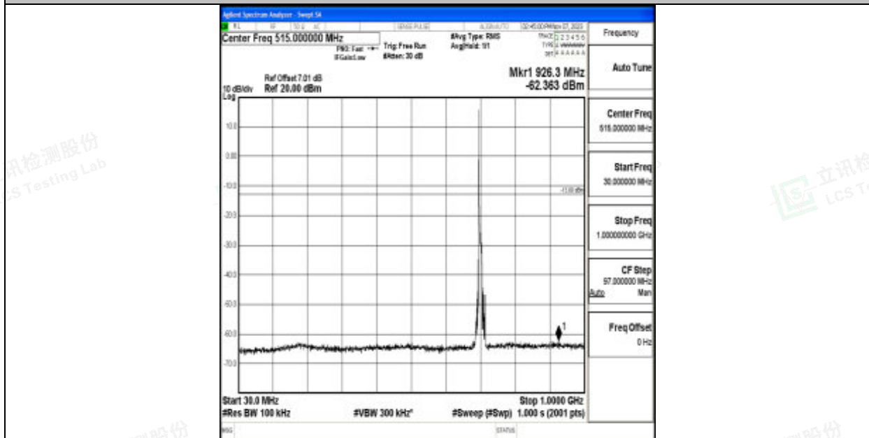
Band12_10MHz_64QAM_23095_1RB#0_30~1000_30~1000
