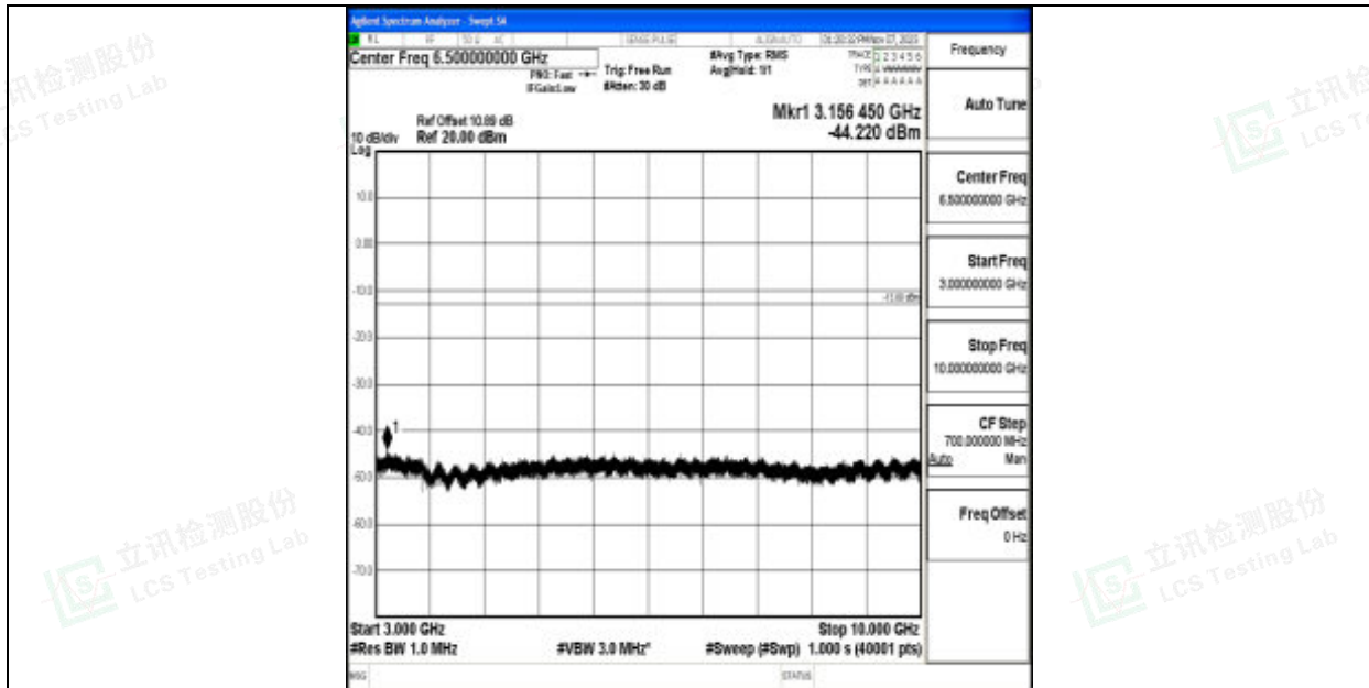
Band12_3MHz_64QAM_23025_1RB#0_3000~10000_3000~10000
