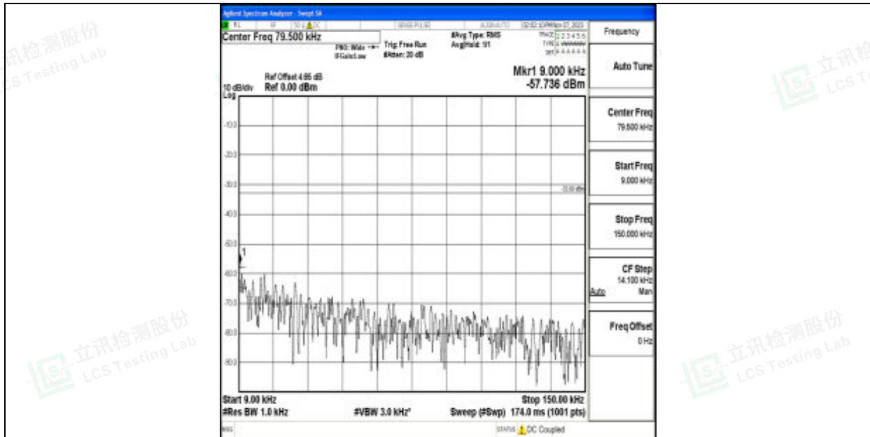
Band12_5MHz_QPSK_23095_1RB#0_0.009~0.15_0.009~0.15
