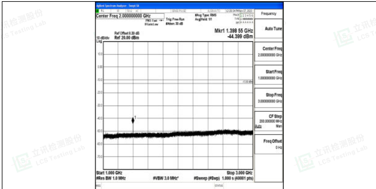
Band12_1.4MHz_QPSK_23017_1RB#0_1000~3000_1000~3000
