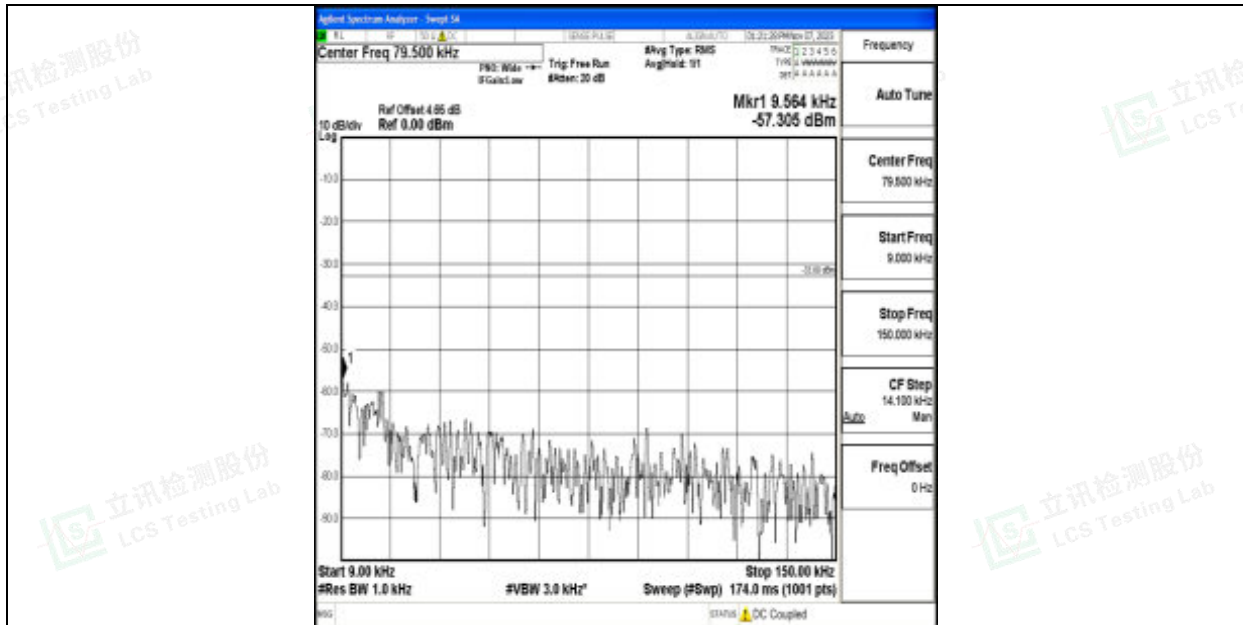
Band12_3MHz_16QAM_23095_1RB#0_0.009~0.15_0.009~0.15
