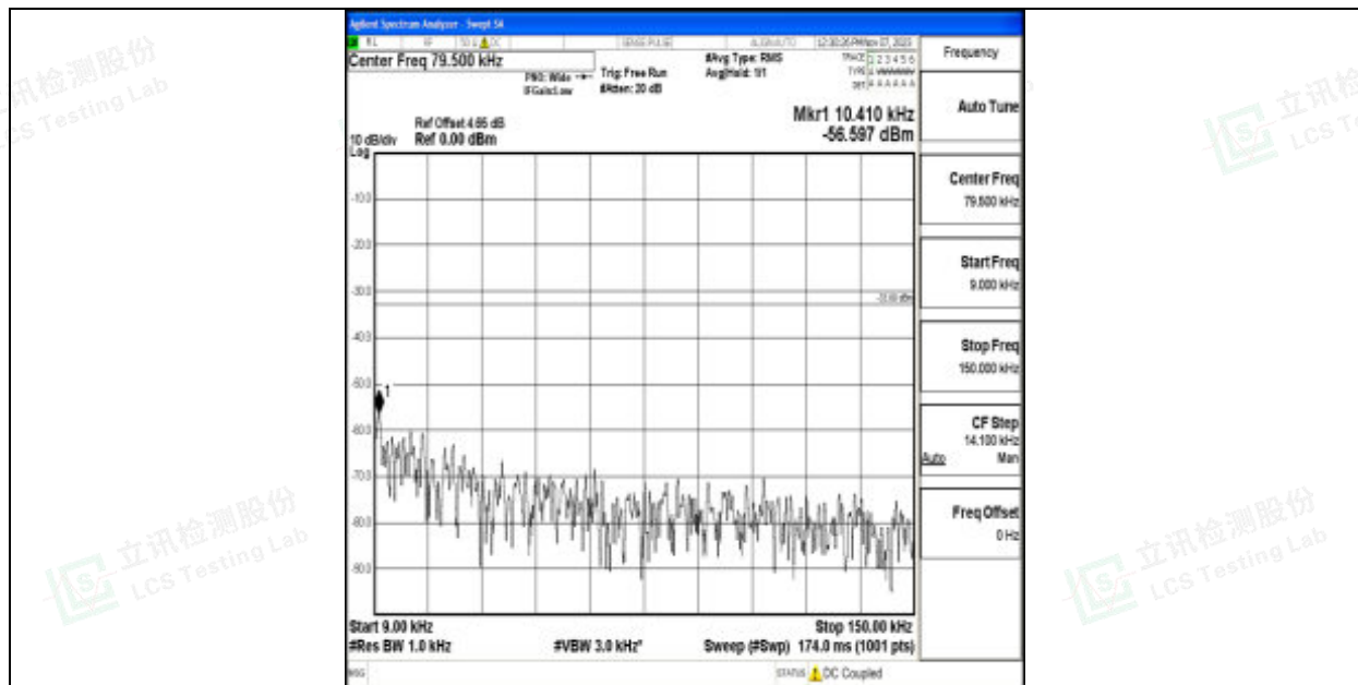
Band12_1.4MHz_QPSK_23095_1RB#0_0.009~0.15_0.009~0.15
