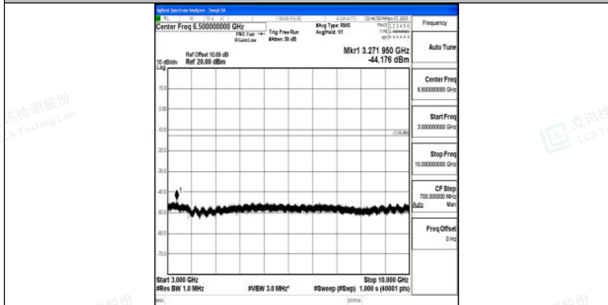
Band12_10MHz_16QAM_23130_1RB#0_3000~10000_3000~10000
