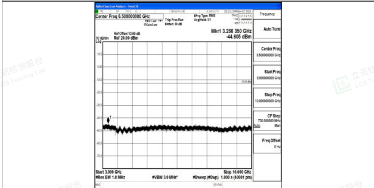
Band12_3MHz_QPSK_23095_1RB#0_3000~10000_3000~10000
