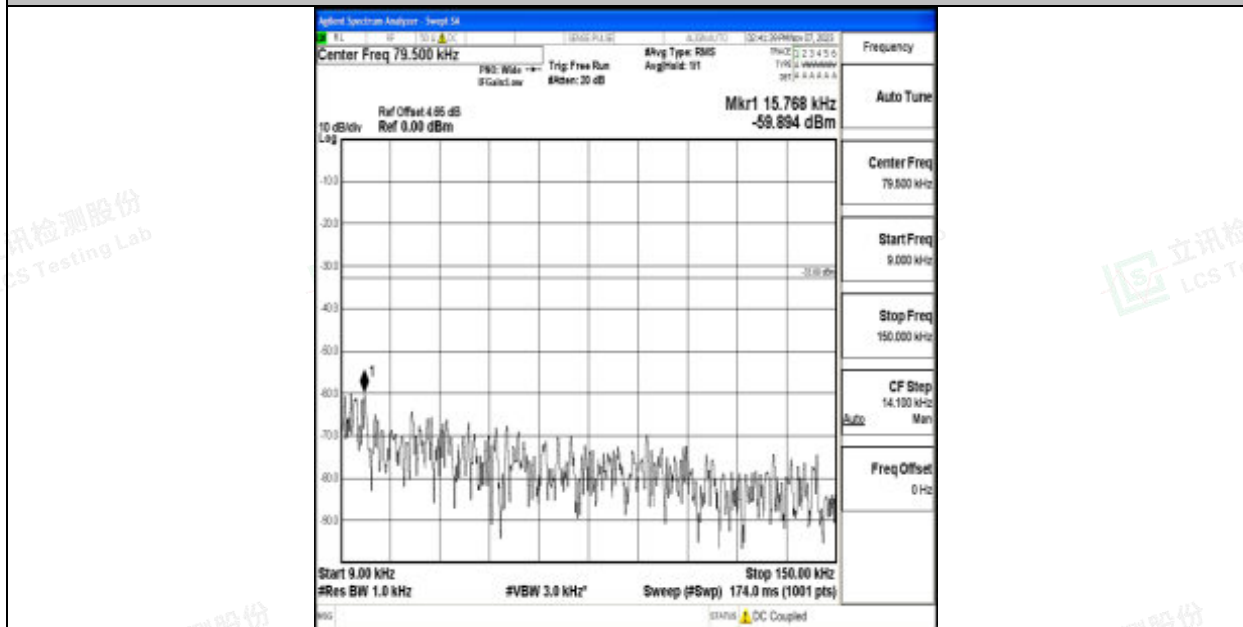
Band12_10MHz_16QAM_23060_1RB#0_0.009~0.15_0.009~0.15
