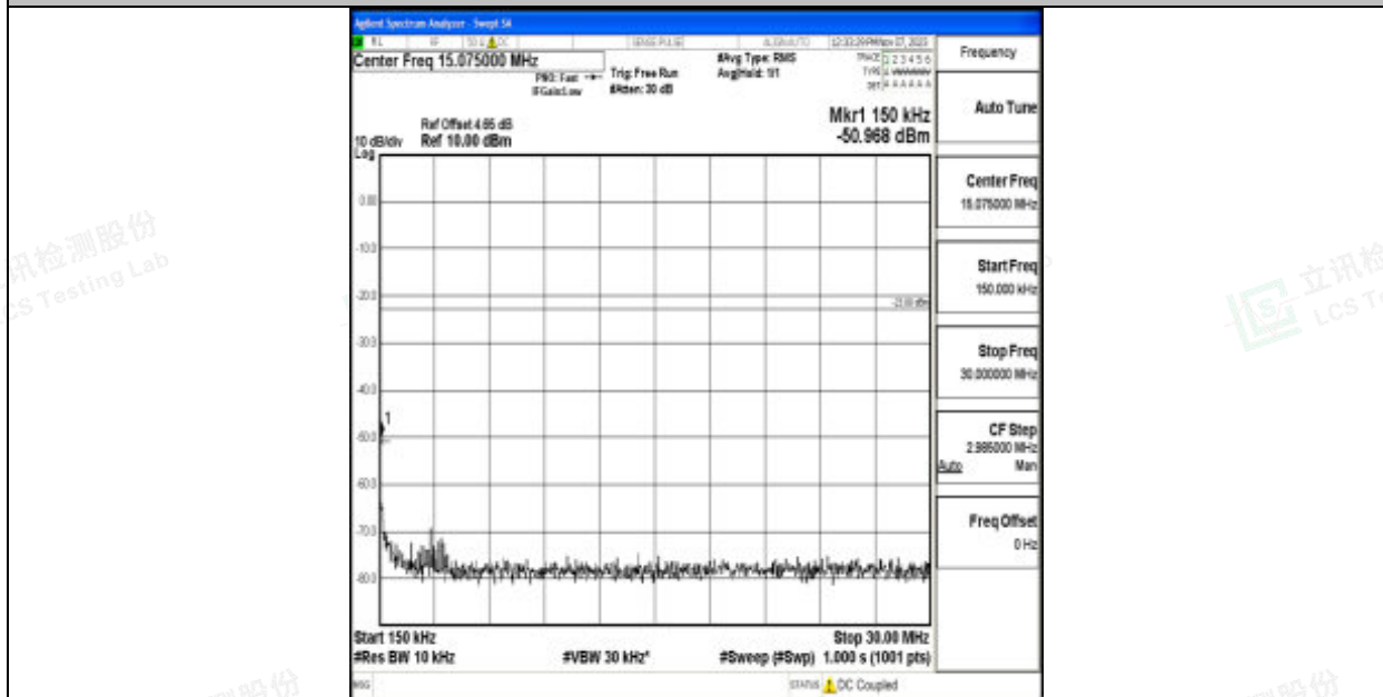
Band12_1.4MHz_16QAM_23173_1RB#0_0.15~30_0.15~30
