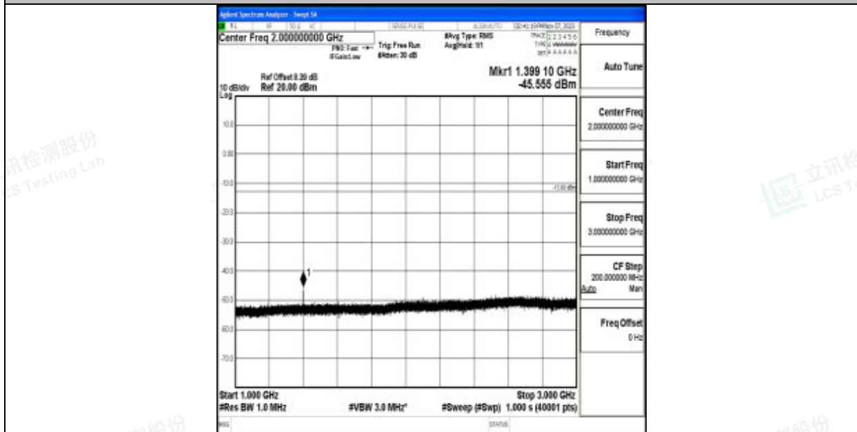
Band12_10MHz_QPSK_23060_1RB#0_1000~3000_1000~3000
