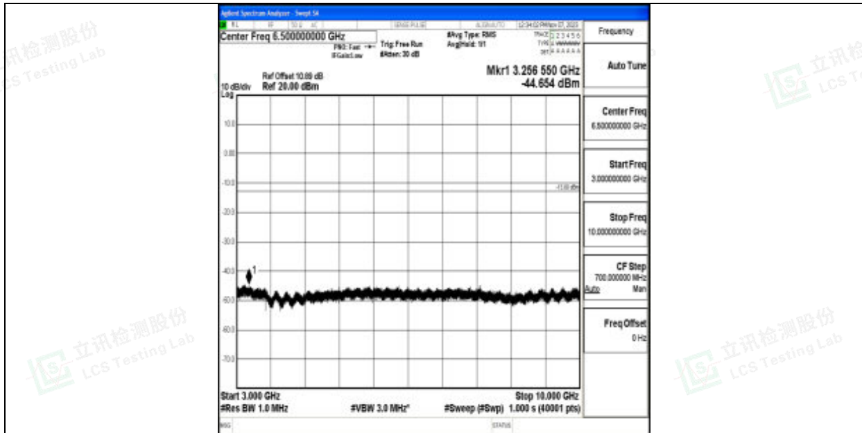
Band12_1.4MHz_16QAM_23173_1RB#0_3000~10000_3000~10000
