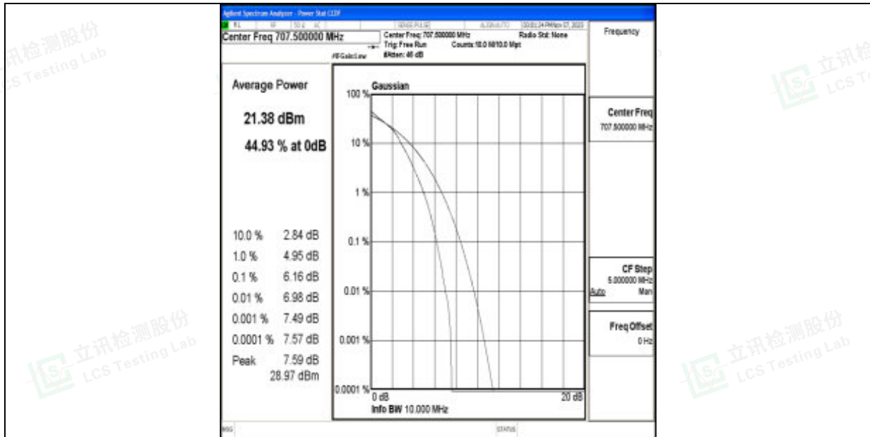
Band12-10MHz-16QAM-23095-50RB#0-PASS
