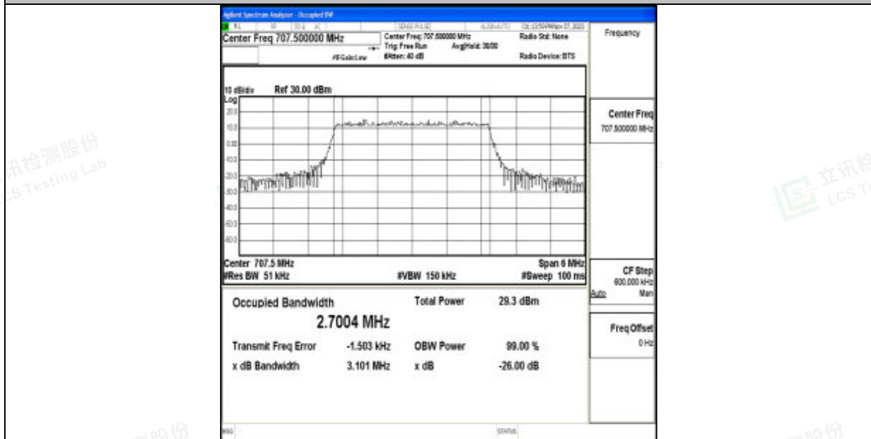
Band12-3MHz-16QAM-23095-15RB#0-PASS
