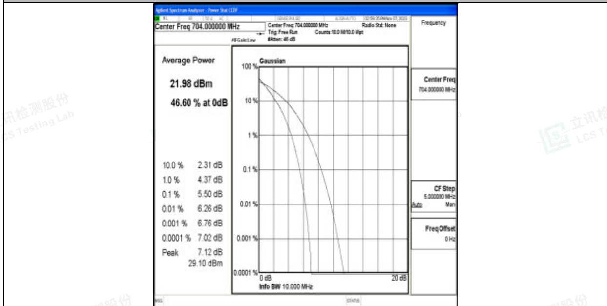
Band12-10MHz-64QAM-23060-50RB#0-PASS
