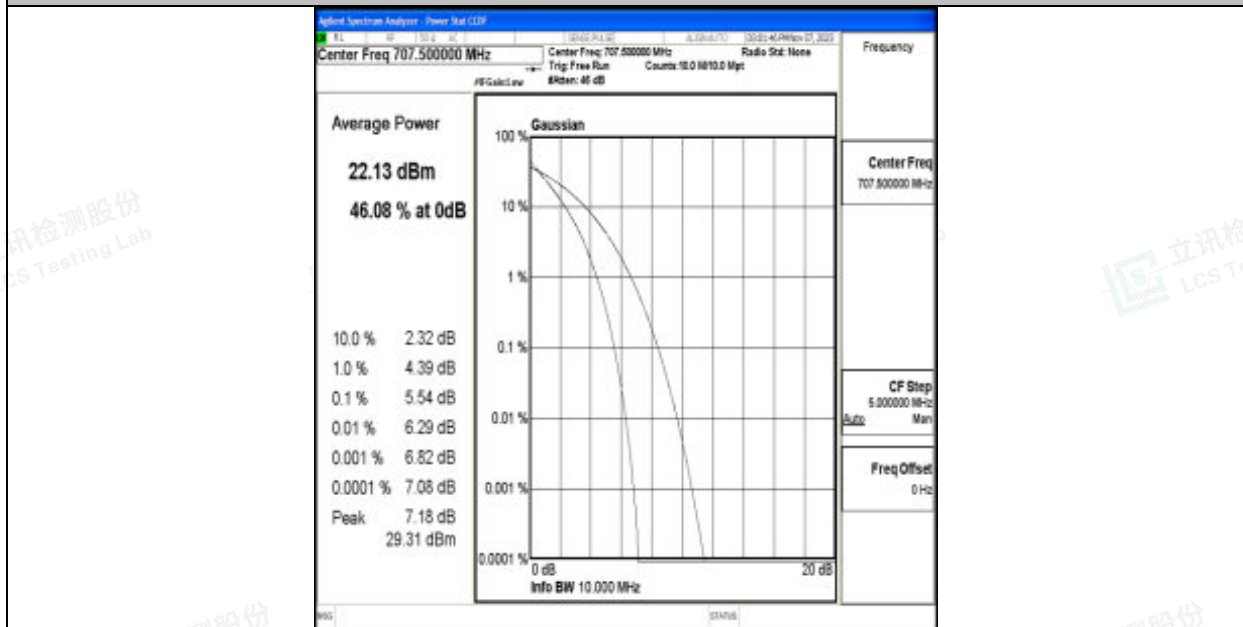
Band12-10MHz-64QAM-23095-50RB#0-PASS
