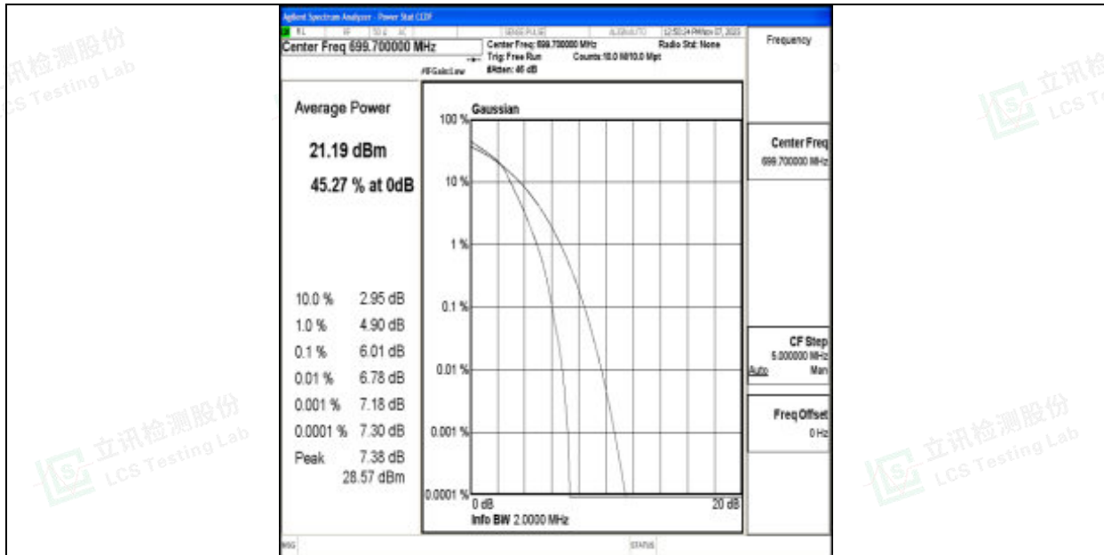
Band12-1.4MHz-16QAM-23017-6RB#0-PASS
