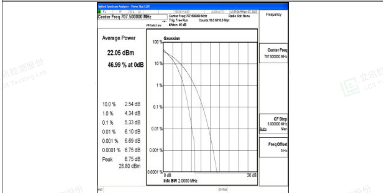
Band12-1.4MHz-64QAM-23095-6RB#0-PASS
