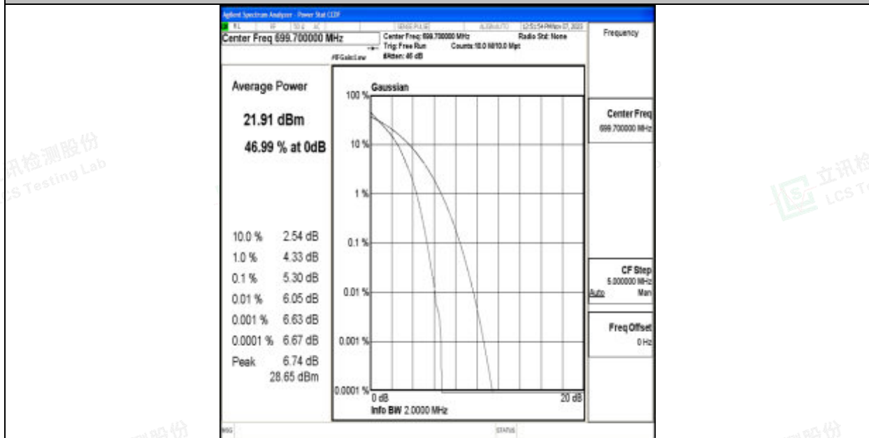
Band12-1.4MHz-64QAM-23017-6RB#0-PASS
