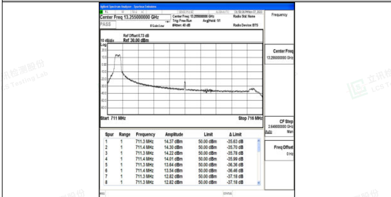
Band12_5MHz_64QAM_23155_1RB#0
