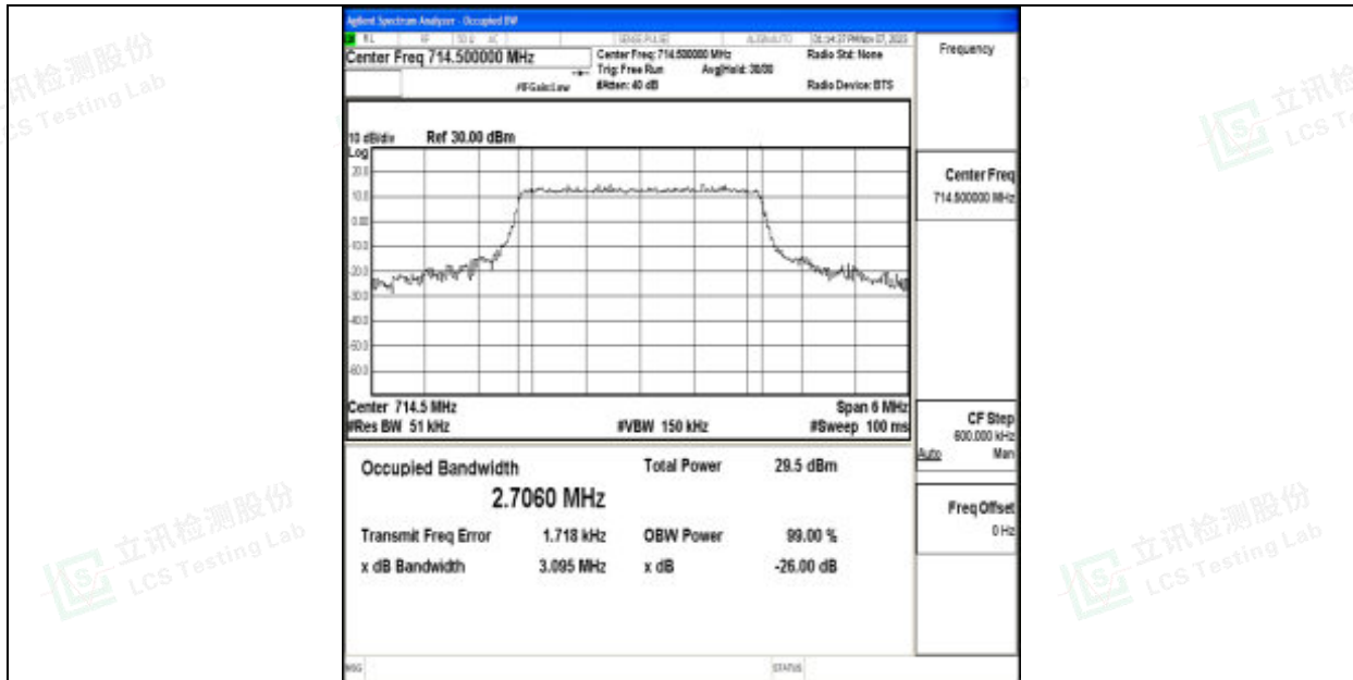
Band12-3MHz-16QAM-23165-15RB#0-PASS
