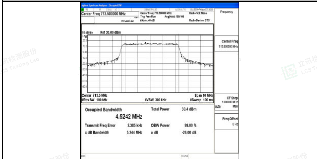
Band12-5MHz-16QAM-23155-25RB#0-PASS
