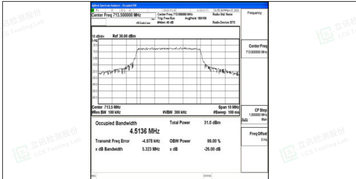
Band12-5MHz-QPSK-23155-25RB#0-PASS
