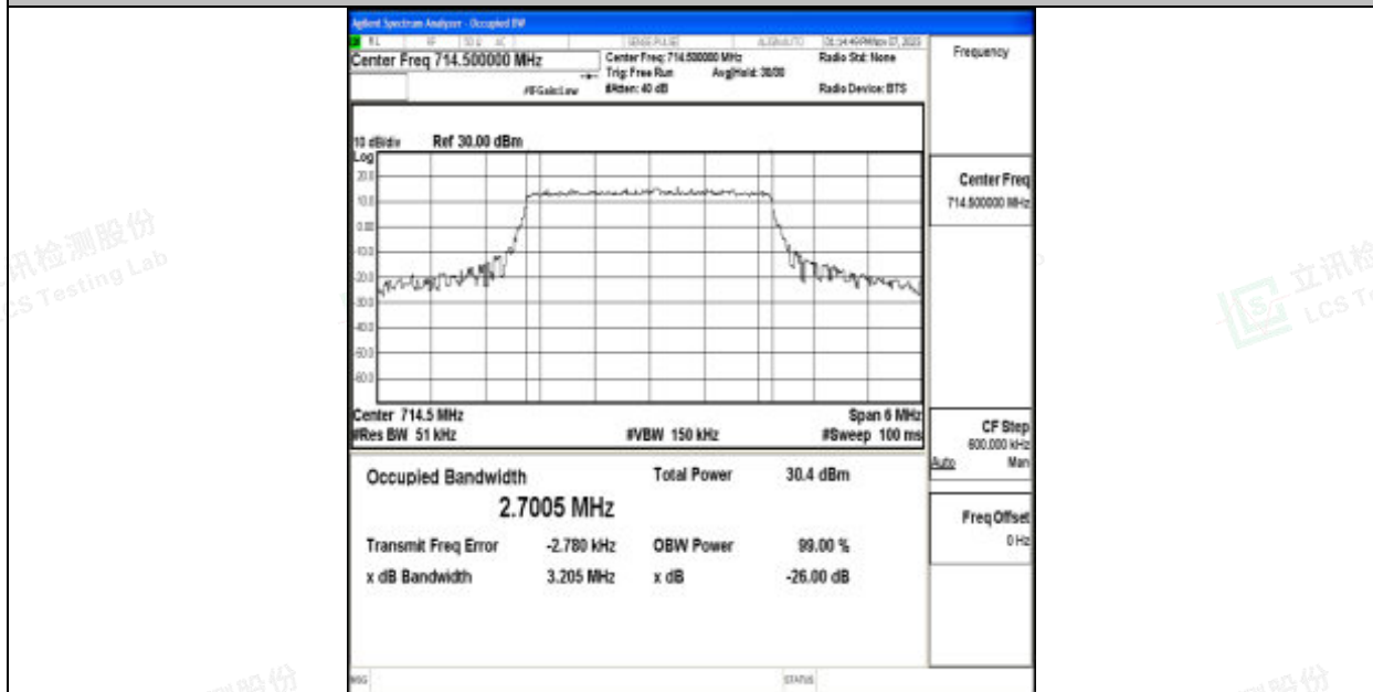
Band12-3MHz-64QAM-23165-15RB#0-PASS
