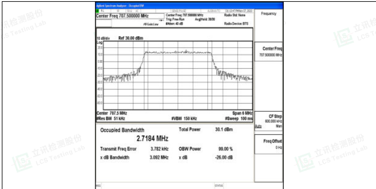
Band12-3MHz-QPSK-23095-15RB#0-PASS
