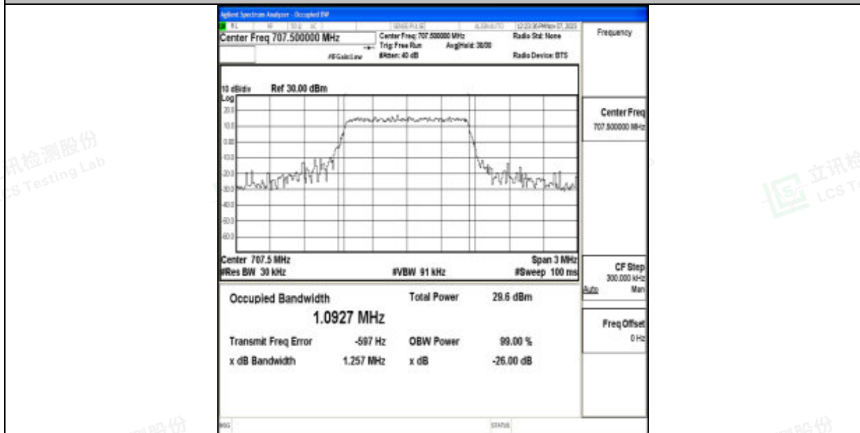
Band12-1.4MHz-QPSK-23095-6RB#0-PASS
