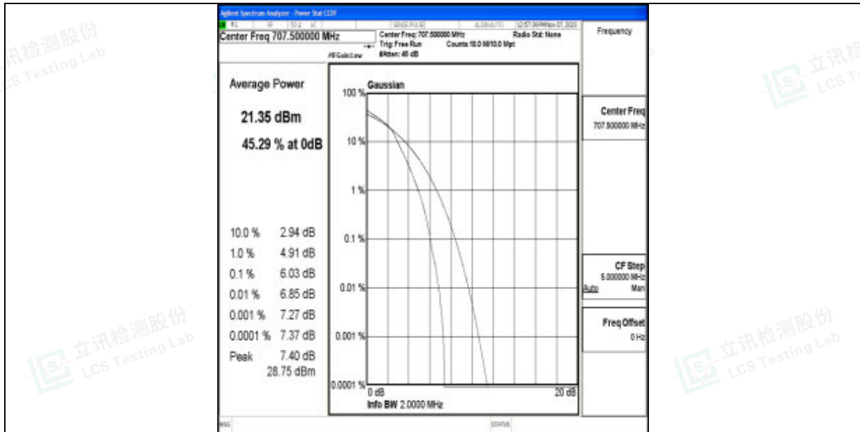
Band12-1.4MHz-16QAM-23095-6RB#0-PASS
