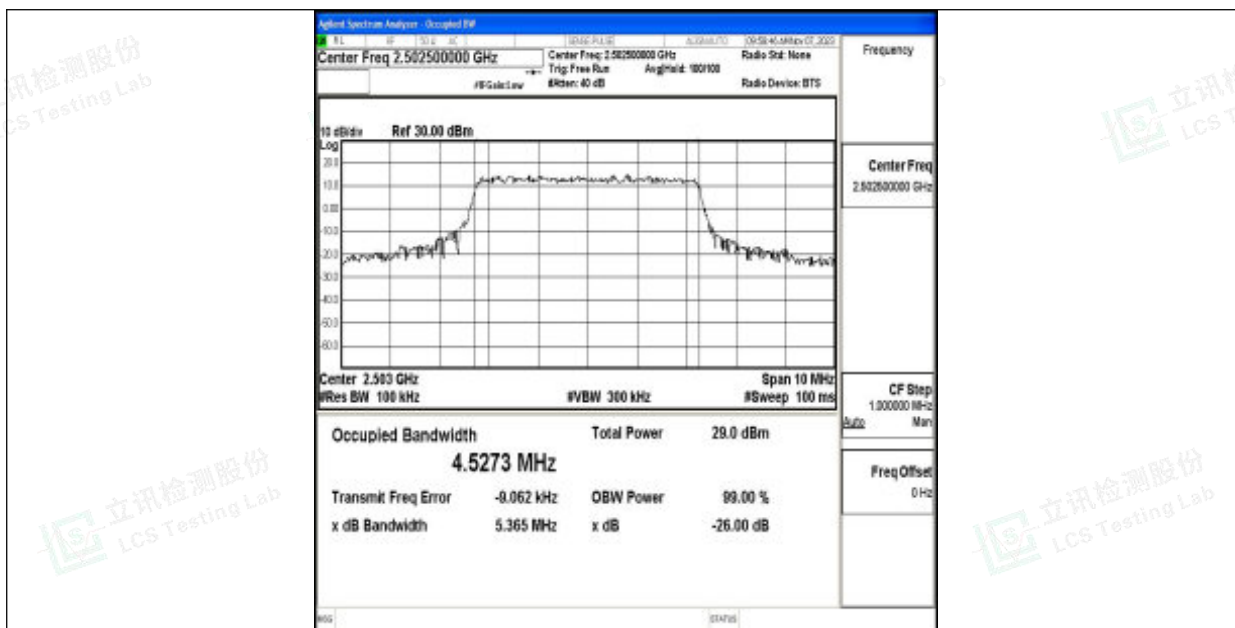
Band7-5MHz-64QAM-20775-25RB#0-PASS
