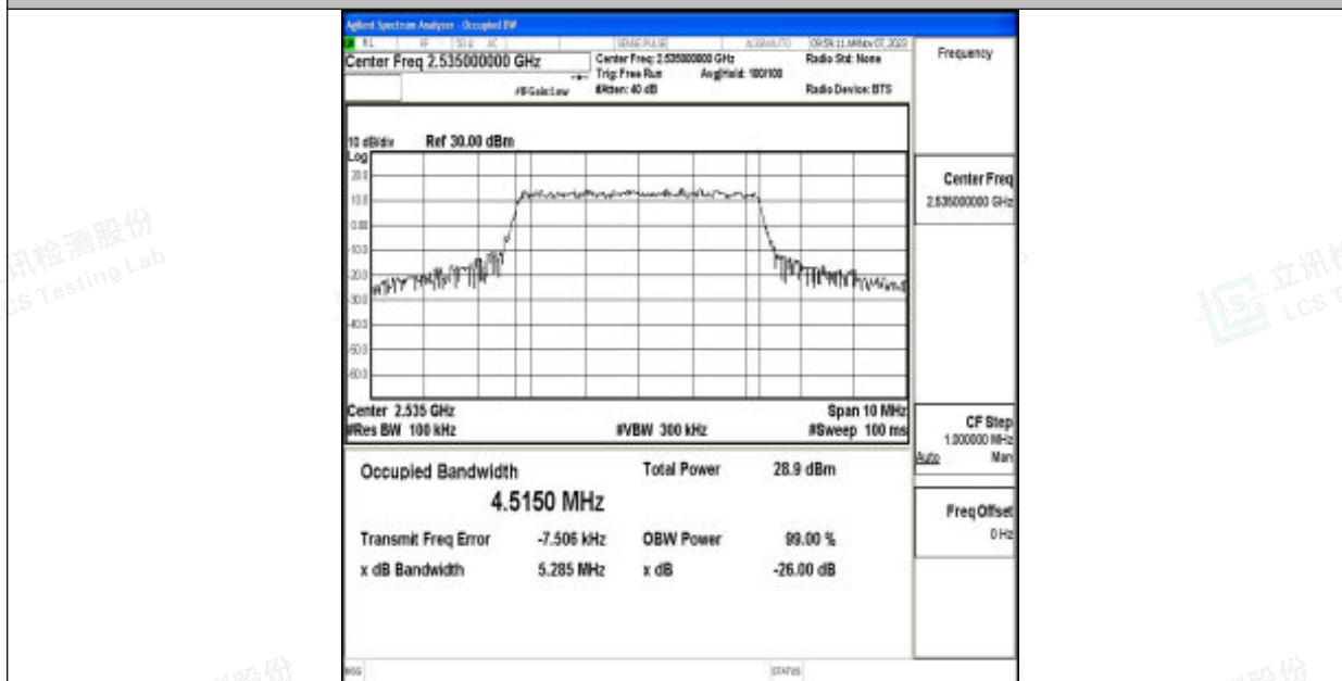
Band7-5MHz-QPSK-21100-25RB#0-PASS
