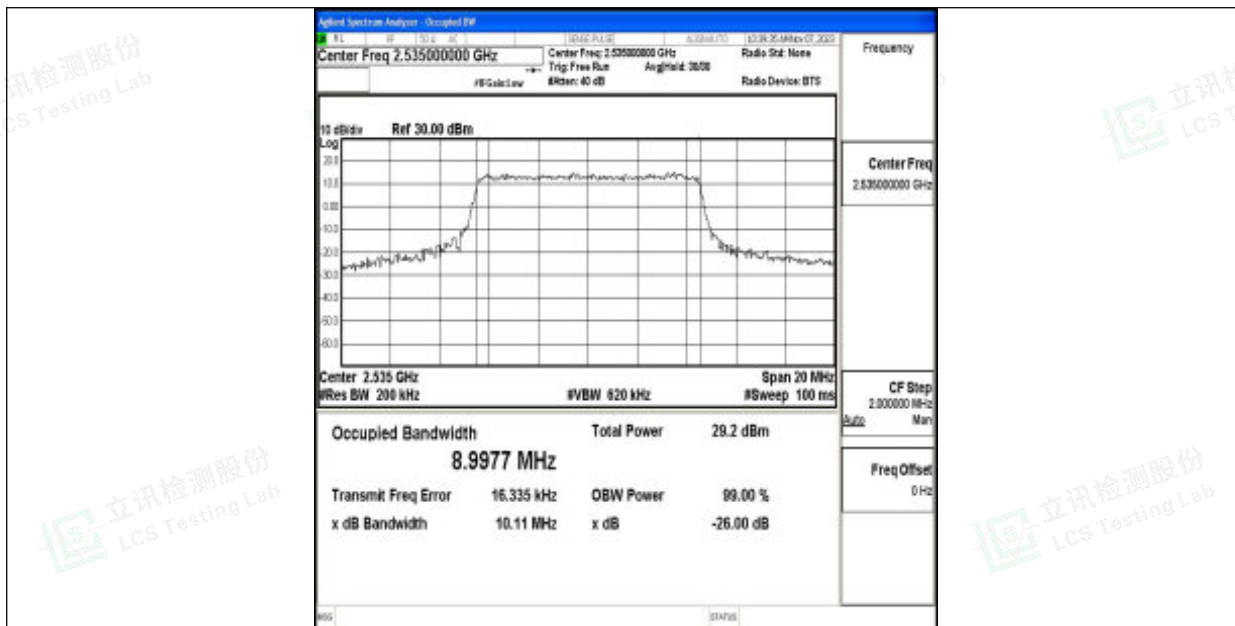
Band7-10MHz-64QAM-21100-50RB#0-PASS
