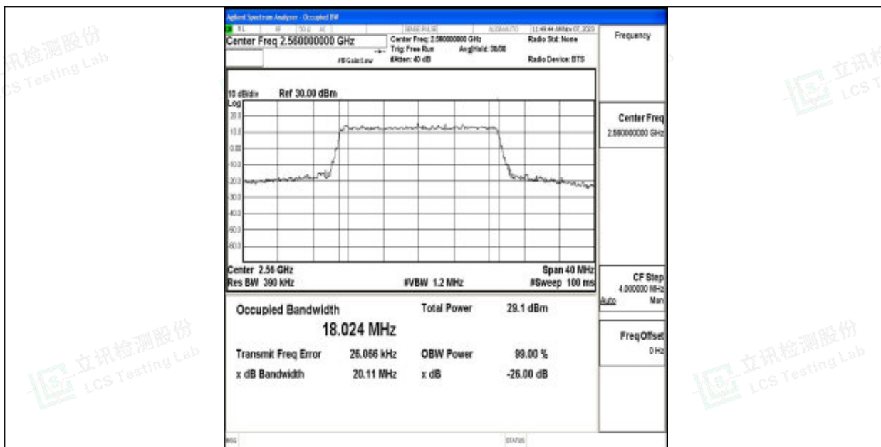
Band7-20MHz-16QAM-21350-100RB#0-PASS
