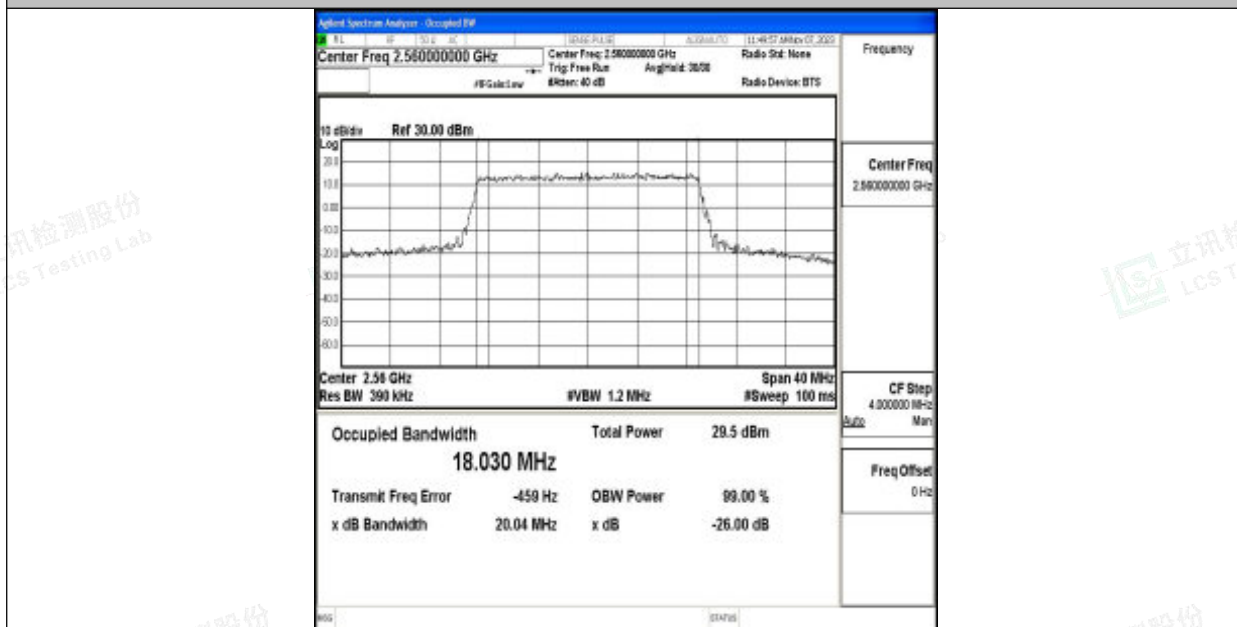
Band7-20MHz-64QAM-21350-100RB#0-PASS
