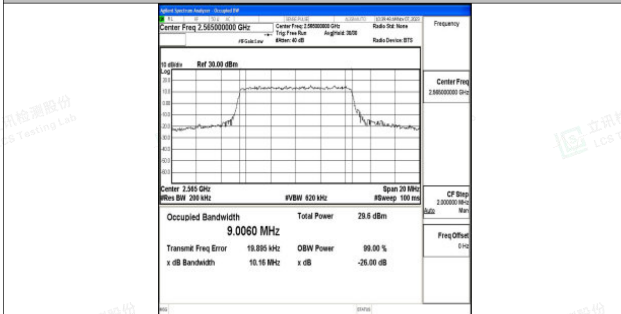
Band7-10MHz-QPSK-21400-50RB#0-PASS
