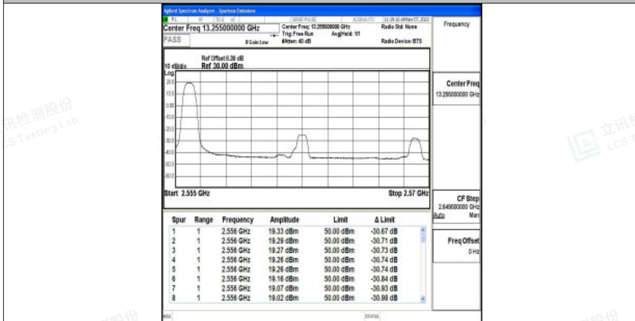
Band7_15MHz_64QAM_21375_1RB#0
