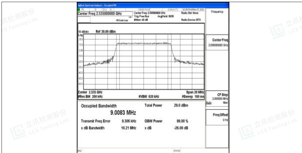
Band7-10MHz-QPSK-21100-50RB#0-PASS
