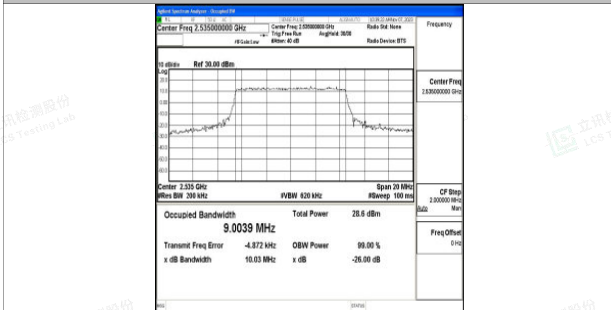
Band7-10MHz-16QAM-21100-50RB#0-PASS
