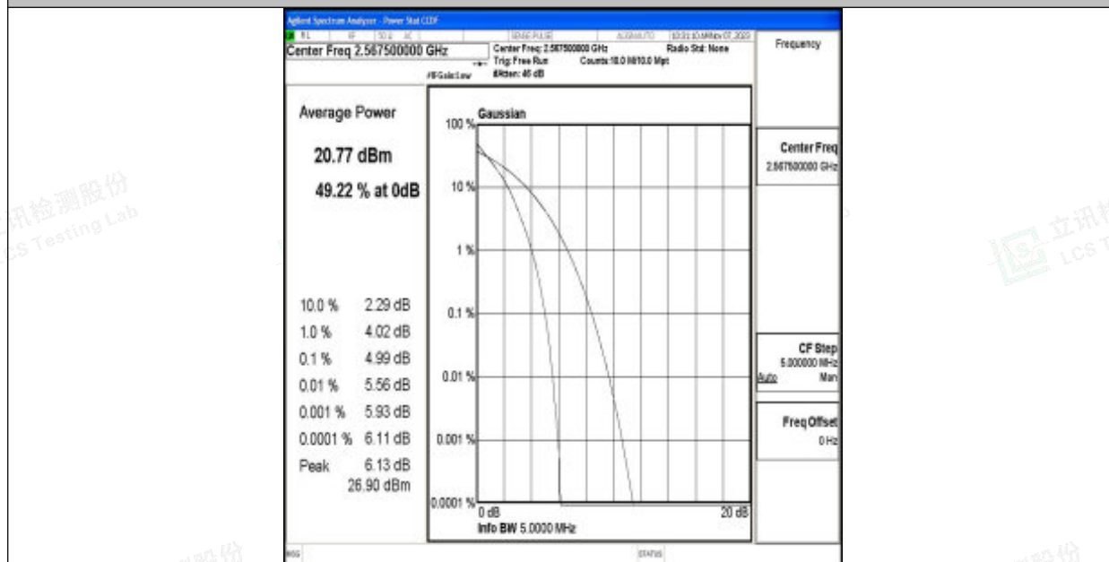
Band7-5MHz-64QAM-21425-25RB#0-PASS
