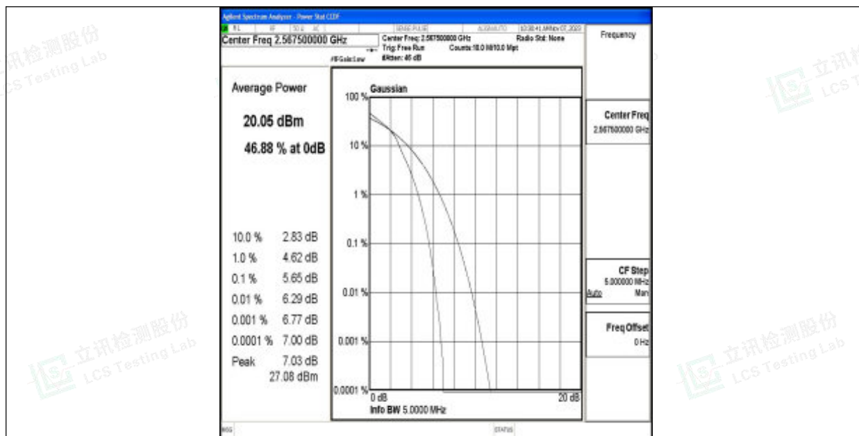
Band7-5MHz-16QAM-21425-25RB#0-PASS
