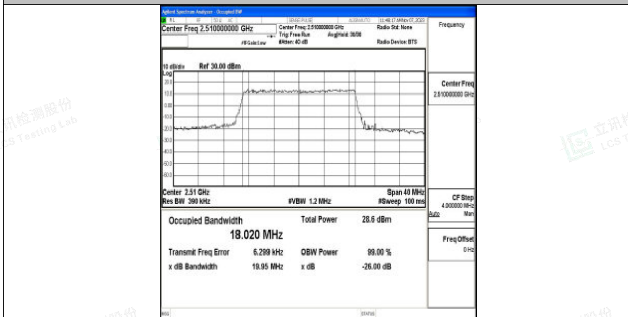
Band7-20MHz-QPSK-20850-100RB#0-PASS
