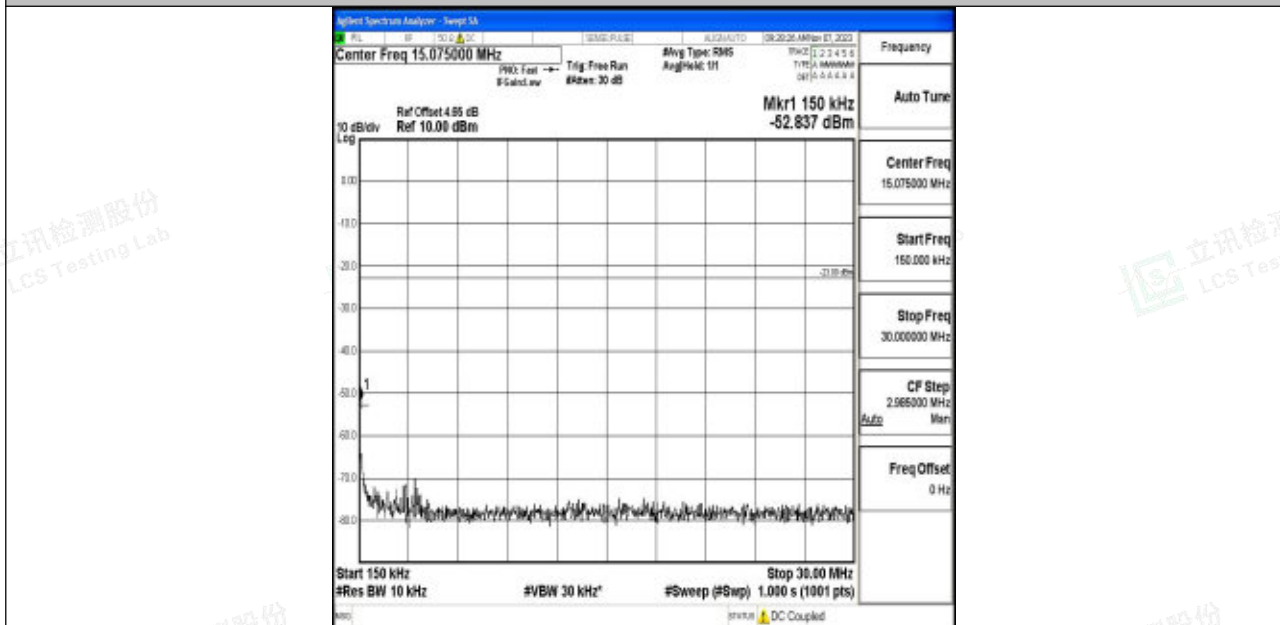
Band5_10MHz_QPSK_20450_1RB#0_0.15~30_0.15~30
