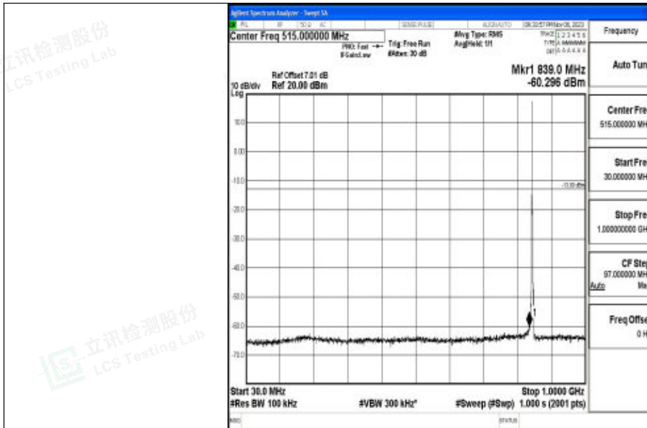
Band5_3MHz_QPSK_20635_1RB#0_30~1000_30~1000
