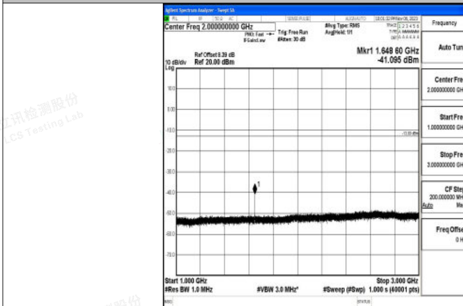
Band5_5MHz_16QAM_20425_1RB#0_1000~3000_1000~3000
