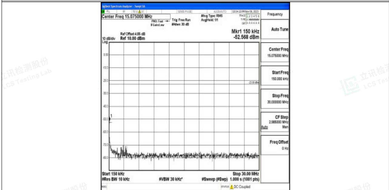
Band5_5MHz_64QAM_20525_1RB#0_0.15~30_0.15~30
