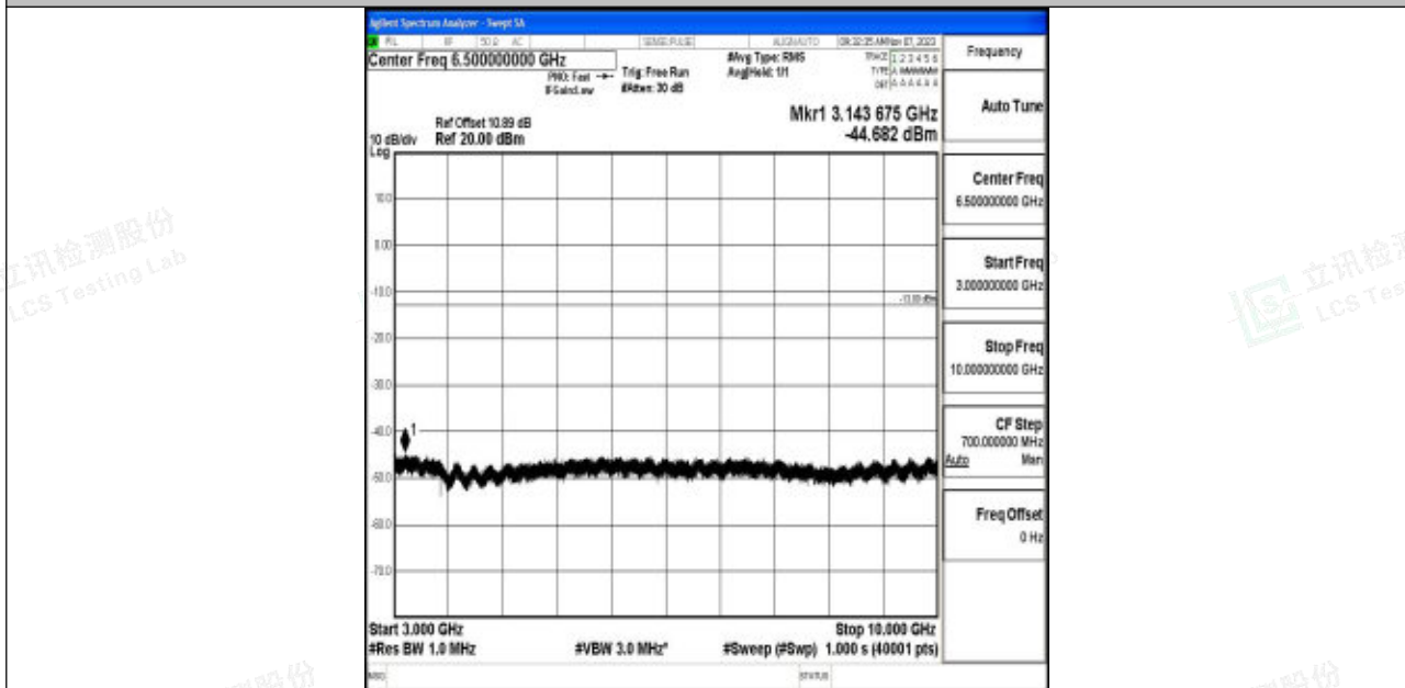
Band5_10MHz_64QAM_20525_1RB#0_3000~10000_3000~10000
