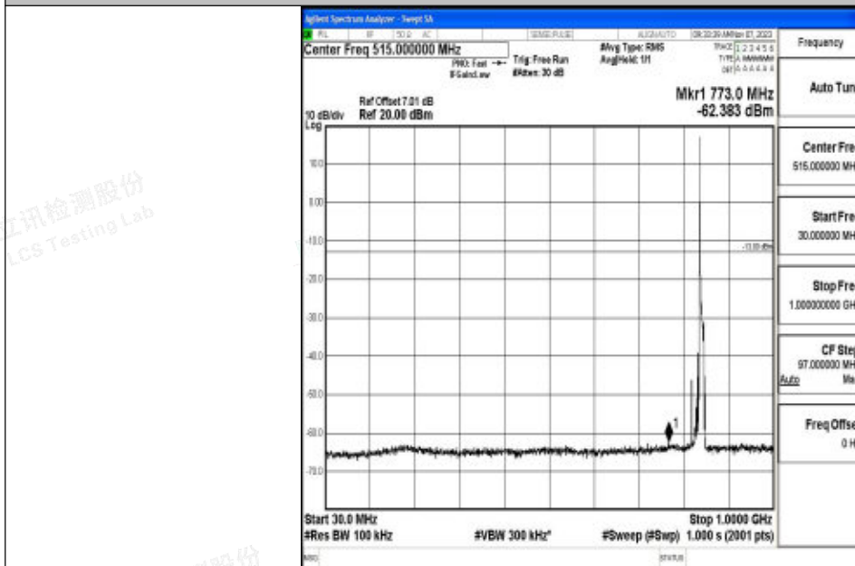
Band5_10MHz_16QAM_20600_1RB#0_30~1000_30~1000
