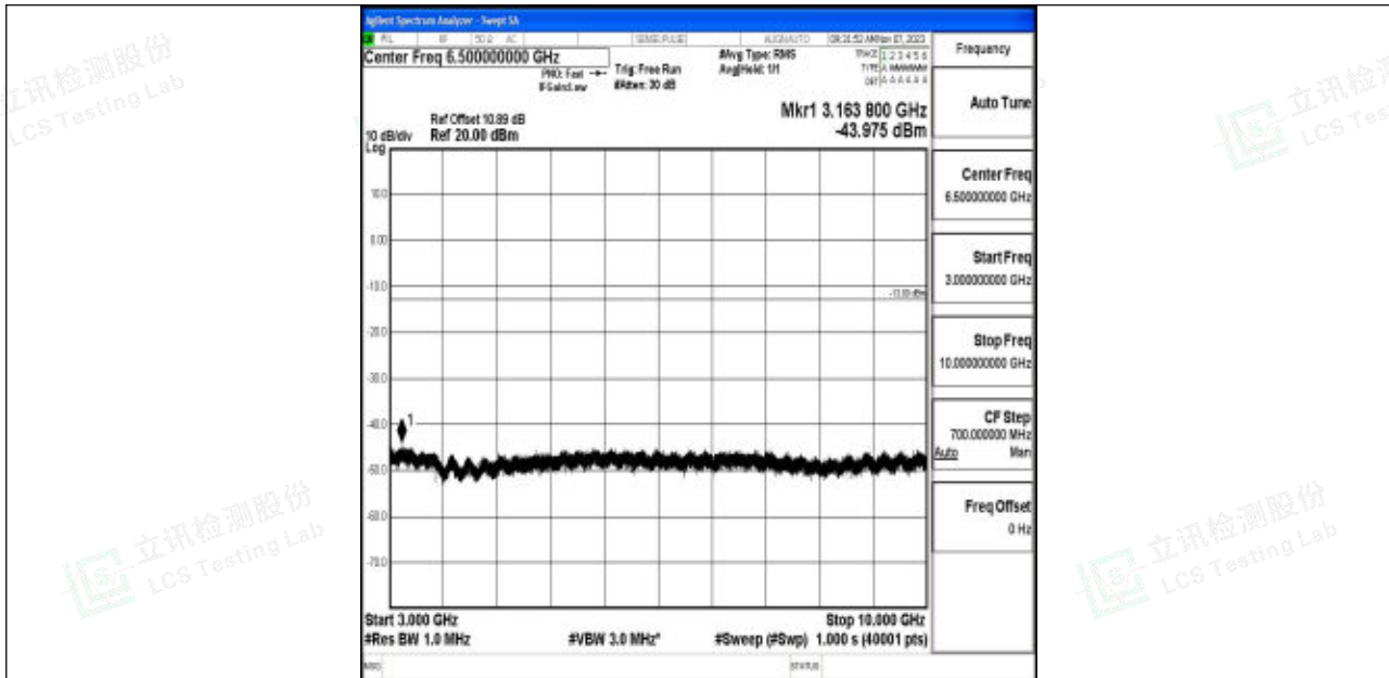
Band5_10MHz_16QAM_20525_1RB#0_3000~10000_3000~10000
