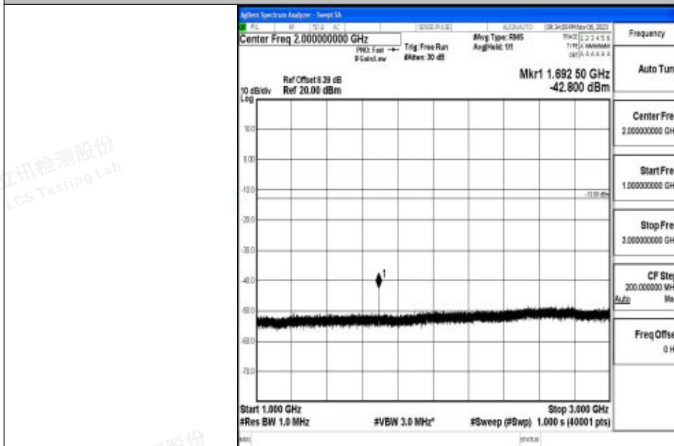
Band5_3MHz_QPSK_20635_1RB#0_1000~3000_1000~3000
