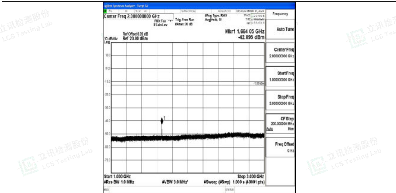
Band5_10MHz_64QAM_20525_1RB#0_1000~3000_1000~3000
