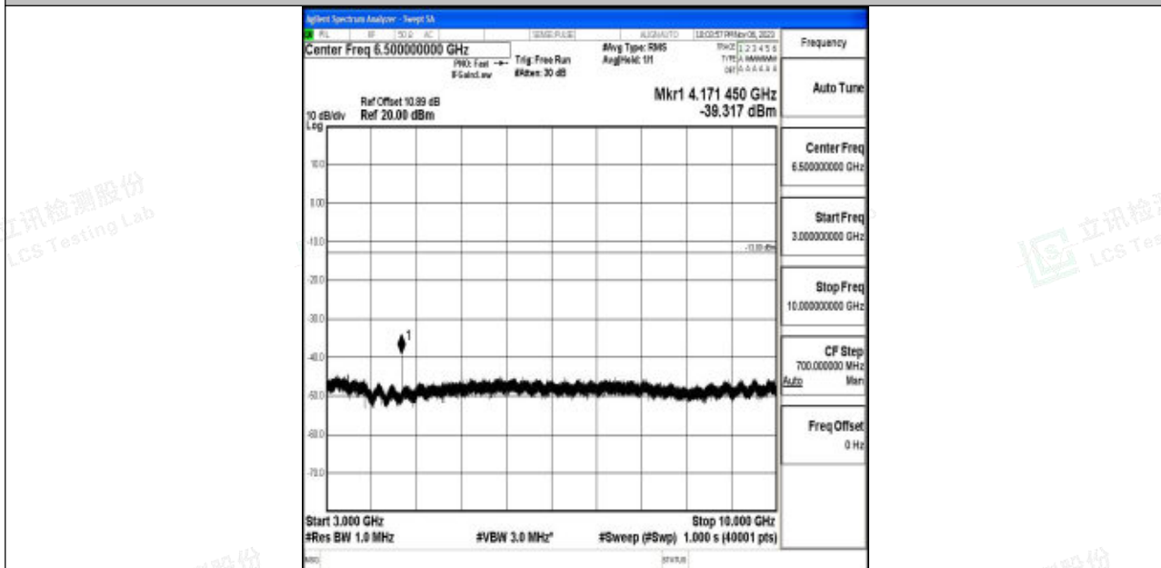
Band5_5MHz_16QAM_20525_1RB#0_3000~10000_3000~10000
