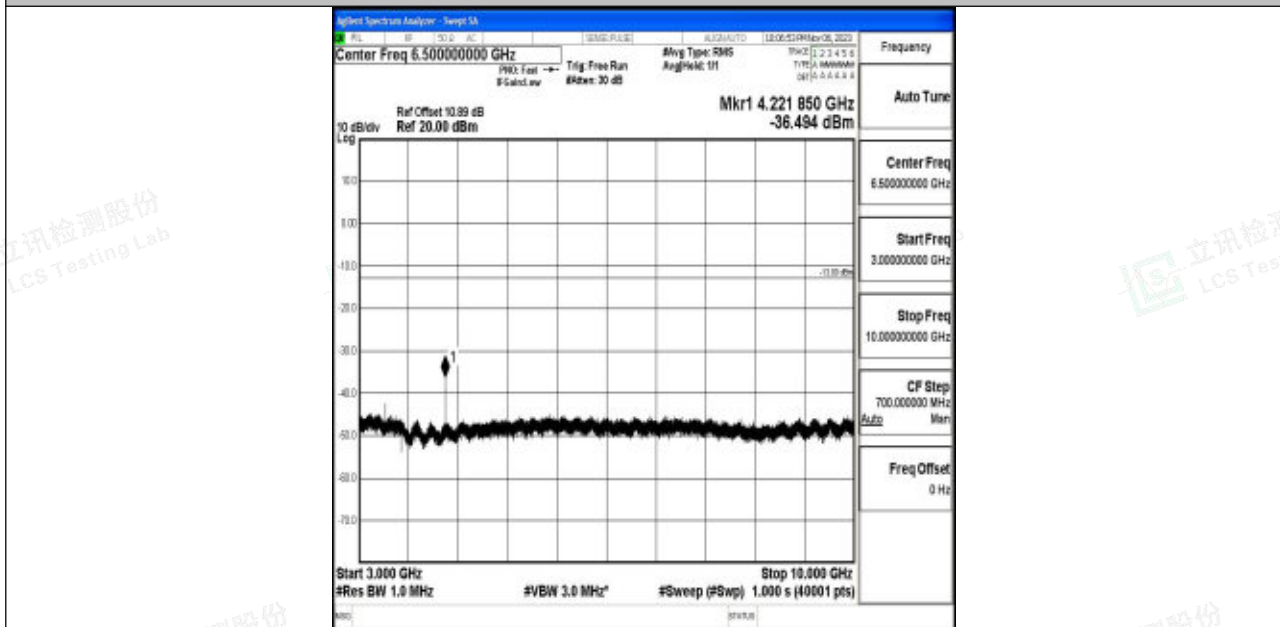
Band5_5MHz_64QAM_20625_1RB#0_3000~10000_3000~10000
