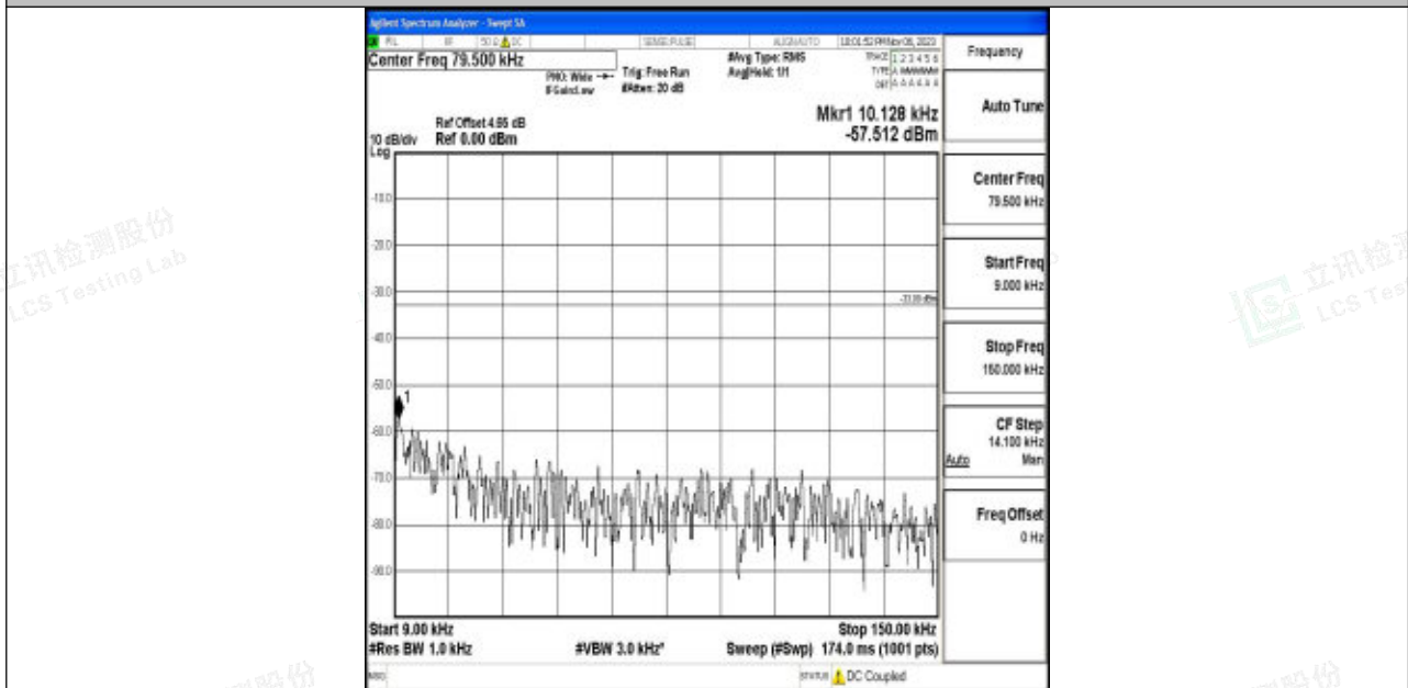
Band5_5MHz_64QAM_20425_1RB#0_0.009~0.15_0.009~0.15
