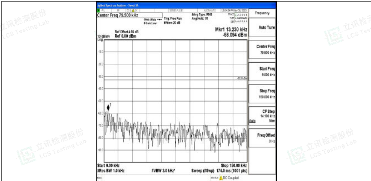
Band5_5MHz_64QAM_20525_1RB#0_0.009~0.15_0.009~0.15
