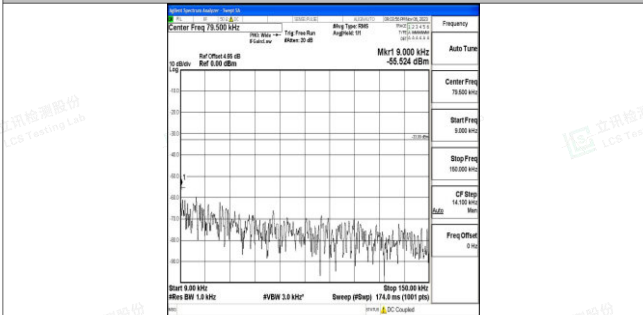
Band5_1.4MHz_64QAM_20643_1RB#0_0.009~0.15_0.009~0.15
