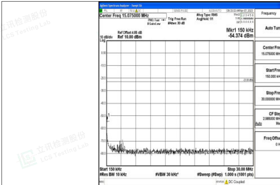
Band5_10MHz_16QAM_20600_1RB#0_0.15~30_0.15~30
