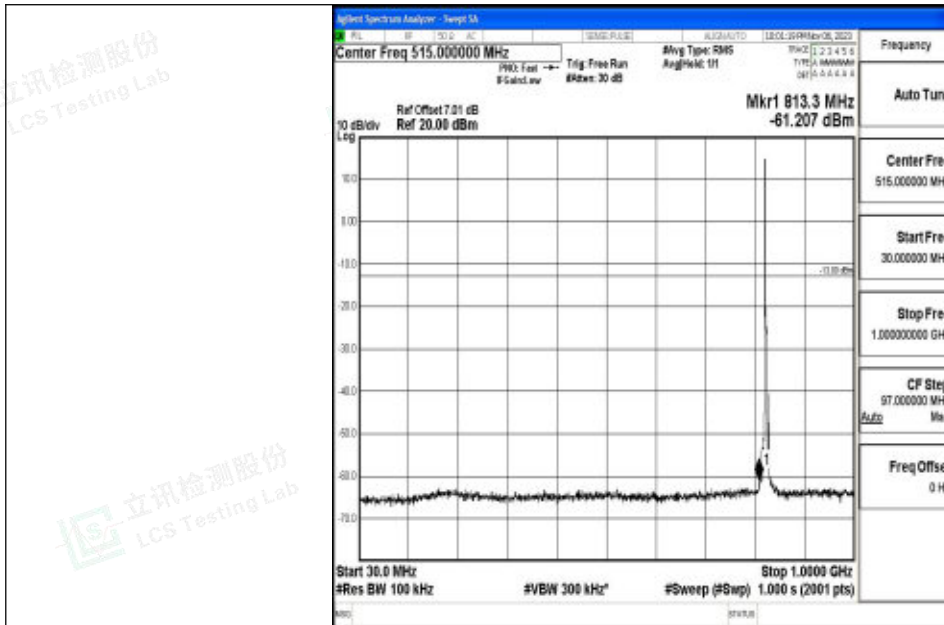
Band5_5MHz_16QAM_20425_1RB#0_30~1000_30~1000
