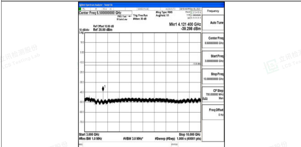
Band5_1.4MHz_64QAM_20407_1RB#0_3000~10000_3000~10000
