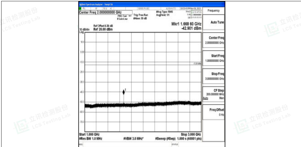
Band5_5MHz_16QAM_20525_1RB#0_1000~3000_1000~3000
