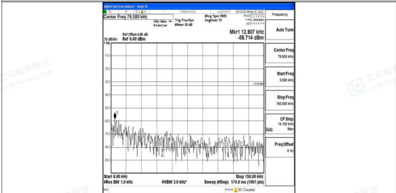
Band5_10MHz_16QAM_20600_1RB#0_0.009~0.15_0.009~0.15
