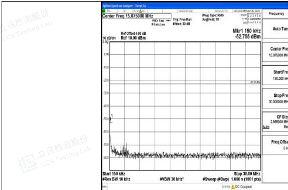
Band5_5MHz_QPSK_20425_1RB#0_0.15~30_0.15~30
