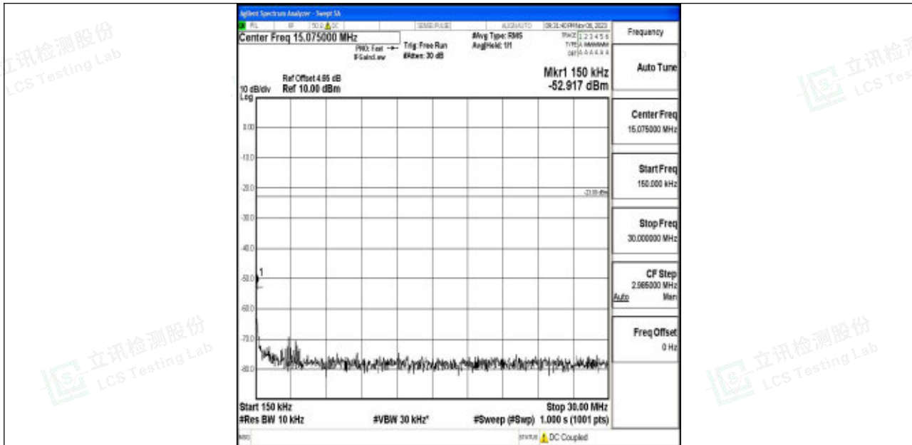
Band5_3MHz_QPSK_20525_1RB#0_0.15~30_0.15~30
