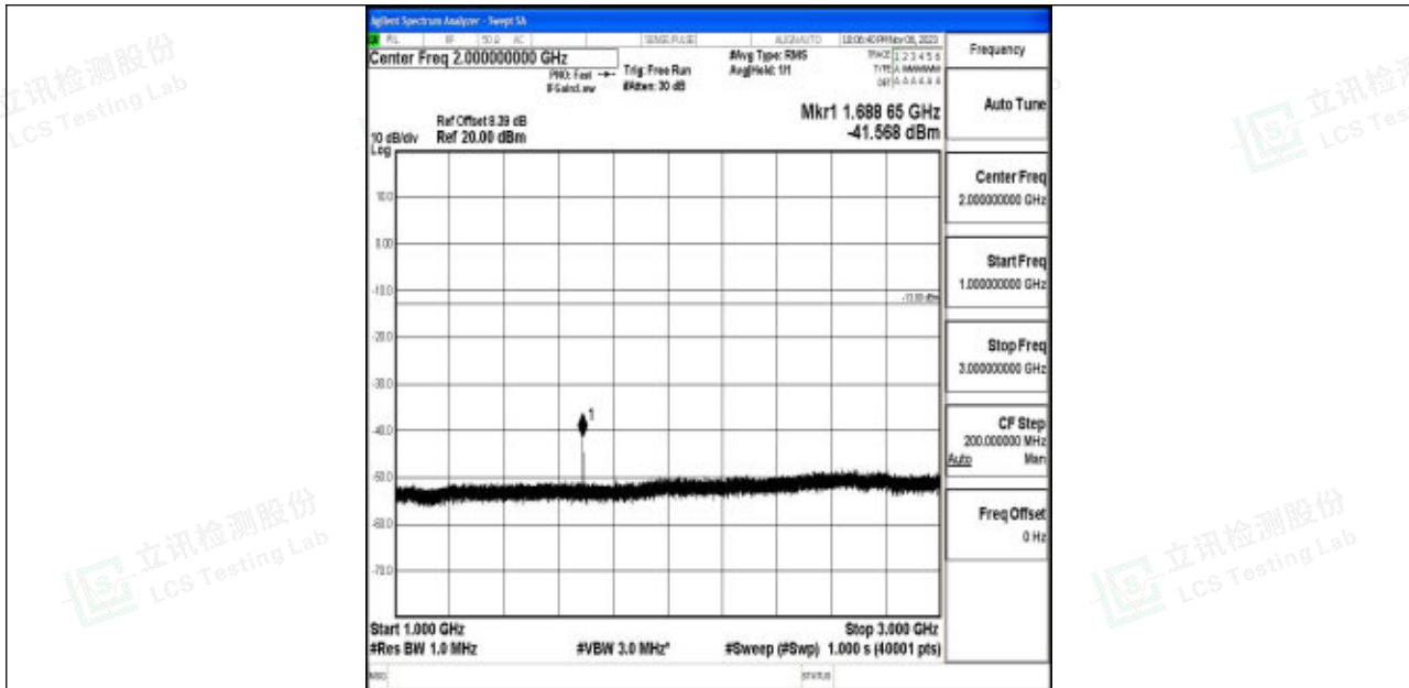
Band5_5MHz_64QAM_20625_1RB#0_1000~3000_1000~3000
