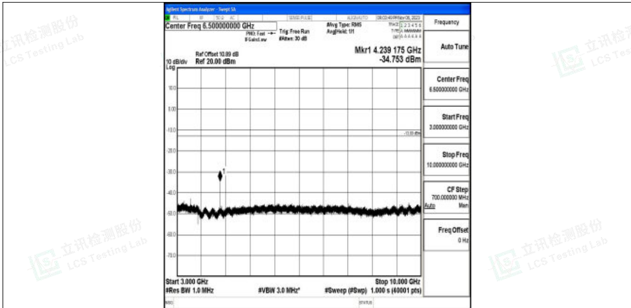
Band5_1.4MHz_16QAM_20643_1RB#0_3000~10000_3000~10000
