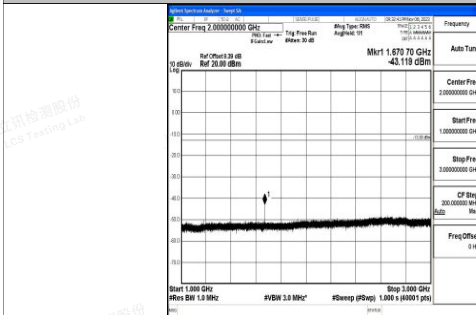
Band5_3MHz_16QAM_20525_1RB#0_1000~3000_1000~3000
