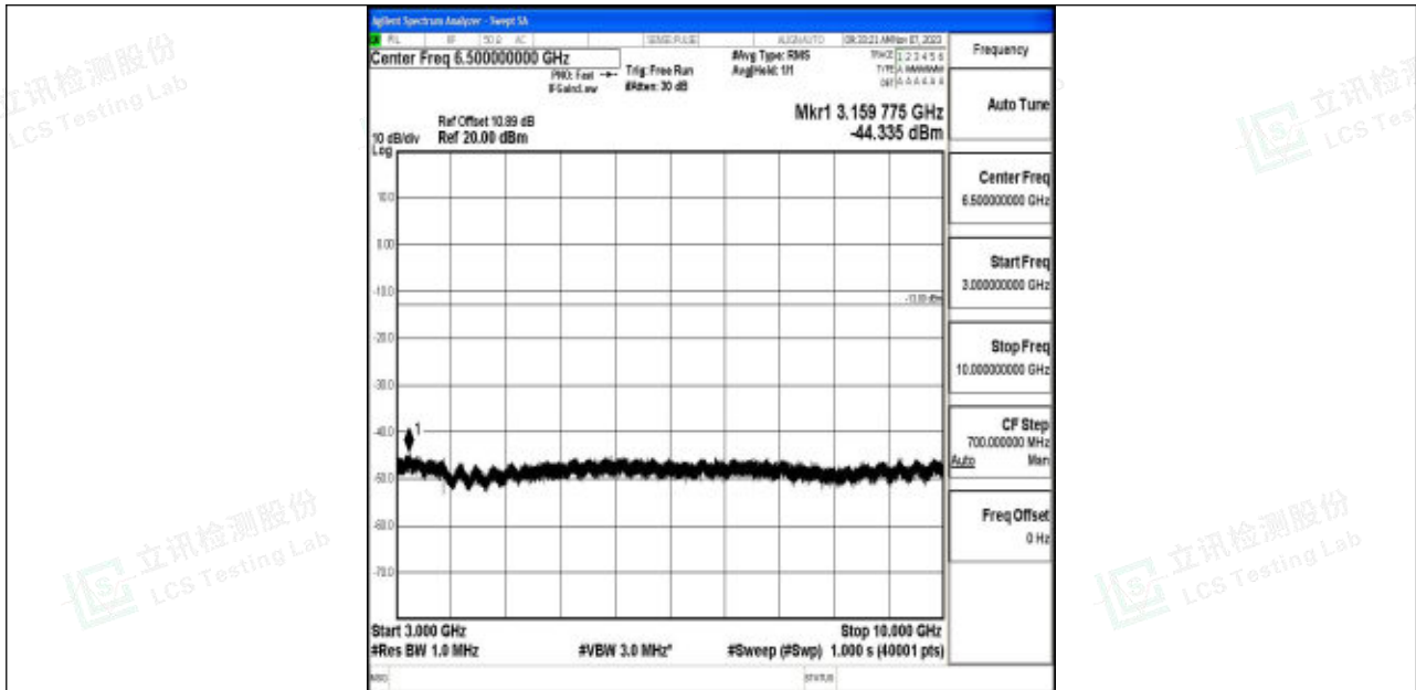
Band5_10MHz_QPSK_20600_1RB#0_3000~10000_3000~10000
