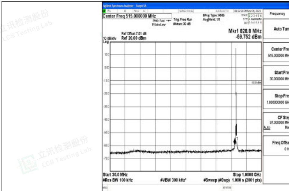
Band5_3MHz_16QAM_20525_1RB#0_30~1000_30~1000
