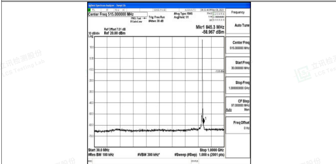
Band5_3MHz_QPSK_20525_1RB#0_30~1000_30~1000
