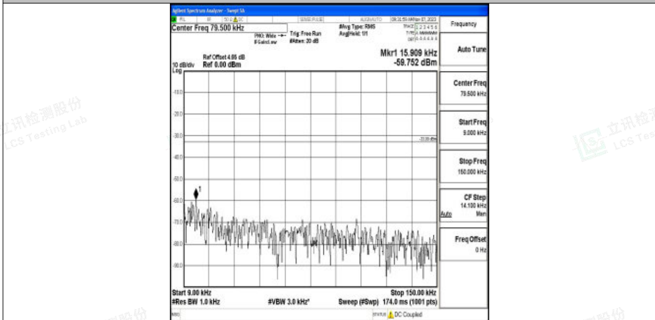
Band5_10MHz_64QAM_20525_1RB#0_0.009~0.15_0.009~0.15
