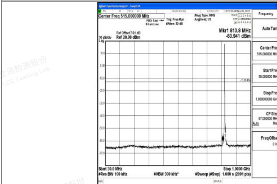
Band5_5MHz_QPSK_20425_1RB#0_30~1000_30~1000
