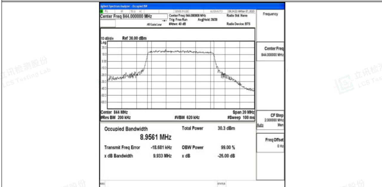
Band5-10MHz-QPSK-20600-50RB#0-PASS
