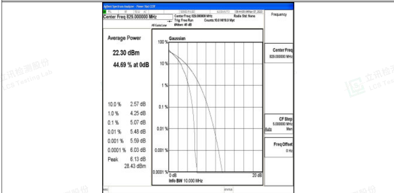
Band5-10MHz-QPSK-20450-1RB#0-PASS
