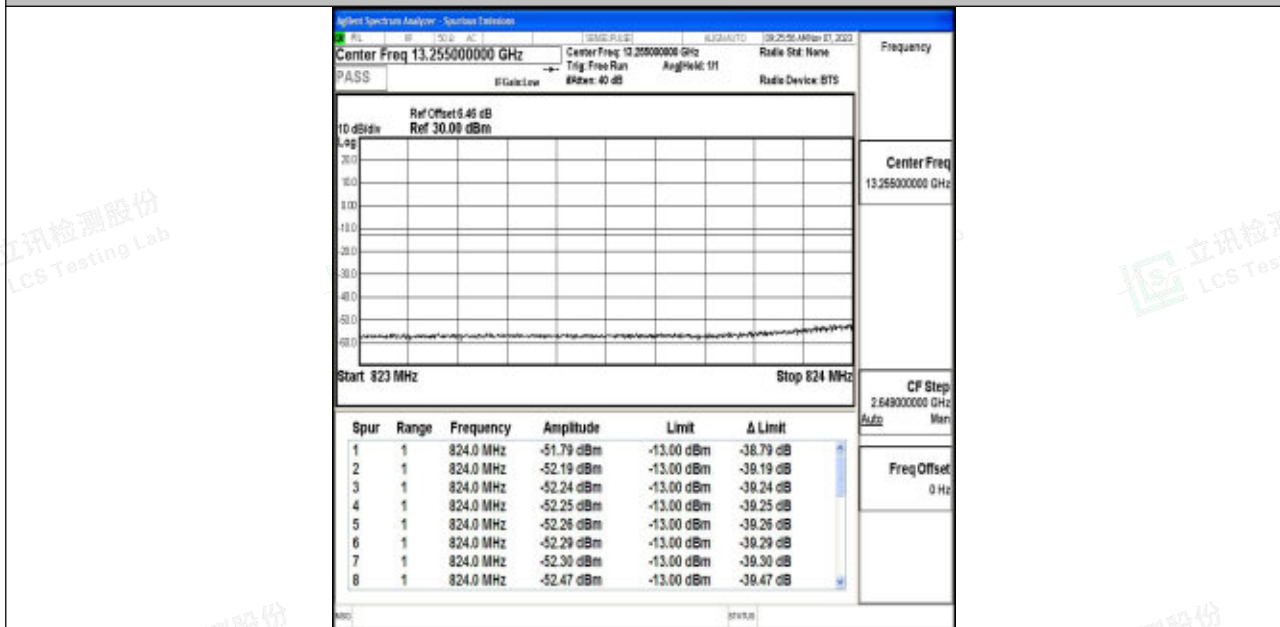
Band5_10MHz_QPSK_20450_1RB#49
