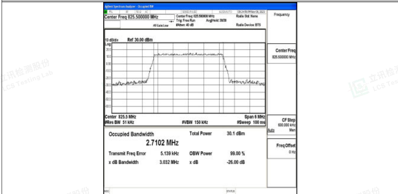
Band5-3MHz-64QAM-20415-15RB#0-PASS
