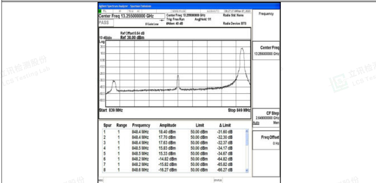
Band5_10MHz_16QAM_20600_1RB#49
