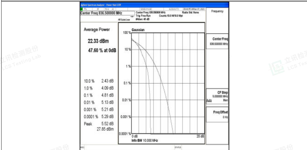
Band5-10MHz-64QAM-20525-1RB#0-PASS
