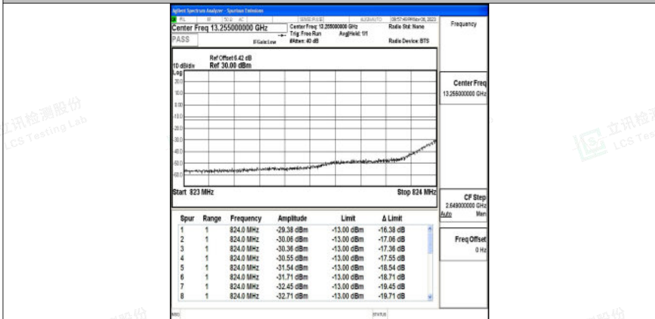
Band5_5MHz_16QAM_20425_1RB#0
