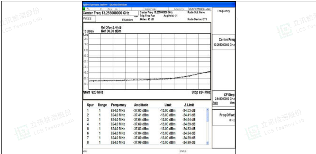
Band5_10MHz_64QAM_20450_1RB#0
