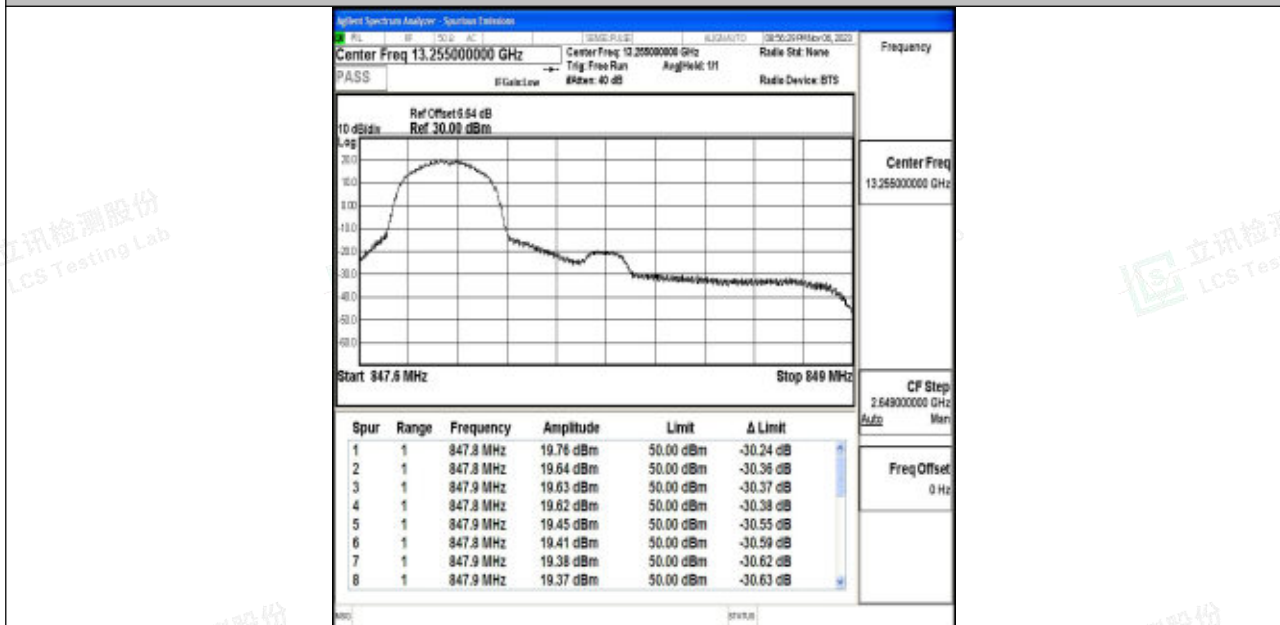
Band5_1.4MHz_64QAM_20643_1RB#0
