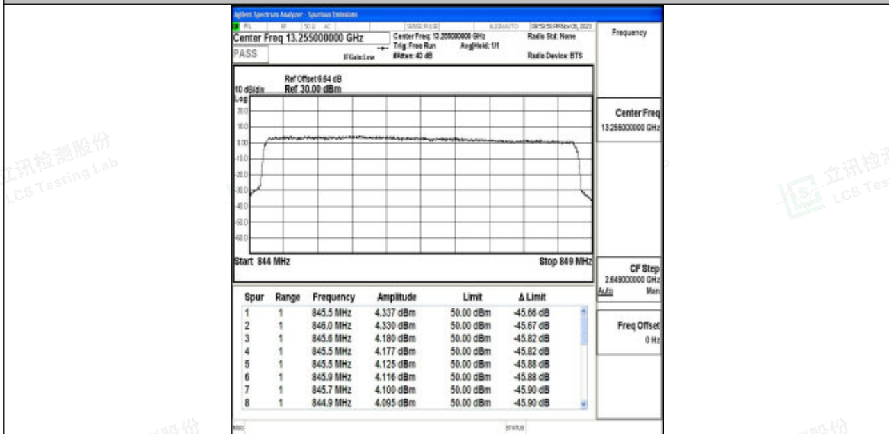
Band5_5MHz_64QAM_20625_25RB#0
