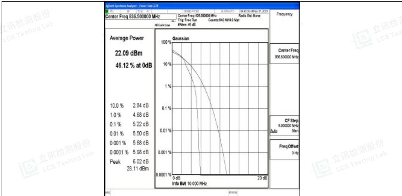
Band5-10MHz-16QAM-20525-1RB#0-PASS
