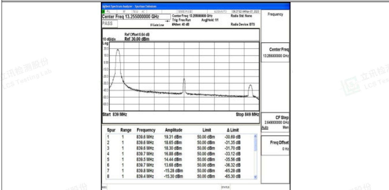
Band5_10MHz_64QAM_20600_1RB#0
