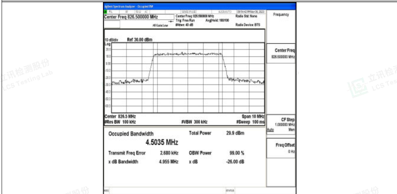
Band5-5MHz-16QAM-20425-25RB#0-PASS
