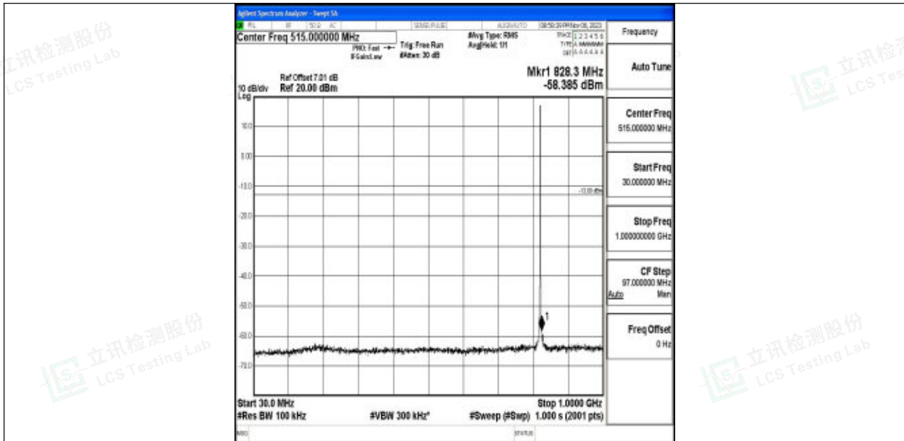
Band5_1.4MHz_16QAM_20407_1RB#0_30~1000_30~1000
