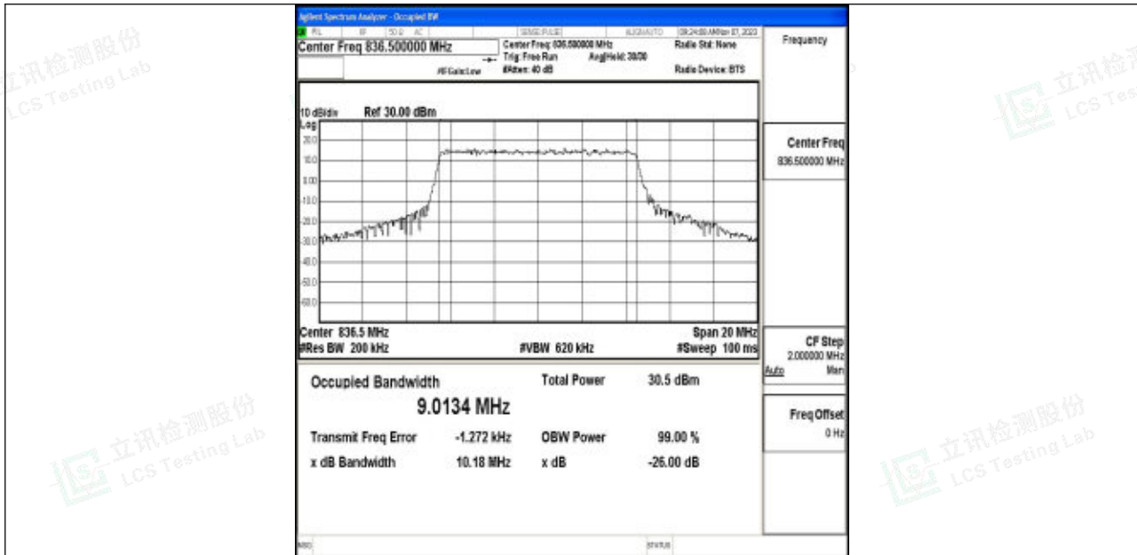
Band5-10MHz-64QAM-20525-50RB#0-PASS
