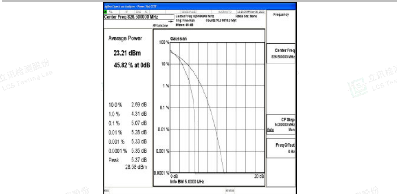
Band5-5MHz-QPSK-20425-1RB#0-PASS
