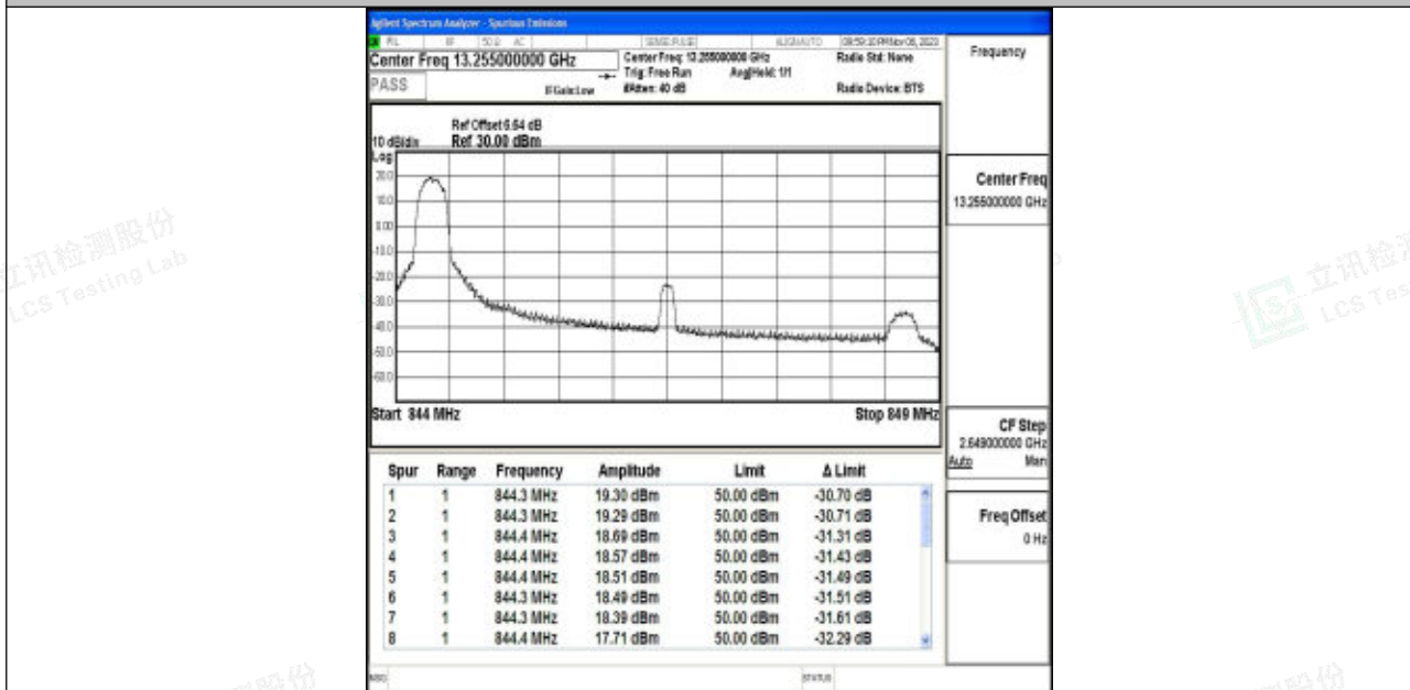
Band5_5MHz_64QAM_20625_1RB#0
