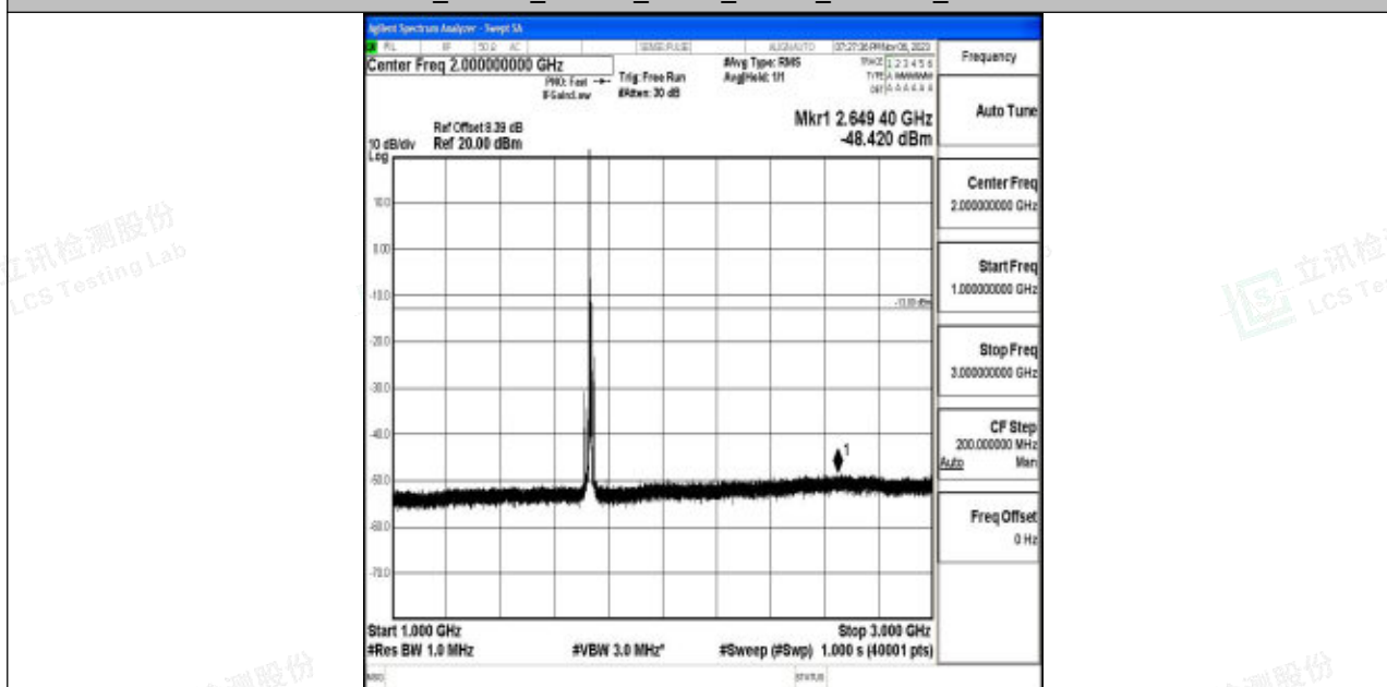
Band4_10MHz_16QAM_20175_1RB#0_1000~3000_1000~3000
