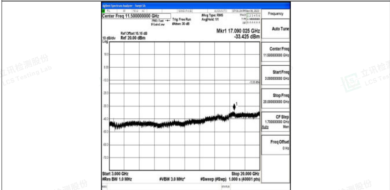
Band4_5MHz_QPSK_20375_1RB#0_3000~20000_3000~20000
