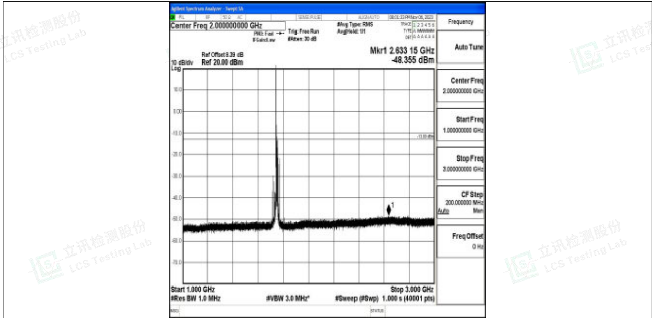
Band4_15MHz_64QAM_20325_1RB#0_1000~3000_1000~3000
