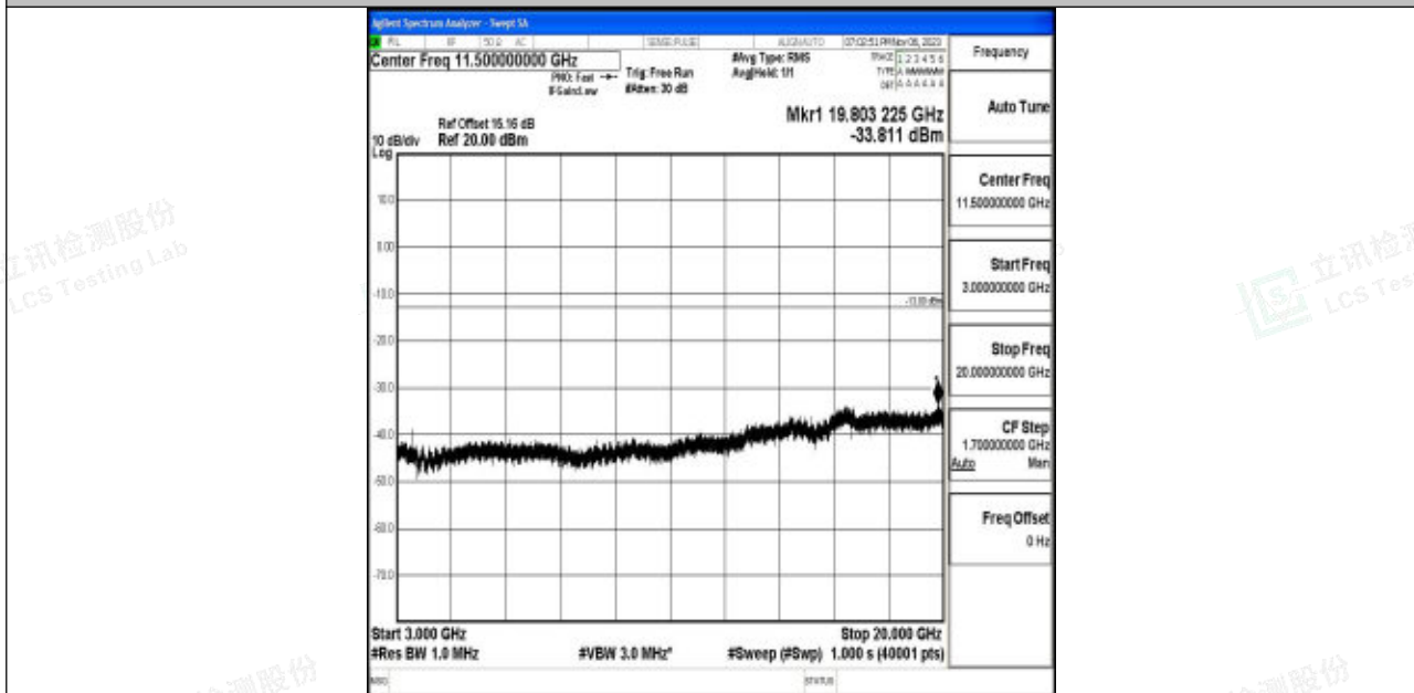
Band4_5MHz_64QAM_20375_1RB#0_3000~20000_3000~20000
