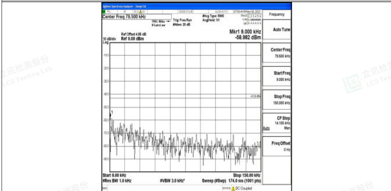
Band4_15MHz_QPSK_20325_1RB#0_0.009~0.15_0.009~0.15
