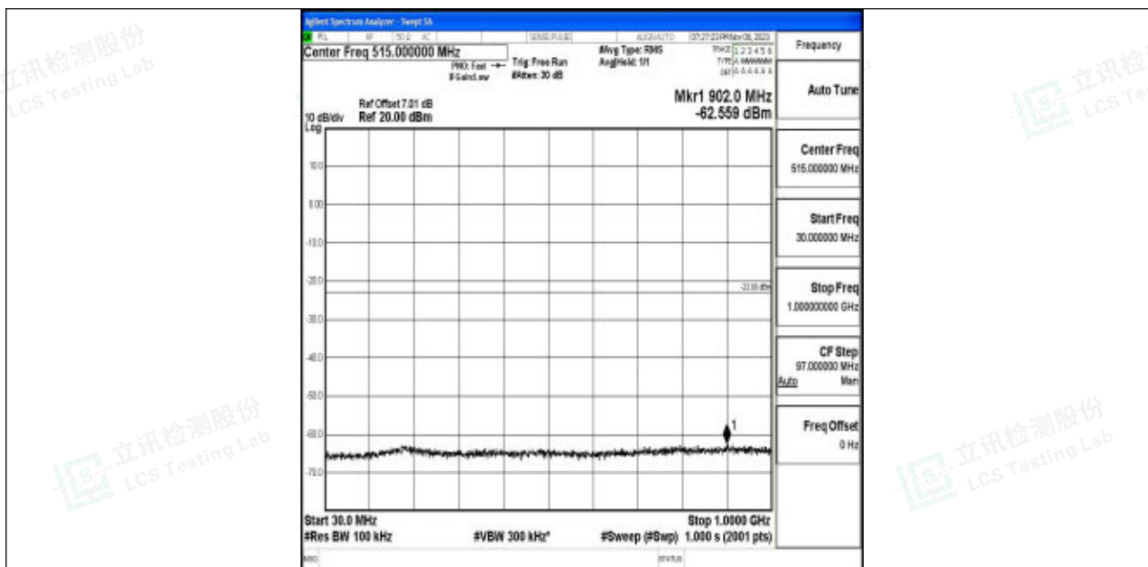
Band4_10MHz_16QAM_20175_1RB#0_30~1000_30~1000
