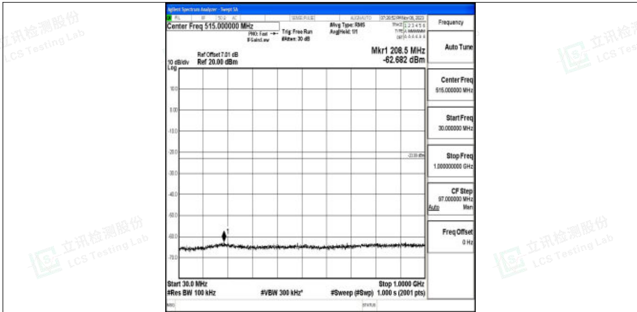
Band4_10MHz_QPSK_20350_1RB#0_30~1000_30~1000
