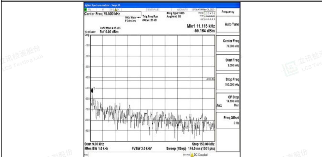
Band4_15MHz_64QAM_20025_1RB#0_0.009~0.15_0.009~0.15
