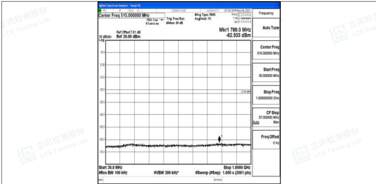
Band4_10MHz_64QAM_20350_1RB#0_30~1000_30~1000
