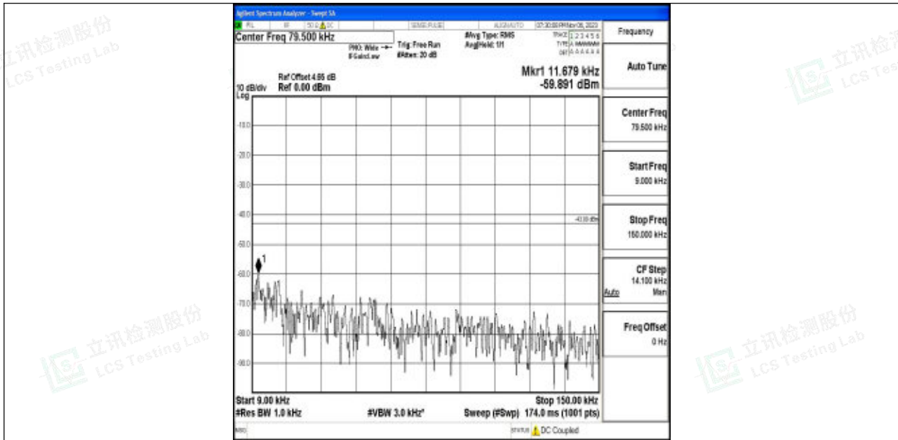
Band4_10MHz_64QAM_20350_1RB#0_0.009~0.15_0.009~0.15
