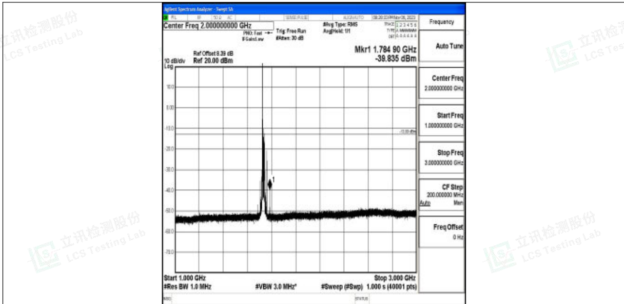
Band4_20MHz_QPSK_20175_1RB#0_1000~3000_1000~3000
