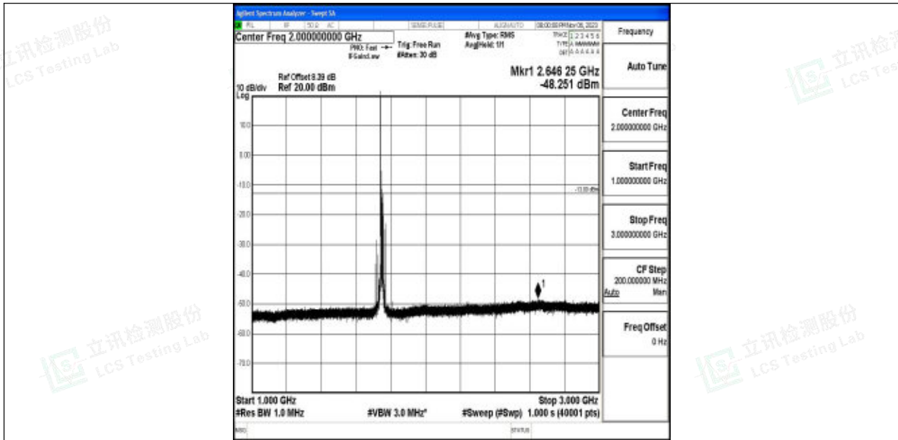
Band4_15MHz_QPSK_20325_1RB#0_1000~3000_1000~3000
