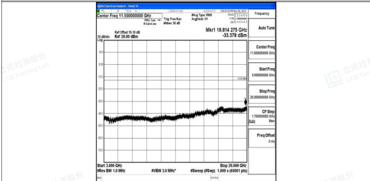
Band4_15MHz_QPSK_20325_1RB#0_3000~20000_3000~20000
