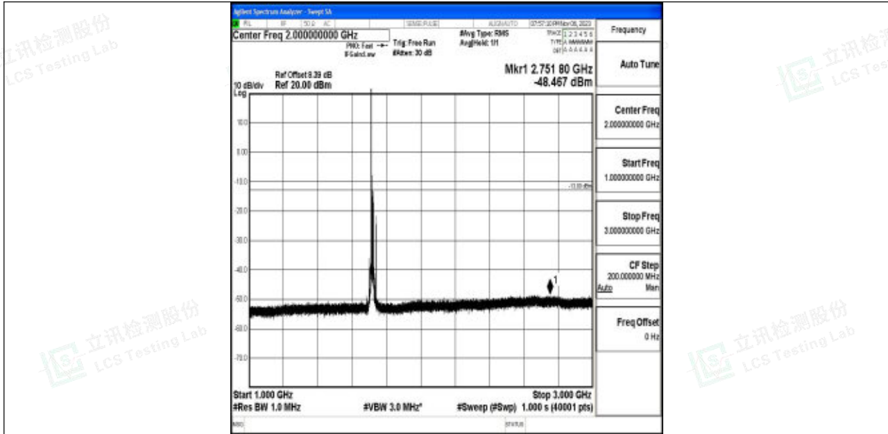
Band4_15MHz_64QAM_20025_1RB#0_1000~3000_1000~3000
