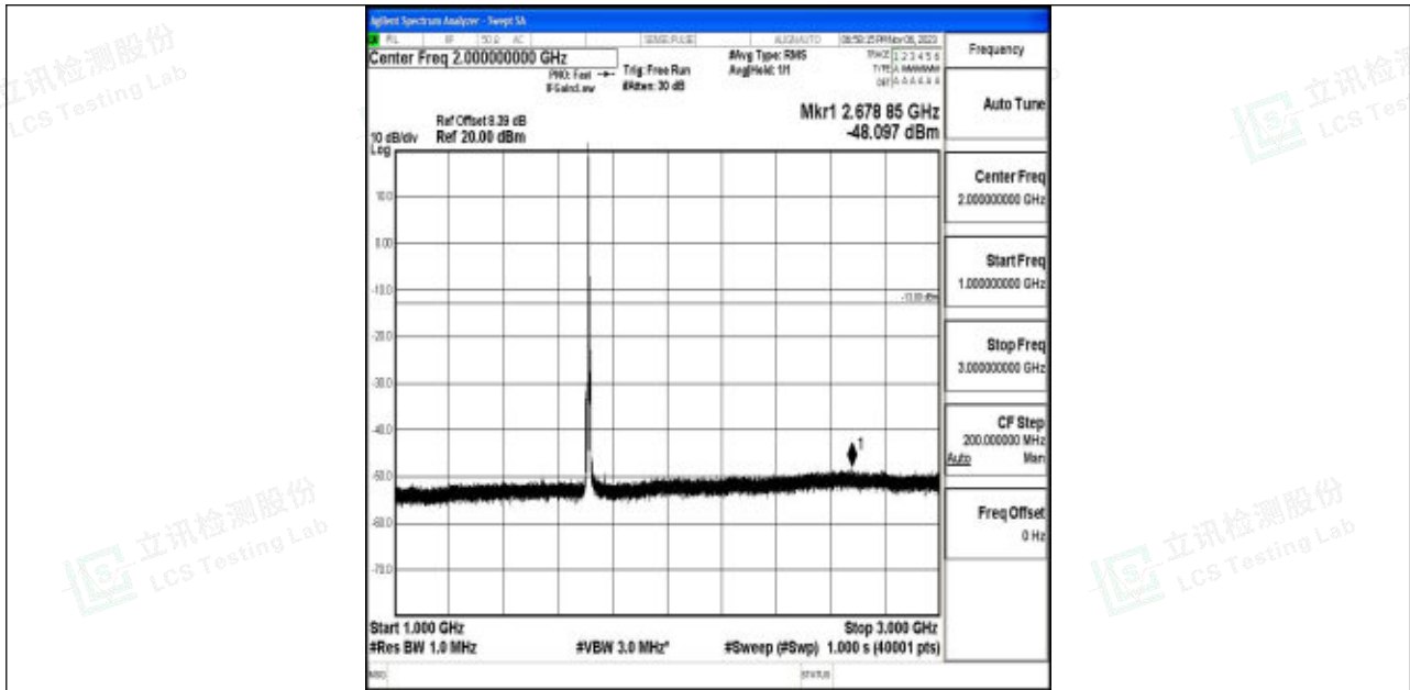
Band4_5MHz_64QAM_19975_1RB#0_1000~3000_1000~3000
