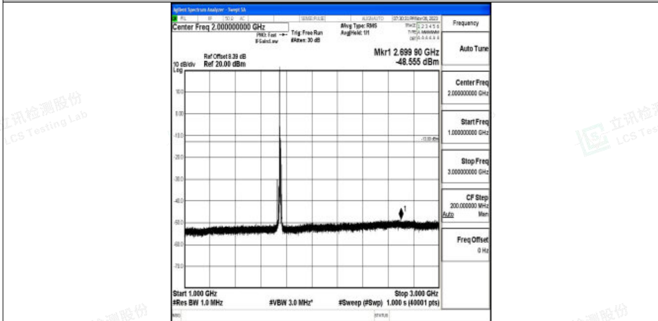
Band4_10MHz_64QAM_20350_1RB#0_1000~3000_1000~3000
