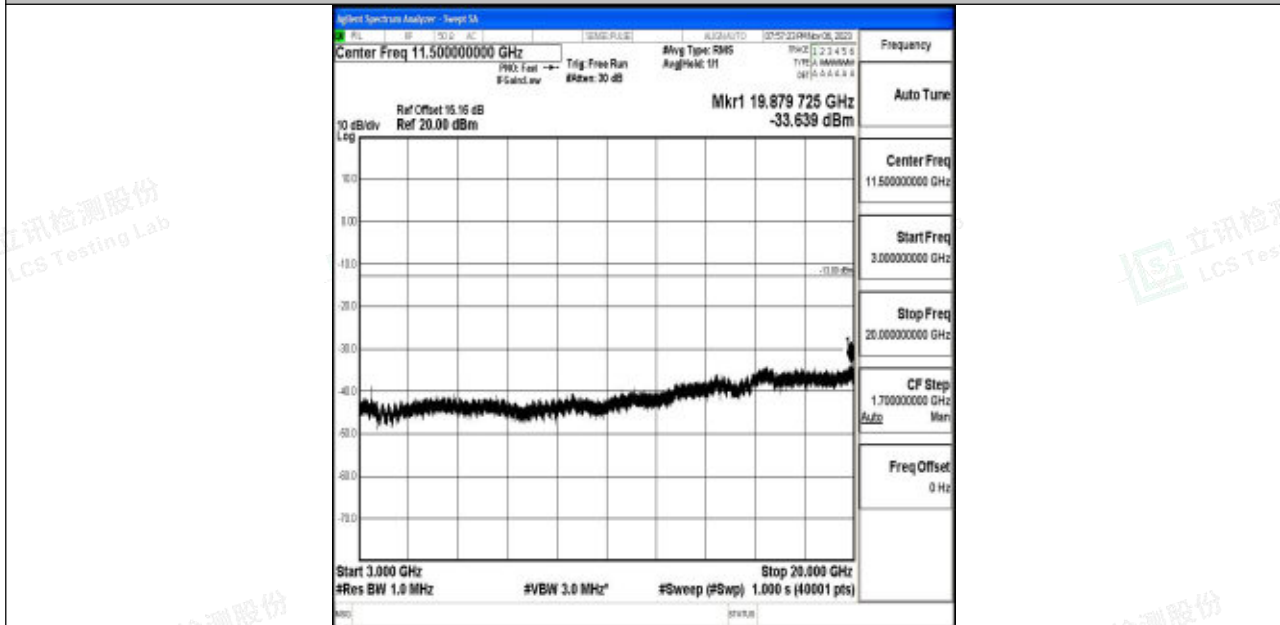
Band4_15MHz_64QAM_20025_1RB#0_3000~20000_3000~20000
