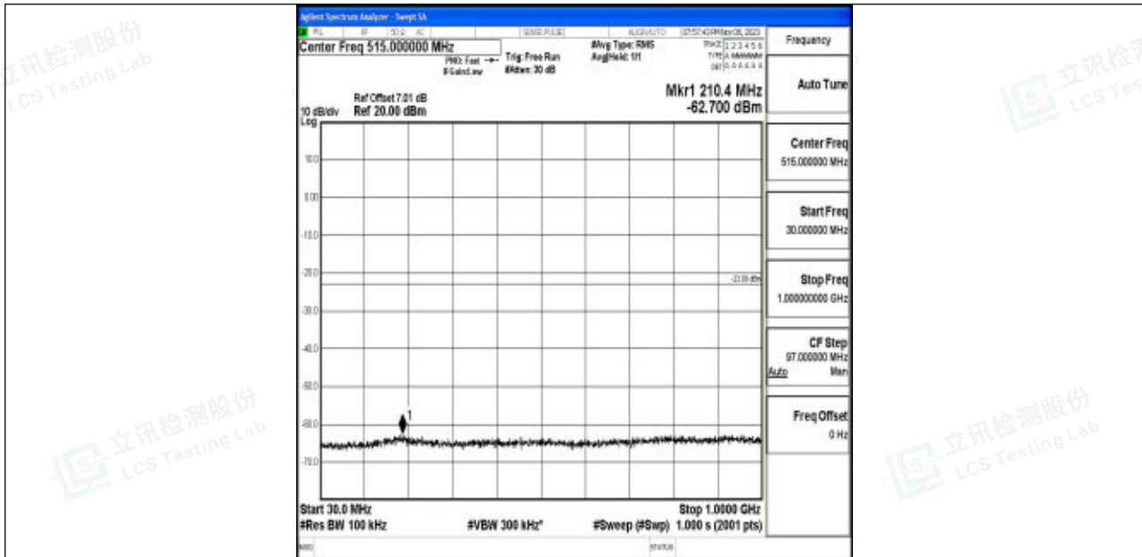
Band4_15MHz_QPSK_20175_1RB#0_30~1000_30~1000
