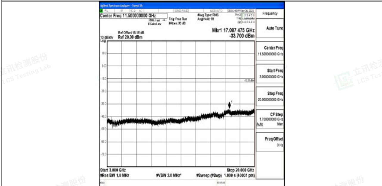
Band4_15MHz_64QAM_20325_1RB#0_3000~20000_3000~20000
