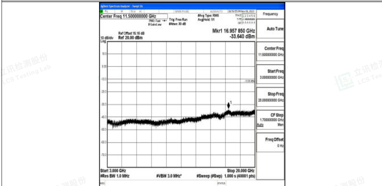
Band4_5MHz_16QAM_20175_1RB#0_3000~20000_3000~20000
