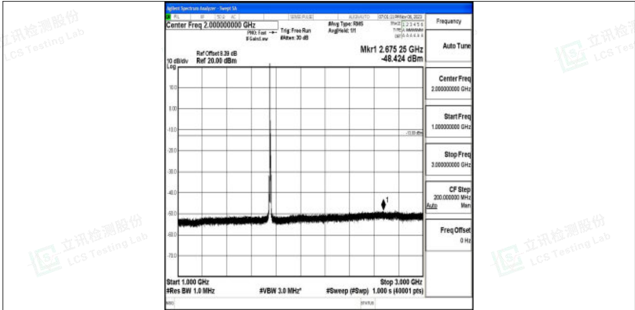
Band4_5MHz_QPSK_20375_1RB#0_1000~3000_1000~3000
