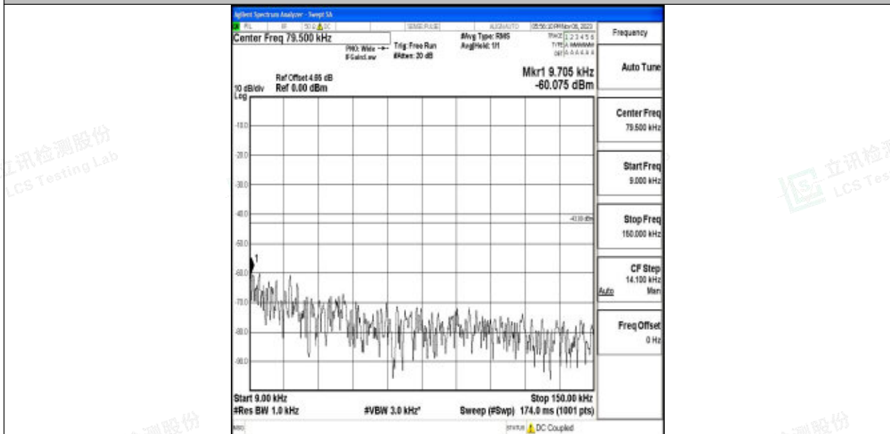
Band4_1.4MHz_64QAM_19957_1RB#0_0.009~0.15_0.009~0.15
