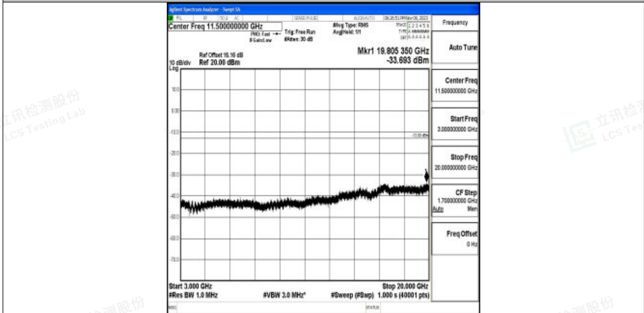
Band4_3MHz_QPSK_20175_1RB#0_3000~20000_3000~20000
