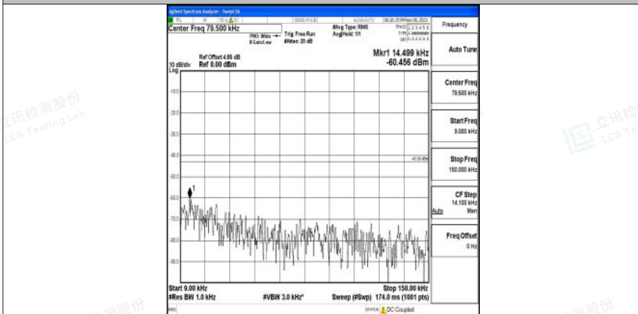
Band4_3MHz_QPSK_20175_1RB#0_0.009~0.15_0.009~0.15
