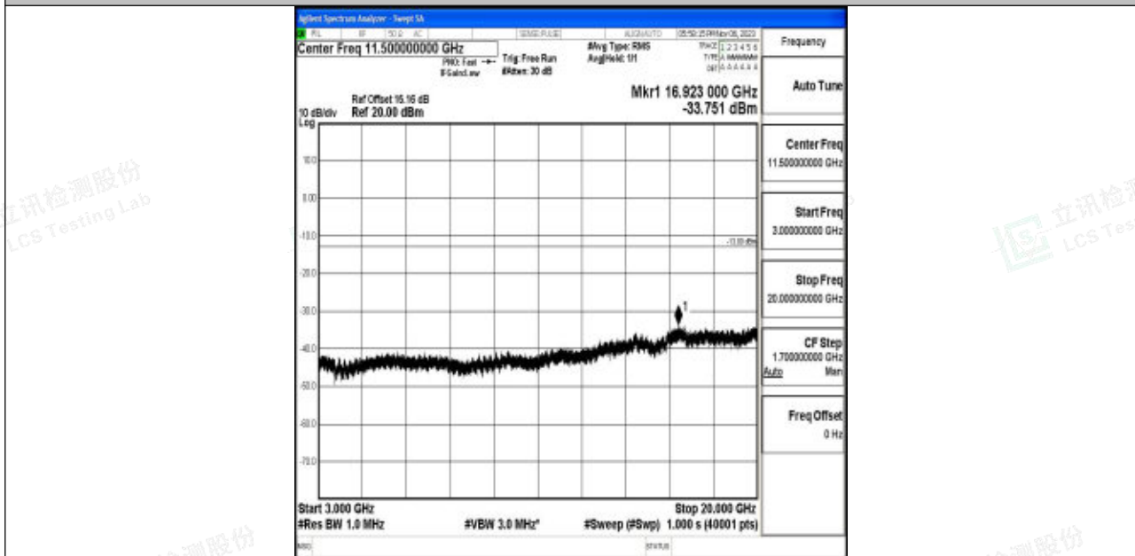
Band4_1.4MHz_16QAM_20175_1RB#0_3000~20000_3000~20000
