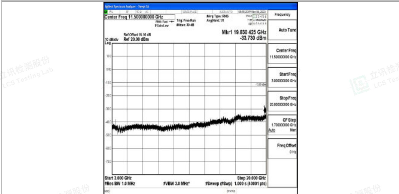
Band4_1.4MHz_QPSK_19957_1RB#0_3000~20000_3000~20000
