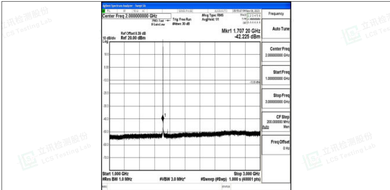
Band4_1.4MHz_QPSK_19957_1RB#0_1000~3000_1000~3000
