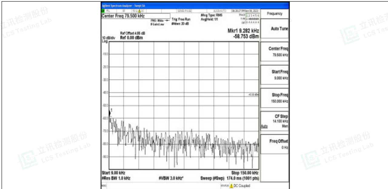
Band4_3MHz_QPSK_20385_1RB#0_0.009~0.15_0.009~0.15
