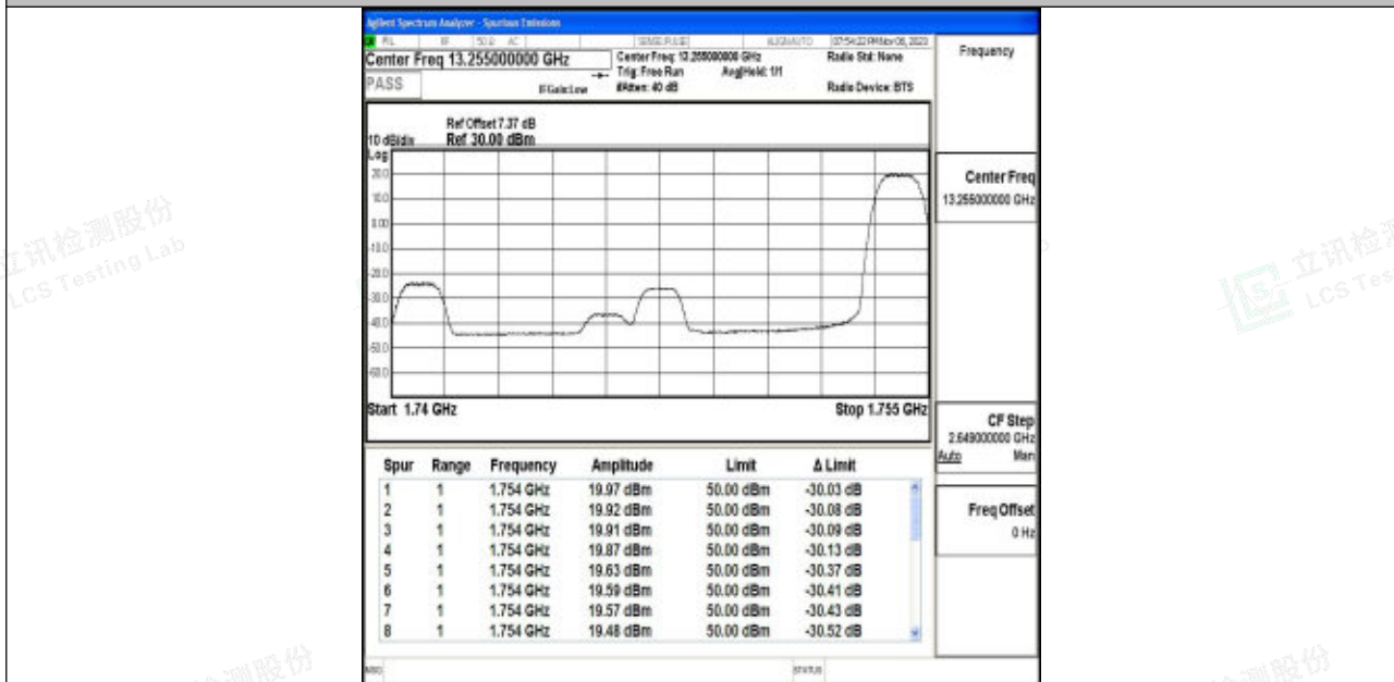
Band4_15MHz_16QAM_20325_1RB#74
