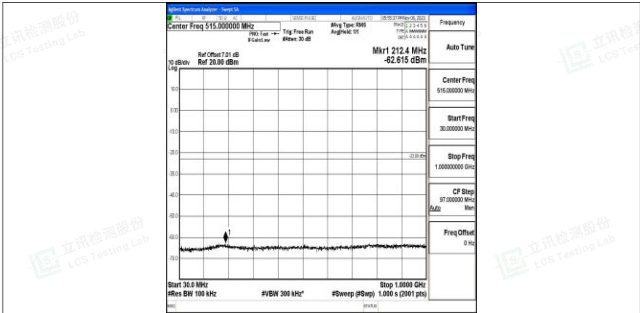
Band4_1.4MHz_16QAM_19957_1RB#0_30~1000_30~1000
