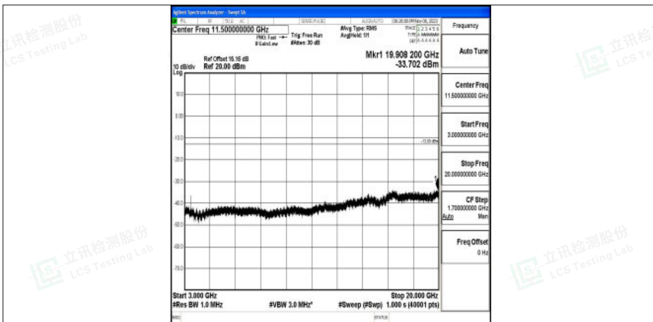
Band4_3MHz_64QAM_19965_1RB#0_3000~20000_3000~20000
