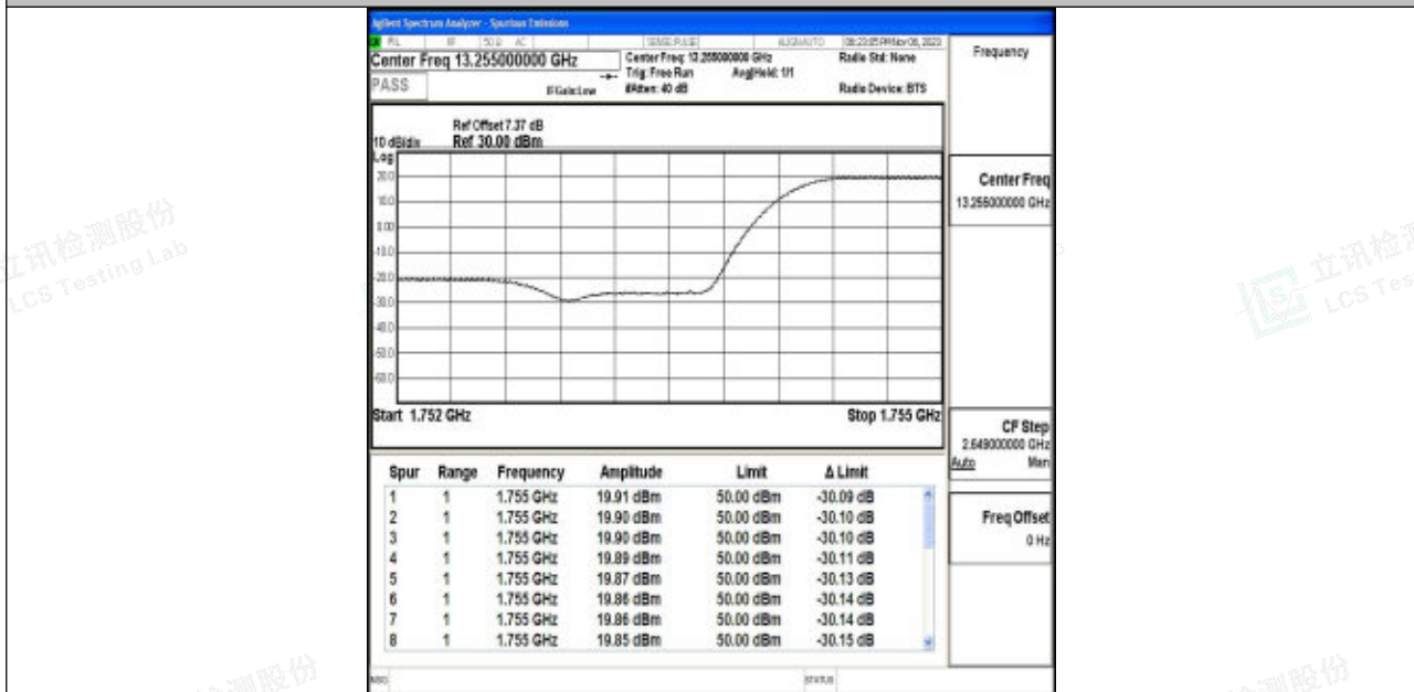
Band4_3MHz_16QAM_20385_1RB#14
