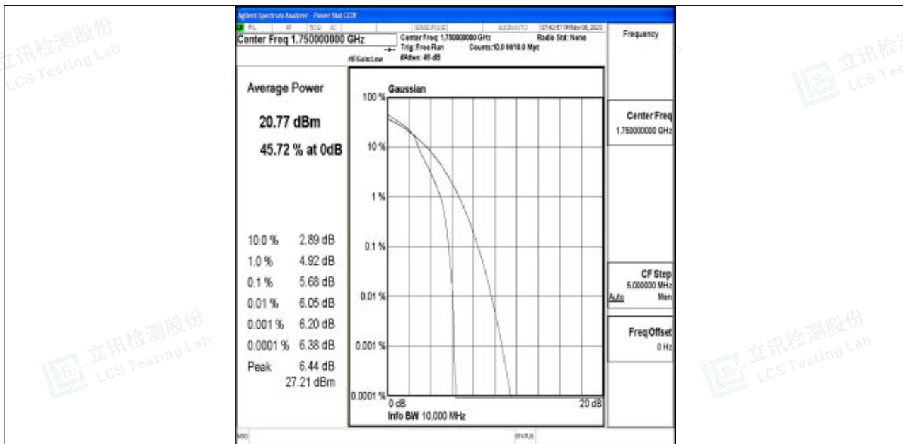
Band4-10MHz-16QAM-20350-1RB#0-PASS
