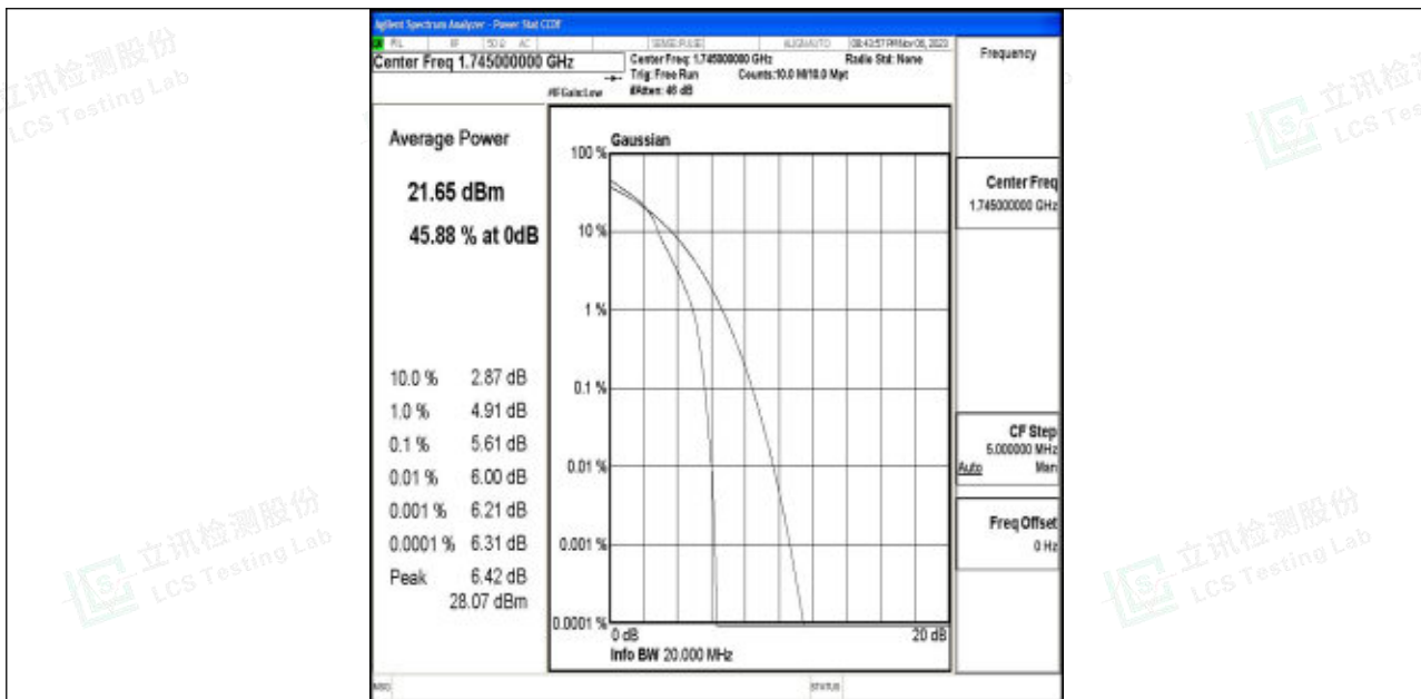
Band4-20MHz-16QAM-20300-1RB#0-PASS
