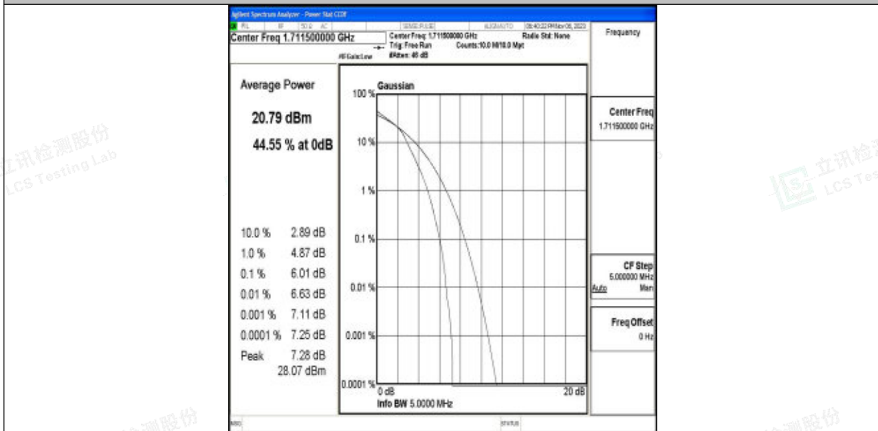
Band4-3MHz-16QAM-19965-15RB#0-PASS
