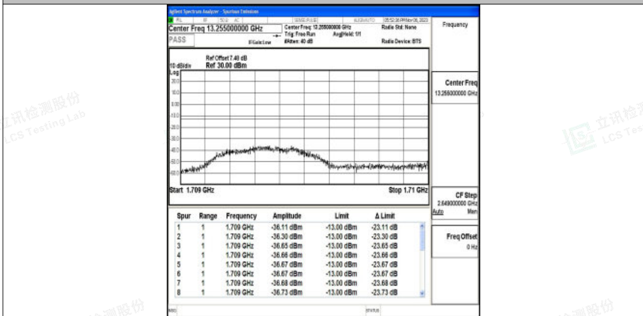
Band4_1.4MHz_64QAM_19957_1RB#5
