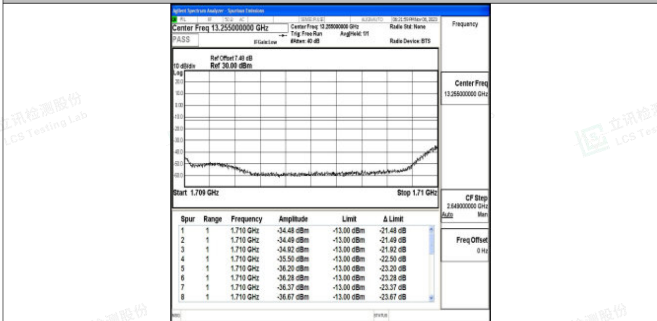
Band4_3MHz_64QAM_19965_1RB#14
