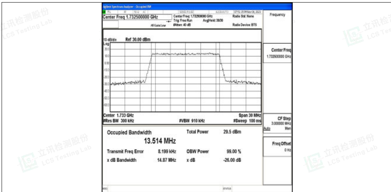
Band4-15MHz-16QAM-20175-75RB#0-PASS
