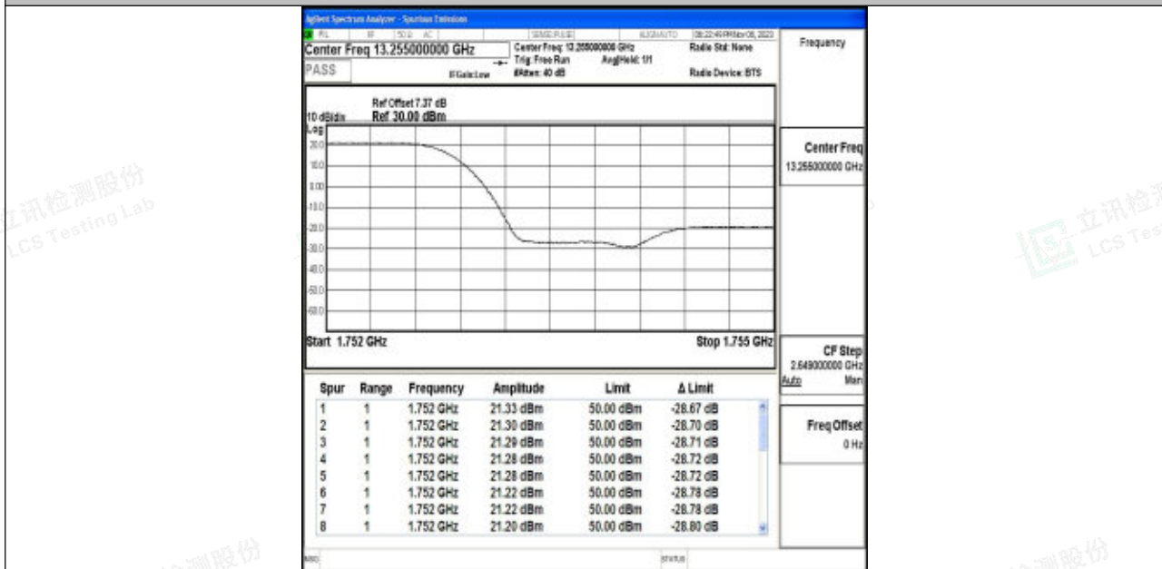
Band4_3MHz_64QAM_20385_1RB#0
