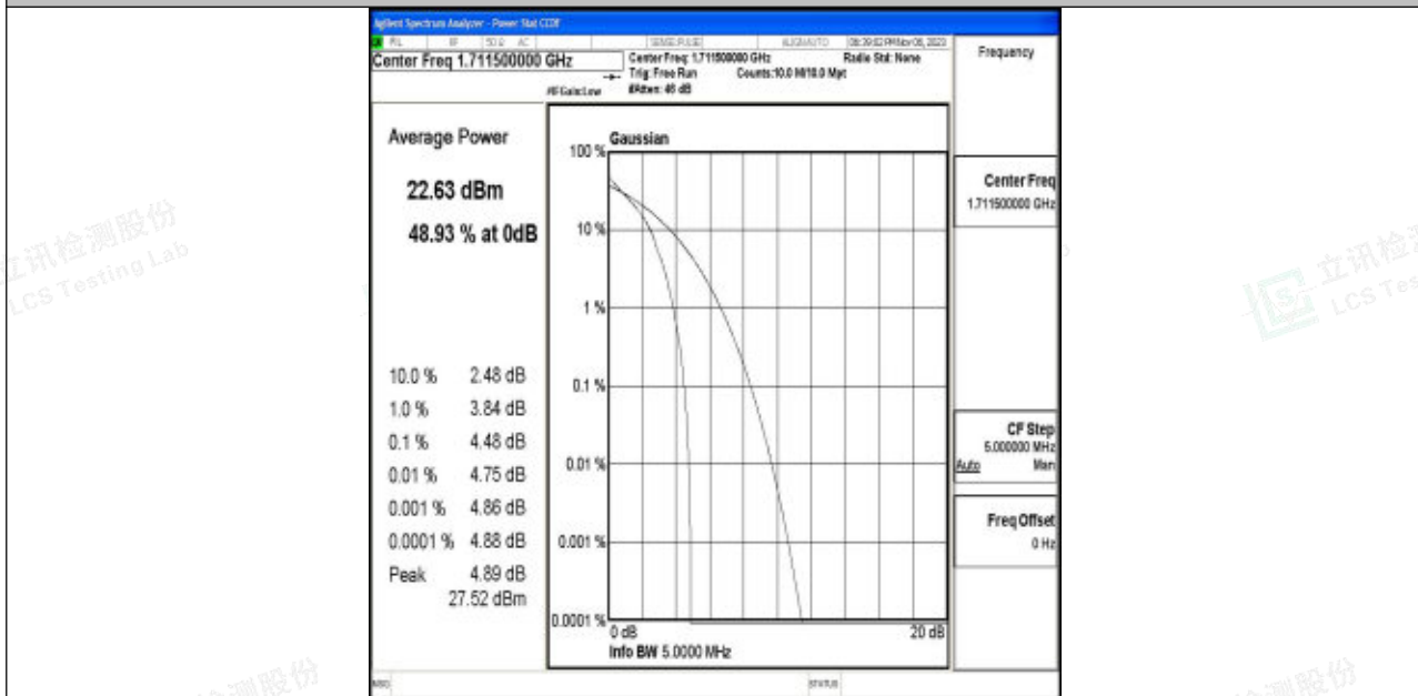
Band4-3MHz-64QAM-19965-1RB#0-PASS
