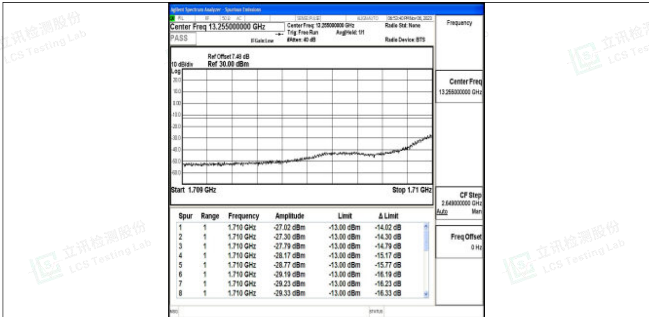
Band4_5MHz_QPSK_19975_1RB#0
