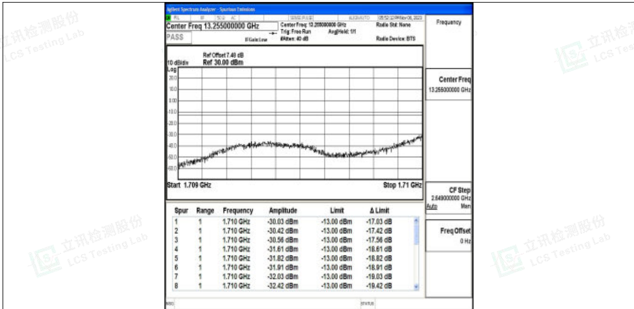
Band4_1.4MHz_64QAM_19957_1RB#0
