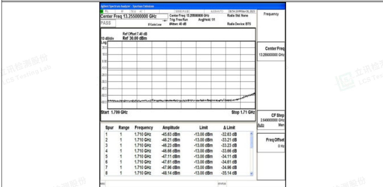
Band4_5MHz_64QAM_19975_1RB#24
