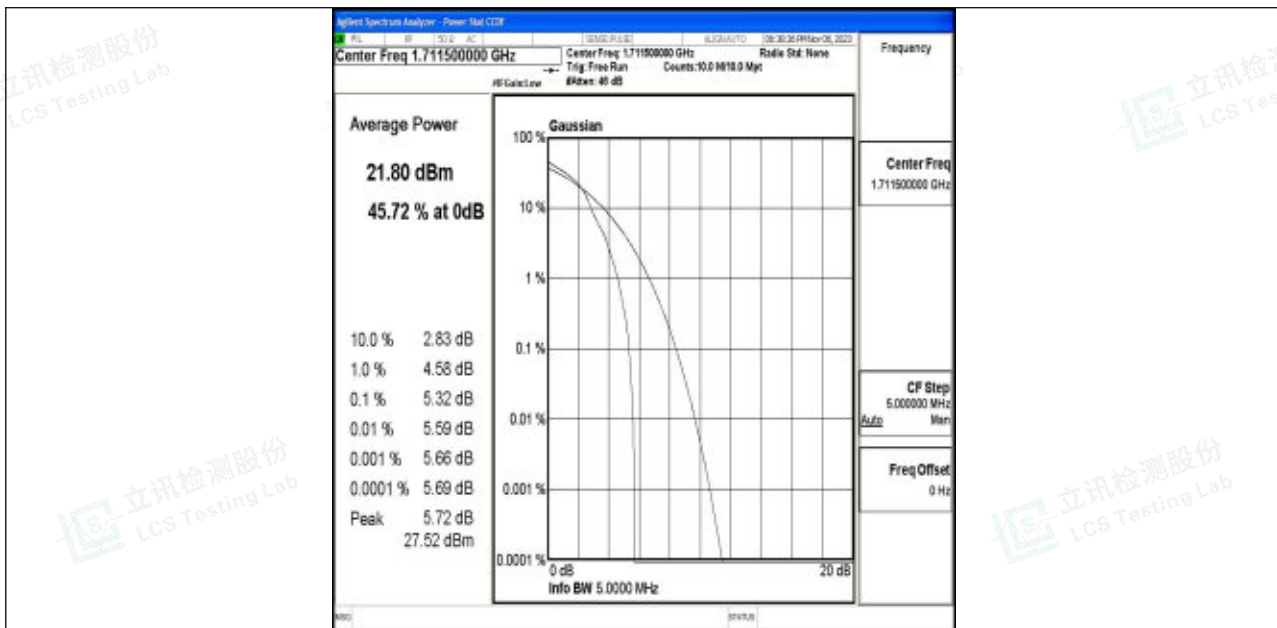
Band4-3MHz-16QAM-19965-1RB#0-PASS
