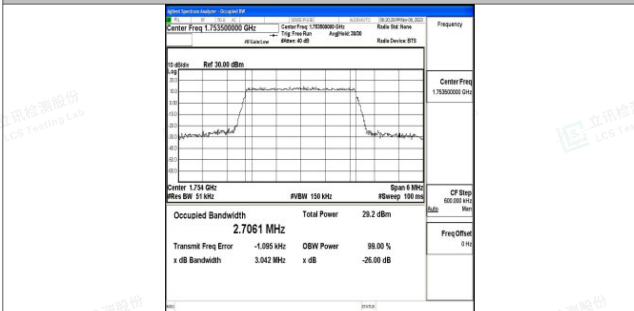
Band4-3MHz-QPSK-20385-15RB#0-PASS
