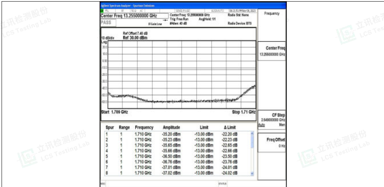
Band4_3MHz_16QAM_19965_1RB#14
