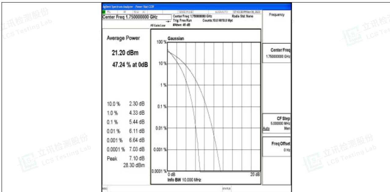
Band4-10MHz-QPSK-20350-50RB#0-PASS
