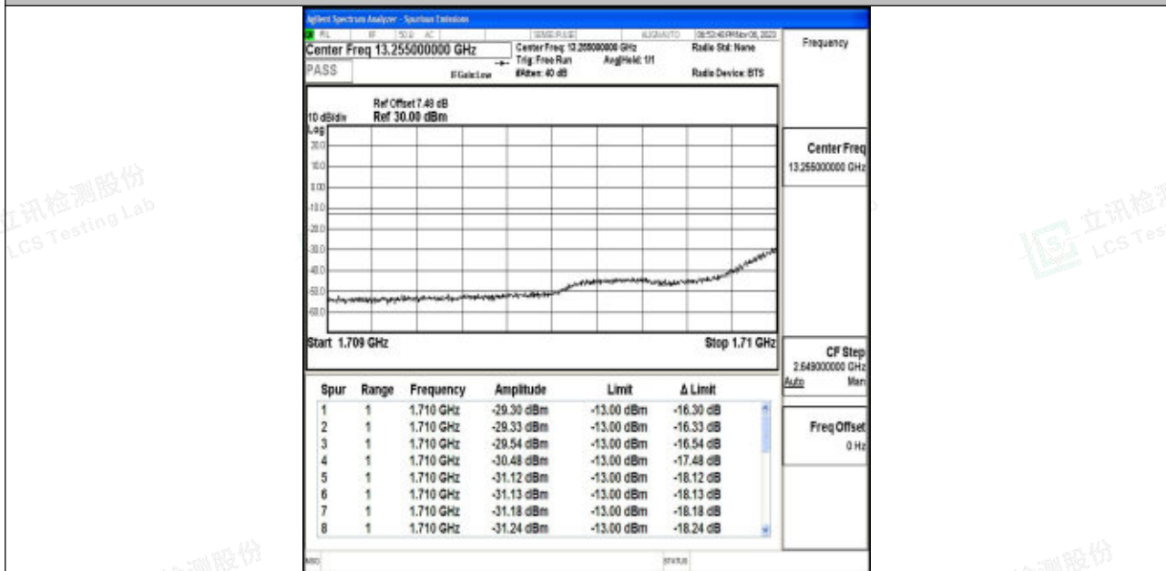
Band4_5MHz_16QAM_19975_1RB#0
