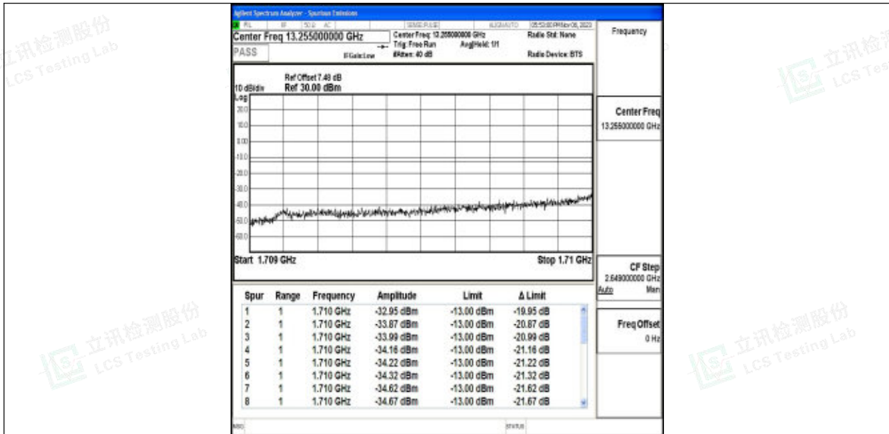
Band4_1.4MHz_64QAM_19957_6RB#0
