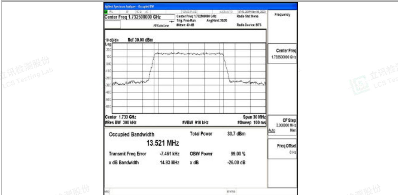
Band4-15MHz-64QAM-20175-75RB#0-PASS
