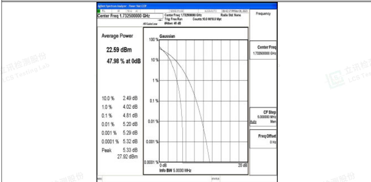
Band4-3MHz-64QAM-20175-1RB#0-PASS
