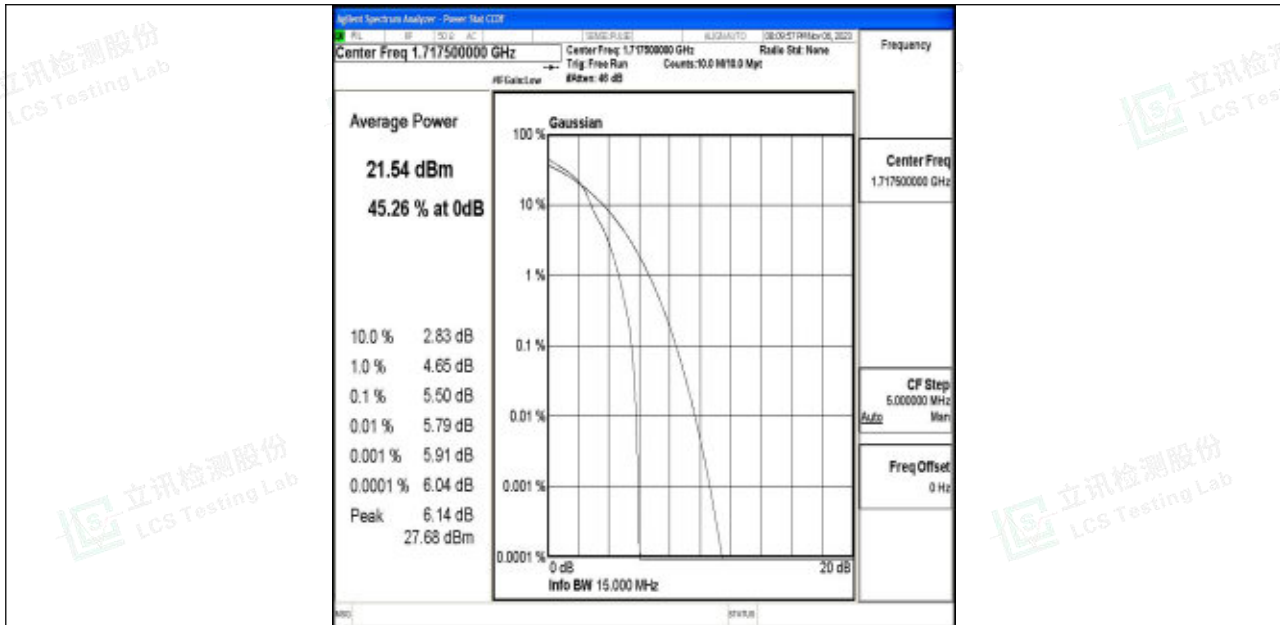
Band4-15MHz-16QAM-20025-1RB#0-PASS
