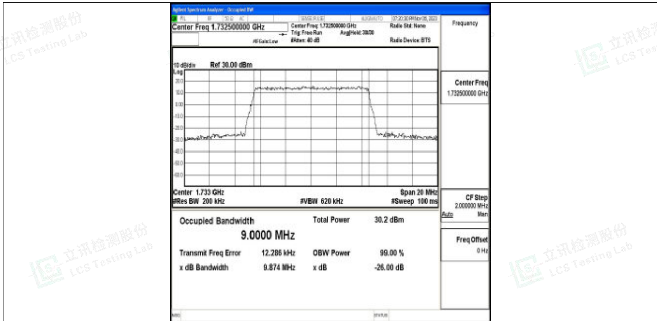
Band4-10MHz-64QAM-20175-50RB#0-PASS
