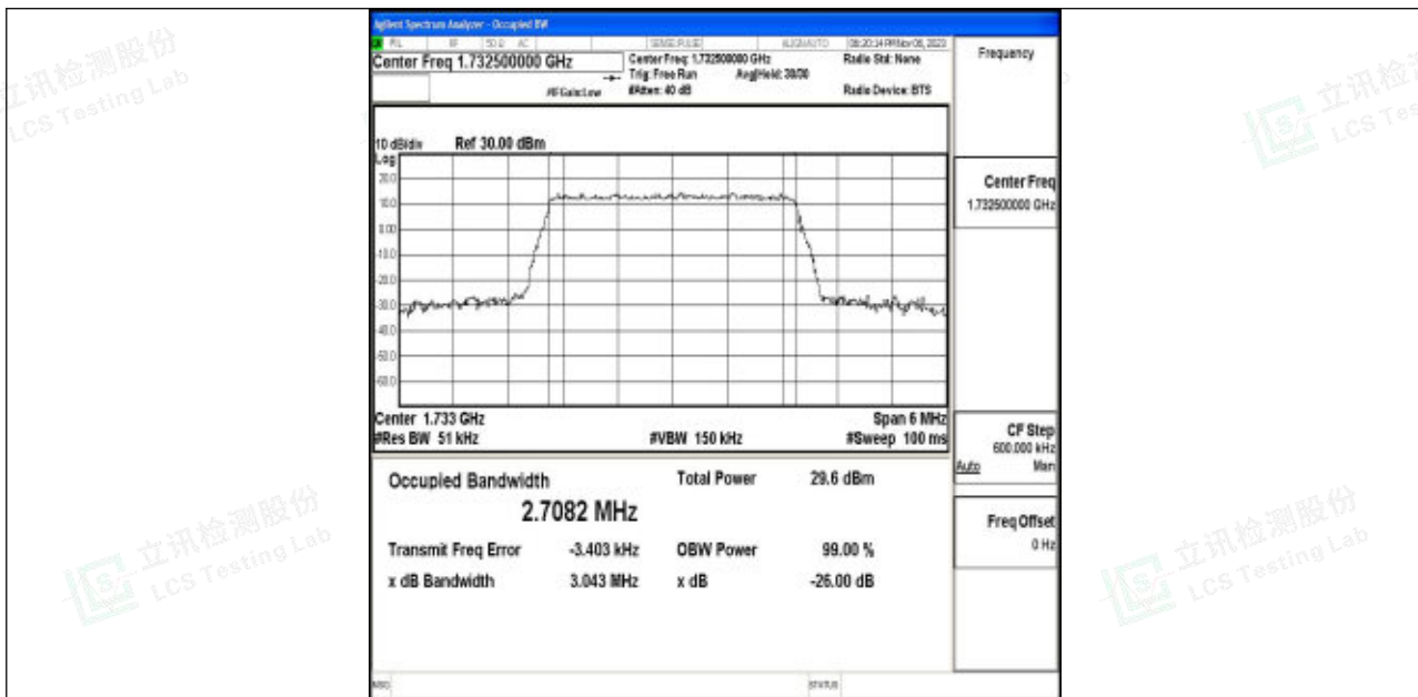
Band4-3MHz-64QAM-20175-15RB#0-PASS
