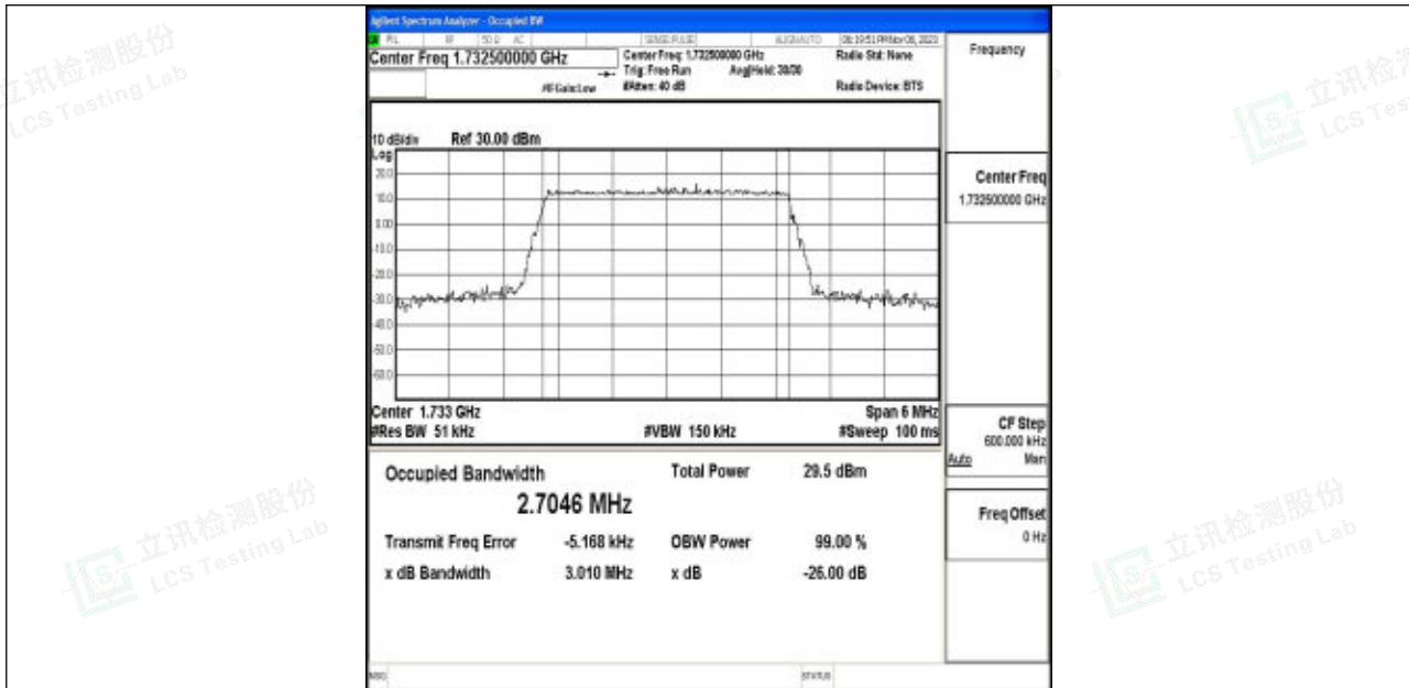
Band4-3MHz-QPSK-20175-15RB#0-PASS
