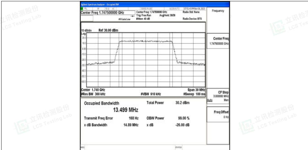
Band4-15MHz-QPSK-20325-75RB#0-PASS
