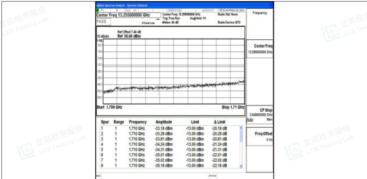
Band4_1.4MHz_QPSK_19957_6RB#0
