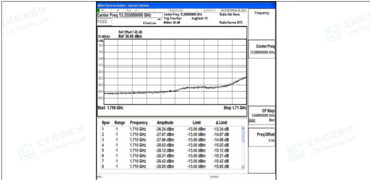
Band4_5MHz_64QAM_19975_1RB#0
