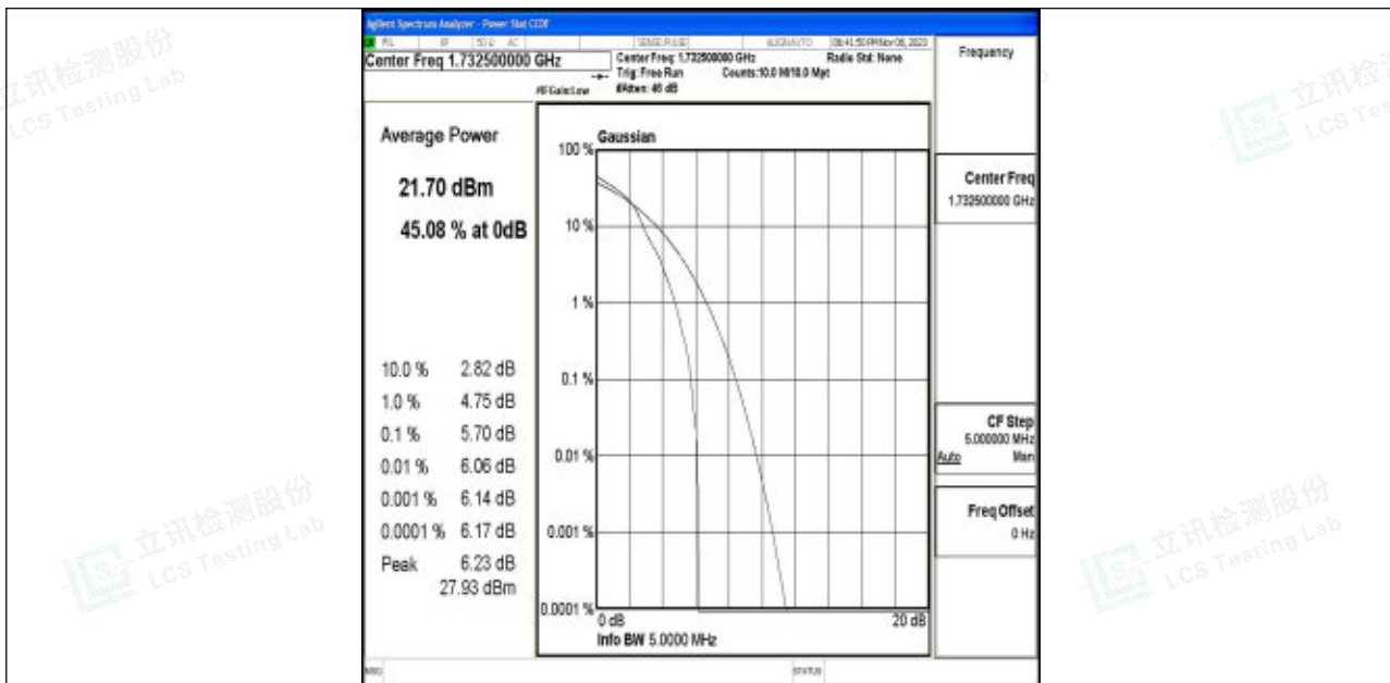
Band4-3MHz-16QAM-20175-1RB#0-PASS
