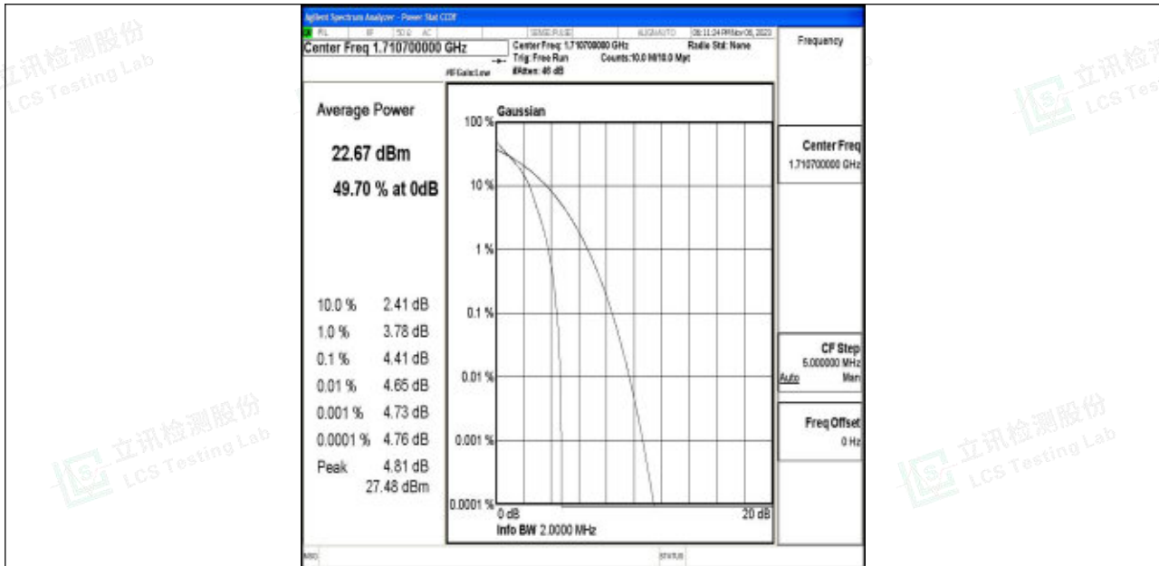
Band4-1.4MHz-64QAM-19957-1RB#0-PASS
