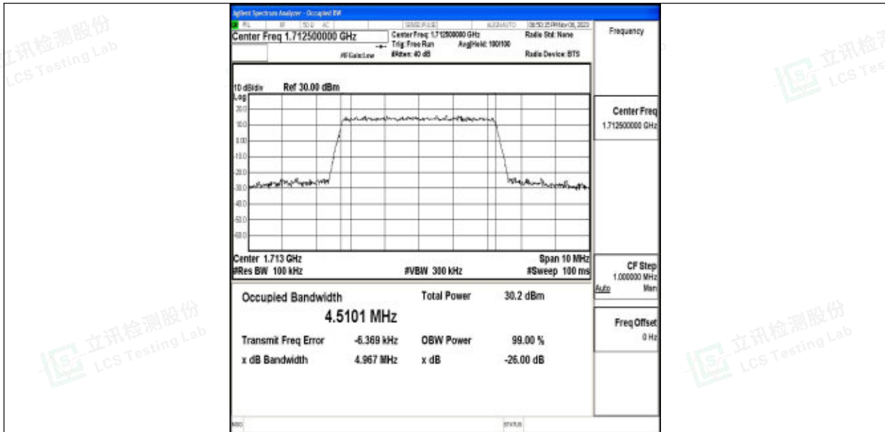
Band4-5MHz-QPSK-19975-25RB#0-PASS
