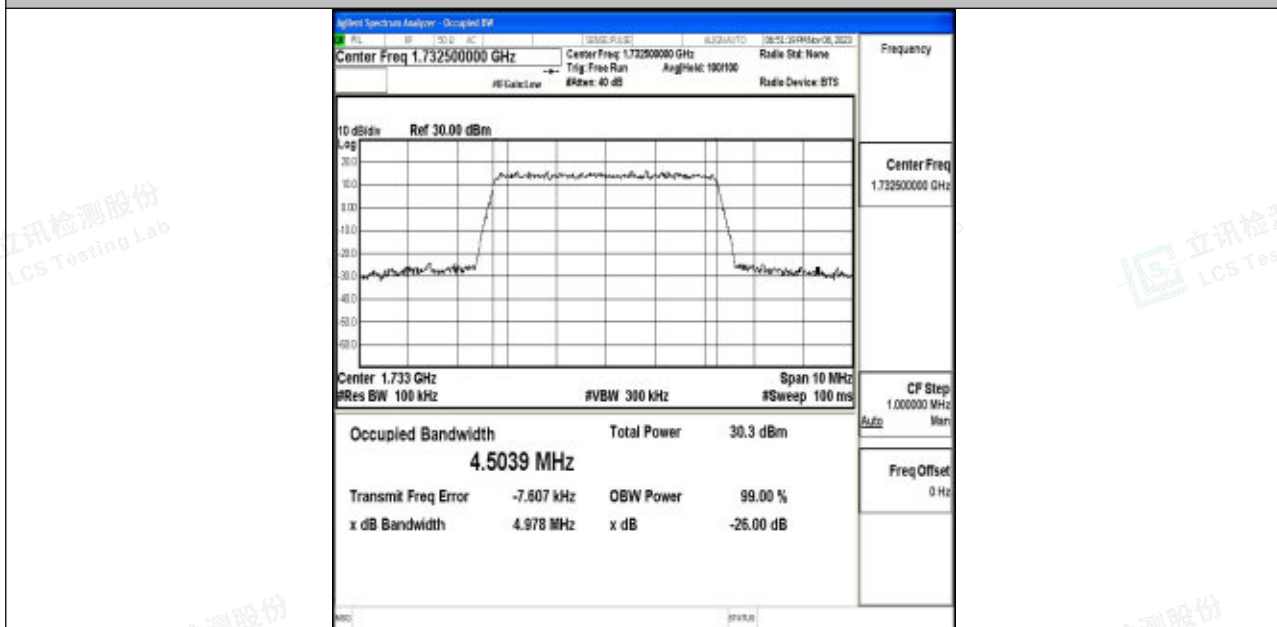
Band4-5MHz-QPSK-20175-25RB#0-PASS
