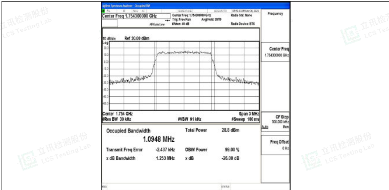
Band4-1.4MHz-QPSK-20393-6RB#0-PASS
