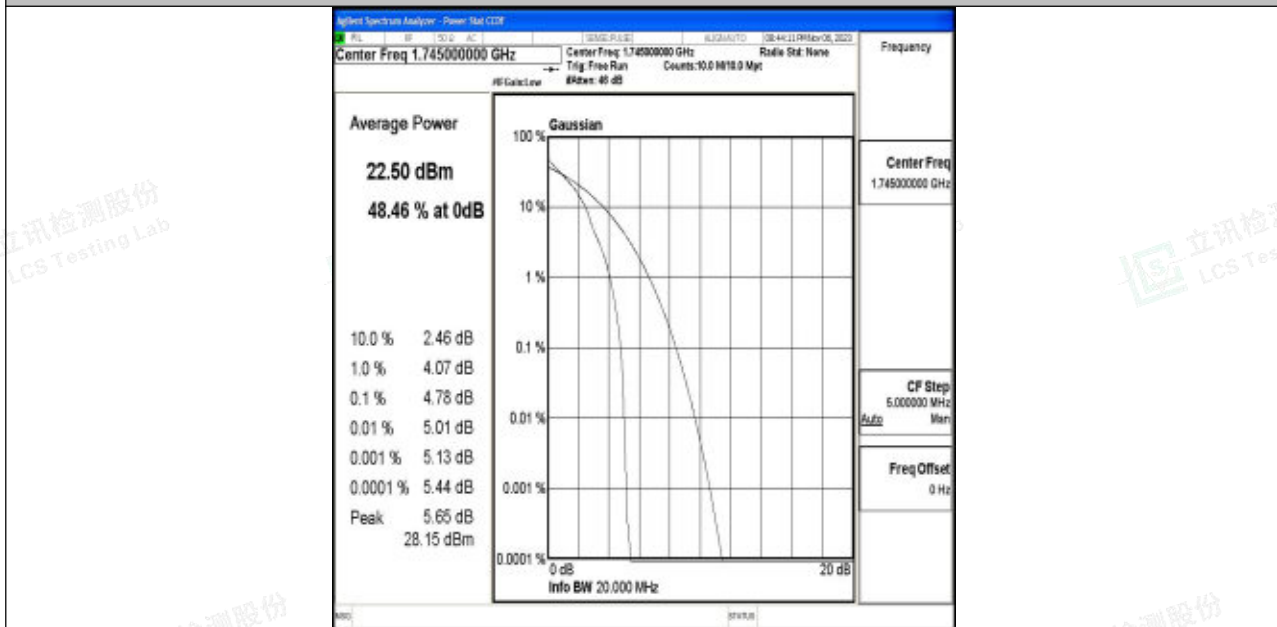
Band4-20MHz-64QAM-20300-1RB#0-PASS
