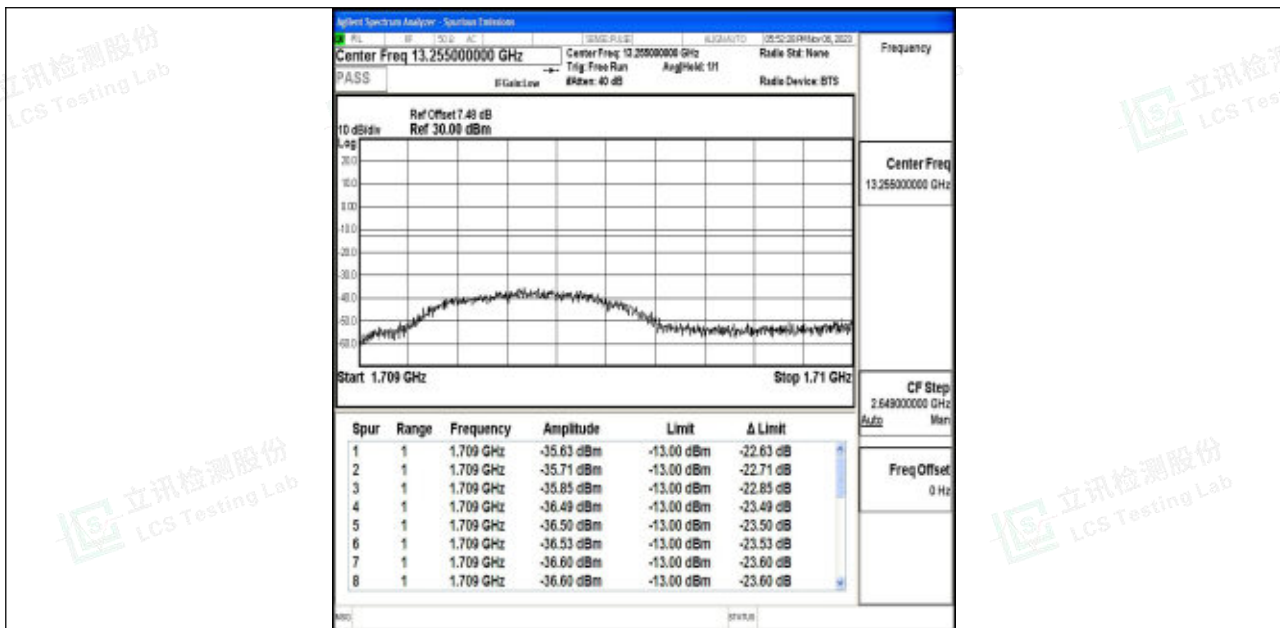
Band4_1.4MHz_16QAM_19957_1RB#5
