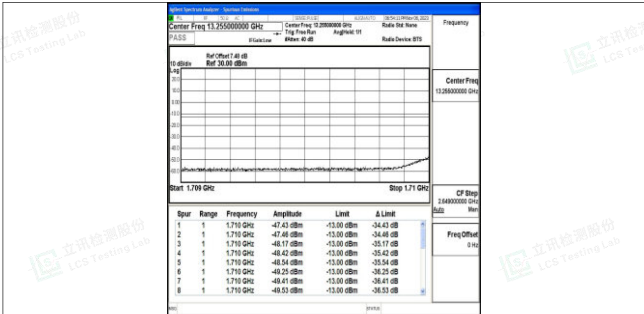
Band4_5MHz_16QAM_19975_1RB#24
