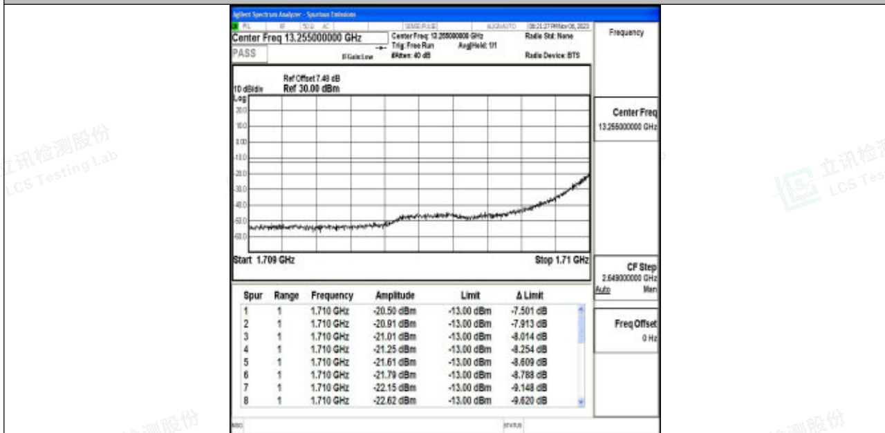
Band4_3MHz_16QAM_19965_1RB#0
