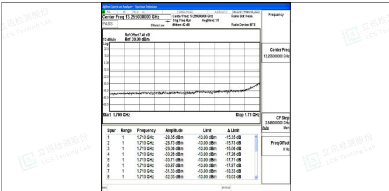
Band4_3MHz_QPSK_19965_15RB#0
