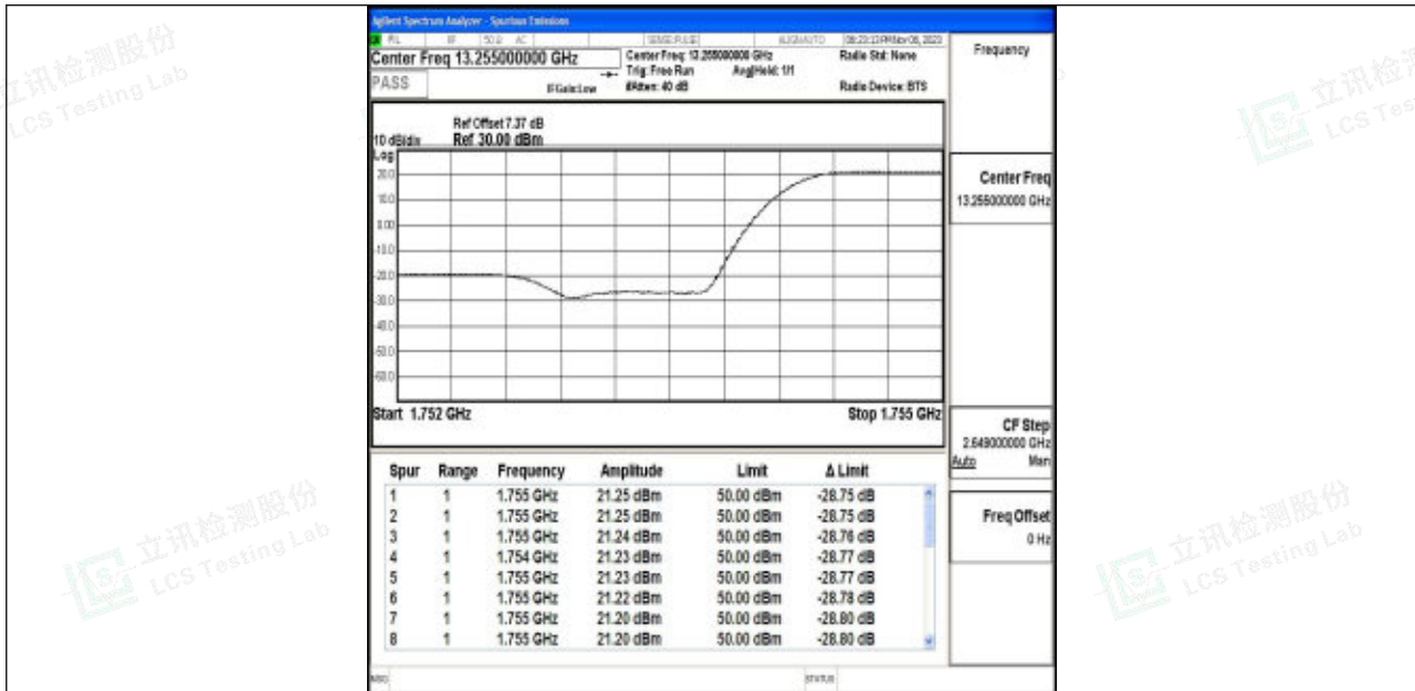
Band4_3MHz_64QAM_20385_1RB#14
