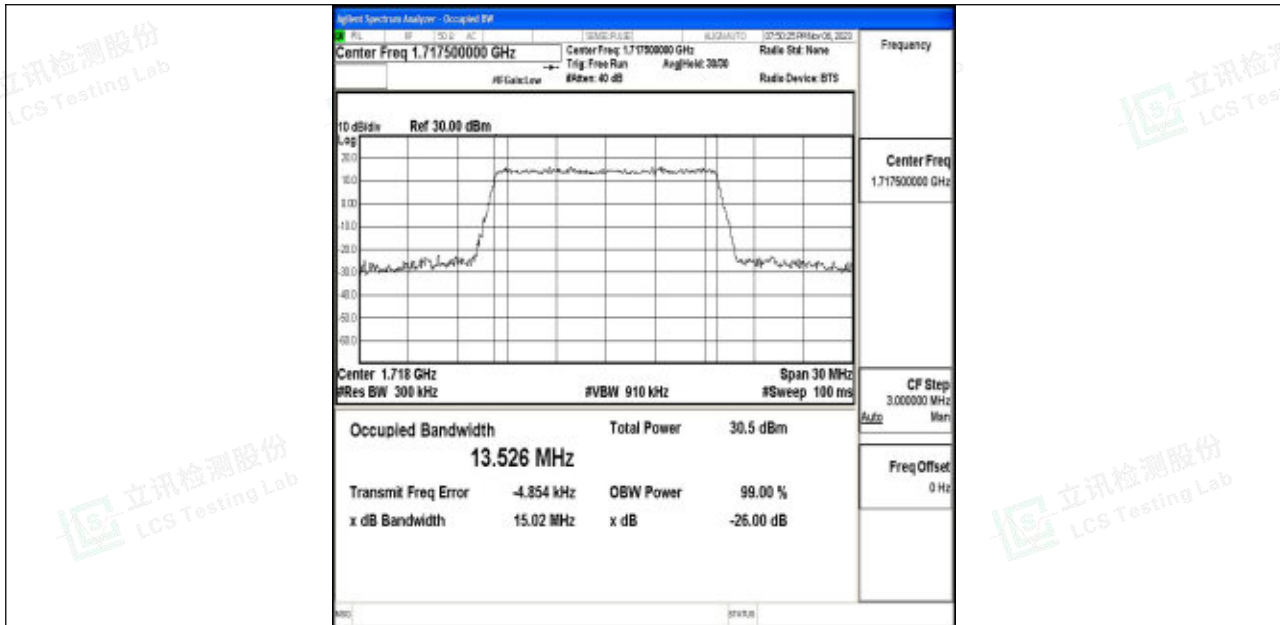
Band4-15MHz-QPSK-20025-75RB#0-PASS
