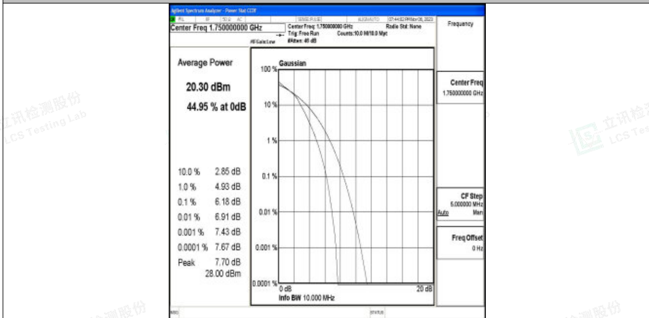
Band4-10MHz-16QAM-20350-50RB#0-PASS
