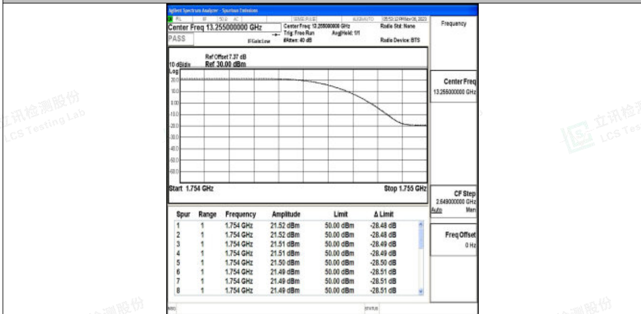
Band4_1.4MHz_QPSK_20393_1RB#0
