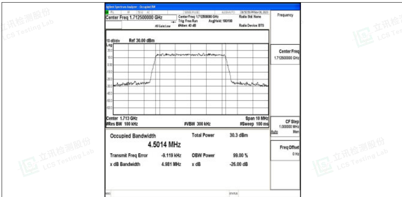
Band4-5MHz-64QAM-19975-25RB#0-PASS
