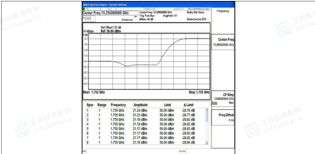
Band4_3MHz_QPSK_20385_1RB#14
