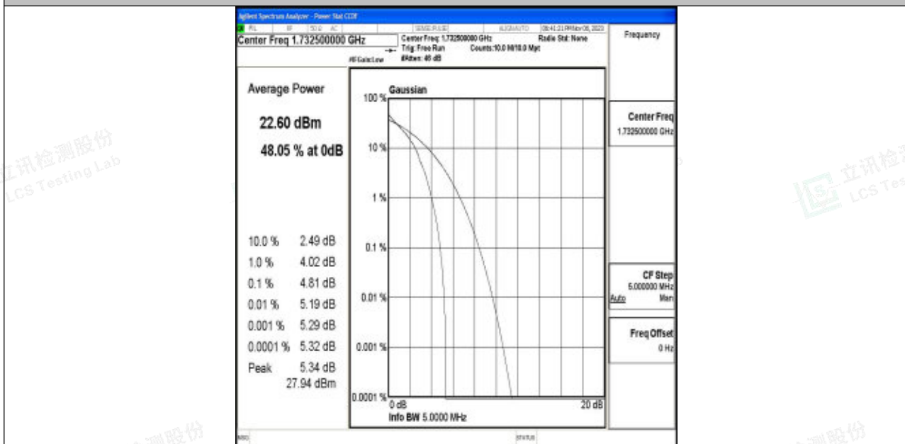
Band4-3MHz-QPSK-20175-1RB#0-PASS
