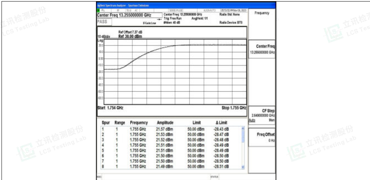
Band4_1.4MHz_64QAM_20393_1RB#5
