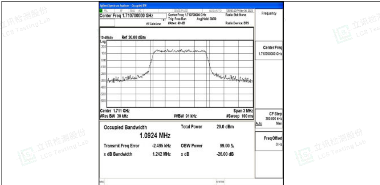
Band4-1.4MHz-64QAM-19957-6RB#0-PASS
