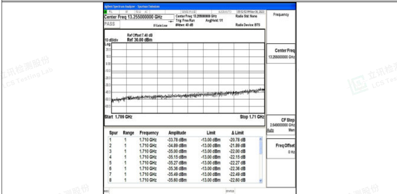
Band4_1.4MHz_16QAM_19957_6RB#0
