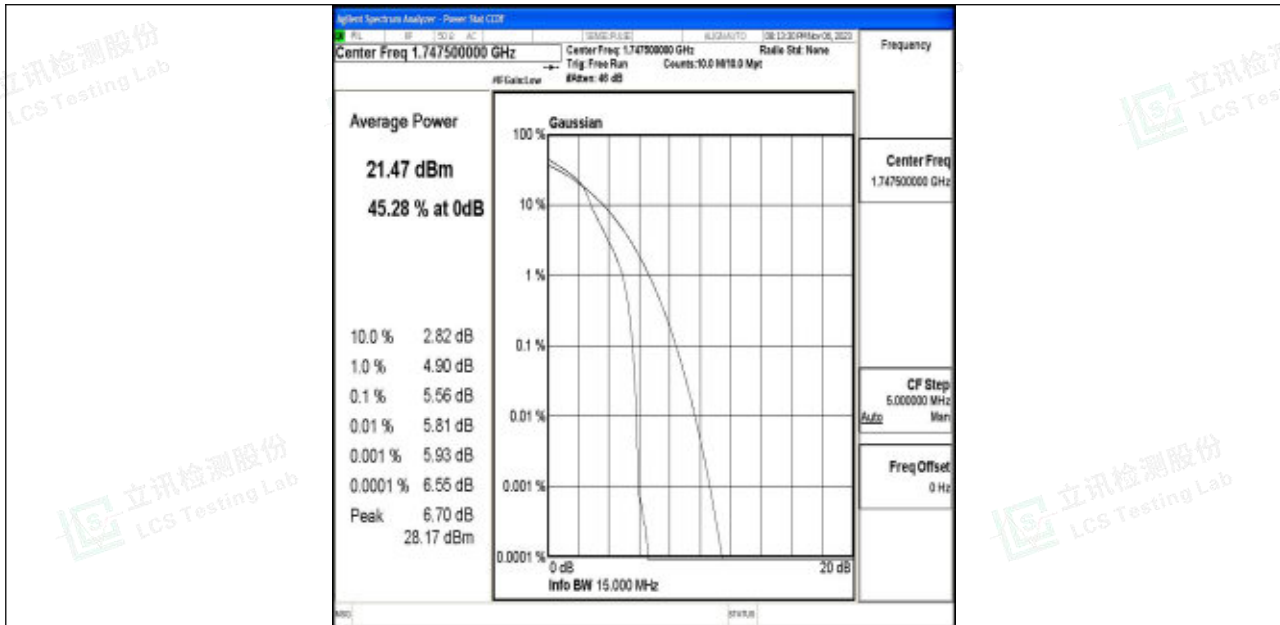
Band4-15MHz-16QAM-20325-1RB#0-PASS
