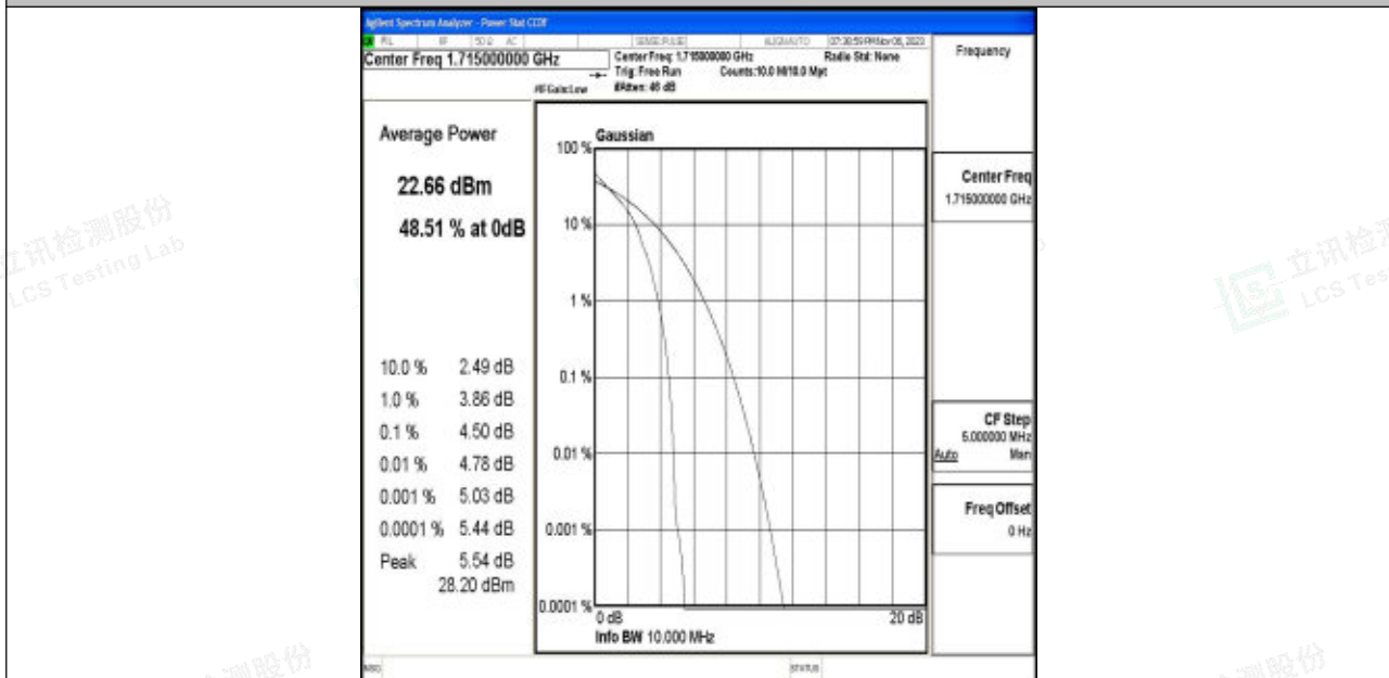
Band4-10MHz-64QAM-20000-1RB#0-PASS
