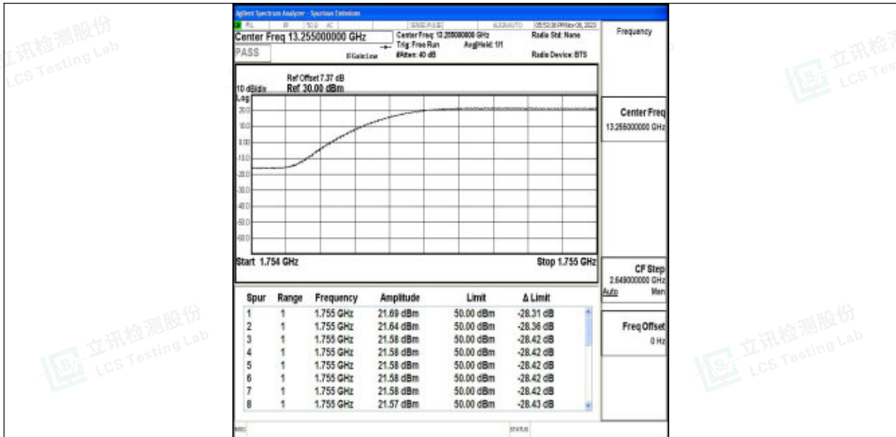
Band4_1.4MHz_QPSK_20393_1RB#5
