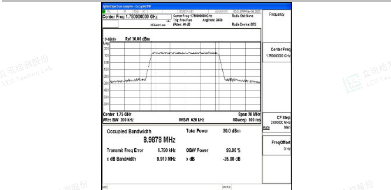
Band4-10MHz-64QAM-20350-50RB#0-PASS
