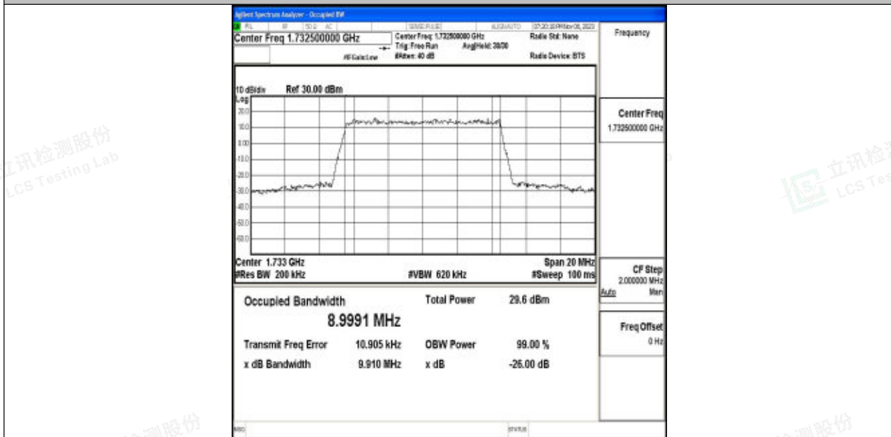
Band4-10MHz-16QAM-20175-50RB#0-PASS
