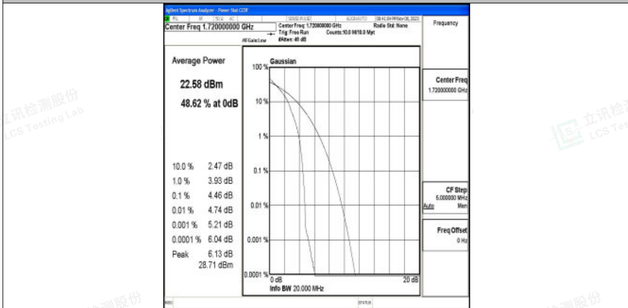
Band4-20MHz-64QAM-20050-1RB#0-PASS
