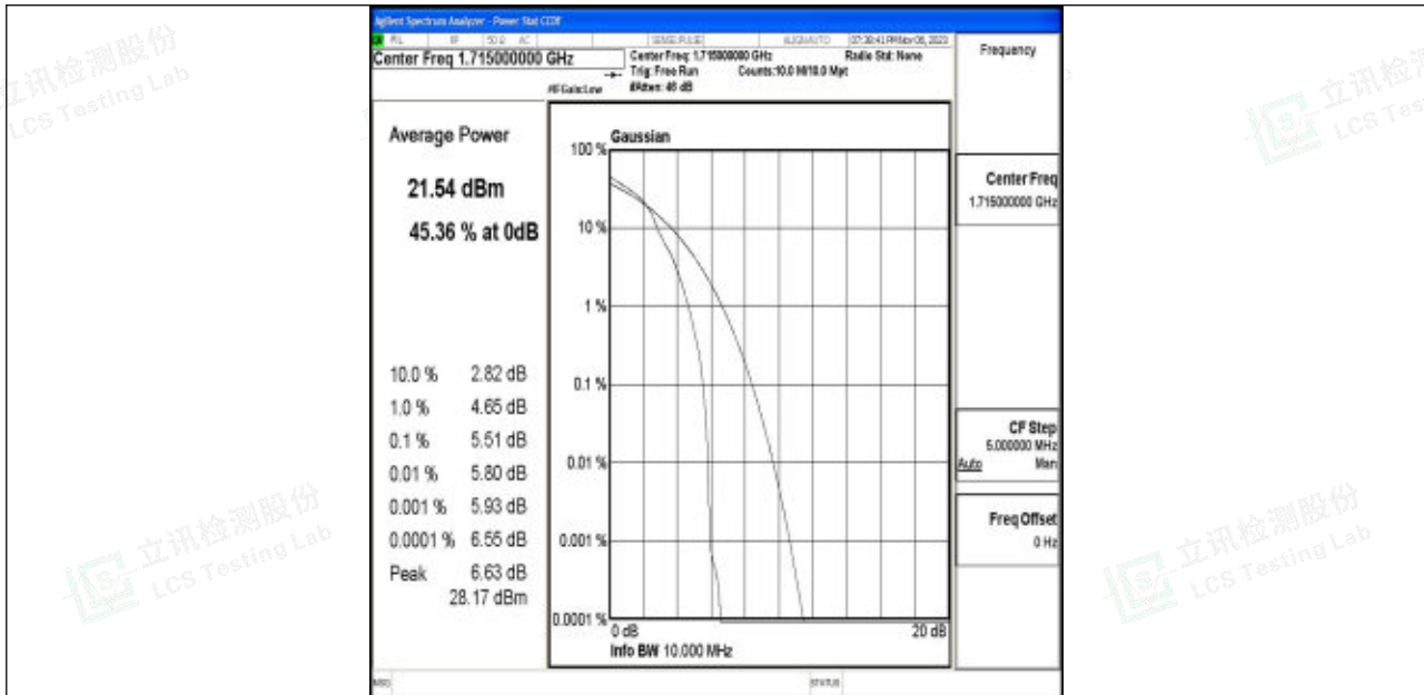
Band4-10MHz-16QAM-20000-1RB#0-PASS
