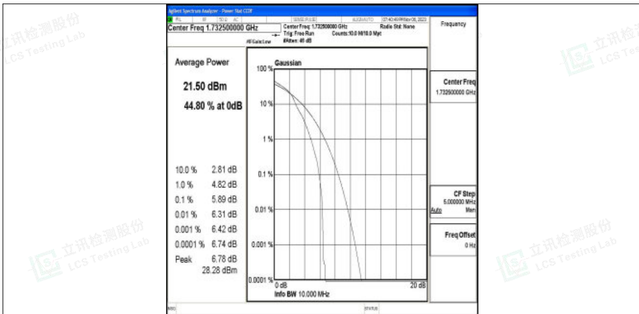
Band4-10MHz-16QAM-20175-1RB#0-PASS
