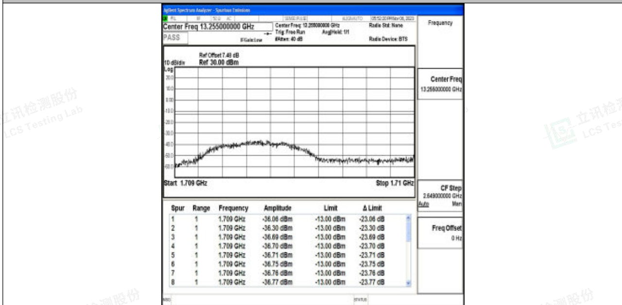
Band4_1.4MHz_QPSK_19957_1RB#5
