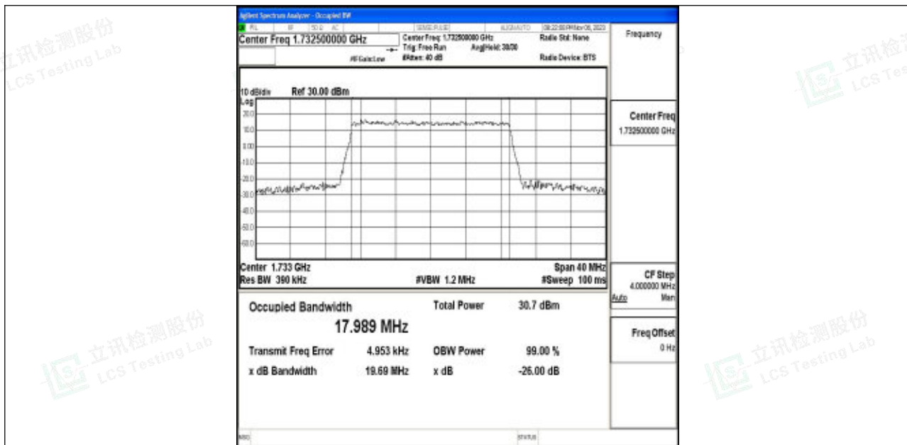
Band4-20MHz-64QAM-20175-100RB#0-PASS
