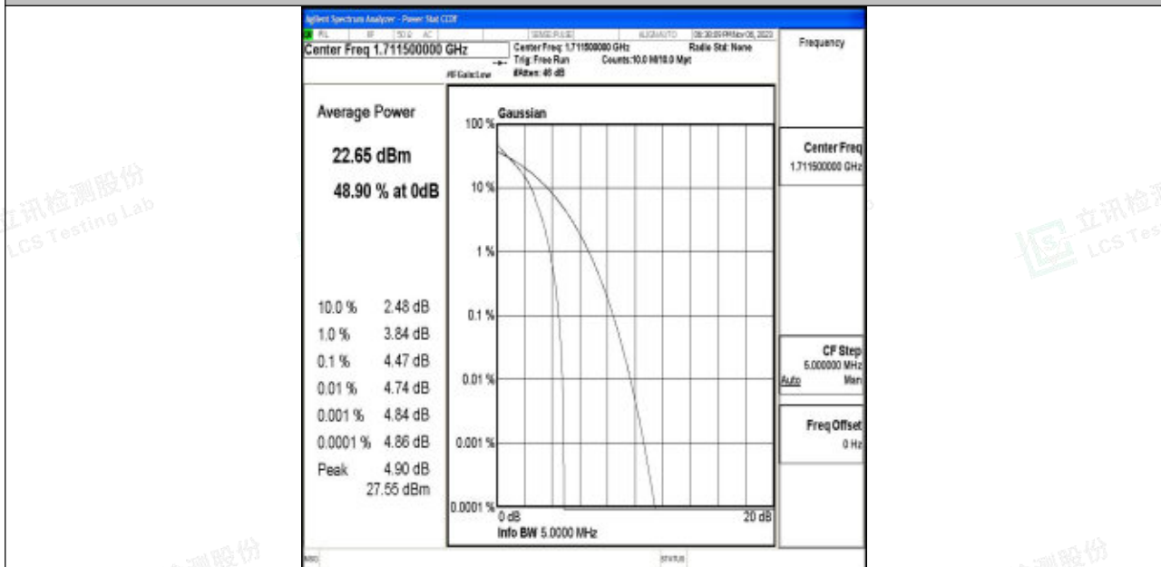
Band4-3MHz-QPSK-19965-1RB#0-PASS
