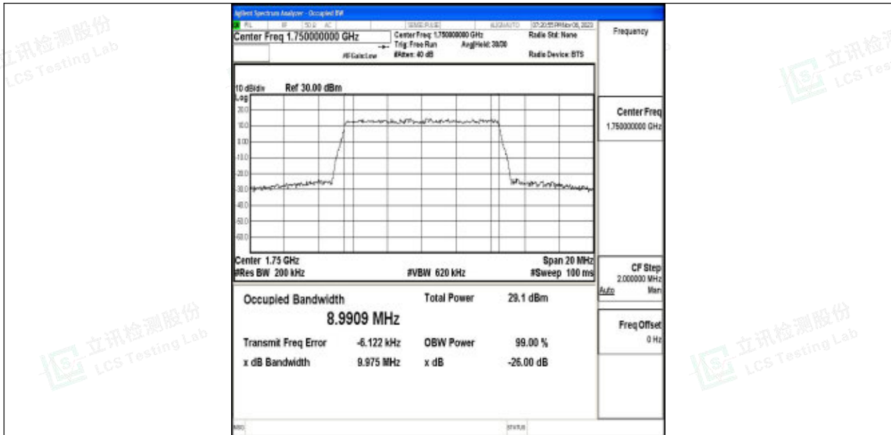
Band4-10MHz-16QAM-20350-50RB#0-PASS
