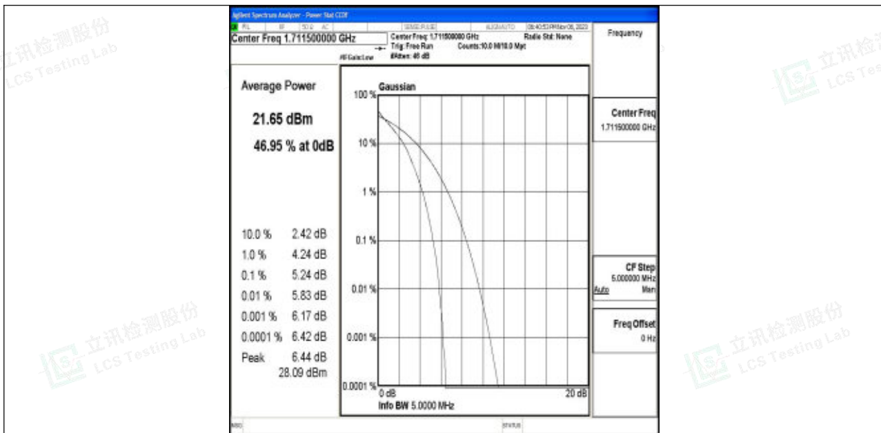
Band4-3MHz-64QAM-19965-15RB#0-PASS
