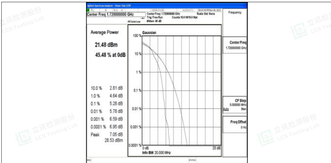
Band4-20MHz-16QAM-20050-1RB#0-PASS
