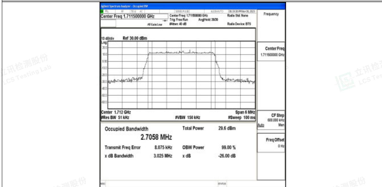
Band4-3MHz-64QAM-19965-15RB#0-PASS
