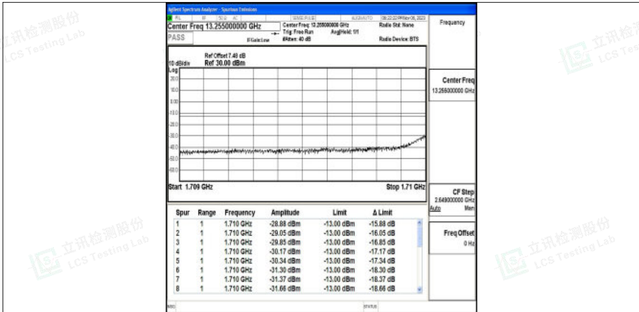
Band4_3MHz_64QAM_19965_15RB#0
