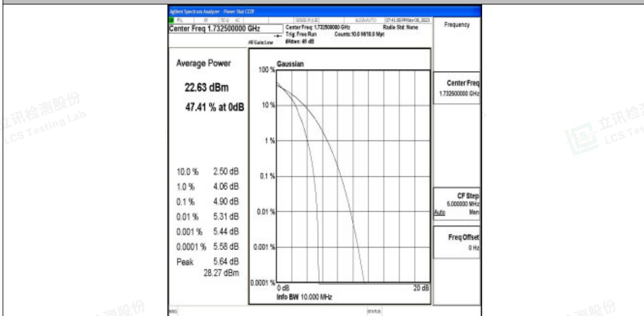
Band4-10MHz-64QAM-20175-1RB#0-PASS
