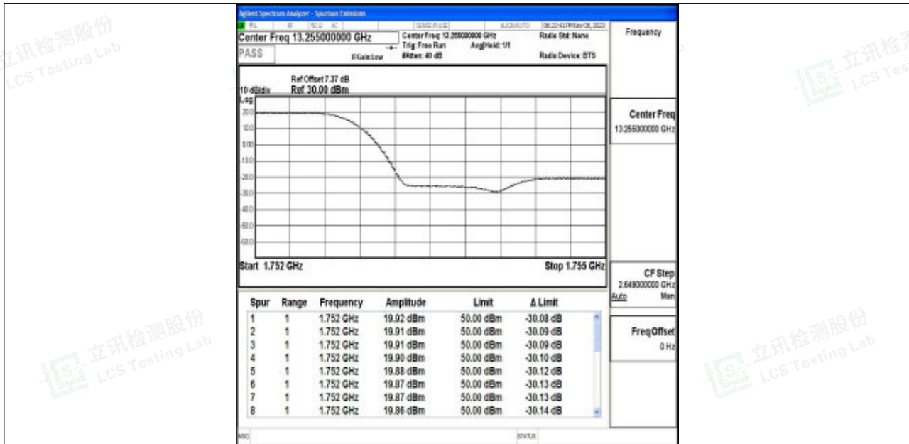
Band4_3MHz_16QAM_20385_1RB#0
