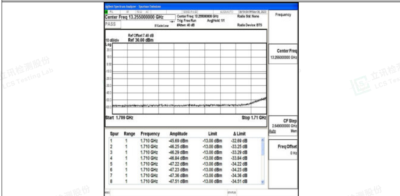
Band4_5MHz_QPSK_19975_1RB#24
