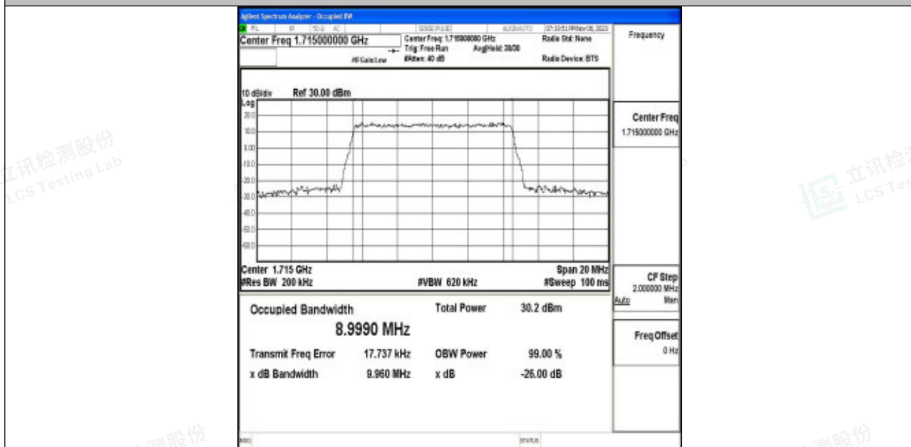
Band4-10MHz-64QAM-20000-50RB#0-PASS
