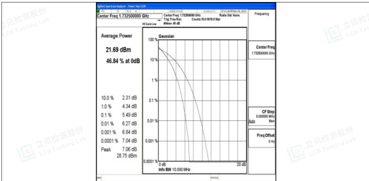
Band4-10MHz-QPSK-20175-50RB#0-PASS
